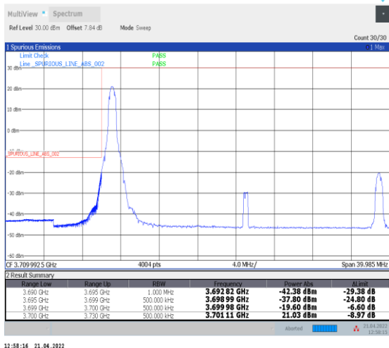
1-N78-3700-3800--30-30-L-1-DFT-PI2BPSK-Edge_1R_B_Left-1@0-Ant0-PASS-see graph
