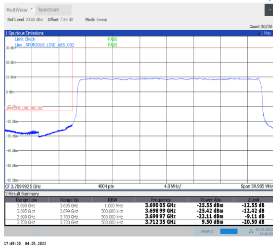
1-N78-3700-3800--30-30-L-3-DFT-PI2BPSK-Outer_Full-75@0-Ant0-PASS-see graph
