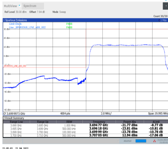
1-N78-3700-3800--30-10-L-3-DFT-PI2BPSK-Outer _Full-24@0-Ant0-PASS-see graph
