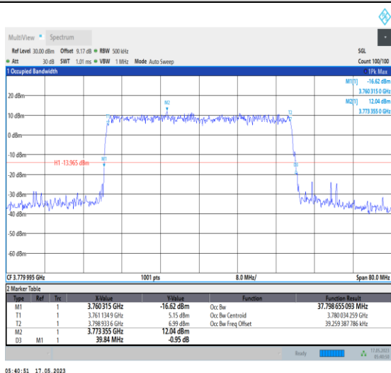
1-N78-3700-3800-PC1-30-40-H-9-CP-256QAM-Oute r Full-106@0-Ant0-37.799-39.840-≤40-PASS
