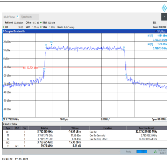
1-N78-3700-3800-PC1-30-40-H-7-CP-16QAM-Outer Full-106@0-Ant0-37.775-39.760-≤40-PASS
