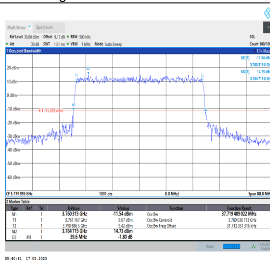
1-N78-3700-3800-PC1-30-40-H-8-CP-64QAM-Outer Full-106@0-Ant0-37.719-39.600-≤40-PASS
