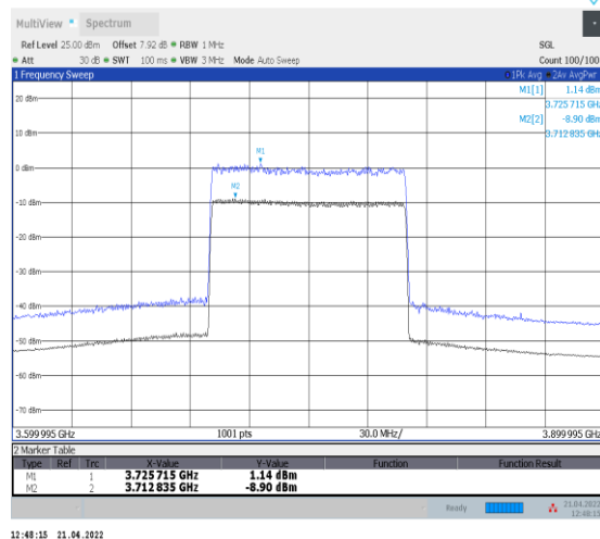
1-N78-3700-3800--30-100-M-2-CP-256QAM-Outer_Full-273@0-Ant0-10.04-100%-0.00-10.04-PASS-≤13
