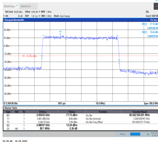
1-N78-3450-3550-PC1-30-90-H-5-DFT-256QAM-Oute_r_Full-240@0-Ant0-85.503-89.100-≤90-PASS
