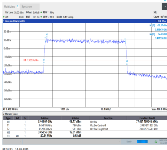
1-N78-3450-3550-PC1-30-80-L-9-CP-256QAM-Outer_Full-217@0-Ant0-77.451-80.640-≤80-PASS
