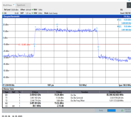
1-N78-3450-3550-PC1-30-90-H-4-DFT-64QAM-Oute_r_Full-240@0-Ant0-85.59-89.100-≤90-PASS
