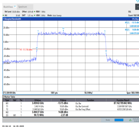
1-N78-3450-3550-PC1-30-90-H-7-CP-16QAM-Outer_Full-245@0-Ant0-87.163-90.720-≤90-PASS
