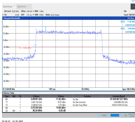
1-N78-3450-3550-PC1-30-90-H-6-CP-QPSK-Outer_Full-245@0-Ant0-87.453-90.540-≤90-PASS
