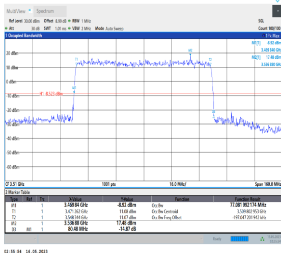
1-N78-3450-3550-PC1-30-80-H-3-DFT-16QAM-Oute_r_Full-216@0-Ant0-77.082-80.480-≤80-PASS
