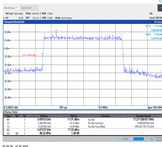
1-N78-3450-3550-PC1-30-80-M-3-DFT-16QAM-Outer_Full-216@0-Ant0-77.212-80.320-≤80-PASS
