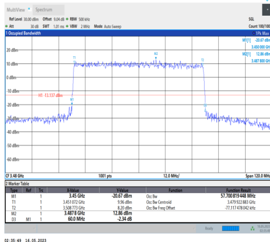
1-N78-3450-3550-PC1-30-60-L-8-CP-64QAM-Outer_Full-162@0-Ant0-57.701-60.000-≤60-PASS
