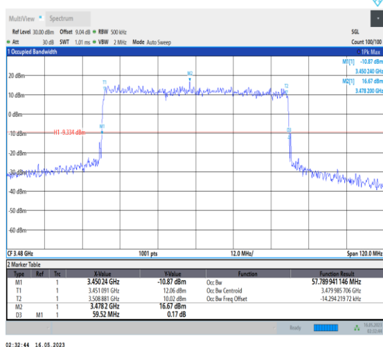
1-N78-3450-3550-PC1-30-60-L-1-DFT-QPSK-Outer_Full-162@0-Ant0-57.79-59.520-≤60-PASS
