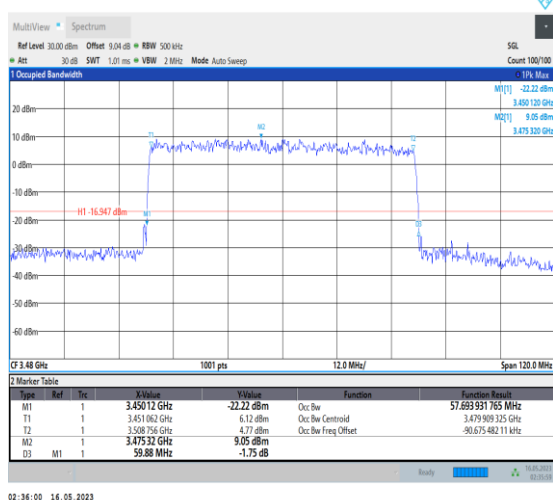
1-N78-3450-3550-PC1-30-60-L-9-CP-256QAM-Outer_Full-162@0-Ant0-57.694-59.880-≤60-PASS
