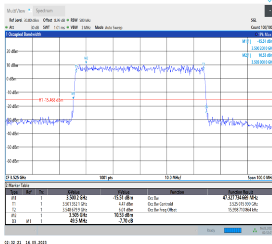
1-N78-3450-3550-PC1-30-50-H-9-CP-256QAM-Outer_Full-133@0-Ant0-47.328-49.500-≤50-PASS
