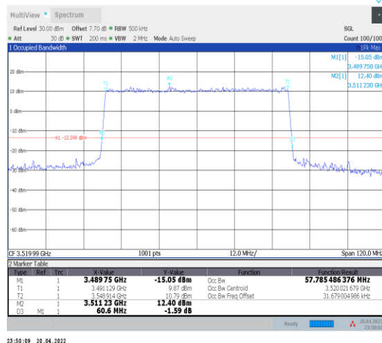
1-N78-3450-3550--30-60-H-6-CP-QPSK-Outer_Full- 162@0-Ant0-57.785-60.600-≤60-PASS
