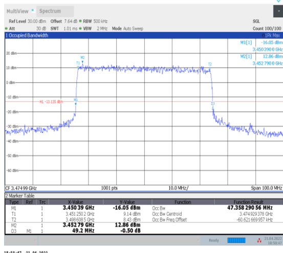
1-N78-3450-3550--30-50-L-6-CP-QPSK-Outer_Full-1 33@0-Ant0-47.358-49.200-≤50-PASS
