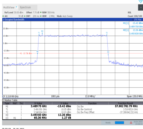
1-N78-3450-3550--30-60-H-7-CP-16QAM-Outer_Full -162@0-Ant0-57.903-60.360-≤60-PASS
