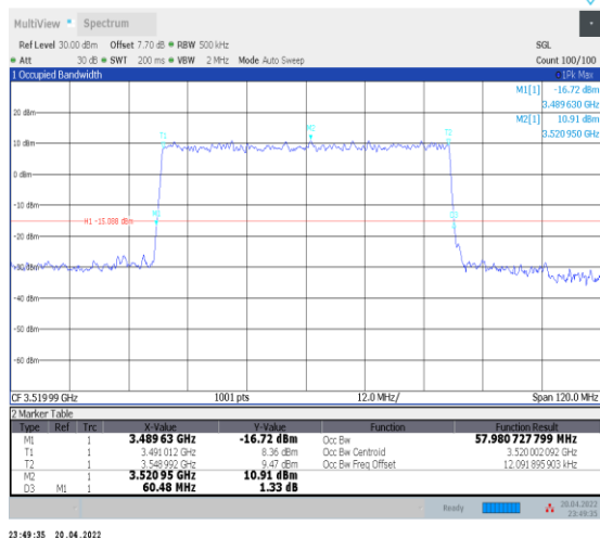
1-N78-3450-3550--30-60-H-5-DFT-256QAM-Outer_F ull-162@0-Ant0-57.981-60.480-≤60-PASS
