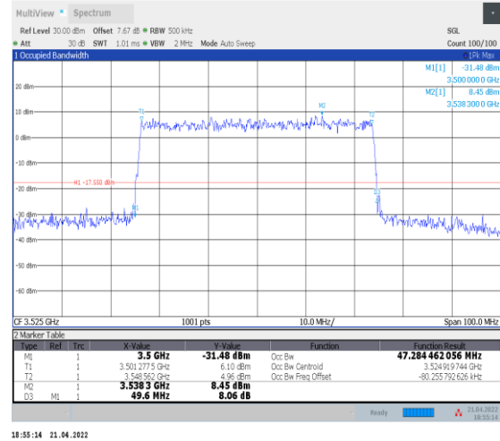
1-N78-3450-3550--30-50-H-9-CP-256QAM-Outer_F ull-133@0-Ant0-47.284-49.600-≤50-PASS
