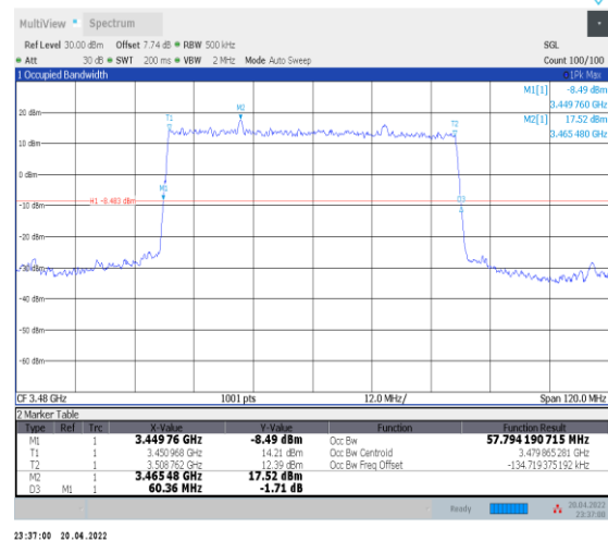
1-N78-3450-3550--30-60-L-2-DFT-PI2BPSK-Outer_ Full-162@0-Ant0-57.794-60.360-≤60-PASS
