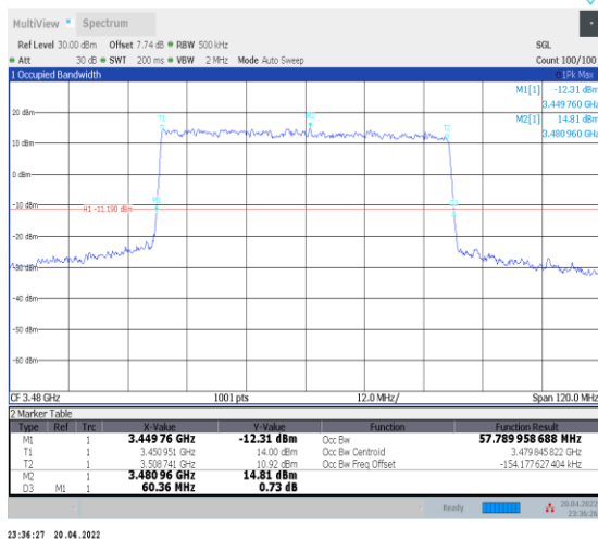
1-N78-3450-3550--30-60-L-1-DFT-QPSK-Outer_Full- 162@0-Ant0-57.79-60.360-≤60-PASS
