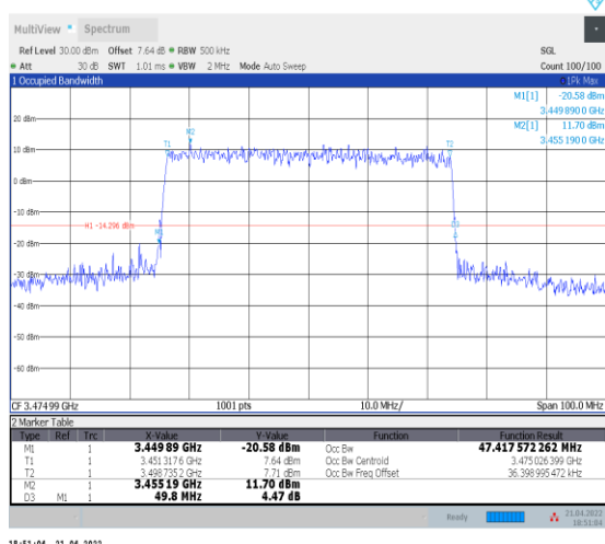
1-N78-3450-3550--30-50-L-8-CP-64QAM-Outer_Full -133@0-Ant0-47.418-49.800-≤50-PASS
