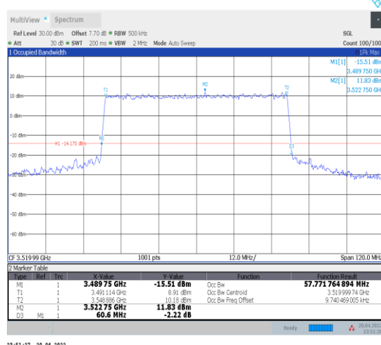
1-N78-3450-3550--30-60-H-8-CP-64QAM-Outer_Full -162@0-Ant0-57.772-60.600-≤60-PASS
