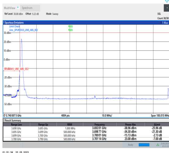
1-N77-3700-3980-PC1-30-90-L-4-CP-QPSK-Edge_1RB_Left-1@0-Ant0-1--PASS-see graph
