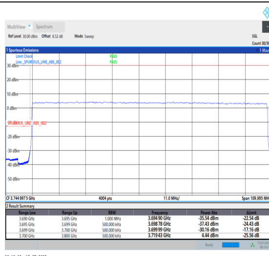
1-N77-3700-3980-PC1-30-100-L-3-DFT-PI2BPSK-Outer_Full-270@0-Ant0-1--PASS-see graph
