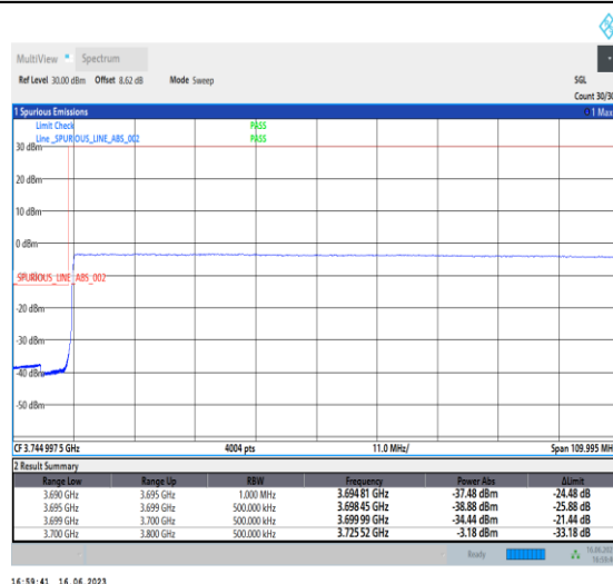
1-N77-3700-3980-PC1-30-100-L-6-CP-QPSK-Outer_Full-273@0-Ant0-1--PASS-see graph
