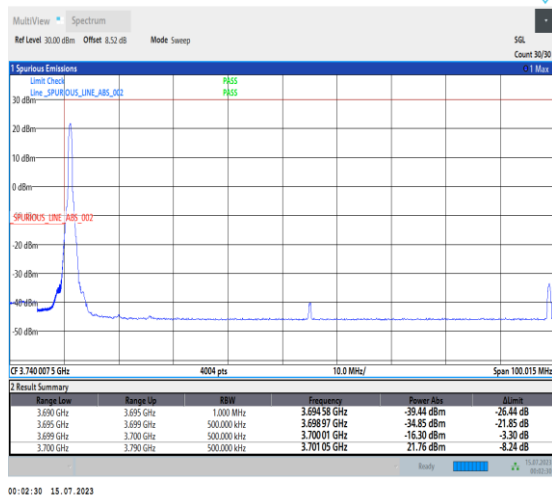
1-N77-3700-3980-PC1-30-90-L-1-DFT-PI2BPSK-Edg_e_1RB_Left-1@0-Ant0-1--PASS-see graph
