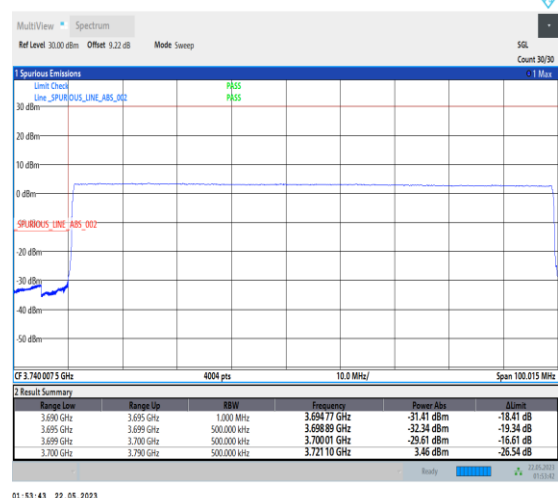
1-N77-3700-3980-PC1-30-90-L-6-CP-QPSK-Outer_Full-245@0-Ant0-1--PASS-see graph
