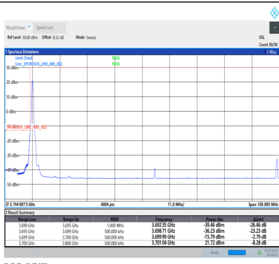
1-N77-3700-3980-PC1-30-100-L-1-DFT-PI2BPSK-Edge_1RB_Left-1@0-Ant0-1--PASS-see graph
