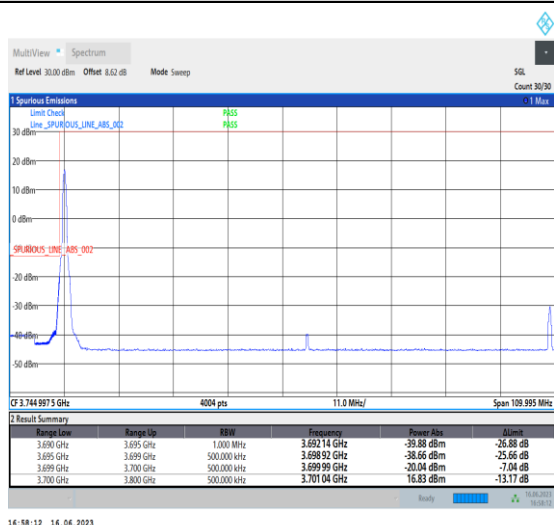
1-N77-3700-3980-PC1-30-100-L-4-CP-QPSK-Edge_1RB_Left-1@0-Ant0-1--PASS-see graph
