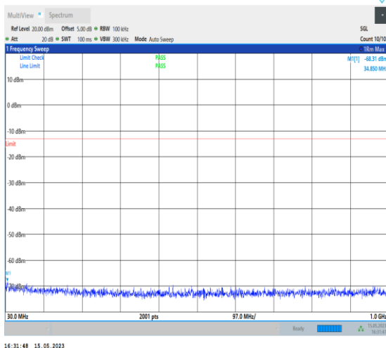
1-N77-3700-3980-PC1-30-100-L-1-DFT-PI2BPSK-In ner_1RB_Left-1@1-30-1000-Ant0-34.85--68.31--13- PASS
