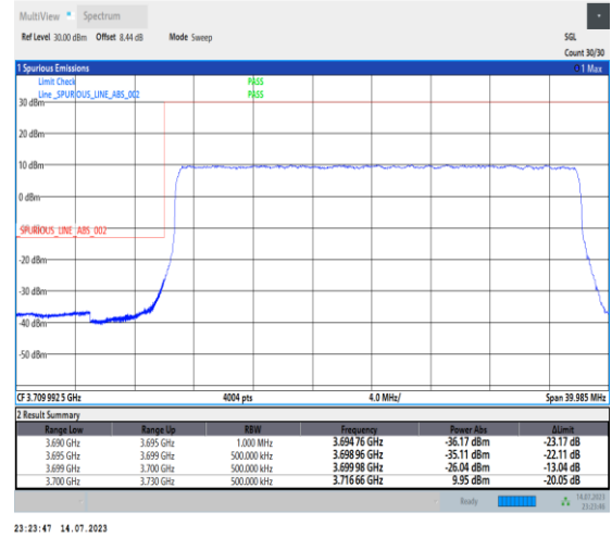
1-N77-3700-3980-PC1-30-30-L-3-DFT-PI2BPSK-Outer_Full-75@0-Ant0-1--PASS-see graph
