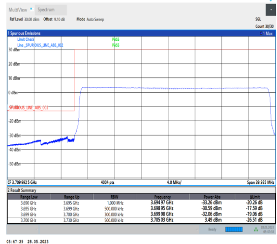
1-N77-3700-3980-PC1-30-30-L-6-CP-QPSK-Outer_Full-78@0-Ant0-1--PASS-see graph
