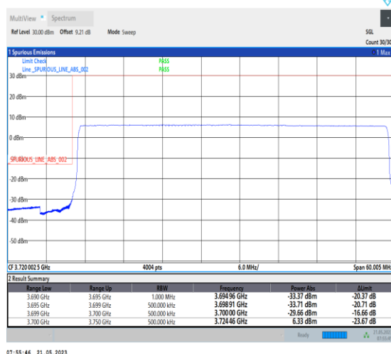
1-N77-3700-3980-PC1-30-50-L-6-CP-QPSK-Outer_Full-133@0-Ant0-1--PASS-see graph
