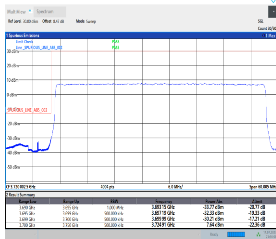
1-N77-3700-3980-PC1-30-50-L-3-DFT-PI2BPSK-Outer_Full-128@0-Ant0-1--PASS-see graph
