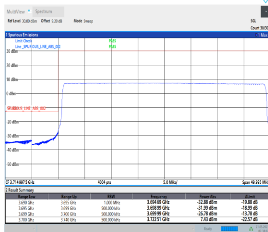
1-N77-3700-3980-PC1-30-40-L-6-CP-QPSK-Outer_Full-106@0-Ant0-1--PASS-see graph
