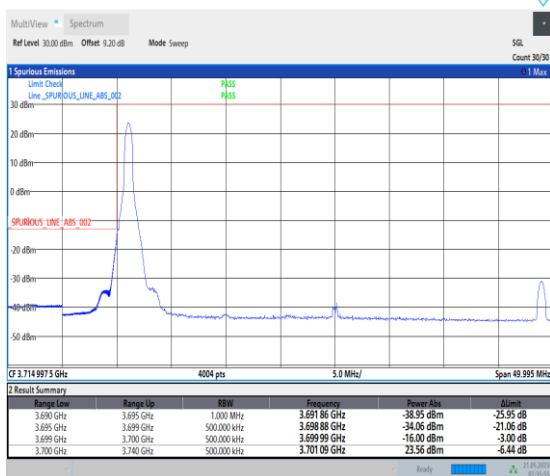
1-N77-3700-3980-PC1-30-40-L-4-CP-QPSK-Edge_1RB_Left-1@0-Ant0-1--PASS-see graph
