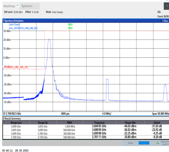
1-N77-3700-3980-PC1-30-30-L-4-CP-QPSK-Edge_1RB_Left-1@0-Ant0-1--PASS-see graph
