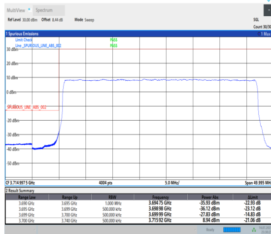
1-N77-3700-3980-PC1-30-40-L-3-DFT-PI2BPSK-Outer_Full-100@0-Ant0-1--PASS-see graph
