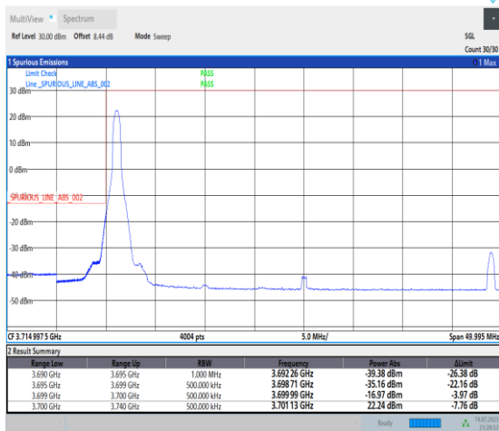
1-N77-3700-3980-PC1-30-40-L-1-DFT-PI2BPSK-Edg_e_1RB_Left-1@0-Ant0-1--PASS-see graph
