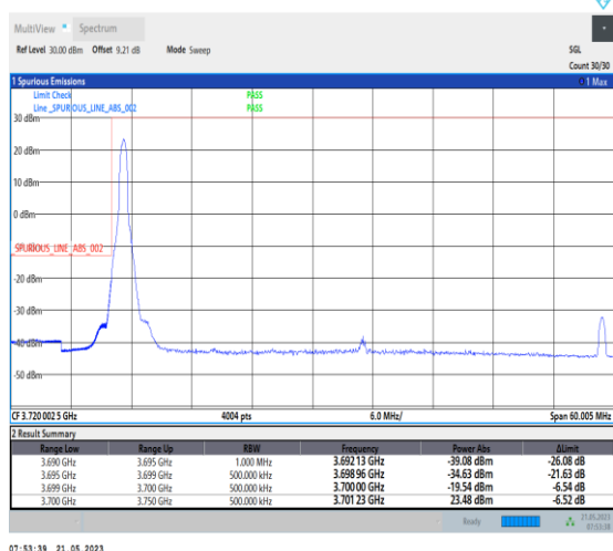
1-N77-3700-3980-PC1-30-50-L-4-CP-QPSK-Edge_1RB_Left-1@0-Ant0-1--PASS-see graph
