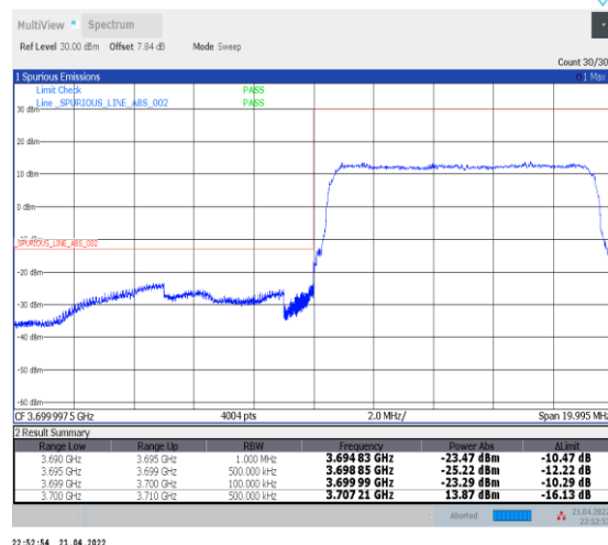
1-N77-3700-3980--30-10-L-3-DFT-PI2BPSK-Outer _Full-24@0-Ant0-PASS-see graph
