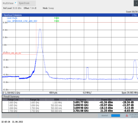
1-N77-3700-3980--30-30-L-1-DFT-PI2BPSK-Edge_1R B_Left-1@0-Ant0-PASS-see graph
