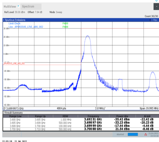
1-N77-3700-3980--30-10-L-4-CP-QPSK-Edge_1RB_L eft-1@0-Ant0-PASS-see graph
