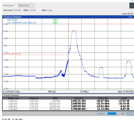
1-N77-3700-3980--30-10-L-1-DFT-PI2BPSK-Edge_1R B_Left-1@0-Ant0-PASS-see graph
