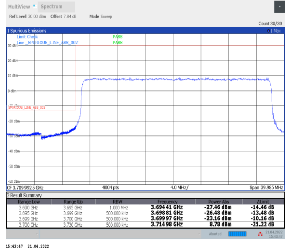
1-N77-3700-3980--30-30-L-3-DFT-PI2BPSK-Outer _Full-75@0-Ant0-PASS-see graph
