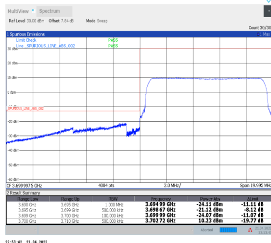
1-N77-3700-3980--30-10-L-6-CP-QPSK-Outer_Ful l-24@0-Ant0-PASS-see graph
