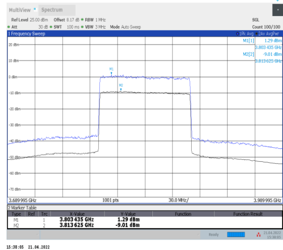
1-N77-3700-3980--30-100-M-2-CP-256QAM-Outer_Full-273@0-Ant0-10.30-100%-0.00-10.30-PASS-≤13
