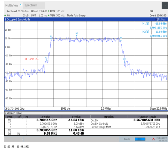
1-N77-3700-3980--30-10-L-4-DFT-64QAM-Outter_Full -24@0-Ant0-8.567-9.580-≤10-PASS
