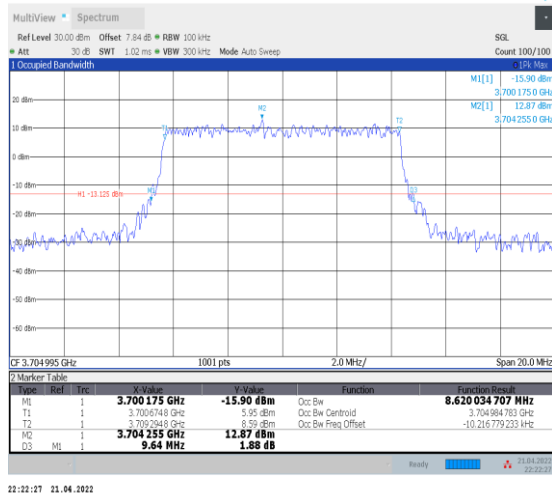
1-N77-3700-3980--30-10-L-3-DFT-16QAM-Outter_Full -24@0-Ant0-8.62-9.640-≤10-PASS
