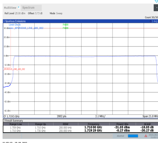
1-N66-PC3-15-20-L-6-CP-QPSK-Outer_Full-106@0-Ant0-seegraph-PASS-see graph
