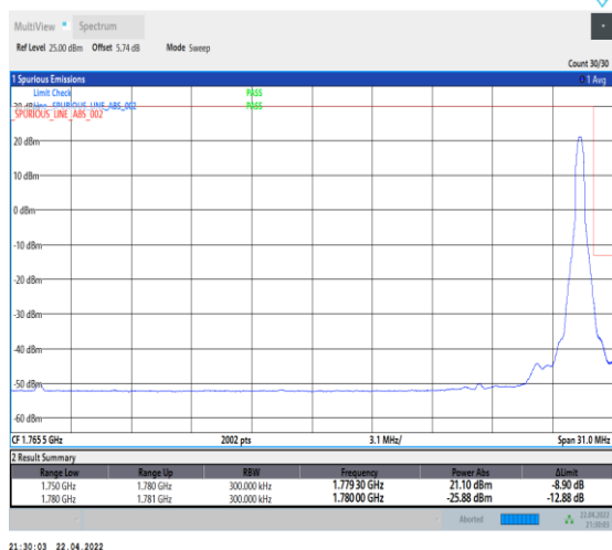
1-N66-PC3-15-30-H-2-DFT-PI2BPSK-Edge_1RB_Righ t-1@159-Ant0-seegraph-PASS-see graph
