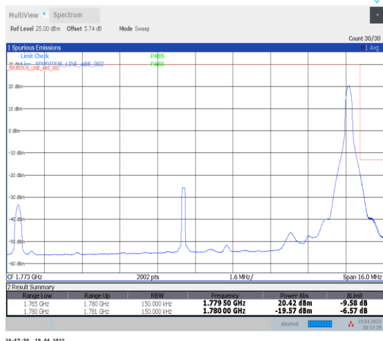
1-N66-PC3-15-15-H-2-DFT-PI2BPSK-Edge_1RB_Right-t-1@78-Ant0-seegraph-PASS-see graph
