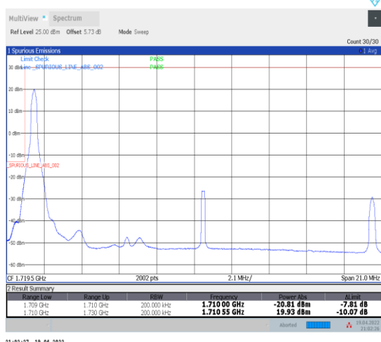
1-N66-PC3-15-20-L-4-CP-QPSK-Edge_1RB_Left-1@0-Ant0-seegraph-PASS-see graph
