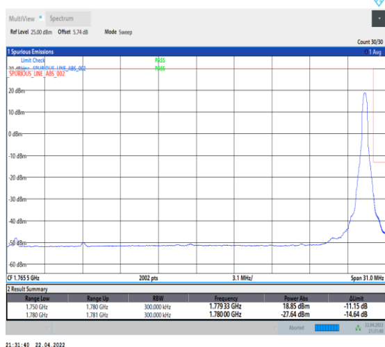
1-N66-PC3-15-30-H-5-CP-QPSK-Edge_1RB_Right-1 @159-Ant0-seegraph-PASS-see graph
