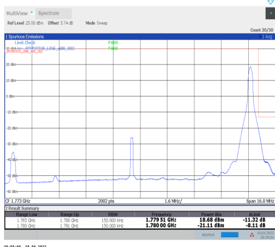
1-N66-PC3-15-15-H-5-CP-QPSK-Edge_1RB_Right-1@78-Ant0-seegraph-PASS-see graph
