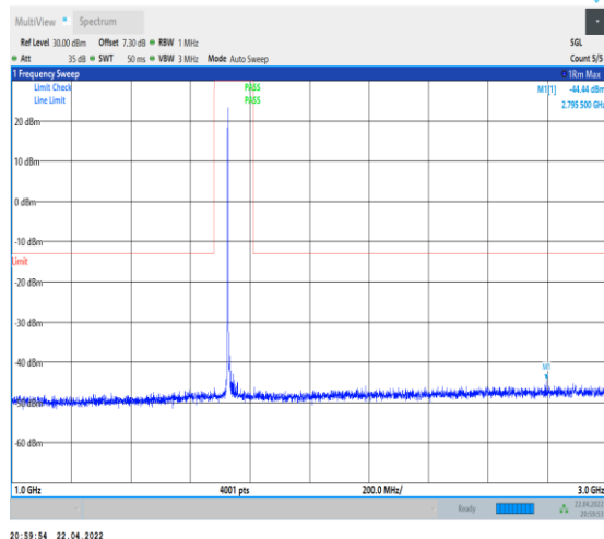
1-N66-PC3-15-40-M-1-DFT-PI2BPSK-Inner_1RB_Le ft-1@1-1000-3000-Ant0--44.44--13-PASS
