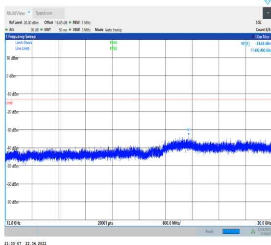
1-N66-PC3-15-40-M-1-DFT-PI2BPSK-Inner_1RB_Le ft-1@1-12000-20000-Ant0--33.38--13-PASS
