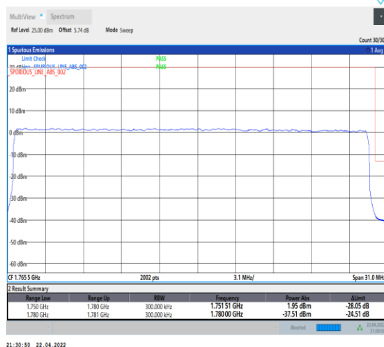
1-N66-PC3-15-30-H-3-DFT-PI2BPSK-Outer_Full-1 60@0-Ant0-seegraph-PASS-see graph
