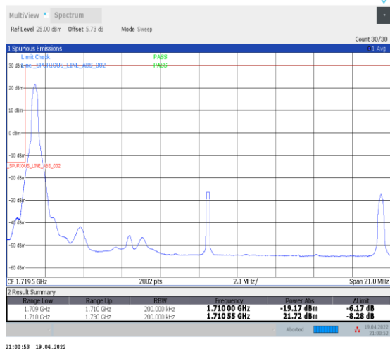
1-N66-PC3-15-20-L-1-DFT-PI2BPSK-Edge_1RB_Left-1@0-Ant0-seegraph-PASS-see graph
