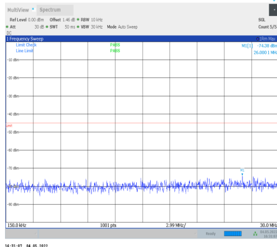
1-N41--30-100-L-1-DFT-PI2BPSK-Inner_1RB_Left-1 @1-0.15-30-Ant0--74.38--45-PASS
