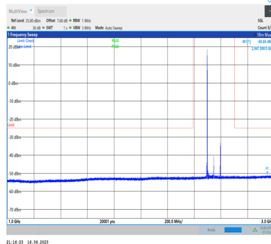
1-N41-PC1-30-100-L-1-DFT-QPSK-Edge_1RB_Left- 1@0-1000-3000-Ant0-2947.30--50.63--25-PASS
