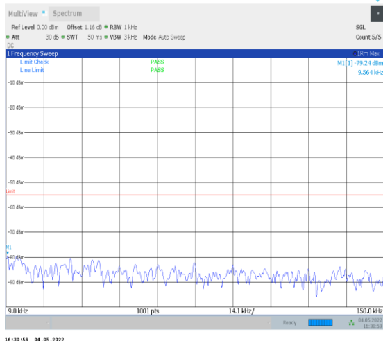
1-N41--30-100-L-1-DFT-PI2BPSK-Inner_1RB_Left-1 @1-0.009-0.15-Ant0--79.24--55-PASS
