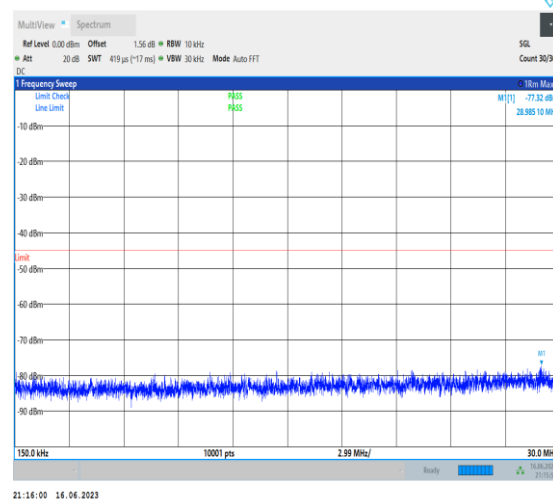
1-N41-PC1-30-100-L-1-DFT-QPSK-Edge_1RB_Left- 1@0-0.15-30-Ant0-28.99--77.32--45-PASS
