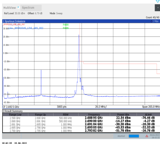
1-N41--30-100-H-5-CP-QPSK-Edge_1RB_Right-1@27 2-Ant0-PASS-see graph
