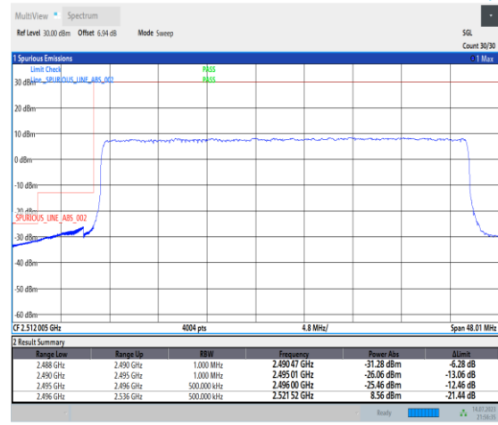
1-N41-PC1-30-40-L-3-DFT-PI2BPSK-Outer_Full-100@0-Ant0-1--PASS-see graph
