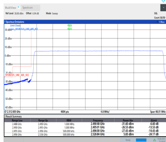
1-N41-PC1-30-40-L-6-CP-QPSK-Outer_Full-106@0-Ant0-1--PASS-see graph
