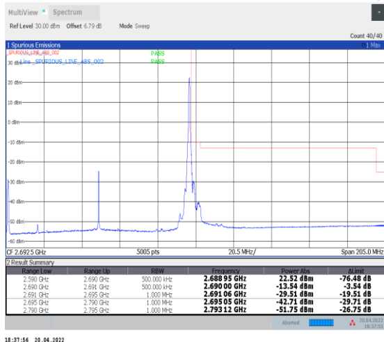
1-N41--30-100-H-2-DFT-PI2BPSK-Edge_1RB_Right-1 @272-Ant0-PASS-see graph
