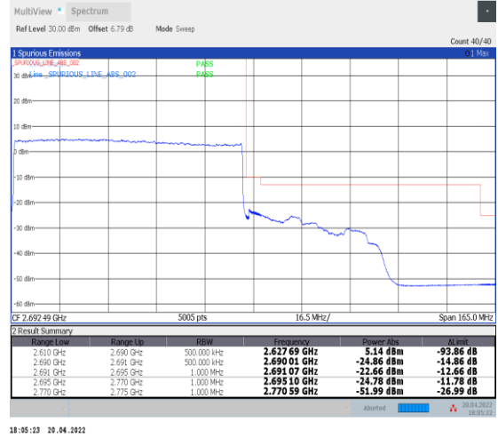
1-N41--30-80-H-3-DFT-PI2BPSK-Outer_Full-216 @0-Ant0-PASS-see graph
