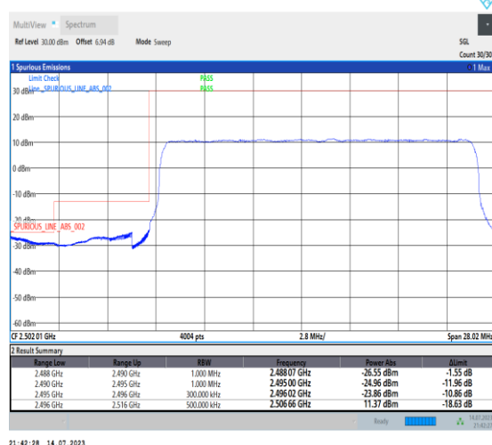
1-N41-PC1-30-20-L-3-DFT-PI2BPSK-Outer_Full-50@0-Ant0-1--PASS-see graph
