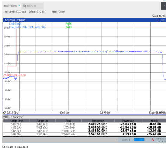
1-N41--30-90-L-3-DFT-PI2BPSK-Outer_Full-240@0-Ant0-PASS-see graph
