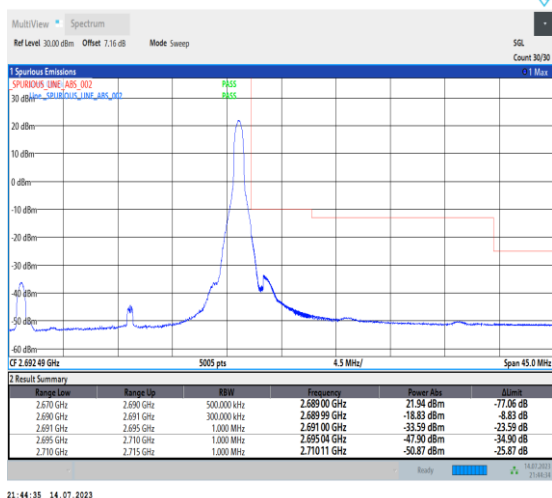
1-N41-PC1-30-20-H-2-DFT-PI2BPSK-Edge_1RB_Righ t-1@50-Ant0-1--PASS-see graph
