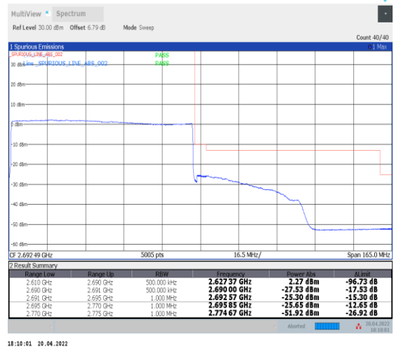
1-N41--30-80-H-6-CP-QPSK-Outer_Full-217@0-A nt0-PASS-see graph
