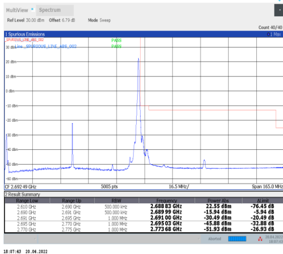
1-N41--30-80-H-5-CP-QPSK-Edge_1RB_Right-1@216 -Ant0-PASS-see graph
