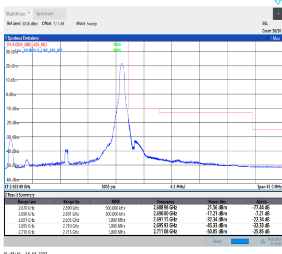
1-N41-PC1-30-20-H-5-CP-QPSK-Edge_1RB_Right-1 @50-Ant0-1--PASS-see graph
