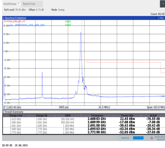
1-N41--30-80-H-2-DFT-PI2BPSK-Edge_1RB_Right-1@ 216-Ant0-PASS-see graph
