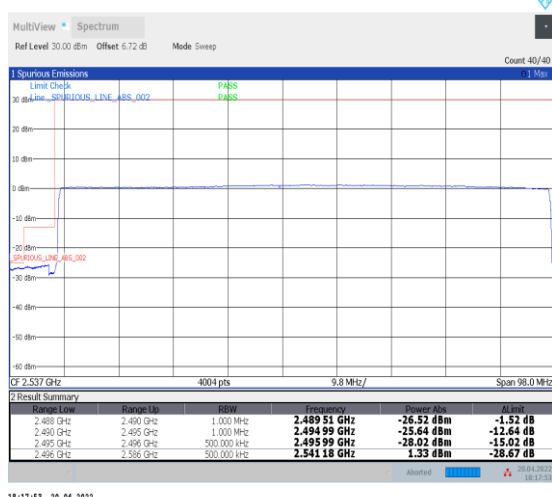
1-N41--30-90-L-6-CP-QPSK-Outer_Full-245@0-Ant0-PASS-see graph
