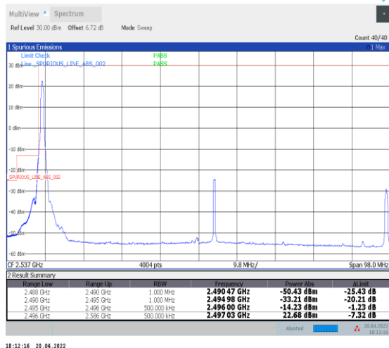
1-N41--30-90-L-1-DFT-PI2BPSK-Edge_1RB_Left-1@0-Ant0-PASS-see graph
