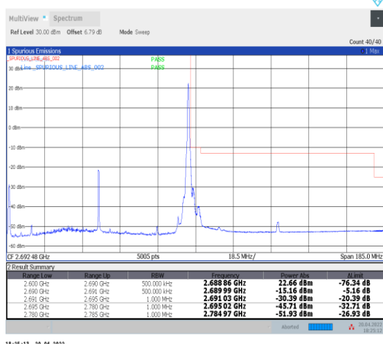
1-N41--30-90-H-5-CP-QPSK-Edge_1RB_Right-1@244 -Ant0-PASS-see graph
