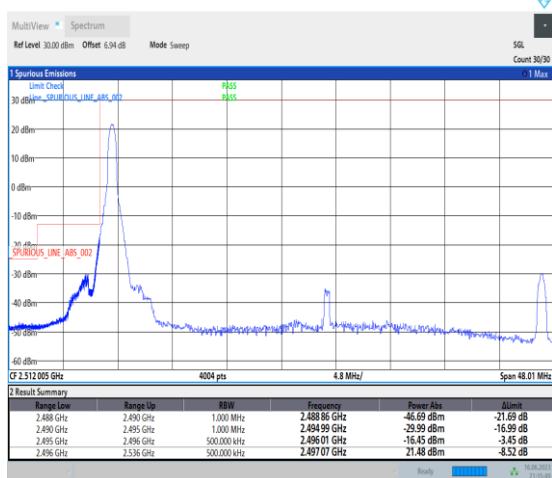
1-N41-PC1-30-40-L-4-CP-QPSK-Edge_1RB_Left-1@0-Ant0-1--PASS-see graph
