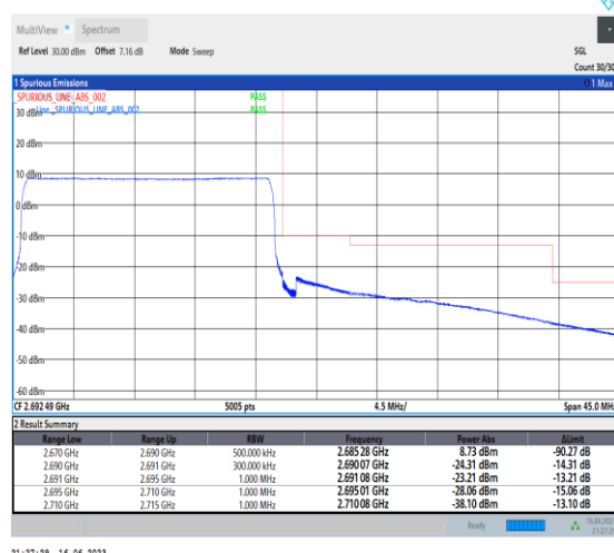
1-N41-PC1-30-20-H-6-CP-QPSK-Outer_Full-51@ 0-Ant0-1--PASS-see graph
