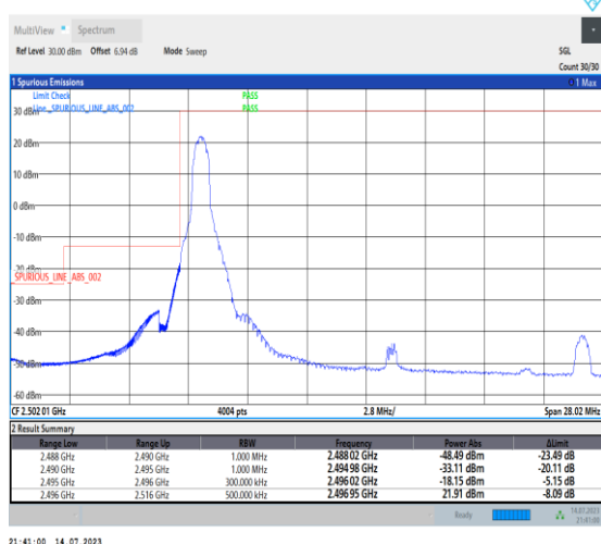
1-N41-PC1-30-20-L-1-DFT-PI2BPSK-Edge_1RB_Left-1@0-Ant0-1--PASS-see graph
