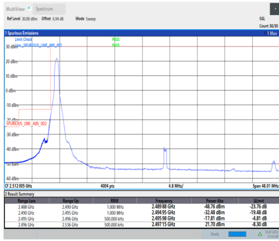
1-N41-PC1-30-40-L-1-DFT-PI2BPSK-Edge_1RB_Left-1@0-Ant0-1--PASS-see graph
