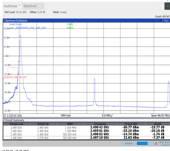
1-N41--30-80-L-1-DFT-PI2BPSK-Edge_1RB_Left-1@0-Ant0-PASS-see graph
