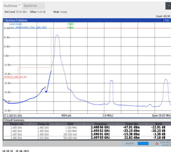
1-N41--30-20-L-1-DFT-PI2BPSK-Edge_1RB_Left-1@0-Ant0-PASS-see graph
