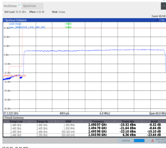
1-N41--30-60-L-3-DFT-PI2BPSK-Outer_Full-162@0-Ant0-PASS-see graph
