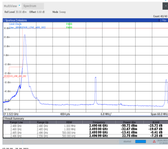
1-N41--30-60-L-1-DFT-PI2BPSK-Edge_1RB_Left-1@0-Ant0-PASS-see graph
