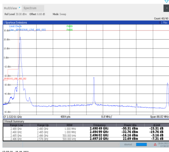
1-N41--30-80-L-4-CP-QPSK-Edge_1RB_Left-1@0-Ant0-PASS-see graph
