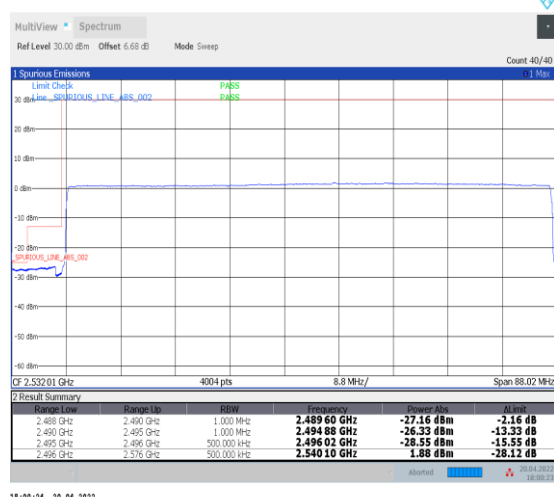
1-N41--30-80-L-6-CP-QPSK-Outer_Full-217@0-Ant0-PASS-see graph
