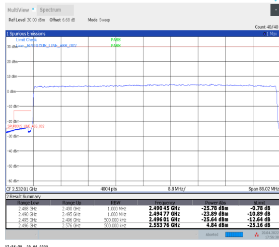
1-N41--30-80-L-3-DFT-PI2BPSK-Outer_Full-216@0-Ant0-PASS-see graph
