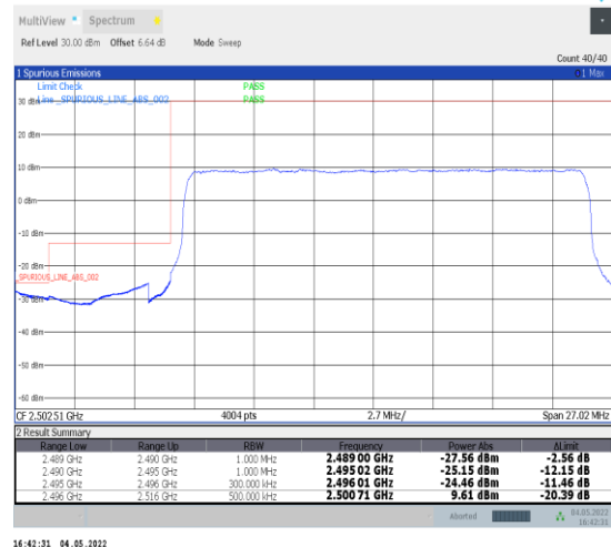
1-N41--30-20-L-3-DFT-PI2BPSK-Outer_Full-50@0-Ant0-PASS-see graph
