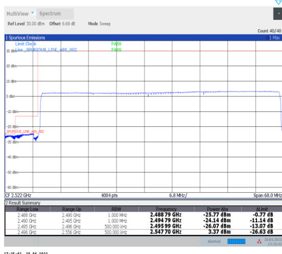
1-N41--30-60-L-6-CP-QPSK-Outer_Full-162@0-Ant0-PASS-see graph
