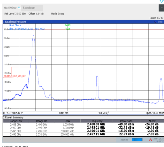
1-N41--30-40-L-4-CP-QPSK-Edge_1RB_Left-1@0-Ant0-PASS-see graph
