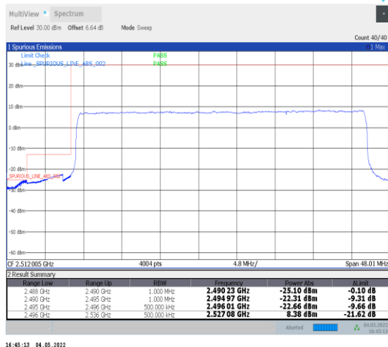
1-N41--30-40-L-3-DFT-PI2BPSK-Outer_Full-100@0-Ant0-PASS-see graph
