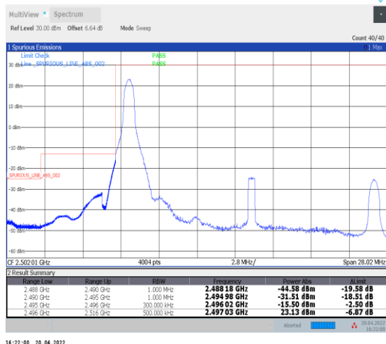
1-N41--30-20-L-4-CP-QPSK-Edge_1RB_Left-1@0-Ant0-PASS-see graph
