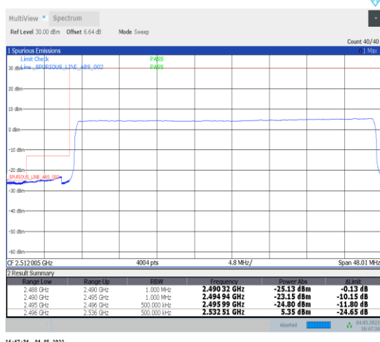
1-N41--30-40-L-6-CP-QPSK-Outer_Full-106@0-Ant0-PASS-see graph
