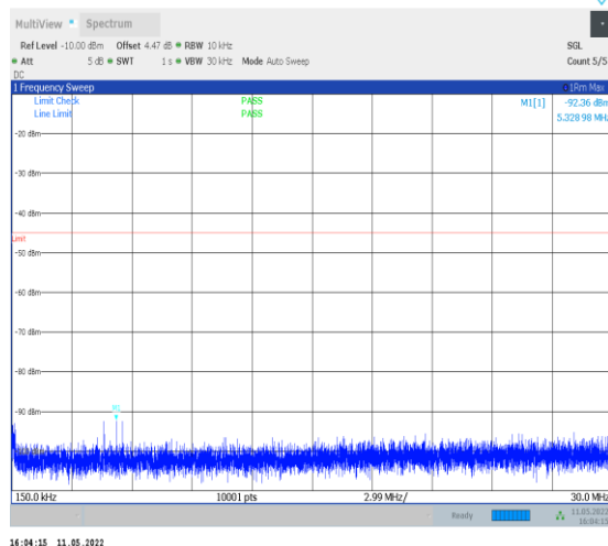
1-N38-PC2-30-40-M-1-DFT-QPSK-Edge_1RB_Left-1 @0-0.15-30-Ant0--92.36--45-PASS
