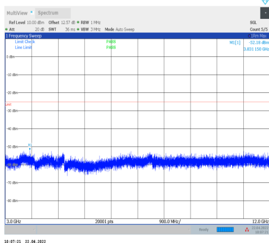
1-N38--30-40-M-1-DFT-PI2BPSK-Inner_1RB_Left-1 @1-3000-12000-Ant0--52.18--25-PASS
