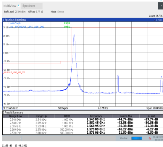
1-N38--30-40-L-4-CP-QPSK-Edge_1RB_Left-1@0-Ant0-PASS-see graph
