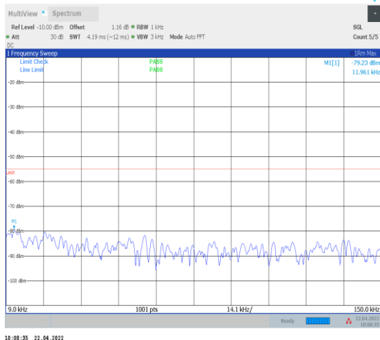
1-N38--30-40-H-1-DFT-PI2BPSK-Inner_1RB_Left-1 @1-0.009-0.15-Ant0--79.23--55-PASS
