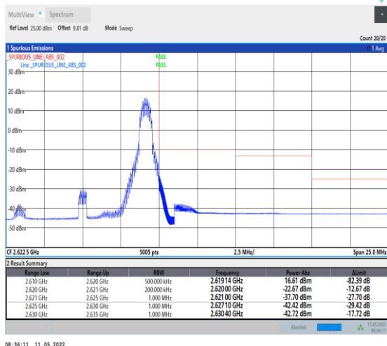
1-N38-PC2-30-10-H-5-CP-QPSK-Edge_1RB_Right-1@ 23-Ant0-PASS-see graph
