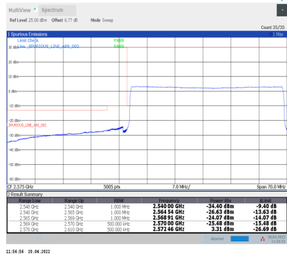
1-N38--30-40-L-6-CP-QPSK-Outer_Full-106@0-Ant0-PASS-see graph
