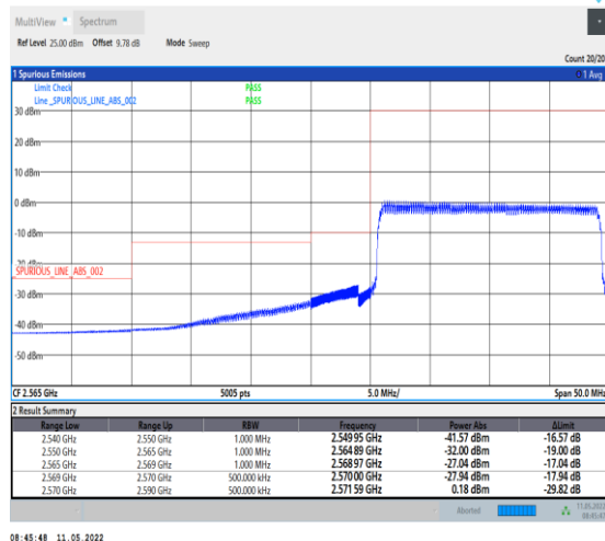
1-N38-PC2-30-20-L-6-CP-QPSK-Outer_Full-51@ 0-Ant0-PASS-see graph
