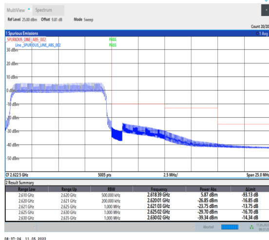
1-N38-PC2-30-10-H-6-CP-QPSK-Outer_Full-24@ 0-Ant0-PASS-see graph
