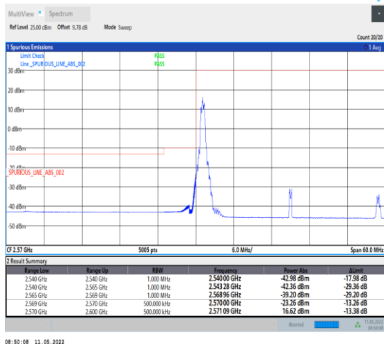
1-N38-PC2-30-30-L-4-CP-QPSK-Edge_1RB_Left-1@0 -Ant0-PASS-see graph
