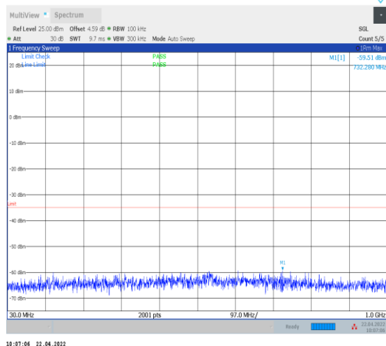
1-N38--30-40-M-1-DFT-PI2BPSK-Inner_1RB_Left-1 @1-30-1000-Ant0--59.51--35-PASS
