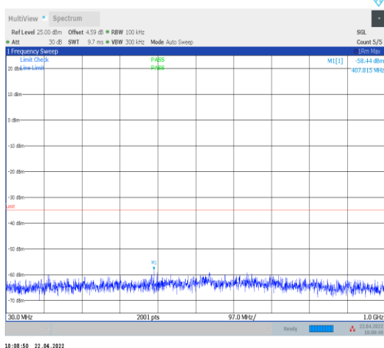
1-N38--30-40-H-1-DFT-PI2BPSK-Inner_1RB_Left-1 @1-30-1000-Ant0--58.44--35-PASS
