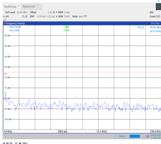
1-N38--30-40-L-1-DFT-PI2BPSK-Inner_1RB_Left-1 @1-0.009-0.15-Ant0--78.06--55-PASS
