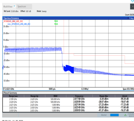
1-N38-PC2-30-30-H-6-CP-QPSK-Outer_Full-78@ 0-Ant0-PASS-see graph
