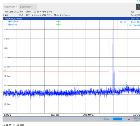
1-N38--30-40-H-1-DFT-PI2BPSK-Inner_1RB_Left-1 @1-1000-3000-Ant0--40.16--25-PASS
