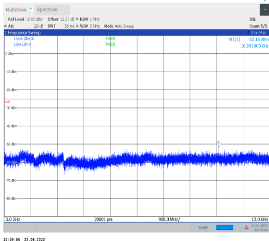
1-N38--30-40-H-1-DFT-PI2BPSK-Inner_1RB_Left-1 @1-3000-12000-Ant0--52.16--25-PASS
