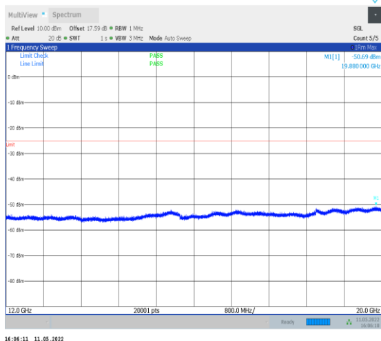
1-N38-PC2-30-40-H-1-DFT-QPSK-Edge_1RB_Left-1 @0-12000-20000-Ant0--50.69--25-PASS
