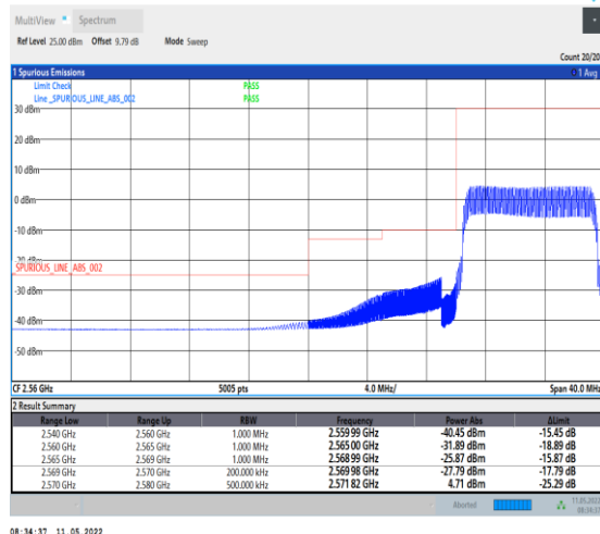
1-N38-PC2-30-10-L-6-CP-QPSK-Outer_Full-24@ 0-Ant0-PASS-see graph
