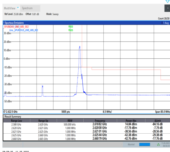
1-N38-PC2-30-40-H-5-CP-QPSK-Edge_1RB_Right-1@ 105-Ant0-PASS-see graph
