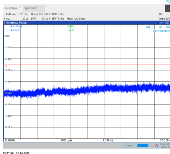
1-N38--30-40-M-1-DFT-PI2BPSK-Inner_1RB_Left-1 @1-12000-27000-Ant0--40.13--25-PASS
