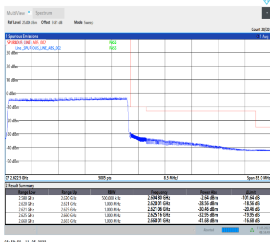
1-N38-PC2-30-40-H-6-CP-QPSK-Outer_Full-106 @0-Ant0-PASS-see graph
