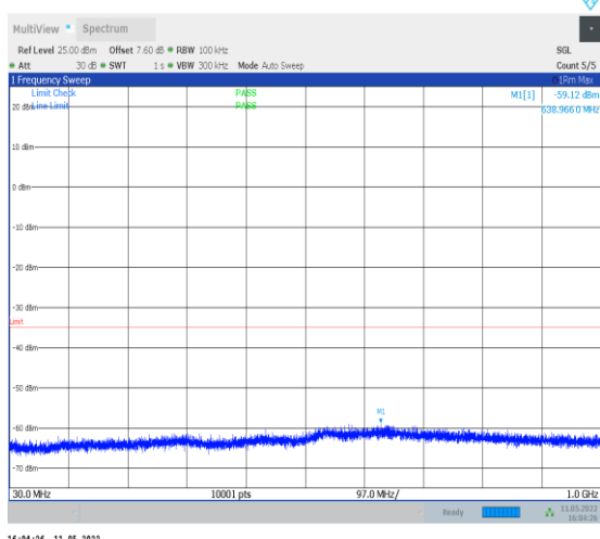
1-N38-PC2-30-40-M-1-DFT-QPSK-Edge_1RB_Left-1 @0-30-1000-Ant0--59.12--35-PASS
