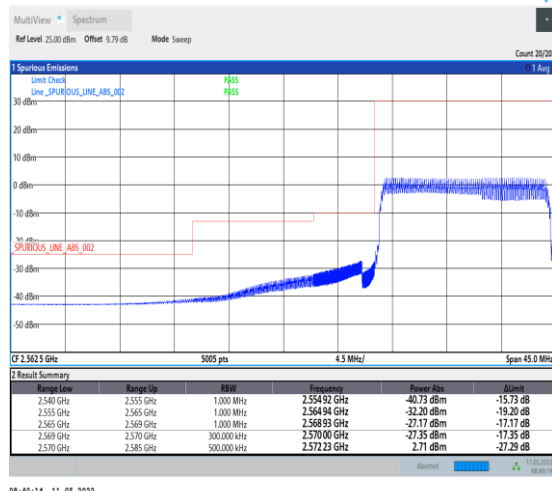
1-N38-PC2-30-15-L-6-CP-QPSK-Outer_Full-38@ 0-Ant0-PASS-see graph
