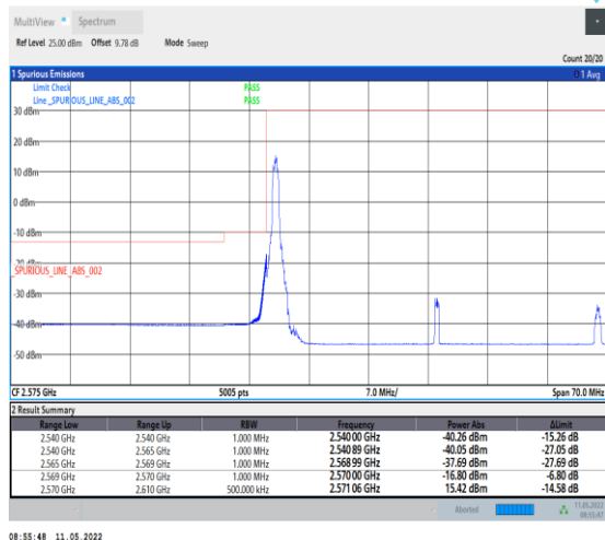
1-N38-PC2-30-40-L-4-CP-QPSK-Edge_1RB_Left-1@0 -Ant0-PASS-see graph
