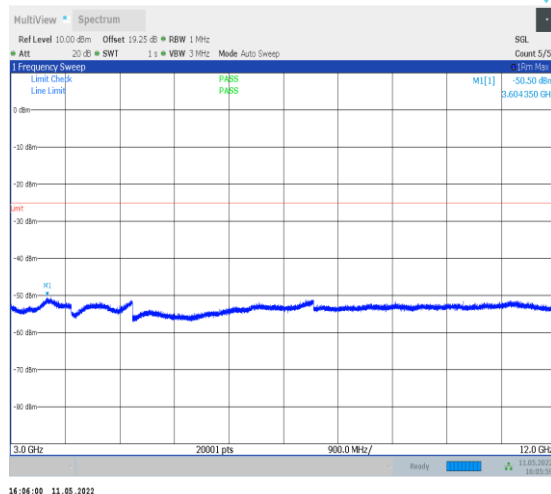
1-N38-PC2-30-40-H-1-DFT-QPSK-Edge_1RB_Left-1 @0-3000-12000-Ant0--50.50--25-PASS
