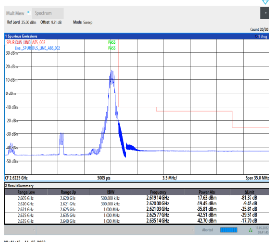
1-N38-PC2-30-15-H-5-CP-QPSK-Edge_1RB_Right-1@ 37-Ant0-PASS-see graph
