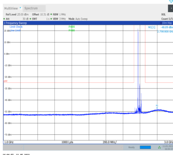
1-N38-PC2-30-40-M-1-DFT-QPSK-Edge_1RB_Left-1 @0-1000-3000-Ant0--48.09--25-PASS
