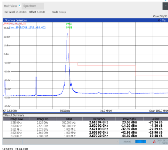
1-N38--30-40-H-2-DFT-PI2BPSK-Edge_1RB_Right-1@ 105-Ant0-PASS-see graph
