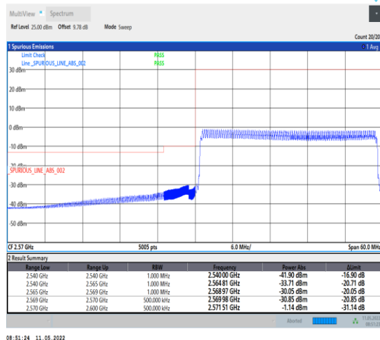
1-N38-PC2-30-30-L-6-CP-QPSK-Outer_Full-78@ 0-Ant0-PASS-see graph
