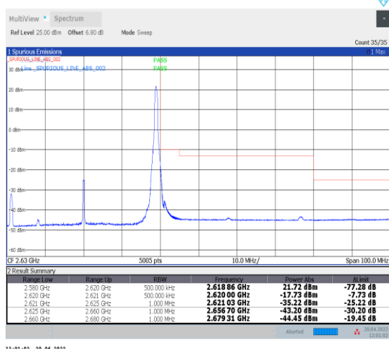
1-N38--30-40-H-5-CP-QPSK-Edge_1RB_Right-1@105 -Ant0-PASS-see graph
