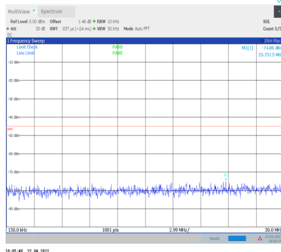
1-N38--30-40-L-1-DFT-PI2BPSK-Inner_1RB_Left-1@ 1-0.15-30-Ant0--74.86--45-PASS
