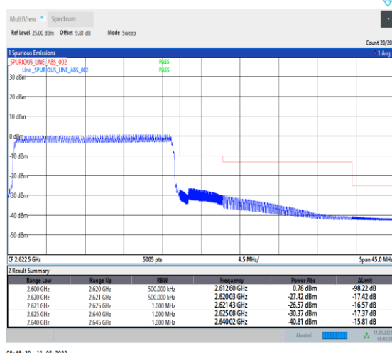
1-N38-PC2-30-20-H-6-CP-QPSK-Outer_Full-51@ 0-Ant0-PASS-see graph
