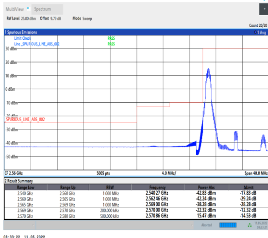
1-N38-PC2-30-10-L-4-CP-QPSK-Edge_1RB_Left-1@0 -Ant0-PASS-see graph
