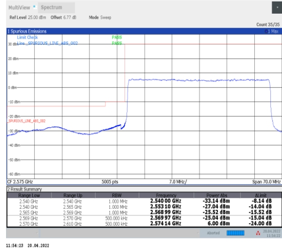
1-N38--30-40-L-3-DFT-PI2BPSK-Outer_Full-100@0-Ant0-PASS-see graph
