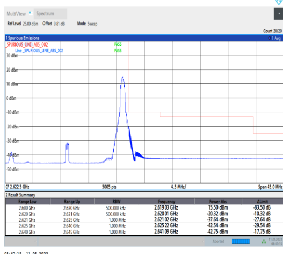
1-N38-PC2-30-20-H-5-CP-QPSK-Edge_1RB_Right-1@ 50-Ant0-PASS-see graph
