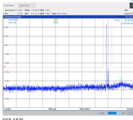
1-N38--30-40-L-1-DFT-PI2BPSK-Inner_1RB_Left-1@ 1-1000-3000-Ant0--39.40--25-PASS
