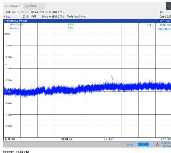
1-N38--30-40-H-1-DFT-PI2BPSK-Inner_1RB_Left-1 @1-12000-27000-Ant0--40.00--25-PASS
