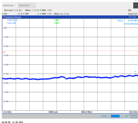
1-N38-PC2-30-40-L-1-DFT-QPSK-Edge_1RB_Left-1 @0-12000-20000-Ant0--50.90--25-PASS
