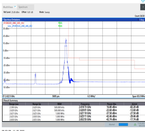
1-N38-PC2-30-30-H-5-CP-QPSK-Edge_1RB_Right-1@ 77-Ant0-PASS-see graph
