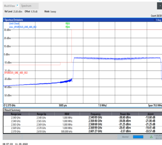
1-N38-PC2-30-40-L-6-CP-QPSK-Outer_Full-106 @0-Ant0-PASS-see graph
