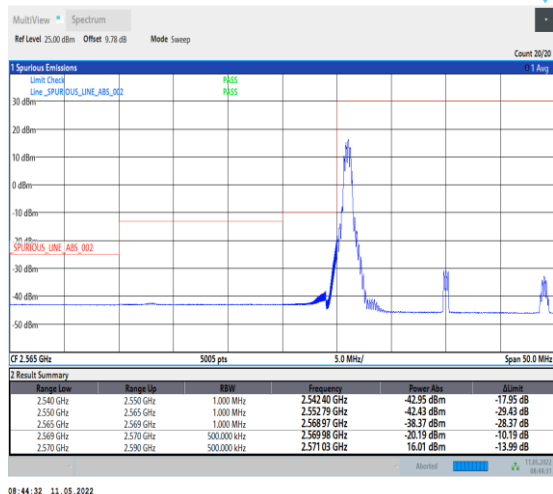
1-N38-PC2-30-20-L-4-CP-QPSK-Edge_1RB_Left-1@0 -Ant0-PASS-see graph
