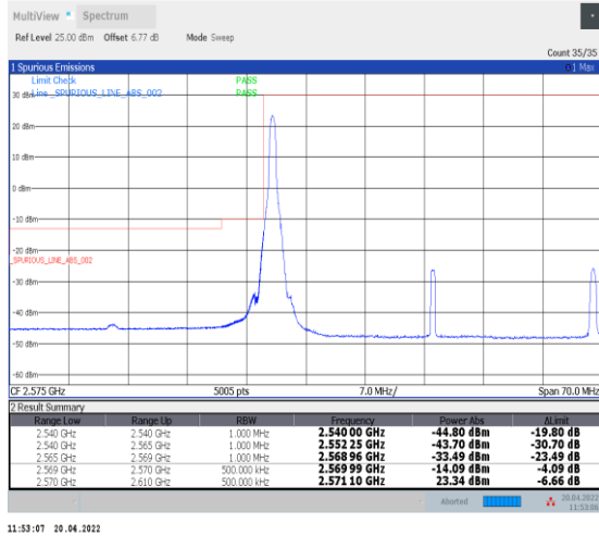
1-N38--30-40-L-1-DFT-PI2BPSK-Edge_1RB_Left-1@0-Ant0-PASS-see graph
