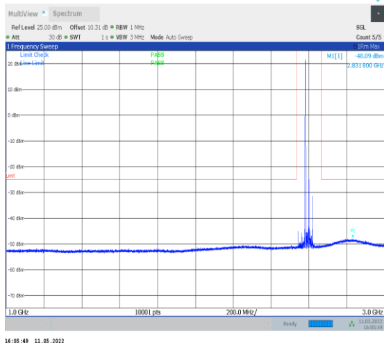
1-N38-PC2-30-40-H-1-DFT-QPSK-Edge_1RB_Left-1 @0-1000-3000-Ant0--48.09--25-PASS
