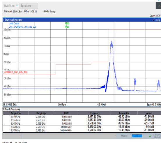
1-N38-PC2-30-15-L-4-CP-QPSK-Edge_1RB_Left-1@0 -Ant0-PASS-see graph
