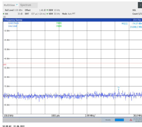
1-N38--30-40-H-1-DFT-PI2BPSK-Inner_1RB_Left-1 @1-0.15-30-Ant0--74.17--45-PASS
