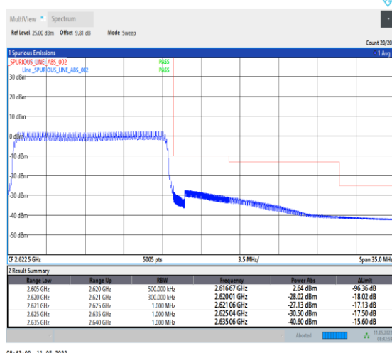
1-N38-PC2-30-15-H-6-CP-QPSK-Outer_Full-38@ 0-Ant0-PASS-see graph
