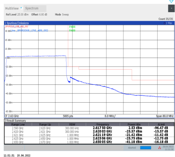
1-N38--30-30-H-6-CP-QPSK-Outer_Full-78@0-Ant0-PASS-see graph
