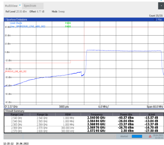
1-N38--30-30-L-6-CP-QPSK-Outer_Full-78@0-Ant0-PASS-see graph
