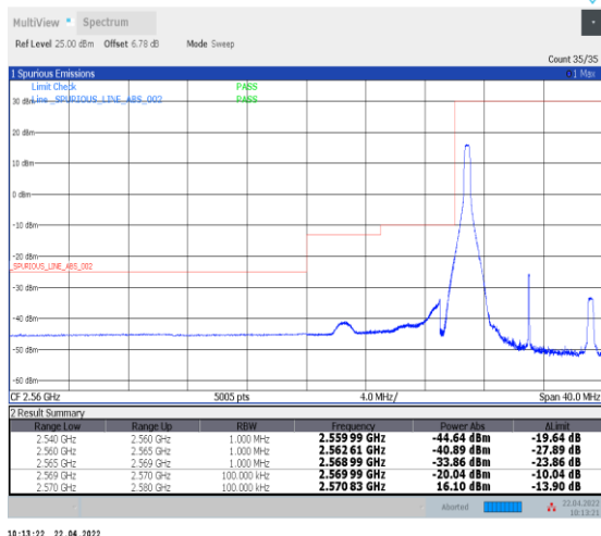
1-N38--30-10-L-4-CP-QPSK-Edge_1RB_Left-1@0-Ant0-PASS-see graph
