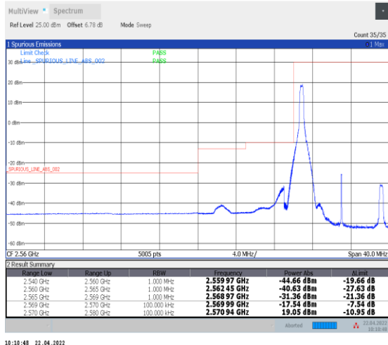
1-N38--30-10-L-1-DFT-PI2BPSK-Edge_1RB_Left-1@0-Ant0-PASS-see graph
