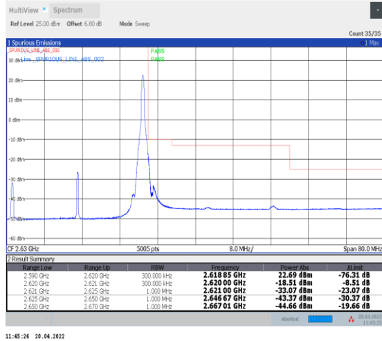
1-N38--30-30-H-2-DFT-PI2BPSK-Edge_1RB_Right-1@77-Ant0-PASS-see graph
