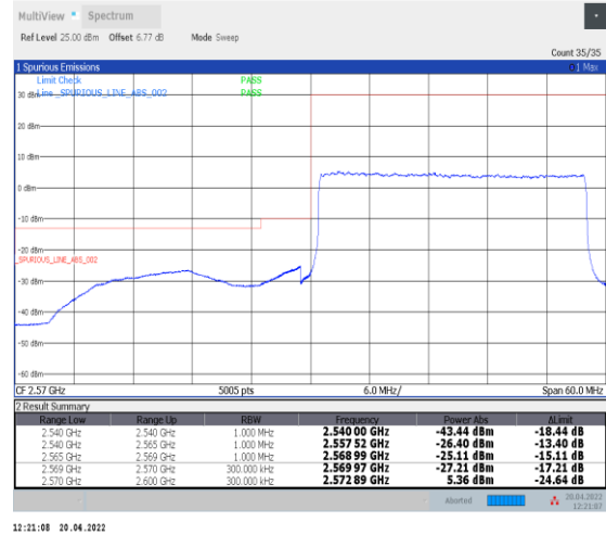
1-N38--30-30-L-3-DFT-PI2BPSK-Outer_Full-75@0-Ant0-PASS-see graph
