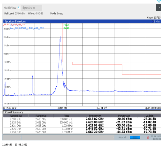
1-N38--30-30-H-5-CP-QPSK-Edge_1RB_Right-1@77-Ant0-PASS-see graph
