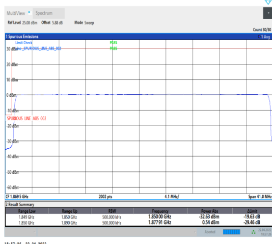
1-N25--15-40-L-6-CP-QPSK-Outer_Full-216@0-Ant0-seegraph-PASS-see graph
