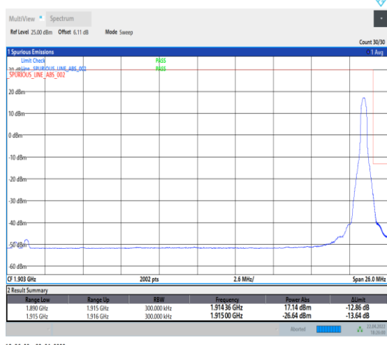
1-N25--15-25-H-5-CP-QPSK-Edge_1RB_Right-1@132 -Ant0-seegraph-PASS-see graph
