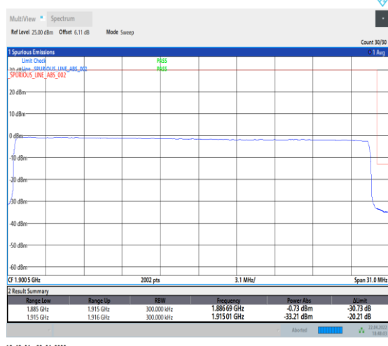
1-N25--15-30-H-6-CP-QPSK-Outer_Full-160@0-A nt0-seegraph-PASS-see graph
