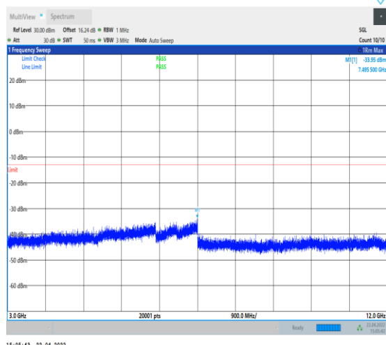
1-N25--15-40-L-1-DFT-PI2BPSK-Inner_1RB_Left-1 @1-3000-12000-Ant0--33.95--13-PASS
