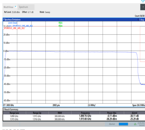
1-N25--15-25-H-6-CP-QPSK-Outer_Full-133@0-A nt0-seegraph-PASS-see graph
