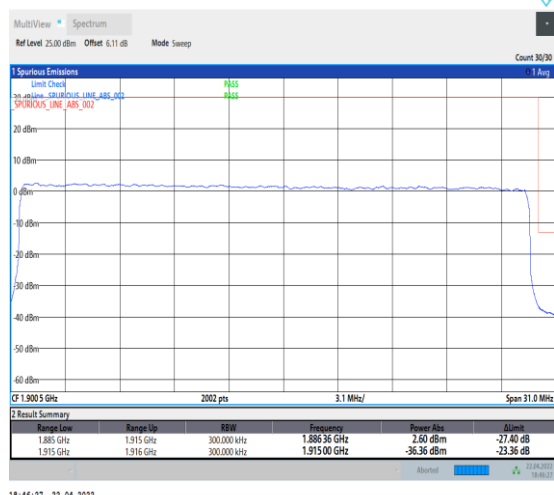
1-N25--15-30-H-3-DFT-PI2BPSK-Outer_Full-160 @0-Ant0-seegraph-PASS-see graph
