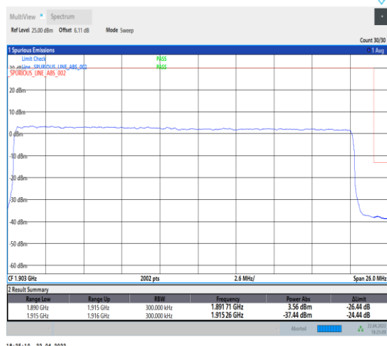
1-N25--15-25-H-3-DFT-PI2BPSK-Outer_Full-128 @0-Ant0-seegraph-PASS-see graph
