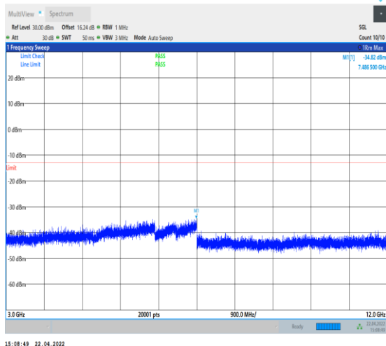
1-N25--15-40-H-1-DFT-PI2BPSK-Inner_1RB_Left-1 @1-3000-12000-Ant0--34.82--13-PASS
