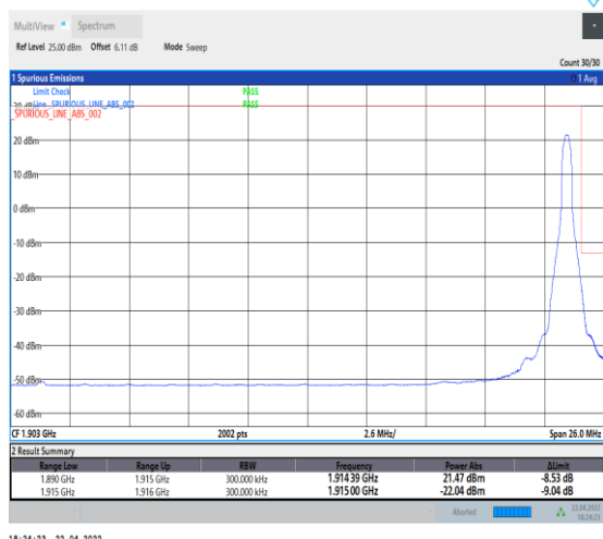
1-N25--15-25-H-2-DFT-PI2BPSK-Edge_1RB_Right-1 @132-Ant0-seegraph-PASS-see graph
