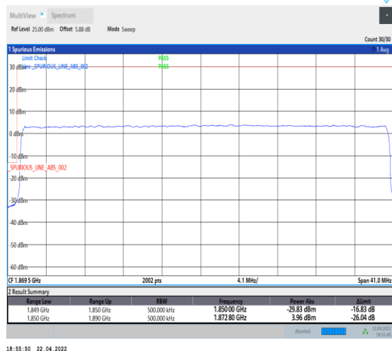
1-N25--15-40-L-3-DFT-PI2BPSK-Outer_Full-216@0-Ant0-seegraph-PASS-see graph
