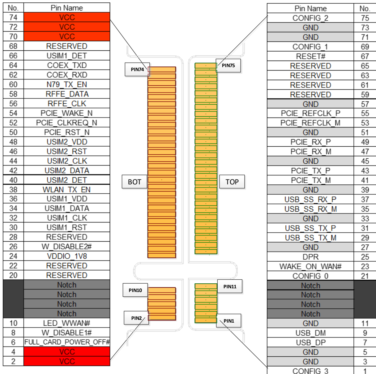
Figure 2: Pin Assignment
