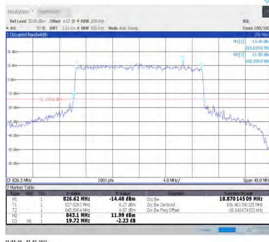
1-N26-824-849--15-20-M-8-CP-64QAM-Outer_Full-1 06@0-Ant1-18.87-19.720-≤20-PASS
