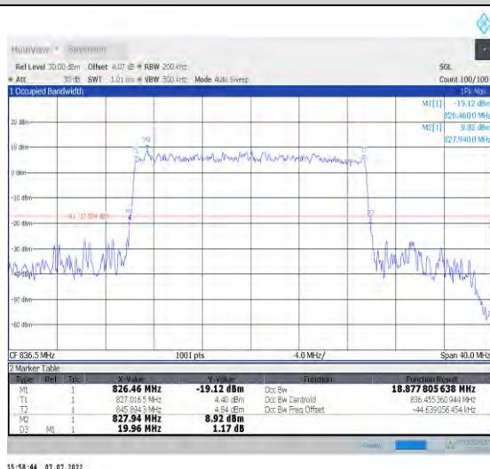
1-N26-824-849--15-20-M-9-CP-256QAM-Outer_Full- 106@0-Ant1-18.878-19.960-≤20-PASS
