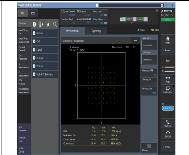
1-N26-814-824--15-10-M-8-CP-64QAM-Outer_Full-52@0-Ant1-see graph-PASS
