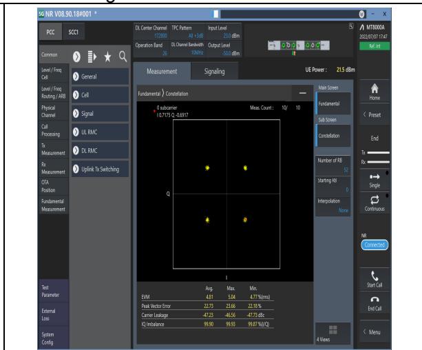
1-N26-814-824--15-10-M-6-CP-QPSK-Outer_Full-52@0-Ant1-see graph-PASS
