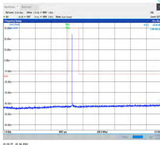
1-N25--15-40-M-1-DFT-PI2BPSK-Inner_1RB_Left-1 @1-1000-3000-Ant1--40.38--13-PASS
