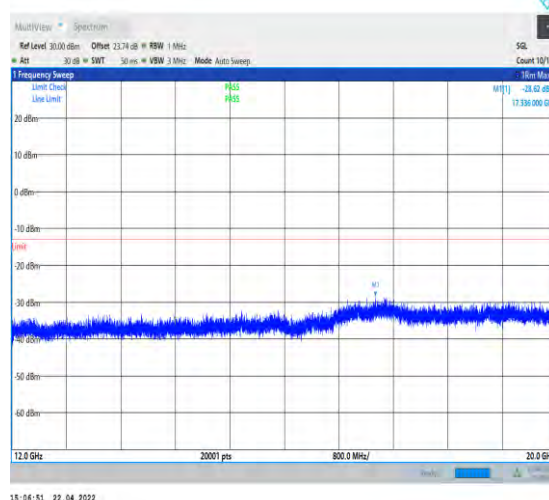
1-N25--15-40-M-1-DFT-PI2BPSK-Inner_1RB_Left-1 @1-12000-20000-Ant1--28.62--13-PASS
