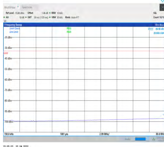
1-N25--15-40-L-1-DFT-PI2BPSK-Inner_1RB_Left-1@ 1-0.15-30-Ant1--96.88--33-PASS
