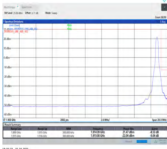
1-N25--15-25-H-2-DFT-PI2BPSK-Edge_1RB_Right-1 @132-Ant1-seegraph-PASS-see graph
