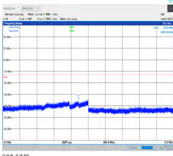
1-N25--15-40-M-1-DFT-PI2BPSK-Inner_1RB_Left-1 @1-3000-12000-Ant1--34.32--13-PASS
