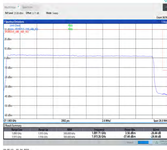
1-N25--15-25-H-3-DFT-PI2BPSK-Outer_Full-128 @0-Ant1-seegraph-PASS-see graph
