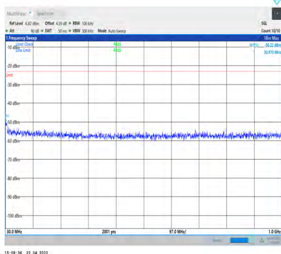
1-N25--15-40-H-1-DFT-PI2BPSK-Inner_1RB_Left-1 @1-30-1000-Ant1--50.22--23-PASS
