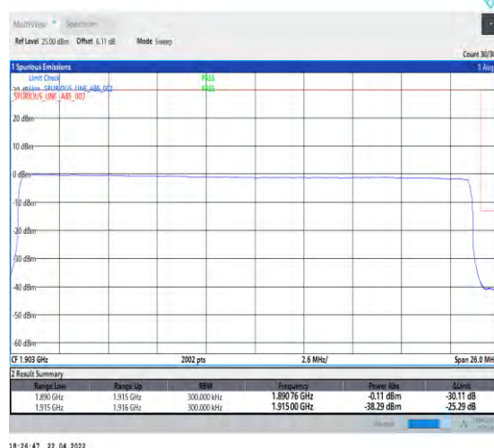
1-N25--15-25-H-6-CP-QPSK-Outer_Full-133@0-A nt1-seegraph-PASS-see graph
