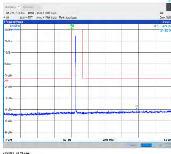
1-N25--15-40-L-1-DFT-PI2BPSK-Inner_1RB_Left-1@ 1-1000-3000-Ant1--40.56--13-PASS
