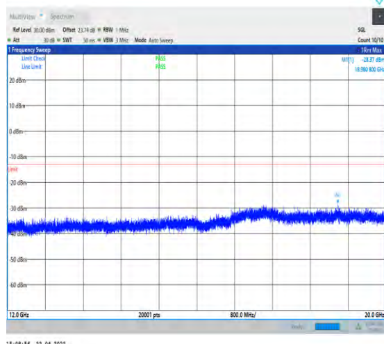
1-N25--15-40-H-1-DFT-PI2BPSK-Inner_1RB_Left-1 @1-12000-20000-Ant1--28.37--13-PASS
