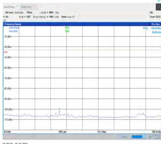
1-N25--15-40-H-1-DFT-PI2BPSK-Inner_1RB_Left-1 @1-0.009-0.15-Ant1--103.29--43-PASS
