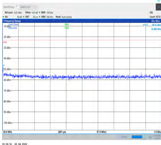
1-N25--15-40-M-1-DFT-PI2BPSK-Inner_1RB_Left-1 @1-30-1000-Ant1--49.92--23-PASS
