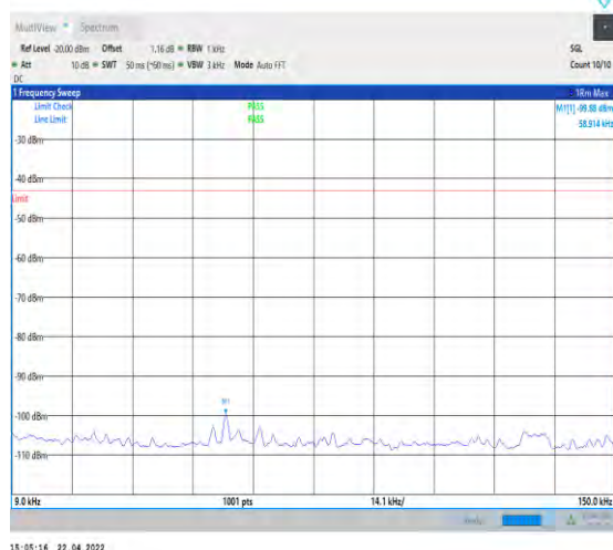
1-N25--15-40-L-1-DFT-PI2BPSK-Inner_1RB_Left-1 @1-0.009-0.15-Ant1--99.88--43-PASS
