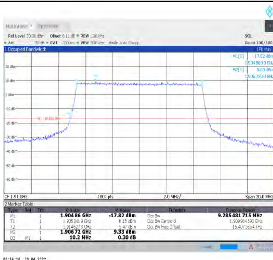
1-N25--15-10-H-6-CP-QPSK-Outer_Full-52@0-Ant1- 9.285-10.200-≤10-PASS
