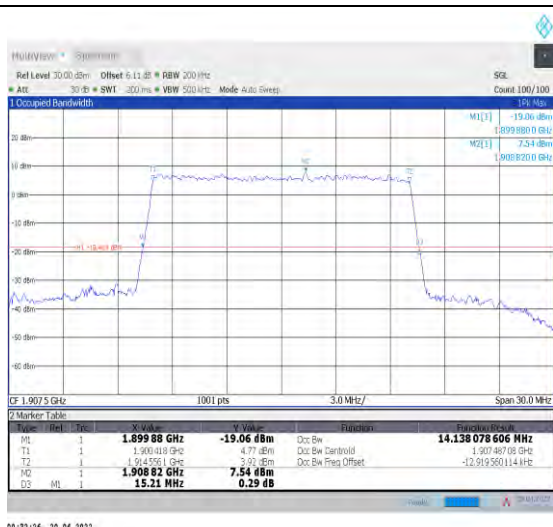
1-N25--15-15-H-9-CP-256QAM-Outer_Full-79@0-An t1-14.138-15.210-≤15-PASS
