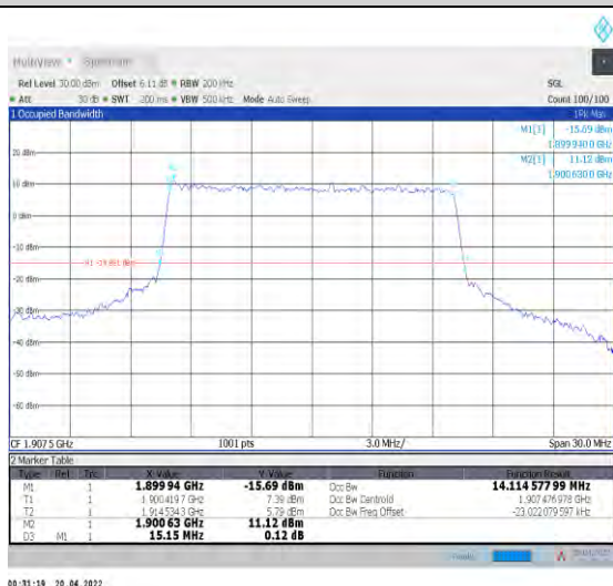
1-N25--15-15-H-7-CP-16QAM-Outer_Full-79@0-Ant 1-14.115-15.150-≤15-PASS
