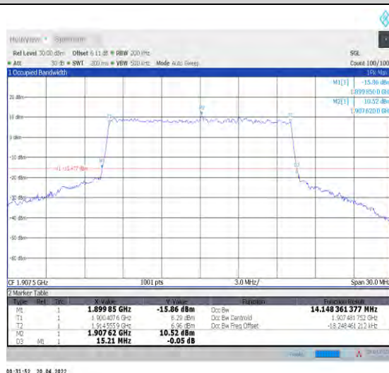
1-N25--15-15-H-8-CP-64QAM-Outer_Full-79@0-Ant 1-14.148-15.210-≤15-PASS
