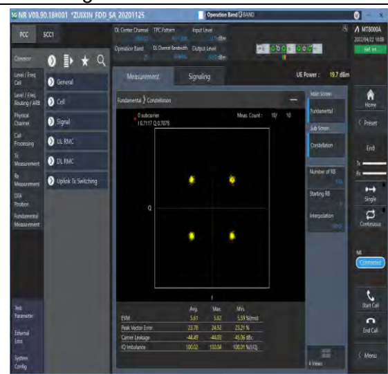
1-N25--15-40-M-6-CP-QPSK-Outer_Full-216@0-Ant1-see graph-PASS
