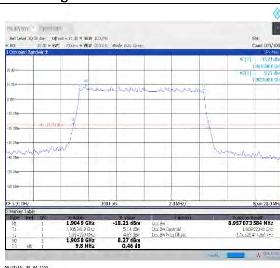
1-N25--15-10-H-5-DFT-256QAM-Outer_Full-50@0-A nt1-8.957-9.800-≤10-PASS
