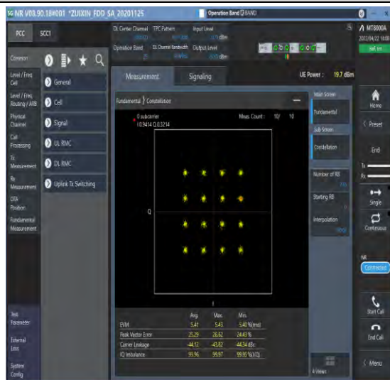
1-N25--15-40-M-7-CP-16QAM-Outer_Full-216@0-Ant1-see graph-PASS
