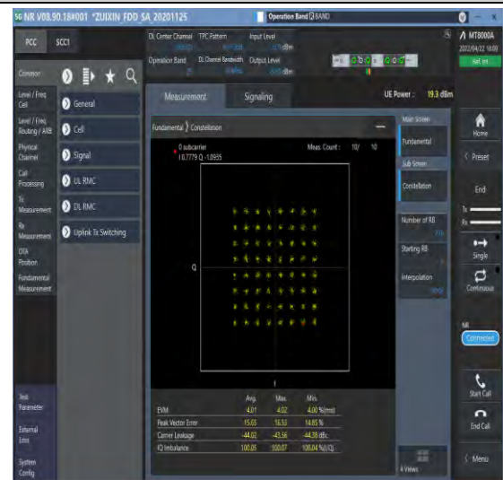
1-N25--15-40-M-8-CP-64QAM-Outer_Full-216@0-Ant1-see graph-PASS
