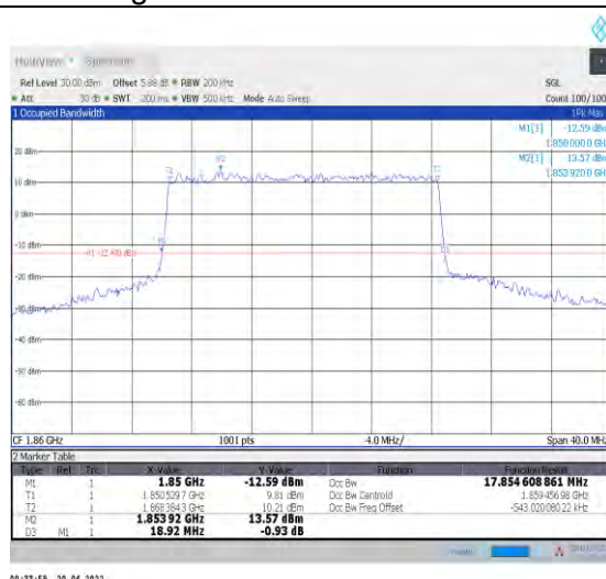
1-N25--15-20-L-1-DFT-QPSK-Outer_Full-100@0-Ant 1-17.855-18.920-≤20-PASS
