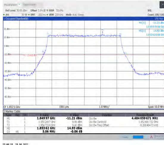
1-N25--15-5-L-2-DFT-PI2BPSK-Outer_Full-25@0-An t1-4.484-5.060-≤5-PASS
