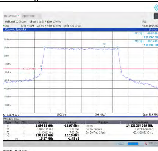
1-N25--15-15-H-6-CP-QPSK-Outer_Full-79@0-Ant1 14.131-15.270-≤15-PASS
