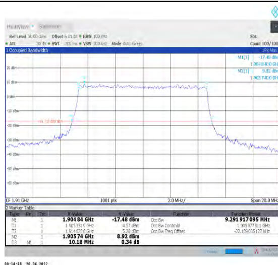
1-N25--15-10-H-7-CP-16QAM-Outer_Full-52@0-Ant 1-9.292-10.180-≤10-PASS
