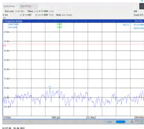
1-N14--15-10-H-1-DFT-PI2BPSK-Inner_1RB_Left-1 @1-0.009-0.15-Ant1--81.64--33-PASS
