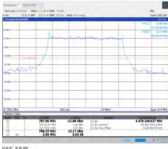
1-N14--15-5-L-3-DFT-16QAM-Outer_Full-25@0-Ant 1-4.476-5.060-≤5-PASS
