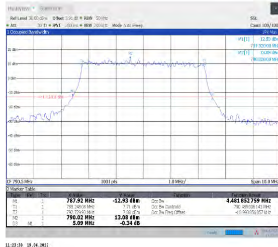
1-N14--15-5-L-4-DFT-64QAM-Outer_Full-25@0-Ant1 -4.482-5.090-≤5-PASS
