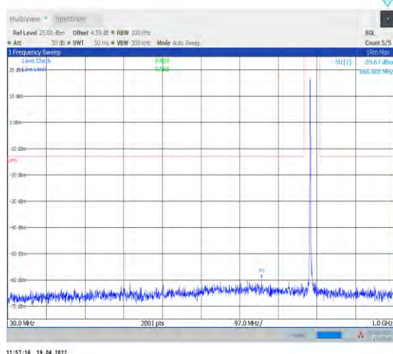
1-N14--15-10-H-1-DFT-PI2BPSK-Inner_1RB_Left-1 @1-30-1000-Ant1--59.67--13-PASS
