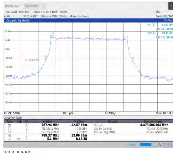
1-N14--15-5-L-2-DFT-PI2BPSK-Outer_Full-25@0-An t1-4.474-5.100-≤5-PASS
