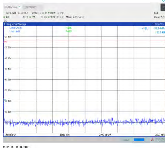
1-N14--15-10-H-1-DFT-PI2BPSK-Inner_1RB_Left-1 @1-0.15-30-Ant1--82.24--23-PASS
