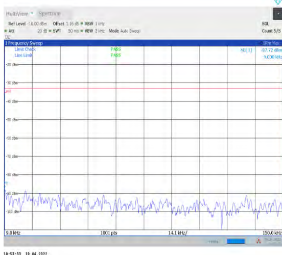
1-N12--15-15-M-1-DFT-PI2BPSK-Inner_1RB_Left-1 @1-0.009-0.15-Ant1--87.72--33-PASS
