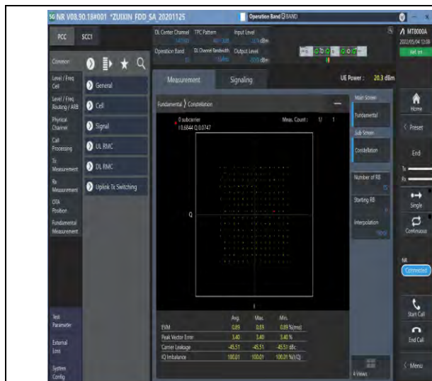
1-N12-PC3-15-15-M-5-DFT-256QAM-Outer_Full-75@0-Ant1-see graph-PASS
