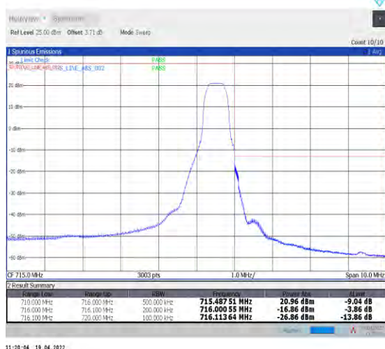
1-N12--15-15-H-5-CP-QPSK-Edge_1RB_Right-1@78-Ant1-PASS-see graph
