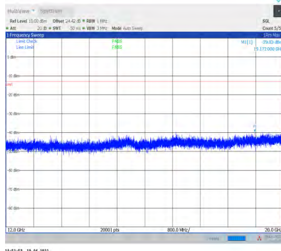
1-N12--15-15-L-1-DFT-PI2BPSK-Inner_1RB_Left-1@ 1-12000-20000-Ant1--39.83--13-PASS
