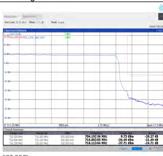
1-N12--15-15-H-3-DFT-PI2BPSK-Outer_Full-75@0-Ant1-PASS-see graph
