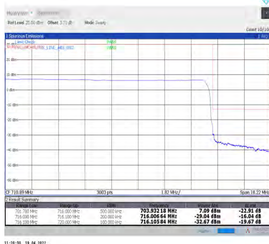
1-N12--15-15-H-6-CP-QPSK-Outer_Full-79@0-Ant1-PASS-see graph
