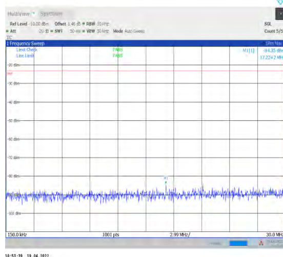
1-N12--15-15-M-1-DFT-PI2BPSK-Inner_1RB_Left-1 @1-0.15-30-Ant1--84.35--23-PASS
