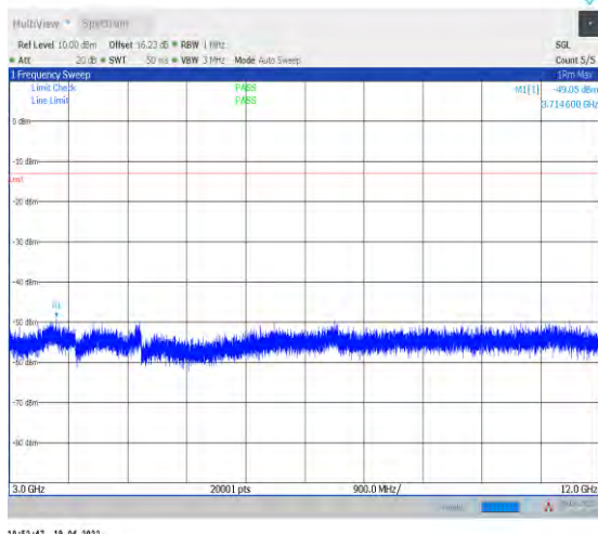
1-N12--15-15-L-1-DFT-PI2BPSK-Inner_1RB_Left-1 @1-3000-12000-Ant1--49.05--13-PASS
