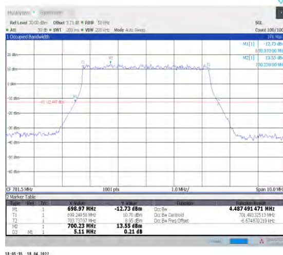
1-N12--15-5-L-2-DFT-PI2BPSK-Outer_Full-25@0-An t1-4.487-5.110-≤5-PASS
