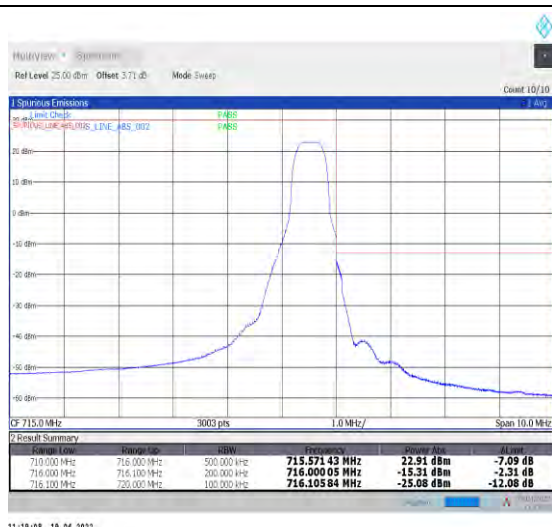
1-N12--15-15-H-2-DFT-PI2BPSK-Edge_1RB_Right-1@78-Ant1-PASS-see graph
