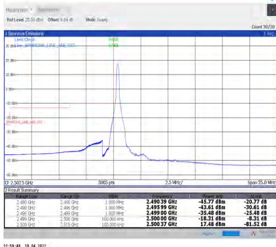
1-N7--15-10-L-4-CP-QPSK-Edge_1RB_Left-1@0-Ant1-PASS-see graph
