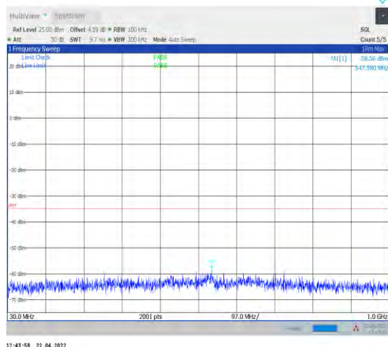
1-N7--15-40-L-1-DFT-PI2BPSK-Inner_1RB_Left-1@ 1-30-1000-Ant1--58.56--35-PASS
