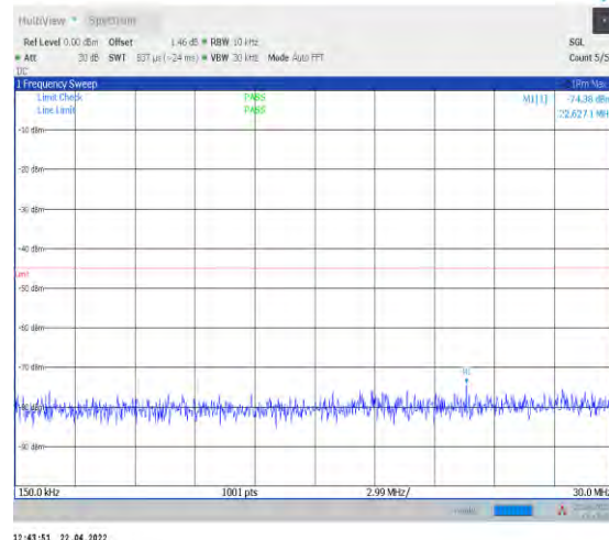
1-N7--15-40-L-1-DFT-PI2BPSK-Inner_1RB_Left-1@ -0.15-30-Ant1--74.38--45-PASS
