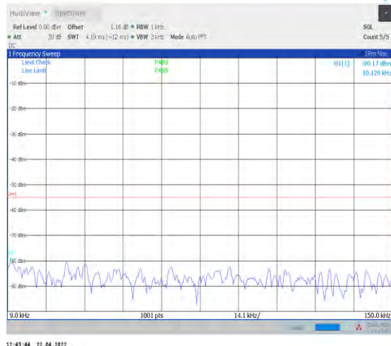
1-N7--15-40-L-1-DFT-PI2BPSK-Inner_1RB_Left-1@ 1-0.009-0.15-Ant1--80.17--55-PASS
