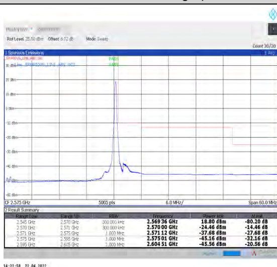
1-N7--15-25-H-5-CP-QPSK-Edge_1RB_Right-1@132-Ant1-PASS-see graph
