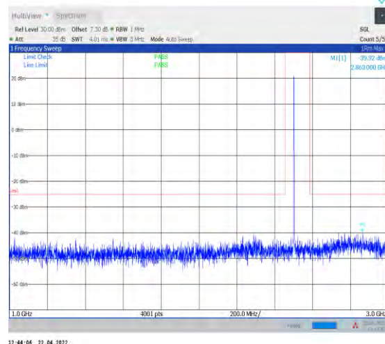
1-N7--15-40-L-1-DFT-PI2BPSK-Inner_1RB_Left-1@ -1000-3000-Ant1--39.92--25-PASS
