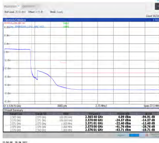
1-N7--15-5-H-6-CP-QPSK-Outer_Full-25@0-Ant1-PASS-see graph
