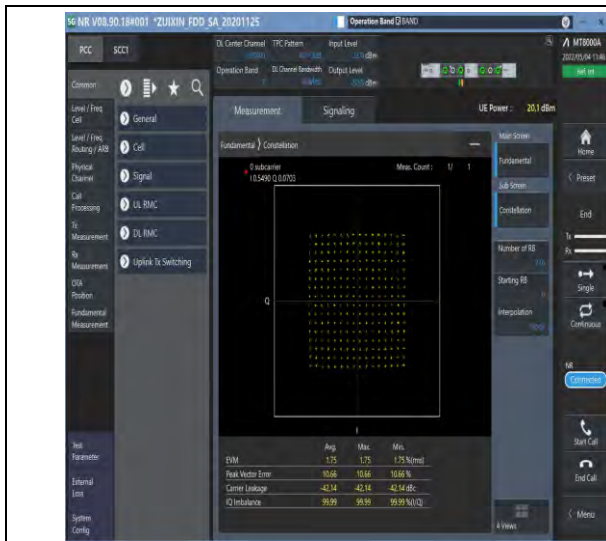
1-N7-PC3-15-40-M-5-DFT-256QAM-Outer_Full-216@0-Ant1-see graph-PASS
