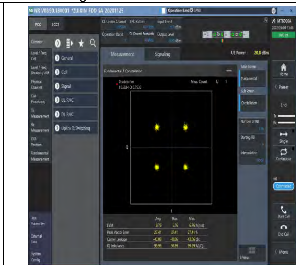
1-N7-PC3-15-40-M-6-CP-QPSK-Outer_Full-216@0-Ant1-see graph-PASS
