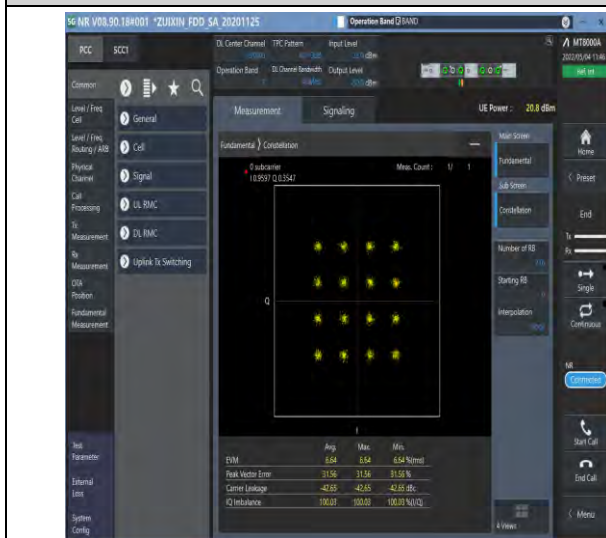
1-N7-PC3-15-40-M-7-CP-16QAM-Outer_Full-216@0-Ant1-see graph-PASS
