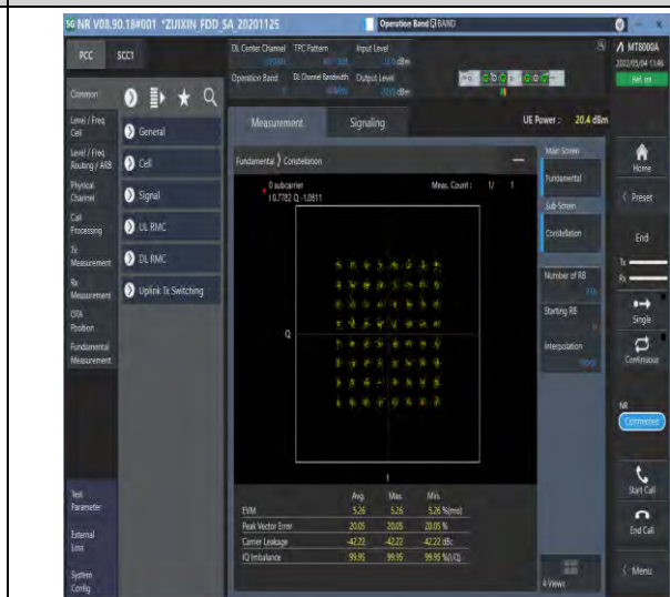
1-N7-PC3-15-40-M-8-CP-64QAM-Outer_Full-216@0-Ant1-see graph-PASS
