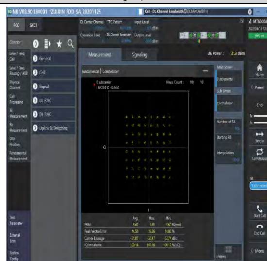
1-N5--15-20-M-8-CP-64QAM-Outer_Full-106@0-A nt1-see graph-PASS
