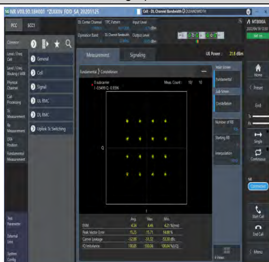
1-N5--15-20-M-7-CP-16QAM-Outer_Full-106@0-A nt1-see graph-PASS
