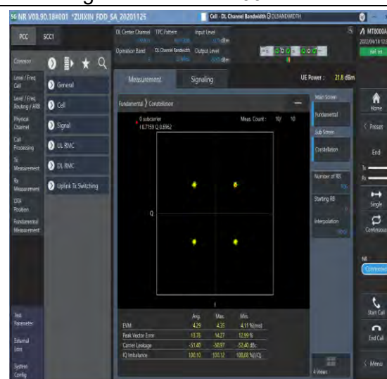
1-N5--15-20-M-6-CP-QPSK-Outer_Full-106@0-A nt1-see graph-PASS
