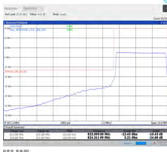
1-N5--15-5-L-6-CP-QPSK-Outer_Full-25@0-Ant1-seegraph-PASS-see graph
