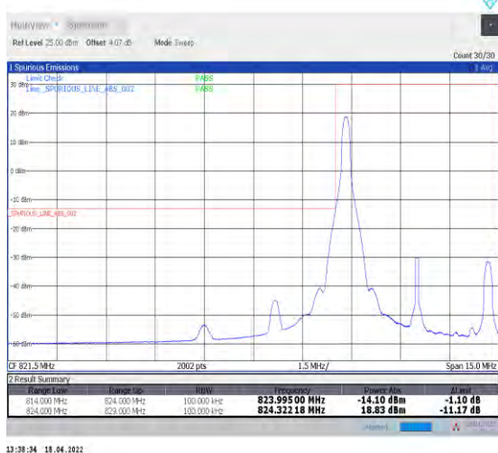
1-N5--15-5-L-4-CP-QPSK-Edge_1RB_Left-1@0-Ant1-s eegraph-PASS-see graph
