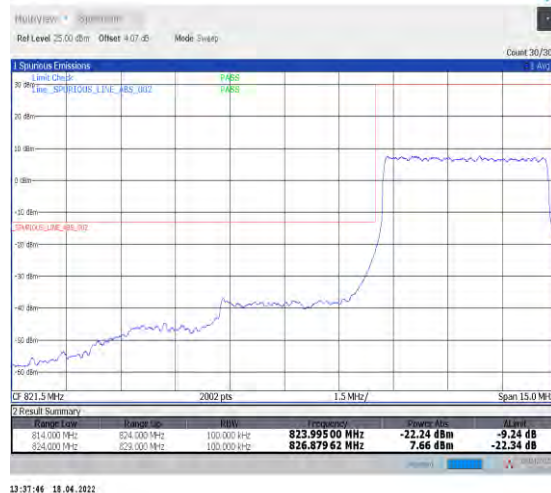
1-N5--15-5-L-3-DFT-PI2BPSK-Outer_Full-25@0-A nt1-seegraph-PASS-see graph
