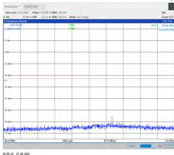
1-N2--15-20-L-1-DFT-PI2BPSK-Inner_1RB_Left-1@ 1-30-1000-Ant1--59.66--23-PASS
