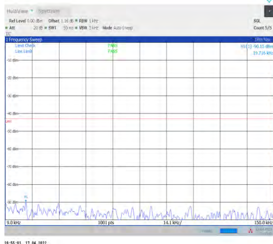
1-N2--15-20-L-1-DFT-PI2BPSK-Inner_1RB_Left-1@ 1-0.009-0.15-Ant1--90.15--43-PASS
