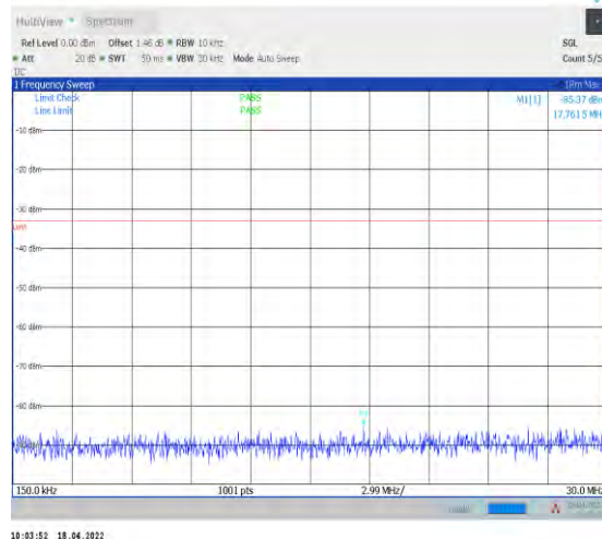
1-N2--15-20-H-1-DFT-PI2BPSK-Inner_1RB_Left-1@ 1-0.15-30-Ant1--85.37--33-PASS
