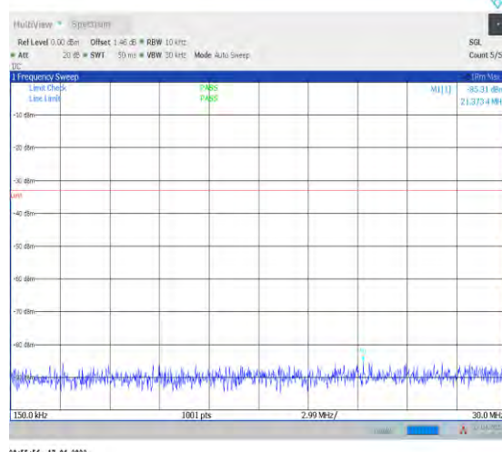
1-N2--15-20-M-1-DFT-PI2BPSK-Inner_1RB_Left-1@ 1-0.15-30-Ant1--85.31--33-PASS
