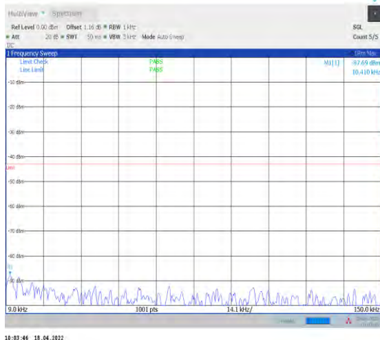
1-N2--15-20-H-1-DFT-PI2BPSK-Inner_1RB_Left-1@ 1-0.009-0.15-Ant1--87.69--43-PASS
