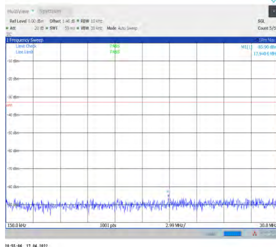
1-N2--15-20-L-1-DFT-PI2BPSK-Inner_1RB_Left-1@ -0.15-30-Ant1--85.90--33-PASS
