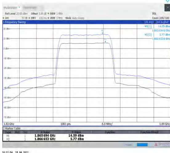
1-N2--15-20-L-1-DFT-256QAM-Outer_Full-100@0-A nt1-8.82-100%-0.00-8.82-PASS≤13
