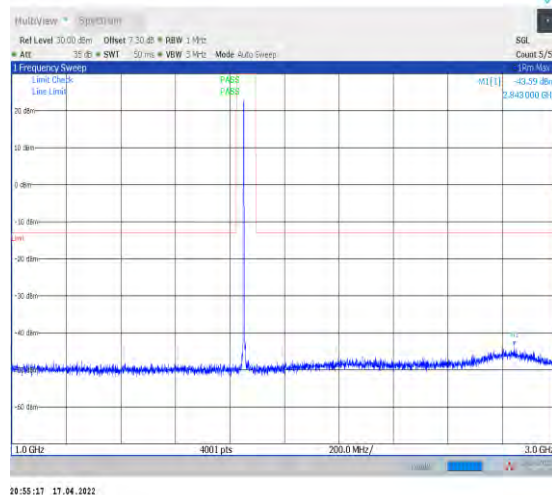
1-N2--15-20-L-1-DFT-PI2BPSK-Inner_1RB_Left-1@ -1000-3000-Ant1--43.59--13-PASS
