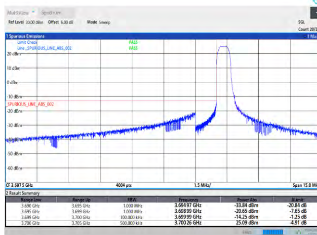
Band43-5MHz-QPSK-44615-25RB#0
