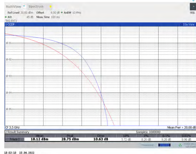
Band42-20MHz-QPSK-42590-100RB#0
