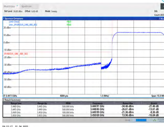
Band42-5MHz-QPSK-42115-25RB#0
