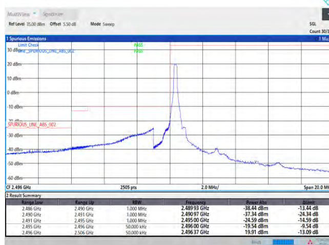
Band41-5MHz-QPSK-39675-25RB#0
