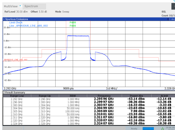
Band30-5MHz-QPSK-27685-25RB#0
