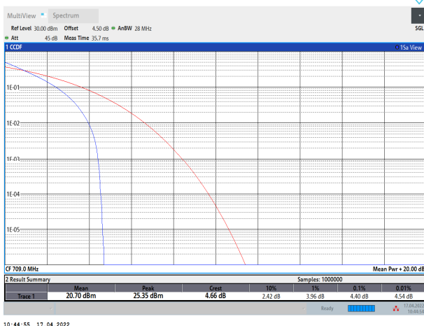
Band17-10MHz-QPSK-23790-50RB#0
