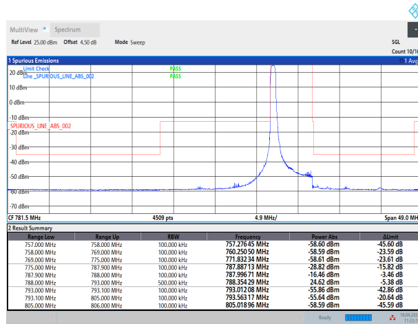
Band14-5MHz-QPSK-23305-1RB#0
