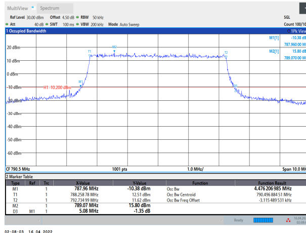
Band14-5MHz-QPSK-23330-25RB#0
