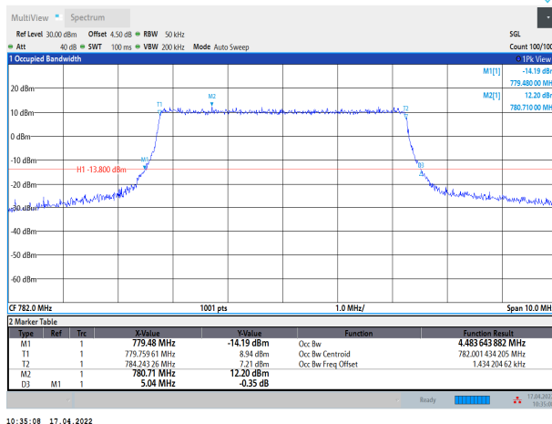
Band13-5MHz-QPSK-23230-25RB#0
