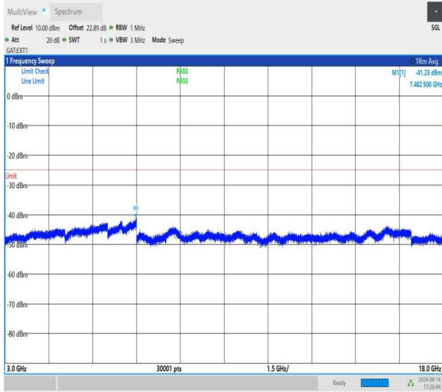
NTNV-n41-PC1.5-30-40-M-CP-QPSK-Edge_1RB_Left-3000-1800 0-PASS
