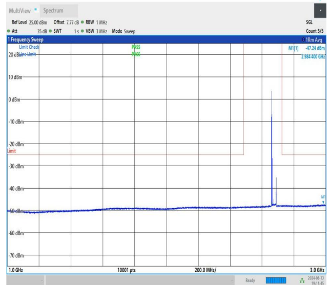
NTNV-n41-PC1.5-30-30-H-CP-QPSK-Edge_1RB_Left-1000-3000-PASS
