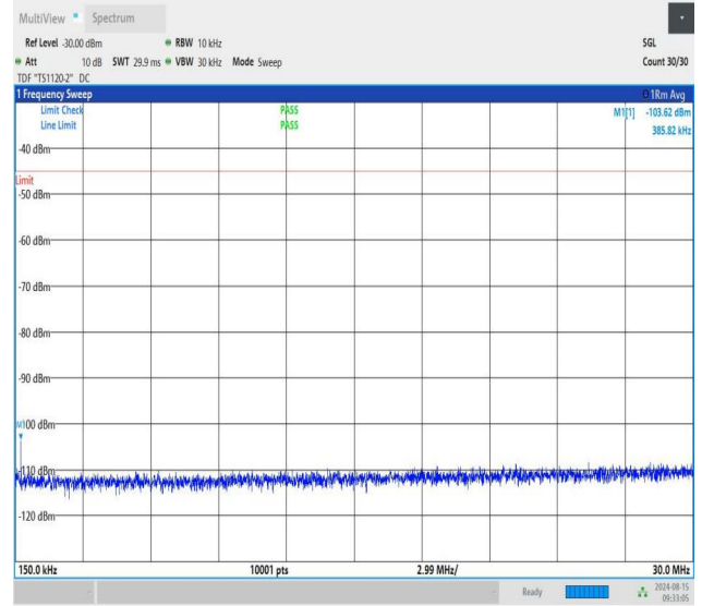
NTNV-n41-PC1.5-30-30-H-CP-QPSK-Edge_1RB_Left-0.15-30-PASS
