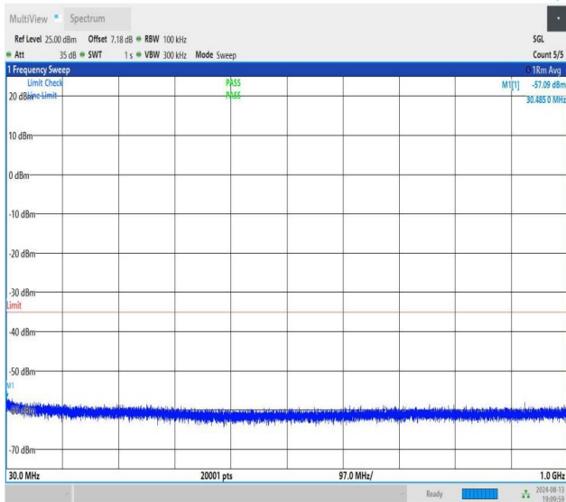
NTNV-n41-PC1.5-30-20-H-CP-QPSK-Edge_1RB_Left-30-1000-PASS
