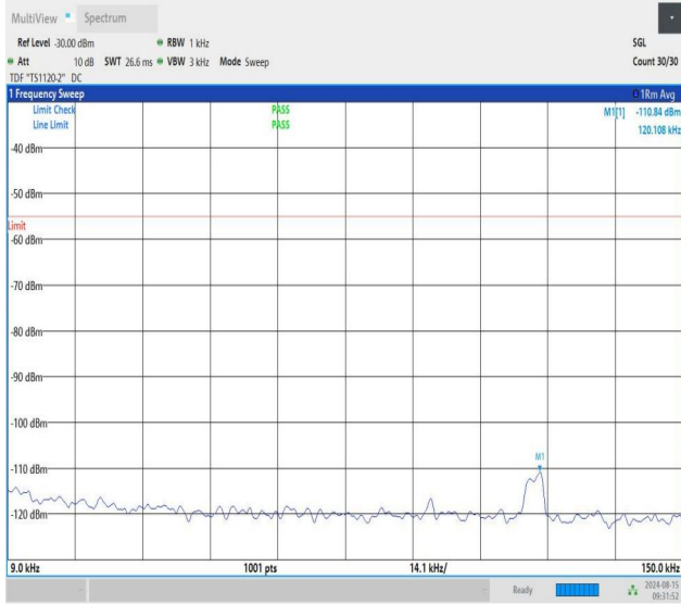
NTNV-n41-PC1.5-30-20-H-CP-QPSK-Edge_1RB_Left-0.009-0.15-PASS
