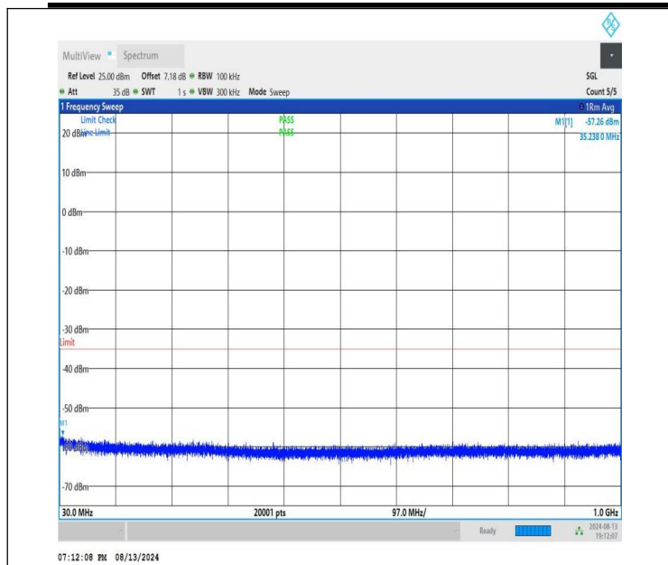
NTNV-n41-PC1.5-30-30-L-CP-QPSK-Edge_1RB_Right-30-1000-P ASS
