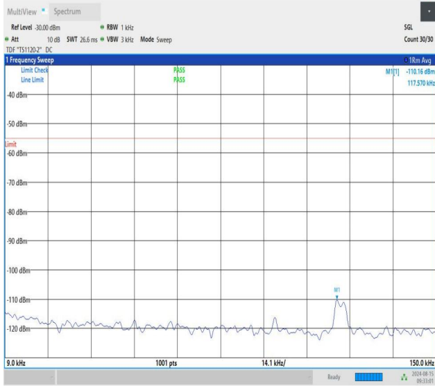
NTNV-n41-PC1.5-30-30-H-CP-QPSK-Edge_1RB_Left-0.009-0.15-PASS
