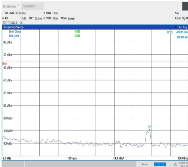
NTNV-n41-PC1.5-30-30-M-CP-QPSK-Edge_1RB_Right-0.009-0.1 5-PASS
