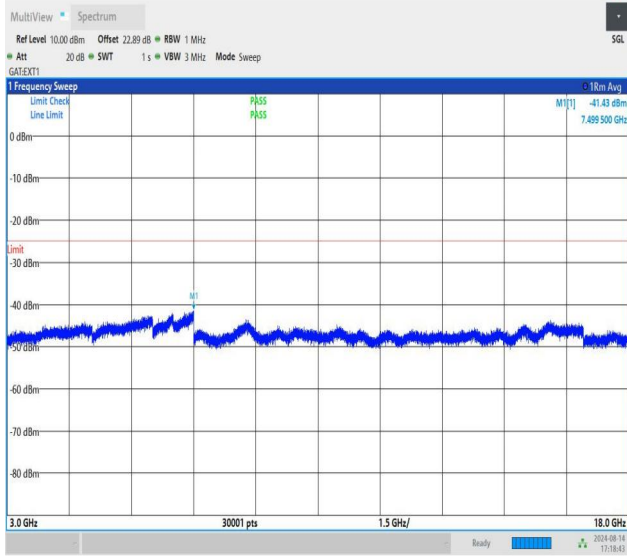
NTNV-n41-PC1.5-30-30-H-CP-QPSK-Edge_1RB_Left-3000-1800 0-PASS
