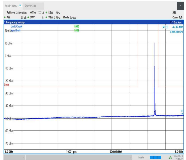
NTNV-n41-PC1.5-30-20-H-CP-QPSK-Edge_1RB_Left-1000-3000-PASS
