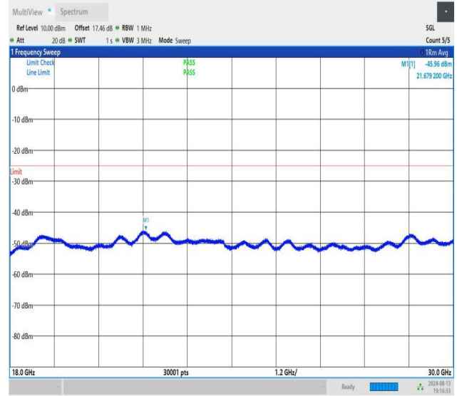
NTNV-n41-PC1.5-30-40-L-CP-QPSK-Edge_1RB_Left-18000-3000 0-PASS
