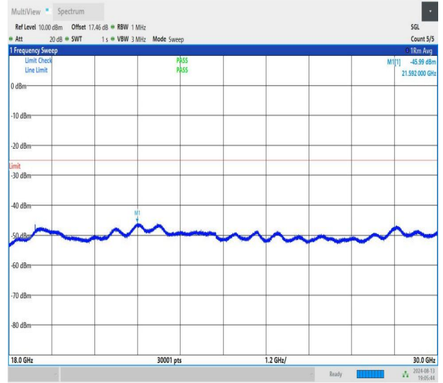
NTNV-n41-PC1.5-30-15-H-CP-QPSK-Edge_1RB_Left-18000-3000 0-PASS
