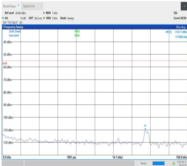
NTNV-n41-PC1.5-30-40-M-CP-QPSK-Edge_1RB_Right-0.009-0.1 5-PASS
