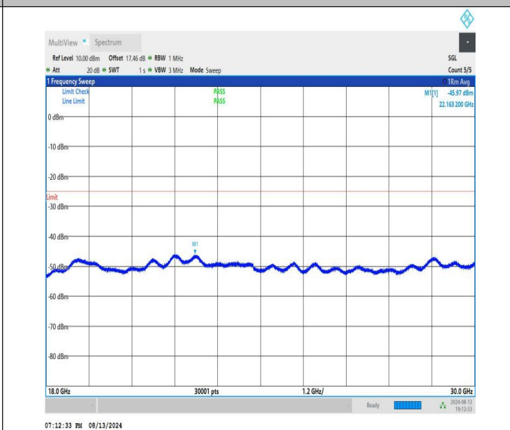
NTNV-n41-PC1.5-30-30-L-CP-QPSK-Edge_1RB_Right-18000-300 00-PASS
