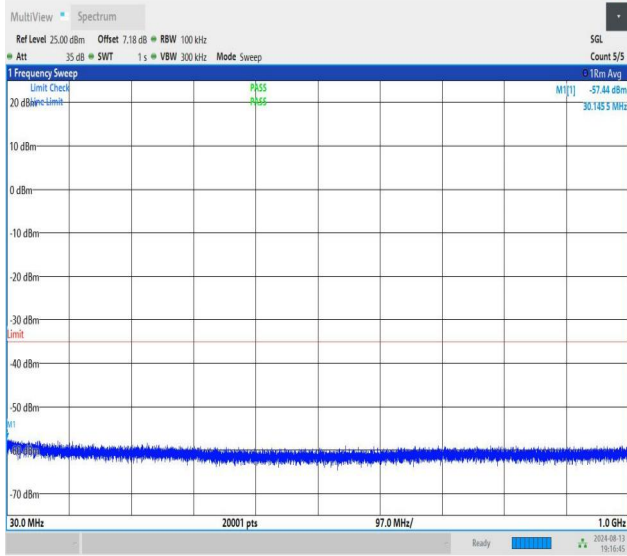
NTNV-n41-PC1.5-30-40-L-CP-QPSK-Edge_1RB_Right-30-1000-P ASS
