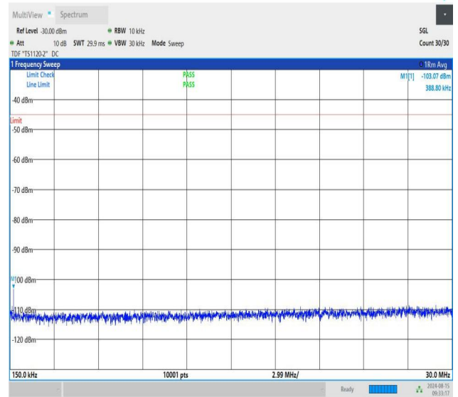
NTNV-n41-PC1.5-30-30-H-CP-QPSK-Edge_1RB_Right-0.15-30-PA SS
