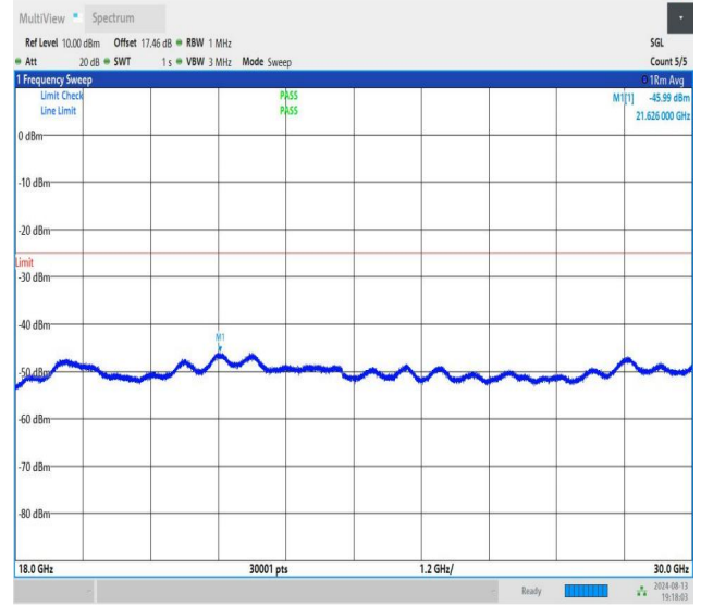
NTNV-n41-PC1.5-30-40-M-CP-QPSK-Edge_1RB_Left-18000-3000 0-PASS
