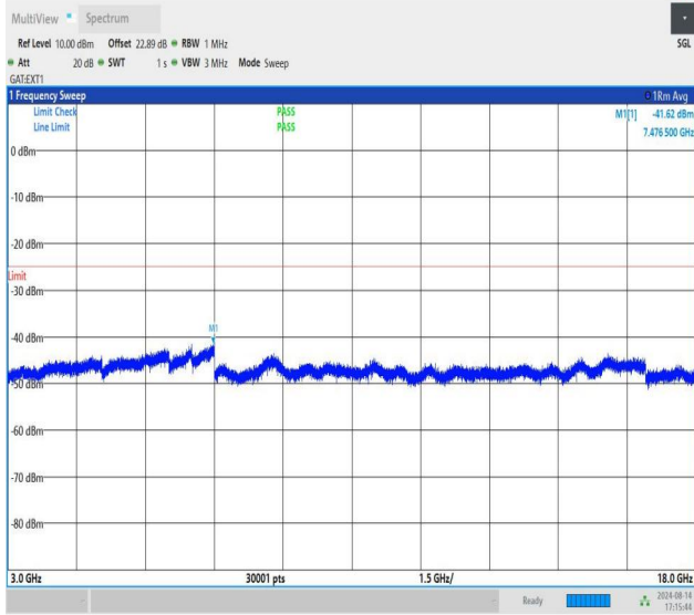
NTNV-n41-PC1.5-30-20-H-CP-QPSK-Edge_1RB_Left-3000-1800 0-PASS
