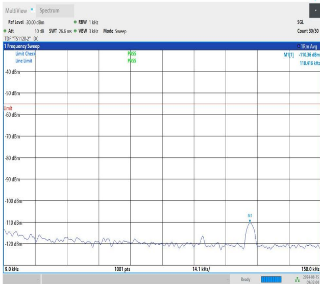
NTNV-n41-PC1.5-30-20-H-CP-QPSK-Edge_1RB_Right-0.009-0.1 5-PASS
