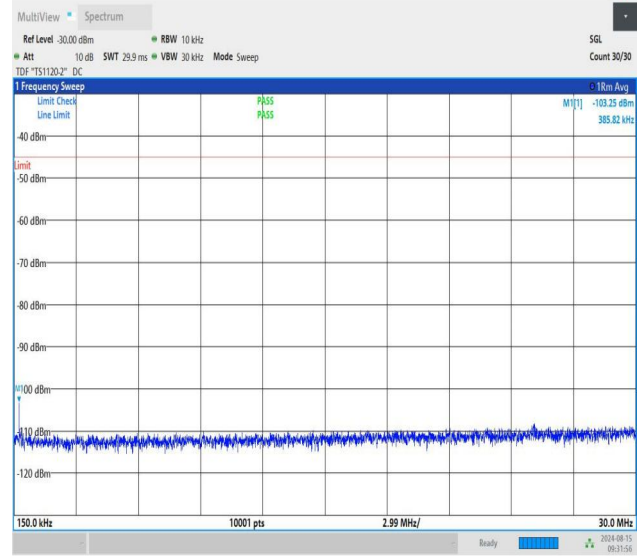
NTNV-n41-PC1.5-30-20-H-CP-QPSK-Edge_1RB_Left-0.15-30-PASS
