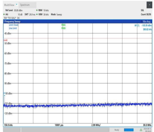
NTNV-n41-PC1.5-30-40-M-CP-QPSK-Edge_1RB_Right-0.15-30-P ASS
