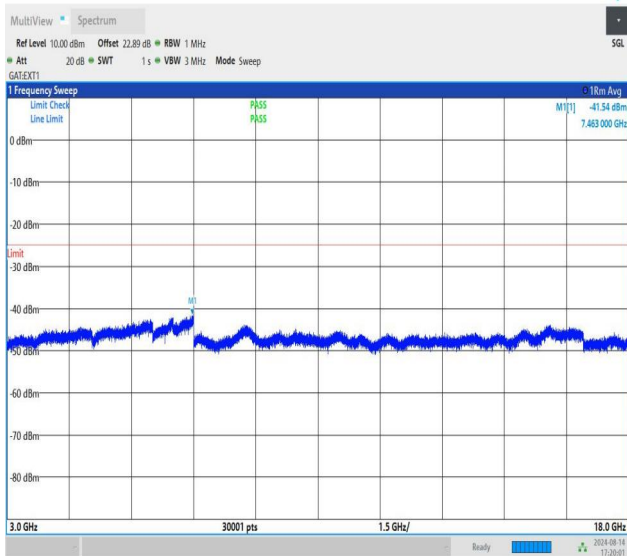
NTNV-n41-PC1.5-30-40-L-CP-QPSK-Edge_1RB_Right-3000-180 00-PASS
