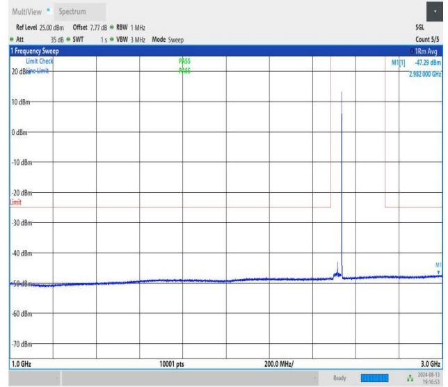
NTNV-n41-PC1.5-30-40-L-CP-QPSK-Edge_1RB_Right-1000-3000- PASS
