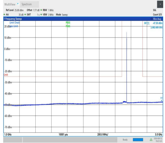
NTNV-n41-PC1.5-30-50-L-CP-QPSK-Edge_1RB_Right-1000-3000- PASS
