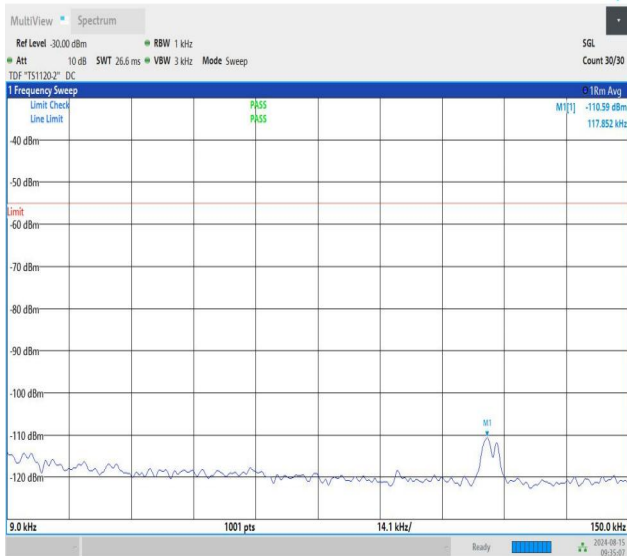
NTNV-n41-PC1.5-30-50-M-CP-QPSK-Edge_1RB_Right-0.009-0.1 5-PASS
