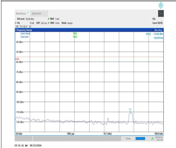
NTNV-n41-PC1.5-30-20-M-CP-QPSK-Edge_1RB_Right-0.009-0.1 5-PASS
