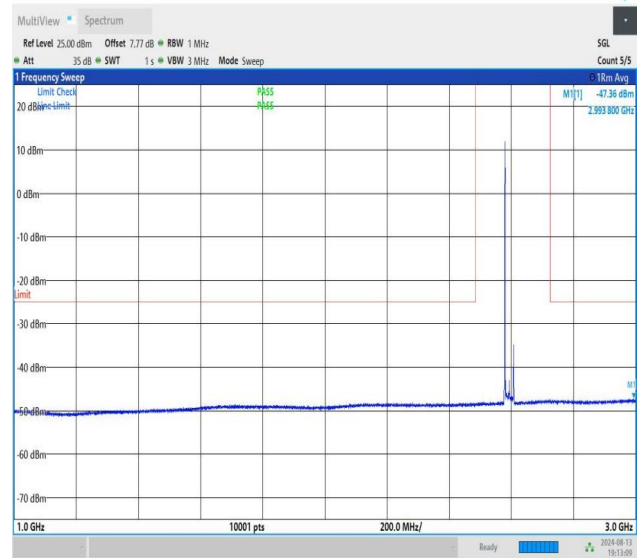
NTNV-n41-PC1.5-30-30-M-CP-QPSK-Edge_1RB_Left-1000-3000-P PASS
