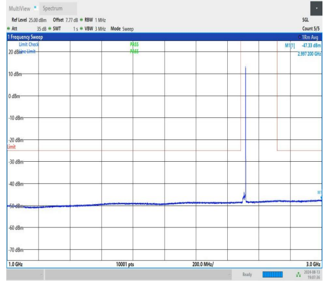
NTNV-n41-PC1.5-30-20-L-CP-QPSK-Edge_1RB_Right-1000-3000- PASS
