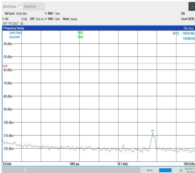
NTNV-n41-PC1.5-30-15-H-CP-QPSK-Edge_1RB_Right-0.009-0.1 5-PASS
