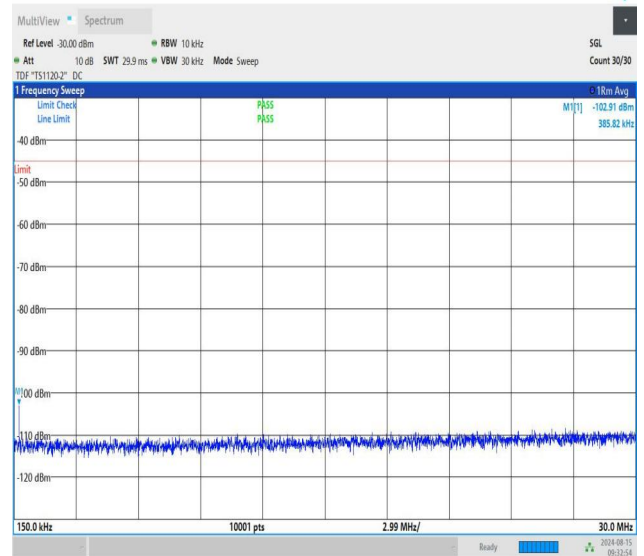
NTNV-n41-PC1.5-30-30-M-CP-QPSK-Edge_1RB_Right-0.15-30-P ASS
