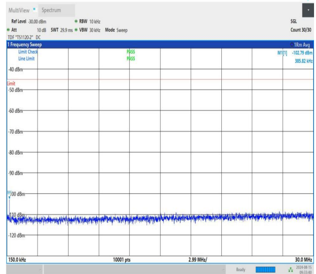
NTNV-n41-PC1.5-30-40-L-CP-QPSK-Edge_1RB_Right-0.15-30-PA SS
