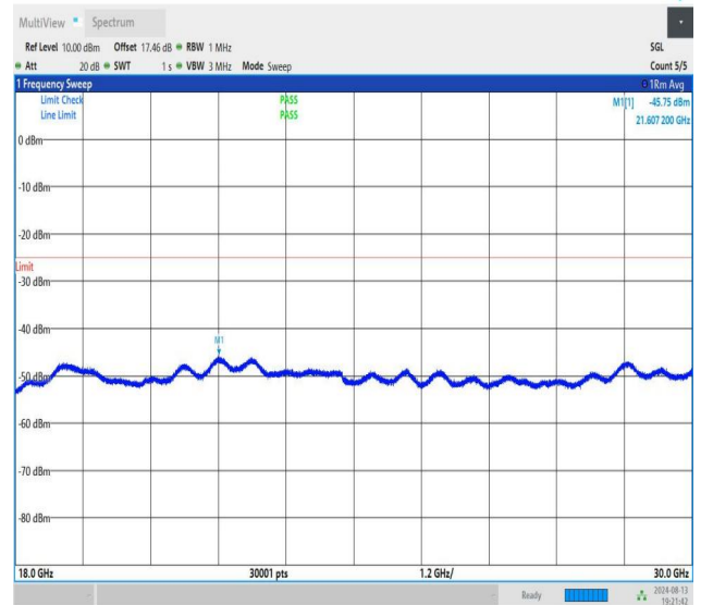
NTNV-n41-PC1.5-30-50-L-CP-QPSK-Edge_1RB_Right-18000-300 00-PASS
