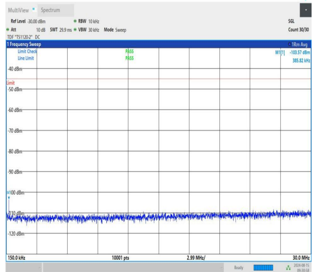
NTNV-n41-PC1.5-30-15-H-CP-QPSK-Edge_1RB_Right-0.15-30-PA SS
