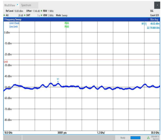
NTNV-n41-PC1.5-30-40-L-CP-QPSK-Edge_1RB_Right-18000-300 00-PASS
