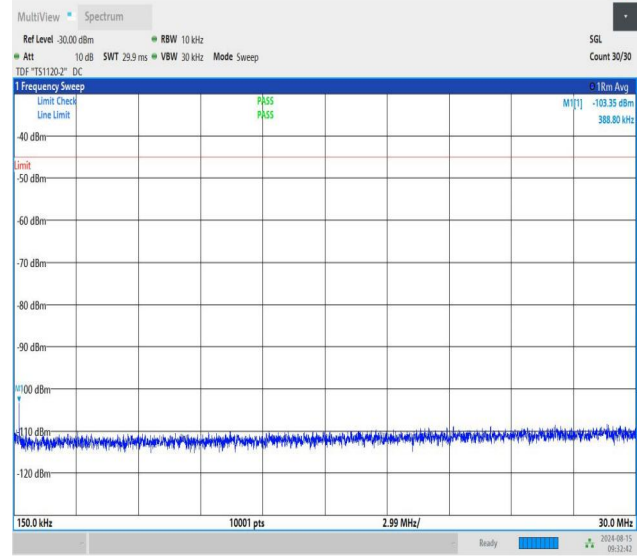
NTNV-n41-PC1.5-30-30-M-CP-QPSK-Edge_1RB_Left-0.15-30-PA SS
