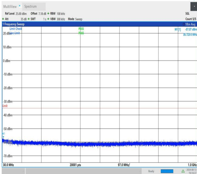
NTNV-n41-PC1.5-30-30-H-CP-QPSK-Edge_1RB_Left-30-1000-PASS
