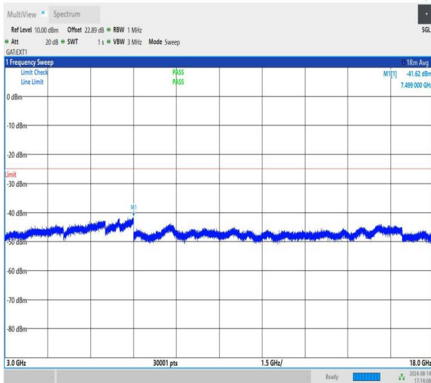
NTNV-n41-PC1.5-30-20-L-CP-QPSK-Edge_1RB_Right-3000-180 00-PASS
