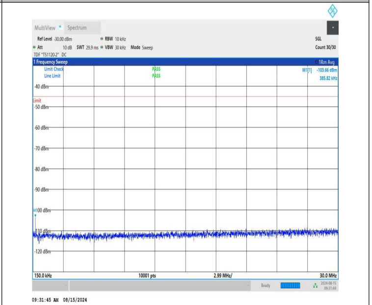
NTNV-n41-PC1.5-30-20-M-CP-QPSK-Edge_1RB_Right-0.15-30-P ASS
