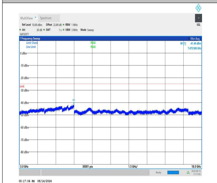
NTNV-n41-PC1.5-30-30-L-CP-QPSK-Edge_1RB_Right-3000-180 00-PASS
