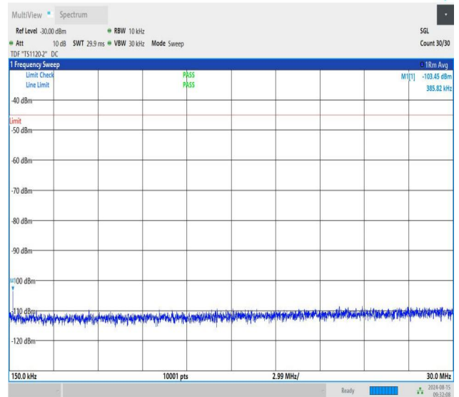
NTNV-n41-PC1.5-30-20-H-CP-QPSK-Edge_1RB_Right-0.15-30-PA SS
