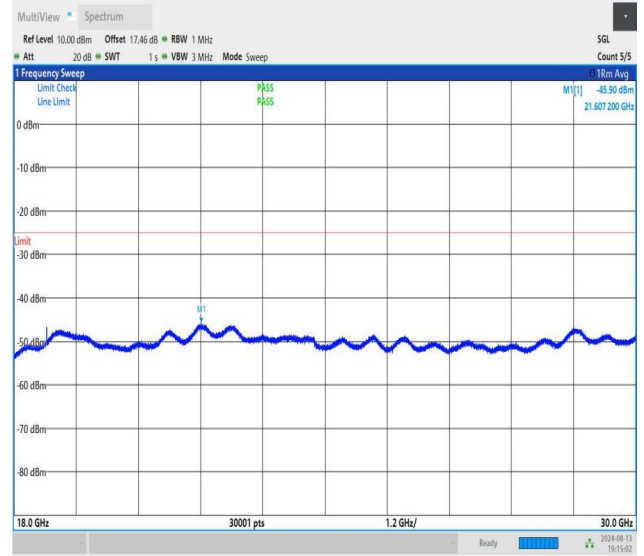
NTNV-n41-PC1.5-30-30-H-CP-QPSK-Edge_1RB_Left-18000-3000 0-PASS
