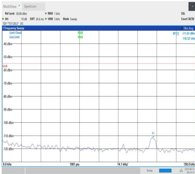
NTNV-n41-PC1.5-30-30-H-CP-QPSK-Edge_1RB_Right-0.009-0.1 5-PASS
