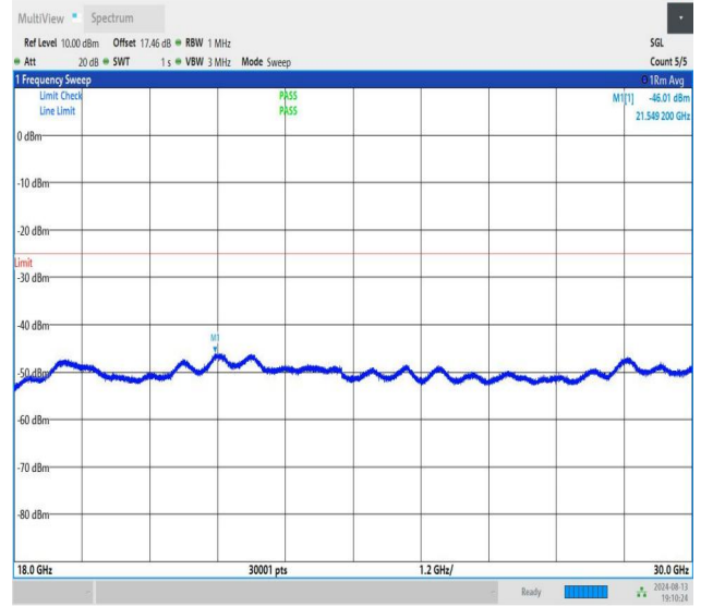
NTNV-n41-PC1.5-30-20-H-CP-QPSK-Edge_1RB_Left-18000-3000 0-PASS
