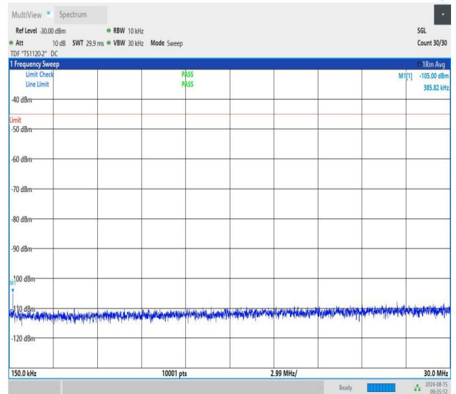
NTNV-n41-PC1.5-30-50-M-CP-QPSK-Edge_1RB_Right-0.15-30-P ASS
