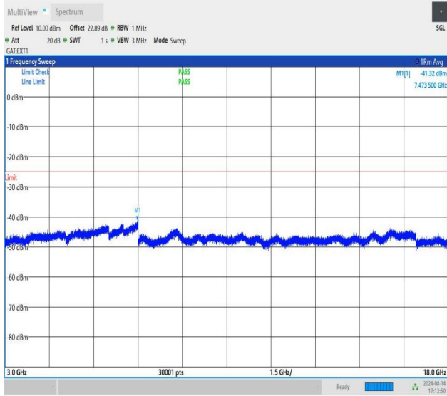
NTNV-n41-PC1.5-30-15-H-CP-QPSK-Edge_1RB_Left-3000-1800 0-PASS
