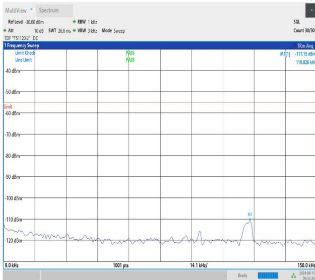
NTNV-n41-PC1.5-30-40-L-CP-QPSK-Edge_1RB_Right-0.009-0.1 5-PASS
