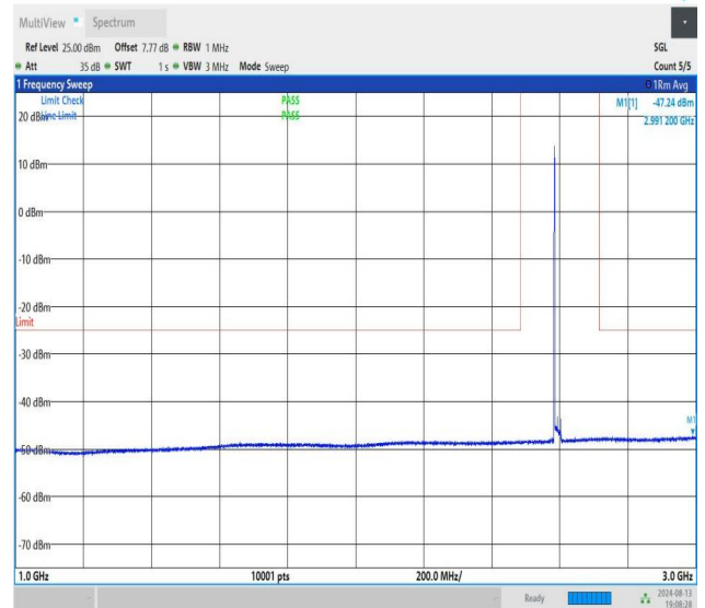
NTNV-n41-PC1.5-30-20-M-CP-QPSK-Edge_1RB_Left-1000-3000-P PASS
