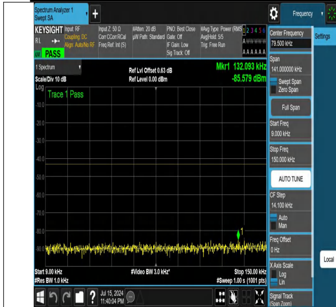
NTNV-DC_12A_n25A-PC3-15-5+15-M+M-N/A-N/A-DFT-QPSK-Edge_1RB_Left-0.009-0.15-PASS
