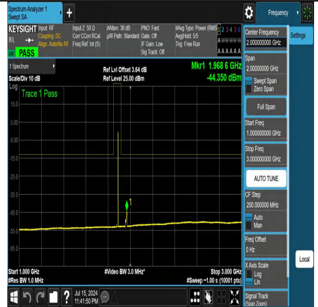
NTNV-DC_12A_n25A-PC3-15-5+15-M+M-N/A-N/A-DFT-QPSK-Edge_1RB_Right-1000-3000-PASS
