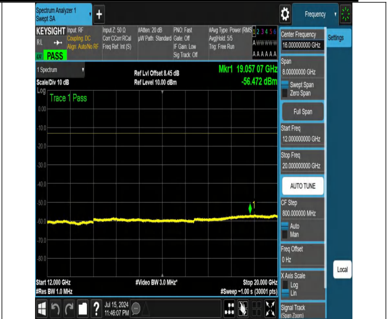
NTNV-DC_12A_n25A-PC3-15-5+15-M+H-N/A-N/A-DFT-QPSK-Edge_1RB_Left-12000-20000-PASS
