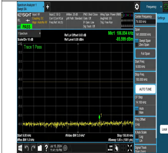
NTNV-DC_12A_n25A-PC3-15-5+15-M+M-N/A-N/A-DFT-QPSK-Edge_1RB_Right-0.009-0.15-PASS
