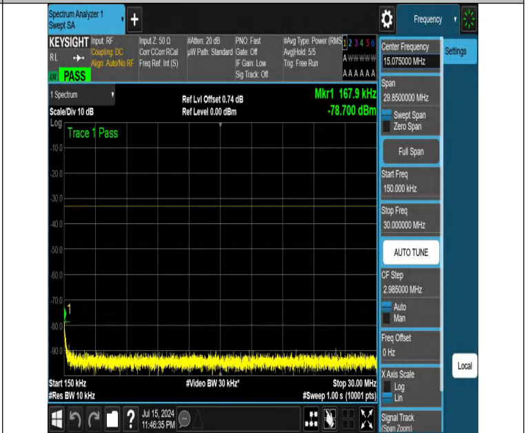
NTNV-DC_12A_n25A-PC3-15-5+15-M+H-N/A-N/A-DFT-QPSK-Edge_1RB_Right-0.15-30-PASS
