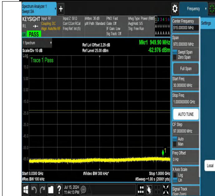
NTNV-DC_12A_n25A-PC3-15-5+15-M+H-N/A-N/A-DFT-PI2BPSK- Edge_1RB_Right-30-1000-PASS
