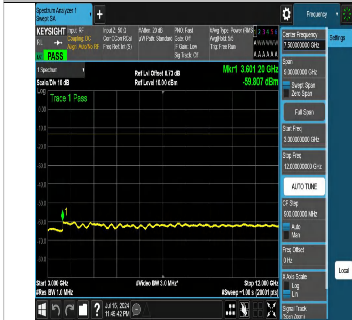
NTNV-DC_12A_n25A-PC3-15-5+20-M+L-N/A-N/A-DFT-PI2BPSK-Edge_1RB_Right-3000-12000-PASS
