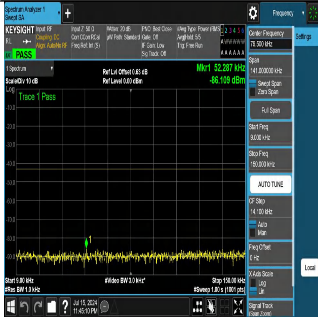
NTNV-DC_12A_n25A-PC3-15-5+15-M+H-N/A-N/A-DFT-QPSK-Edg e_1RB_Left-0.009-0.15-PASS
