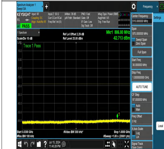
NTNV-DC_12A_n25A-PC3-15-5+15-M+M-N/A-N/A-DFT-QPSK-Edge_1RB_Left-30-1000-PASS
