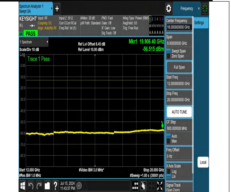
NTNV-DC_12A_n25A-PC3-15-5+15-M+H-N/A-N/A-DFT-PI2BPSK-E dge_1RB_Left-12000-20000-PASS
