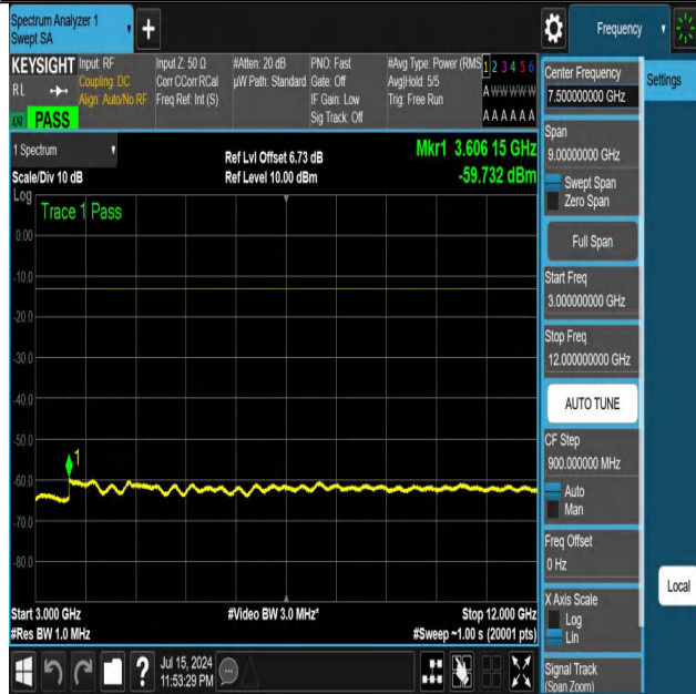
NTNV-DC_12A_n25A-PC3-15-5+20-M+M-N/A-N/A-DFT-PI2BPSK- Edge_1RB_Left-3000-12000-PASS
