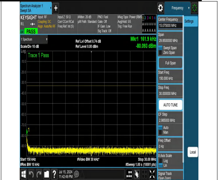
NTNV-DC_12A_n25A-PC3-15-5+15-M+H-N/A-N/A-DFT-PI2BPSK-E dge_1RB_Left-0.15-30-PASS
