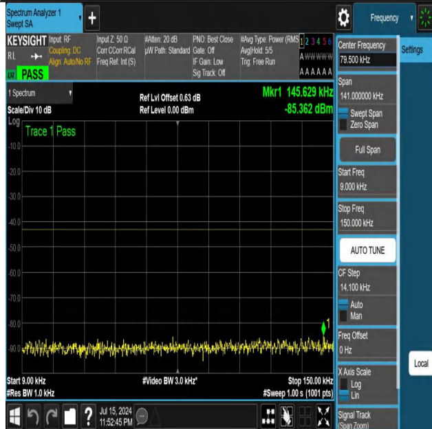
NTNV-DC_12A_n25A-PC3-15-5+20-M+M-N/A-N/A-DFT-PI2BPSK- Edge_1RB_Left-0.009-0.15-PASS
