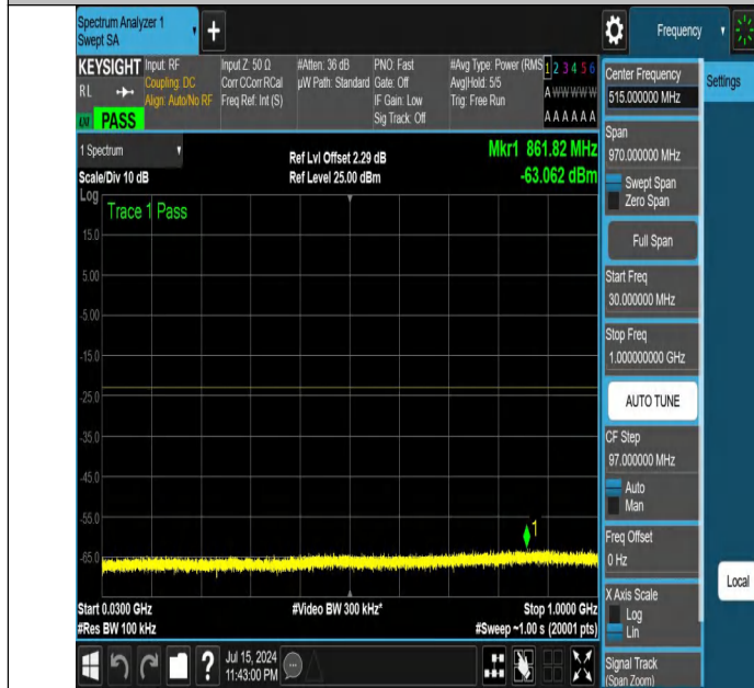
NTNV-DC_12A_n25A-PC3-15-5+15-M+H-N/A-N/A-DFT-PI2BPSK- Edge_1RB_Left-30-1000-PASS
