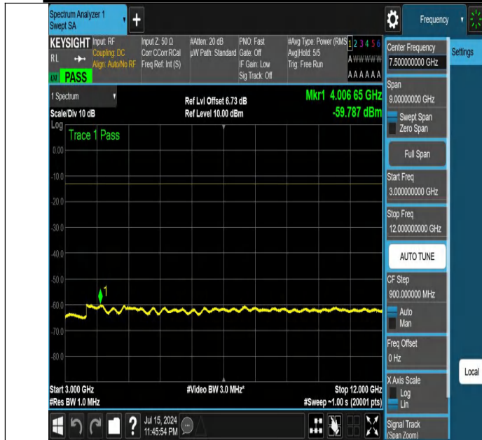
NTNV-DC_12A_n25A-PC3-15-5+15-M+H-N/A-N/A-DFT-QPSK-Edge_1RB_Left-3000-12000-PASS
