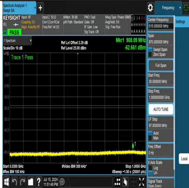
NTNV-DC_12A_n25A-PC3-15-5+20-M+L-N/A-N/A-DFT-QPSK-Edge e_1RB_Right-30-1000-PASS
