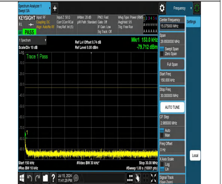
NTNV-DC_12A_n25A-PC3-15-5+15-M+M-N/A-N/A-DFT-QPSK-Edge_1RB_Right-0.15-30-PASS
