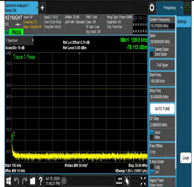
NTNV-DC_12A_n25A-PC3-15-5+15-M+H-N/A-N/A-DFT-QPSK-Edg e_1RB_Left-0.15-30-PASS
