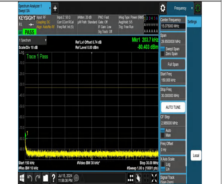
NTNV-DC_12A_n25A-PC3-15-5+20-M+M-N/A-N/A-DFT-QPSK-Edge_1RB_Right-0.15-30-PASS
