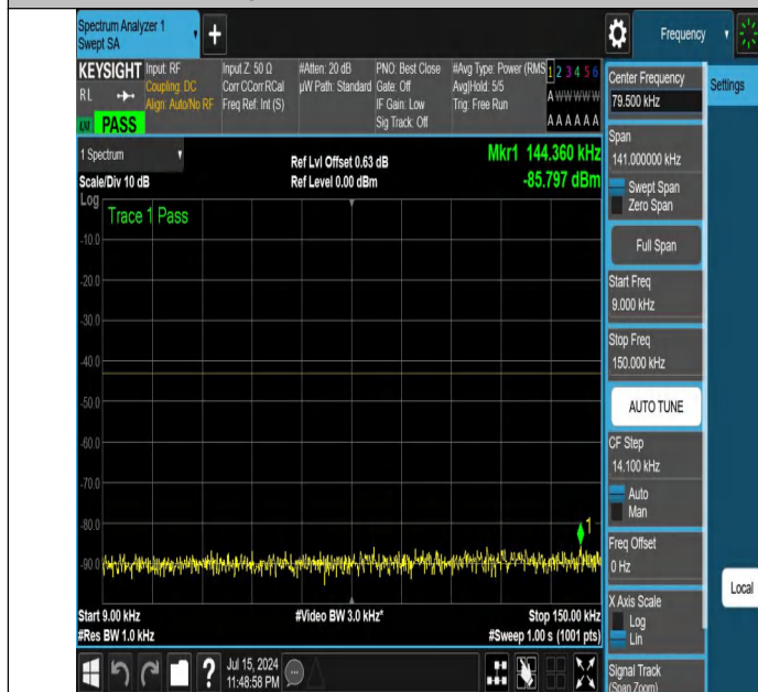
NTNV-DC_12A_n25A-PC3-15-5+20-M+L-N/A-N/A-DFT-PI2BPSK-Edge_1RB_Right-0.009-0.15-PASS
