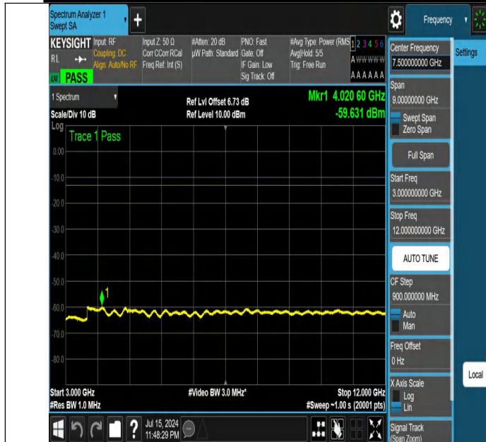
NTNV-DC_12A_n25A-PC3-15-5+20-M+L-N/A-N/A-DFT-PI2BPSK-Edge_1RB_Left-3000-12000-PASS
