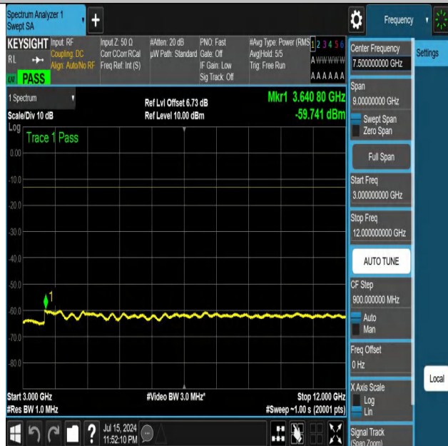
NTNV-DC_12A_n25A-PC3-15-5+20-M+L-N/A-N/A-DFT-QPSK-Edge e_1RB_Right-3000-12000-PASS
