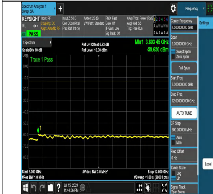
NTNV-DC_12A_n25A-PC3-15-5+15-M+H-N/A-N/A-DFT-PI2BPSK- Edge_1RB_Right-3000-12000-PASS
