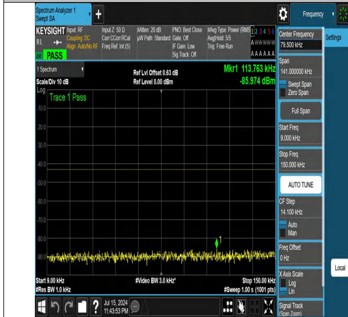
NTNV-DC_12A_n25A-PC3-15-5+15-M+H-N/A-N/A-DFT-PI2BPSK- Edge_1RB_Right-0.009-0.15-PASS
