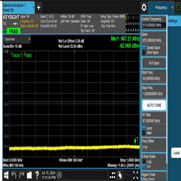
NTNV-DC_12A_n25A-PC3-15-5+15-M+M-N/A-N/A-DFT-QPSK-Edge_1RB_Right-30-1000-PASS
