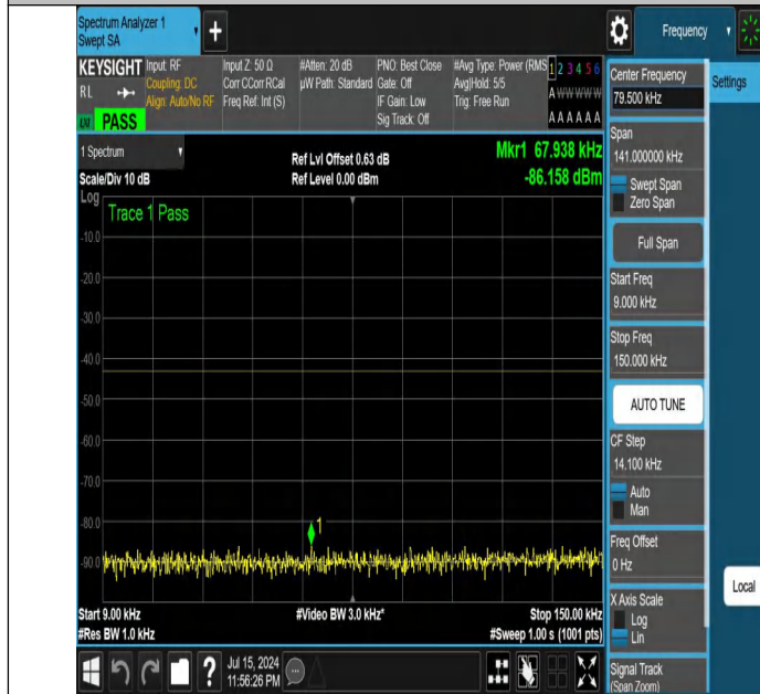
NTNV-DC_12A_n25A-PC3-15-5+20-M+M-N/A-N/A-DFT-QPSK-Edge_1RB_Right-0.009-0.15-PASS
