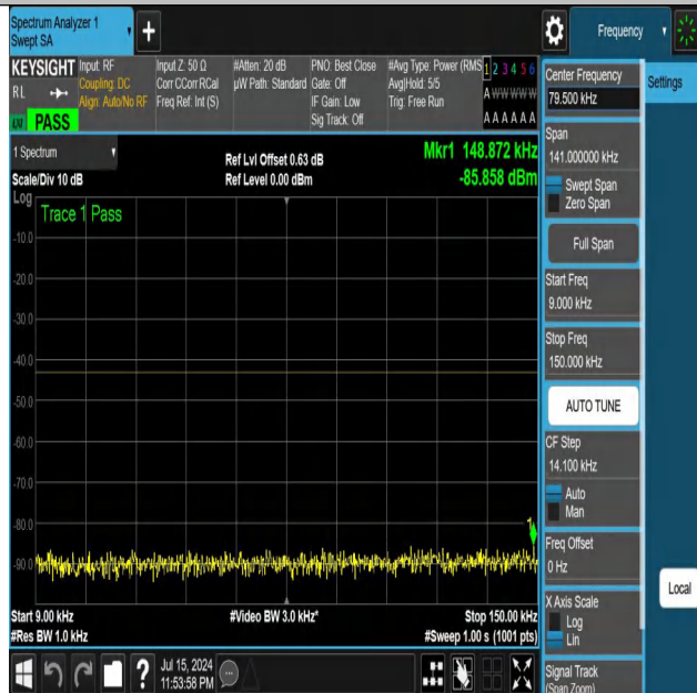
NTNV-DC_12A_n25A-PC3-15-5+20-M+M-N/A-N/A-DFT-PI2BPSK- Edge_1RB_Right-0.009-0.15-PASS
