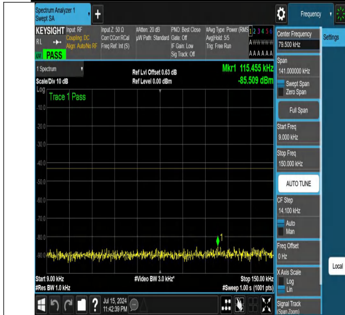
NTNV-DC_12A_n25A-PC3-15-5+15-M+H-N/A-N/A-DFT-PI2BPSK- Edge_1RB_Left-0.009-0.15-PASS
