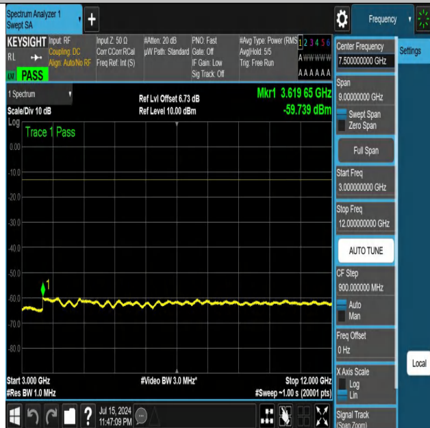
NTNV-DC_12A_n25A-PC3-15-5+15-M+H-N/A-N/A-DFT-QPSK-Edg e_1RB_Right-3000-12000-PASS
