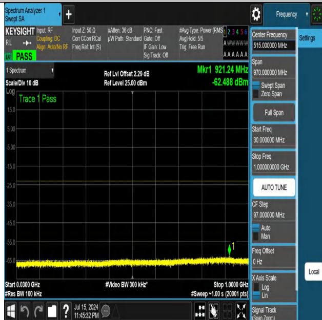
NTNV-DC_12A_n25A-PC3-15-5+15-M+H-N/A-N/A-DFT-QPSK-Edg e_1RB_Left-30-1000-PASS
