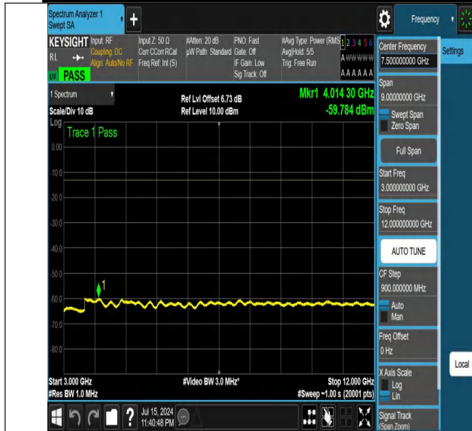
NTNV-DC_12A_n25A-PC3-15-5+15-M+M-N/A-N/A-DFT-QPSK-Edge_1RB_Left-3000-12000-PASS
