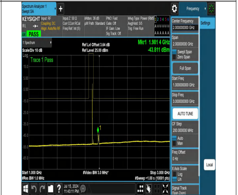
NTNV-DC_12A_n25A-PC3-15-5+15-M+H-N/A-N/A-DFT-PI2BPSK-E dge_1RB_Left-1000-3000-PASS
