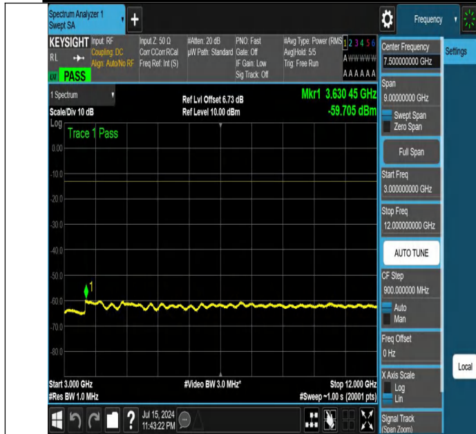
NTNV-DC_12A_n25A-PC3-15-5+15-M+H-N/A-N/A-DFT-PI2BPSK- Edge_1RB_Left-3000-12000-PASS
