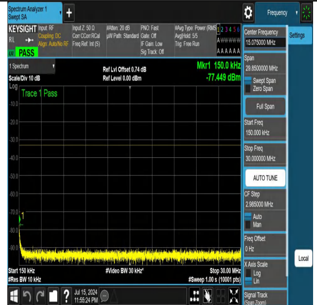
NTNV-DC_12A_n25A-PC3-15-5+20-M+M-N/A-N/A-DFT-QPSK-Edge_1RB_Left-0.15-30-PASS
