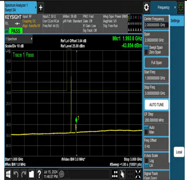
NTNV-DC_12A_n25A-PC3-15-5+15-M+H-N/A-N/A-DFT-QPSK-Edg e_1RB_Right-1000-3000-PASS
