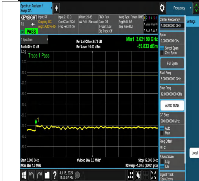
NTNV-DC_12A_n25A-PC3-15-5+20-M+M-N/A-N/A-DFT-QPSK-Edge_1RB_Left-3000-12000-PASS
