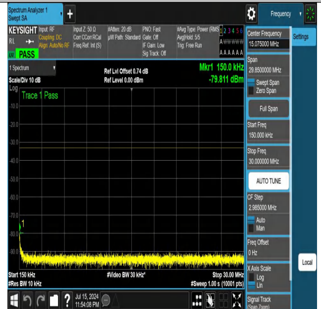
NTNV-DC_12A_n25A-PC3-15-5+20-M+M-N/A-N/A-DFT-PI2BPSK-E dge_1RB_Right-0.15-30-PASS
