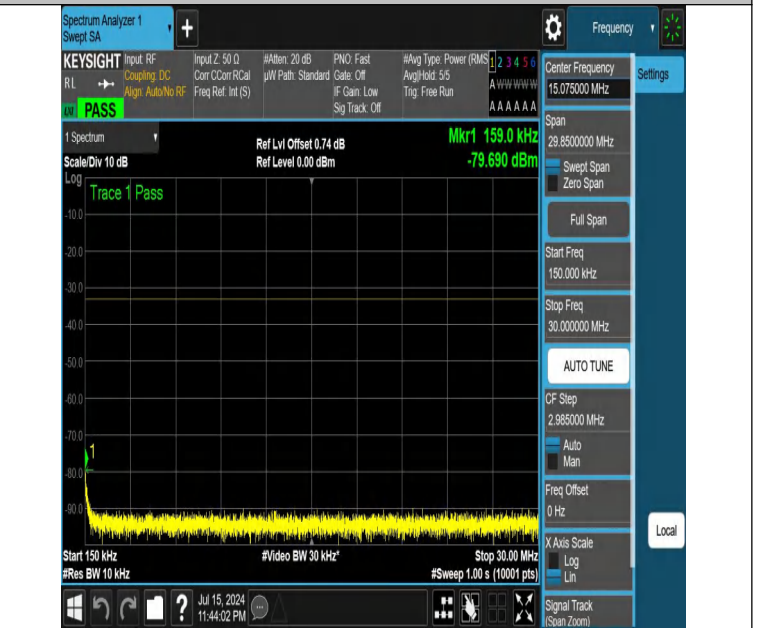
NTNV-DC_12A_n25A-PC3-15-5+15-M+H-N/A-N/A-DFT-PI2BPSK-E dge_1RB_Right-0.15-30-PASS
