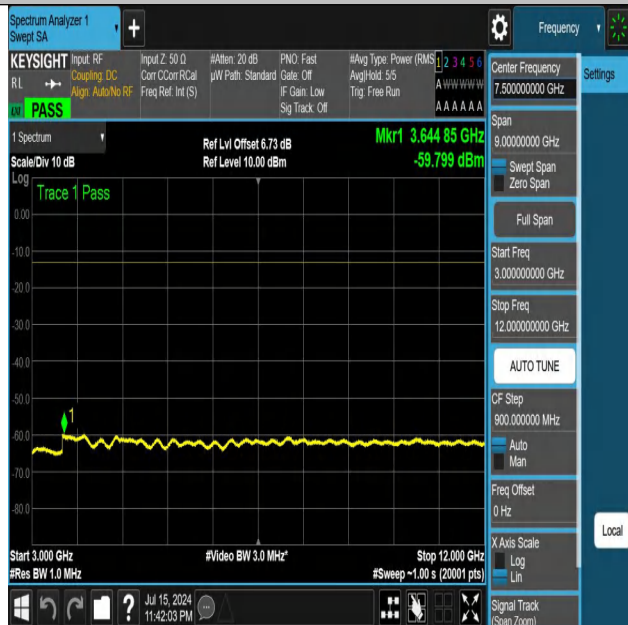
NTNV-DC_12A_n25A-PC3-15-5+15-M+M-N/A-N/A-DFT-QPSK-Edge_1RB_Right-3000-12000-PASS
