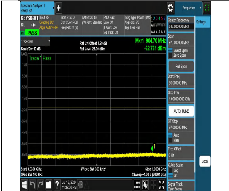
NTNV-DC_12A_n25A-PC3-15-5+15-M+M-N/A-N/A-DFT-PI2BPSK-Edge_1RB_Right-30-1000-PASS
