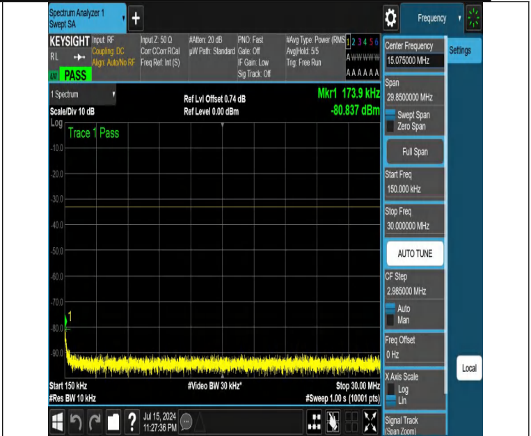
NTNV-DC_12A_n25A-PC3-15-5+10-M+H-N/A/N/A-DFT-PI2BPSK-E dge_1RB_Left-0.15-30-PASS
