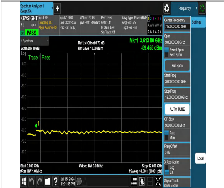
NTNV-DC_12A_n25A-PC3-15-5+10-M+H-N/A-N/A-DFT-QPSK-Edge e_1RB_Right-3000-12000-PASS
