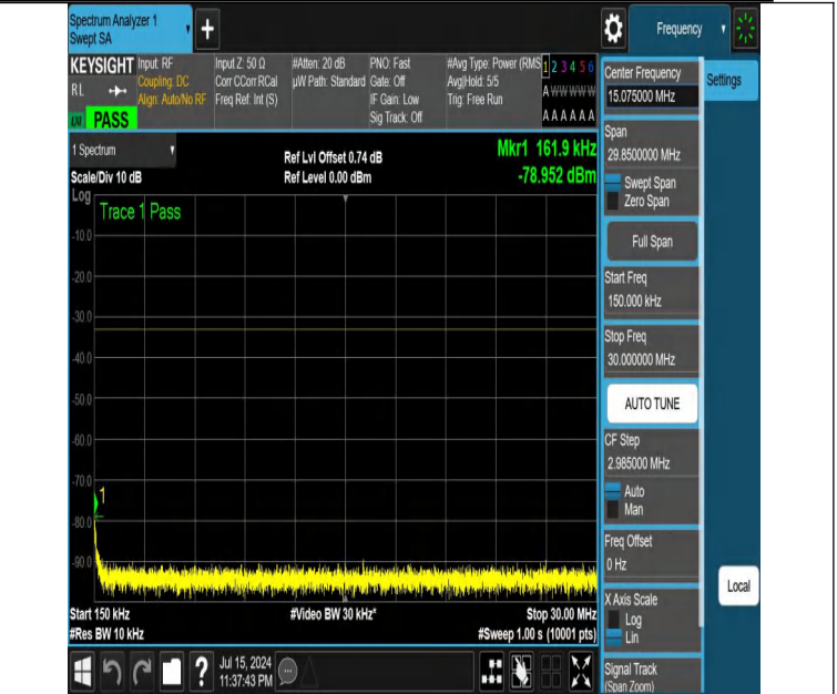
NTNV-DC_12A_n25A-PC3-15-5+15-M+M-N/A-N/A-DFT-PI2BPSK-E dge_1RB_Left-0.15-30-PASS
