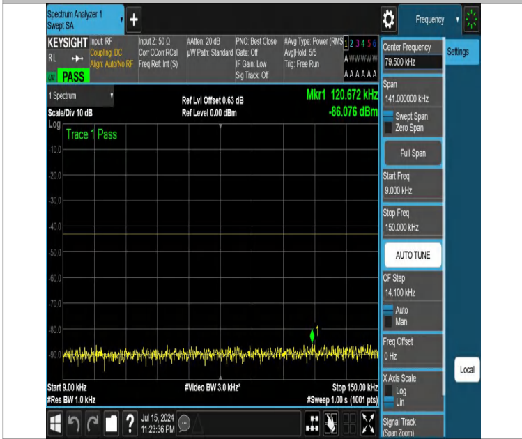
NTNV-DC_12A_n25A-PC3-15-5+10-M+M-N/A-N/A-DFT-PI2BPSK-Edge_1RB_Right-0.009-0.15-PASS
