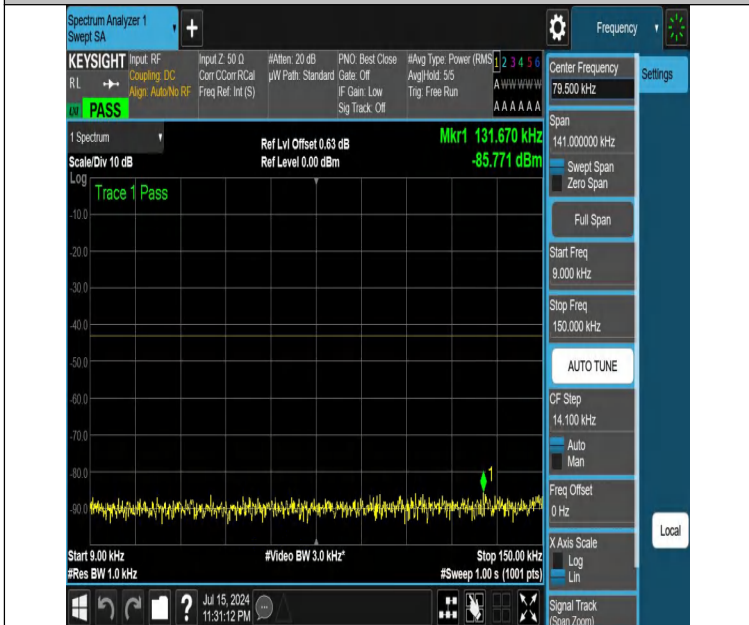
NTNV-DC_12A_n25A-PC3-15-5+10-M+H-N/A-N/A-DFT-QPSK-Edge e_1RB_Right-0.009-0.15-PASS
