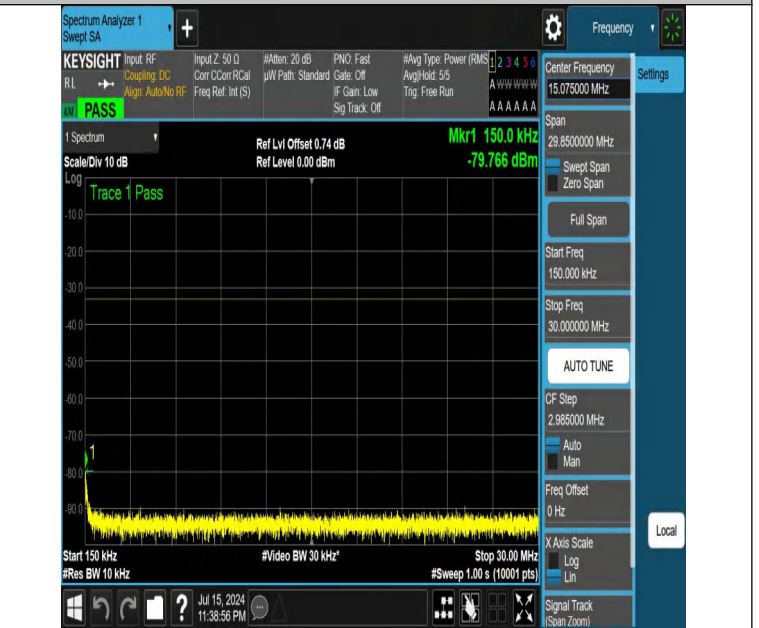
NTNV-DC_12A_n25A-PC3-15-5+15-M+M-N/A-N/A-DFT-PI2BPSK-E dge_1RB_Right-0.15-30-PASS
