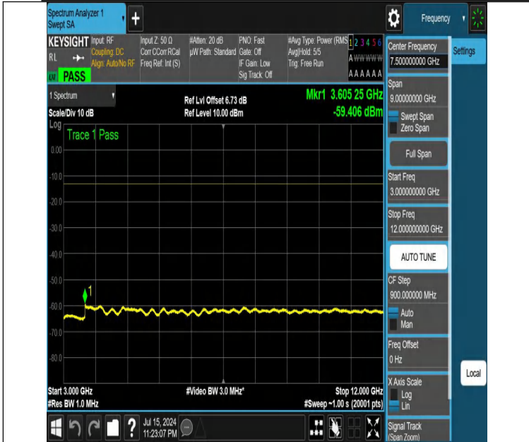
NTNV-DC_12A_n25A-PC3-15-5+10-M+M-N/A-N/A-DFT-PI2BPSK-Edge_1RB_Left-3000-12000-PASS
