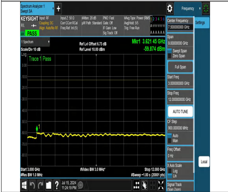
NTNV-DC_12A_n25A-PC3-15-5+10-M+M-N/A-N/A-DFT-PI2BPSK-Edge_1RB_Right-3000-12000-PASS
