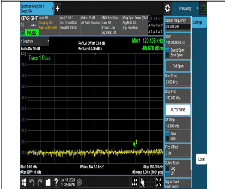
NTNV-DC_12A_n25A-PC3-15-5+15-M+L-N/A-N/A-DFT-PI2BPSK-Edge_1RB_Right-0.009-0.15-PASS
