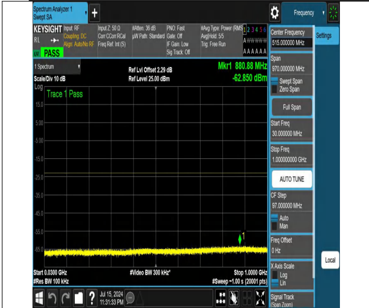
NTNV-DC_12A_n25A-PC3-15-5+10-M+H-N/A-N/A-DFT-QPSK-Edge e_1RB_Right-30-1000-PASS
