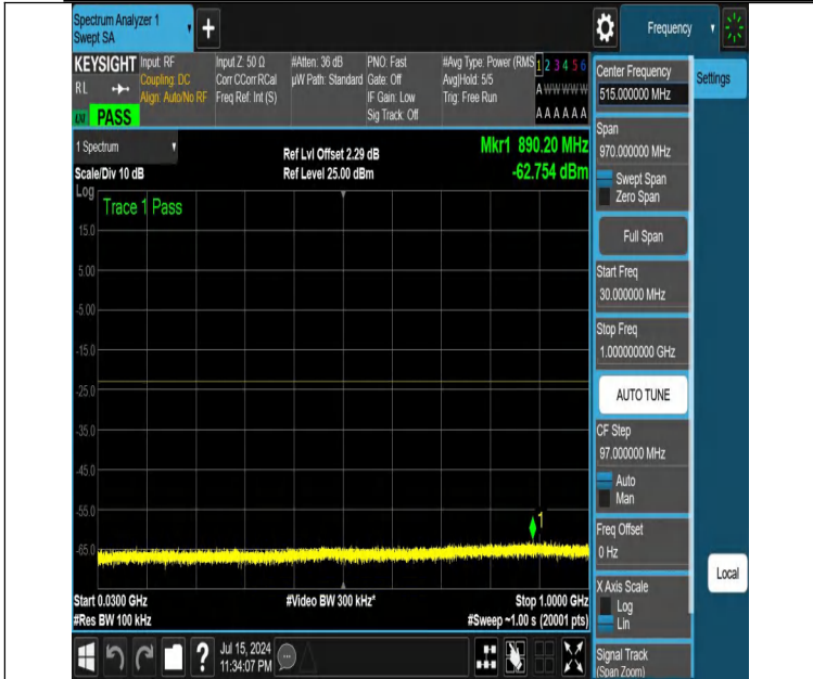
NTNV-DC_12A_n25A-PC3-15-5+15-M+L-N/A-N/A-DFT-PI2BPSK-Edge_1RB_Right-30-1000-PASS
