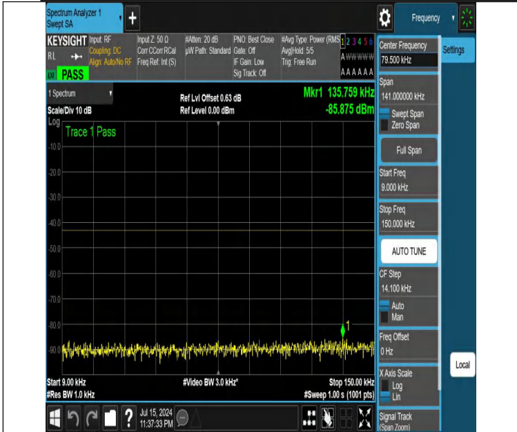
NTNV-DC_12A_n25A-PC3-15-5+15-M+M-N/A-N/A-DFT-PI2BPSK-Edge_1RB_Left-0.009-0.15-PASS
