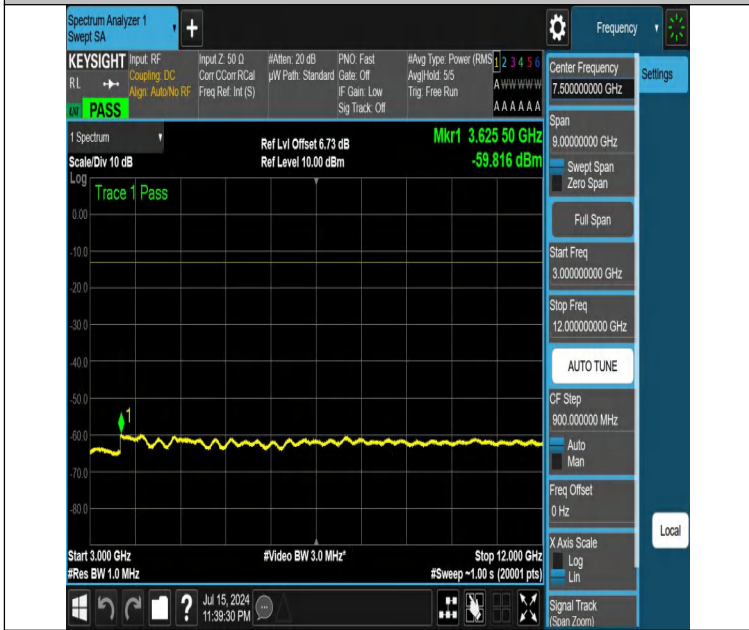
NTNV-DC_12A_n25A-PC3-15-5+15-M+M-N/A-N/A-DFT-PI2BPSK-Edge_1RB_Right-3000-12000-PASS
