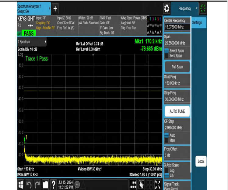
NTNV-DC_12A_n25A-PC3-15-5+10-M+H-N/A-N/A-DFT-QPSK-Edge e_1RB_Right-0.15-30-PASS
