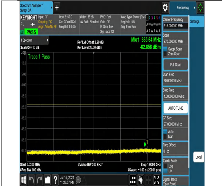
NTNV-DC_12A_n25A-PC3-15-5+10-M+M-N/A-N/A-DFT-PI2BPSK-Edge_1RB_Right-30-1000-PASS
