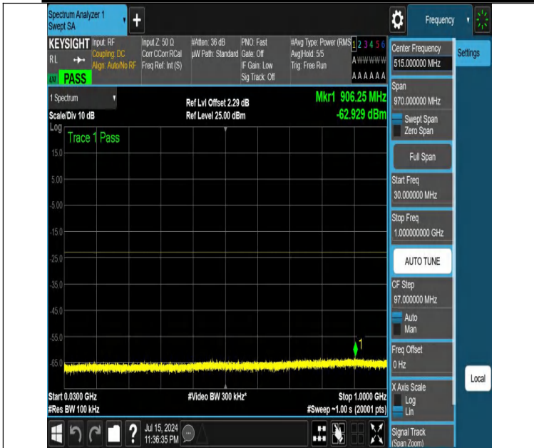
NTNV-DC_12A_n25A-PC3-15-5+15-M+L-N/A-N/A-DFT-QPSK-Edge e_1RB_Right-30-1000-PASS
