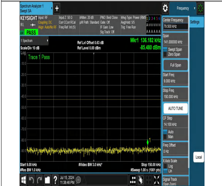
NTNV-DC_12A_n25A-PC3-15-5+15-M+M-N/A-N/A-DFT-PI2BPSK-Edge_1RB_Right-0.009-0.15-PASS
