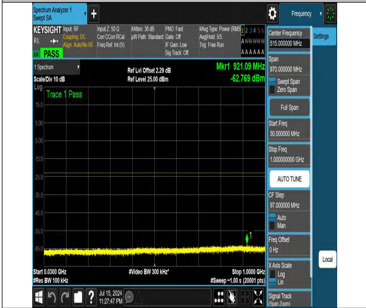
NTNV-DC_12A_n25A-PC3-15-5+10-M+H-N/A/N/A-DFT-PI2BPSK-Edge_1RB_Left-30-1000-PASS
