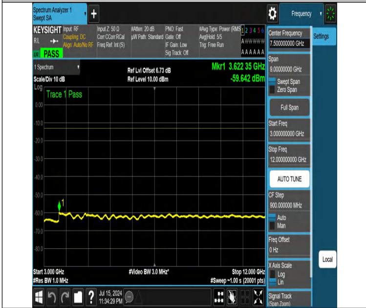
NTNV-DC_12A_n25A-PC3-15-5+15-M+L-N/A-N/A-DFT-PI2BPSK-Edge_1RB_Right-3000-12000-PASS
