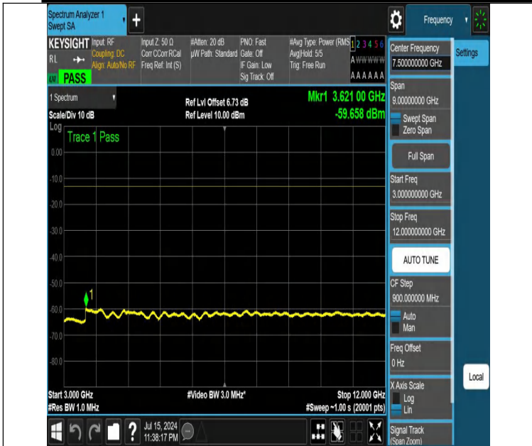
NTNV-DC_12A_n25A-PC3-15-5+15-M+M-N/A-N/A-DFT-PI2BPSK-Edge_1RB_Left-3000-12000-PASS
