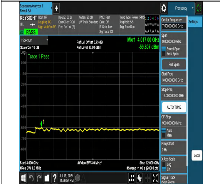
NTNV-DC_12A_n25A-PC3-15-5+15-M+L-N/A-N/A-DFT-QPSK-Edge e_1RB_Right-3000-12000-PASS
