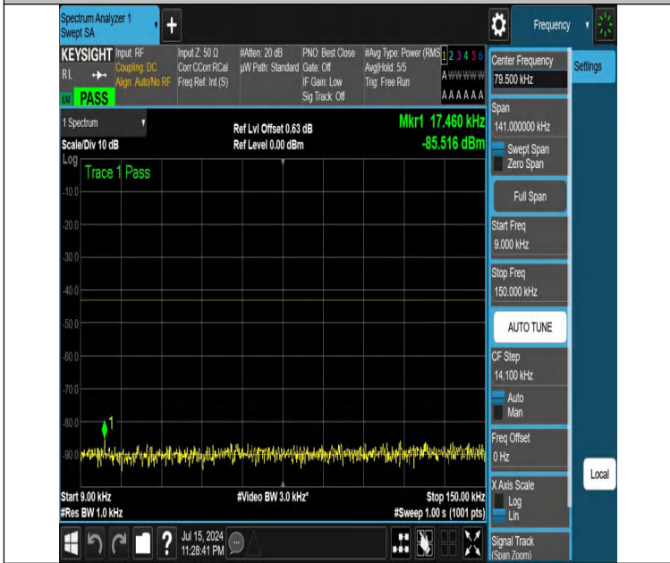
NTNV-DC_12A_n25A-PC3-15-5+10-M+H-N/A-N/A-DFT-PI2BPSK-Edge_1RB_Right-0.009-0.15-PASS
