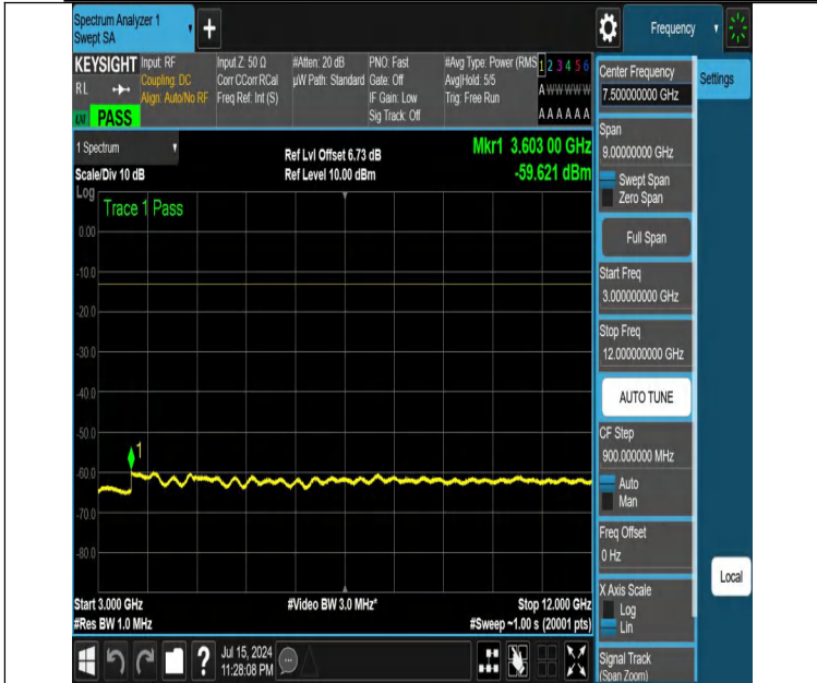
NTNV-DC_12A_n25A-PC3-15-5+10-M+H-N/A-N/A-DFT-PI2BPSK-Edge_1RB_Left-3000-12000-PASS
