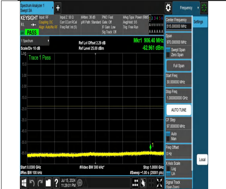
NTNV-DC_12A_n25A-PC3-15-5+10-M+H-N/A-N/A-DFT-PI2BPSK-Edge_1RB_Right-30-1000-PASS
