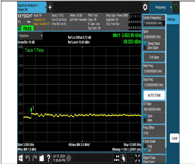
NTNV-DC_12A_n25A-PC3-15-5+10-M+M-N/A-N/A-DFT-QPSK-Edge_1RB_Right-3000-12000-PASS
