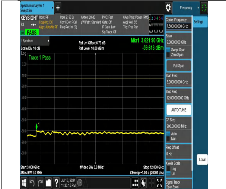
NTNV-DC_12A_n25A-PC3-15-5+15-M+L-N/A-N/A-DFT-PI2BPSK-Edge_1RB_Left-3000-12000-PASS
