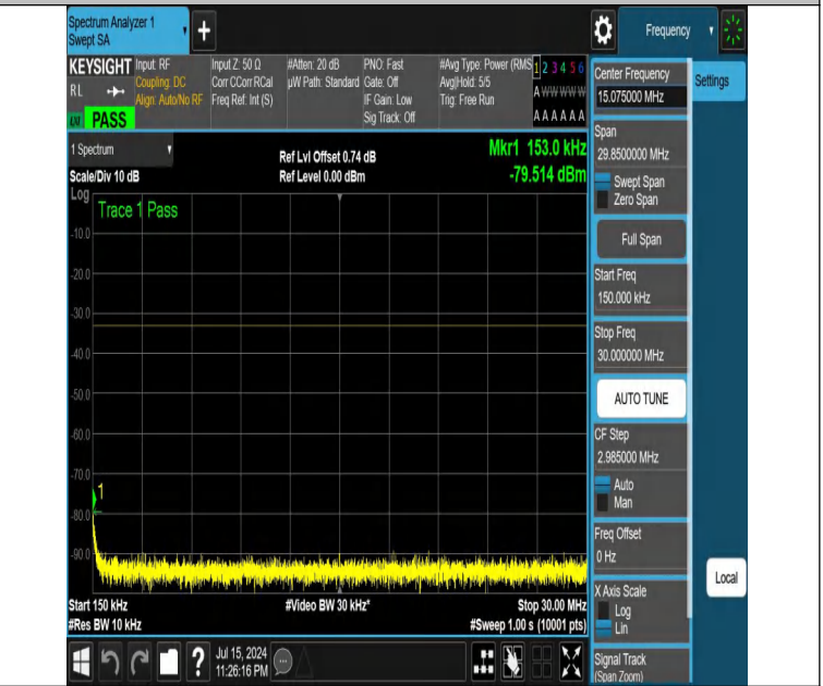
NTNV-DC_12A_n25A-PC3-15-5+10-M+M-N/A-N/A-DFT-QPSK-Edge_1RB_Right-0.15-30-PASS
