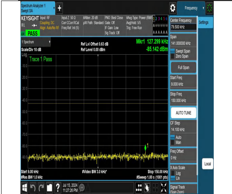
NTNV-DC_12A_n25A-PC3-15-5+10-M+H-N/A/N/A-DFT-PI2BPSK-Edge_1RB_Left-0.009-0.15-PASS
