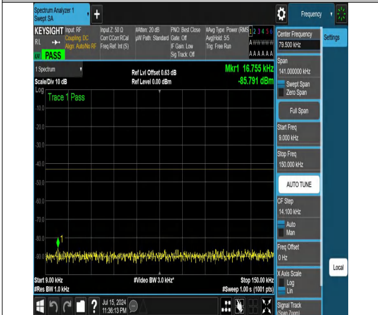
NTNV-DC_12A_n25A-PC3-15-5+15-M+L-N/A-N/A-DFT-QPSK-Edge e_1RB_Right-0.009-0.15-PASS
