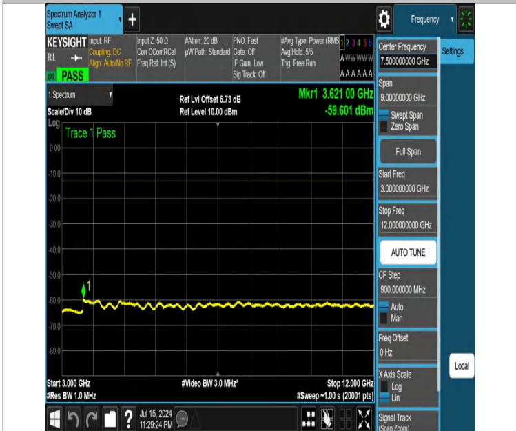
NTNV-DC_12A_n25A-PC3-15-5+10-M+H-N/A-N/A-DFT-PI2BPSK-Edge_1RB_Right-3000-12000-PASS
