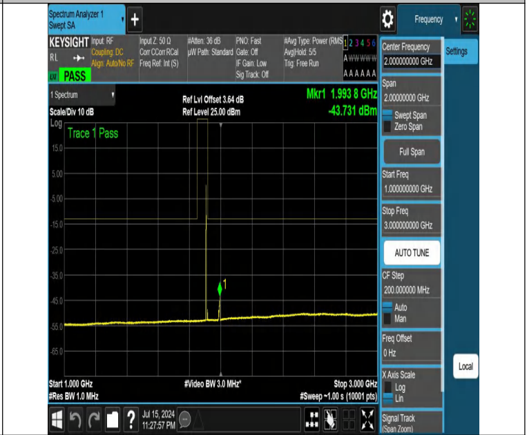
NTNV-DC_12A_n25A-PC3-15-5+10-M+H-N/A/N/A-DFT-PI2BPSK-E dge_1RB_Left-1000-3000-PASS
