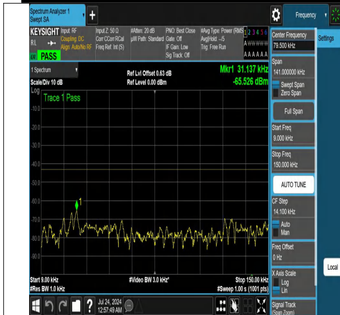
NTNV-N25-PC3-15-25-H-DFT-PI2BPSK-Edge_1RB_Left-0.009-0.15-Ant1-PASS
