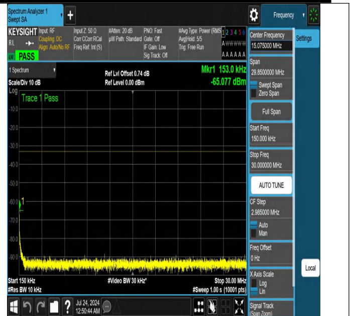
NTNV-N25-PC3-15-25-L-DFT-QPSK-Edge_1RB_Left-0.15-30-Ant1-PASS
