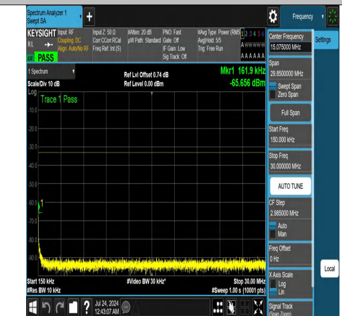
NTNV-N25-PC3-15-20-H-DFT-P12BPSK-Edge_1RB_Right-0.15-3 0-Ant1-PASS
