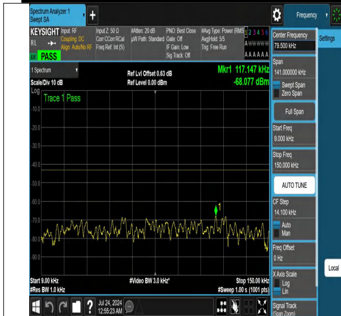
NTNV-N25-PC3-15-25-M-DFT-QPSK-Edge_1RB_Left-0.009-0.15 -Ant1-PASS
