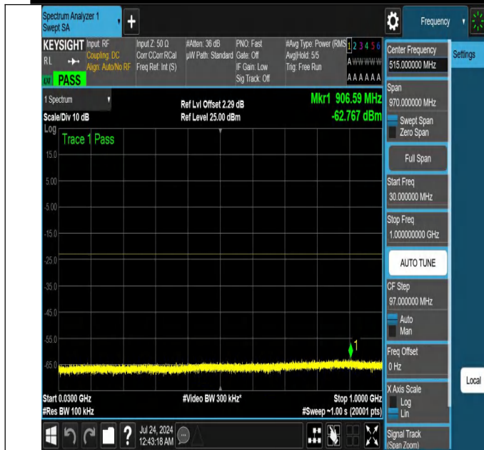
NTNV-N25-PC3-15-20-H-DFT-PI2BPSK-Edge_1RB_Right-30-1000-Ant1-PASS
