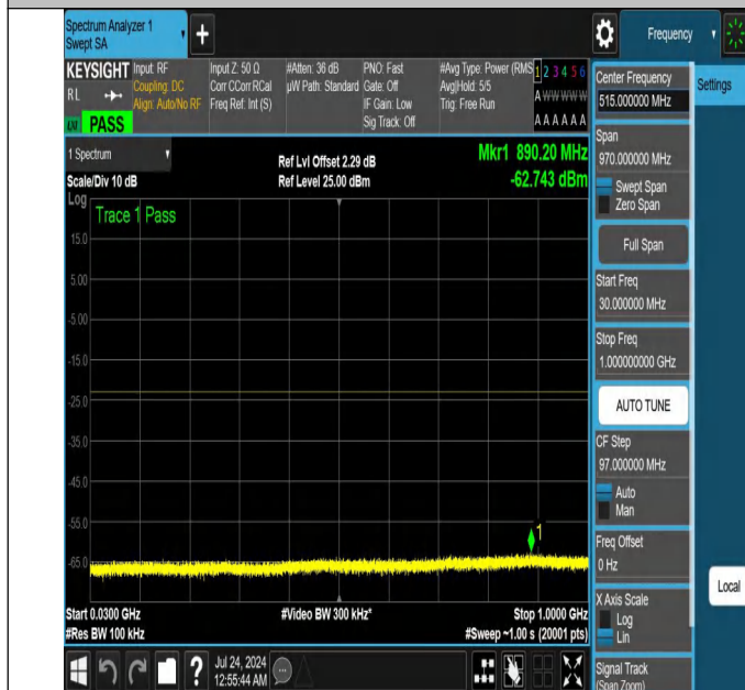
NTNV-N25-PC3-15-25-M-DFT-QPSK-Edge_1RB_Left-30-1000-A nt1-PASS
