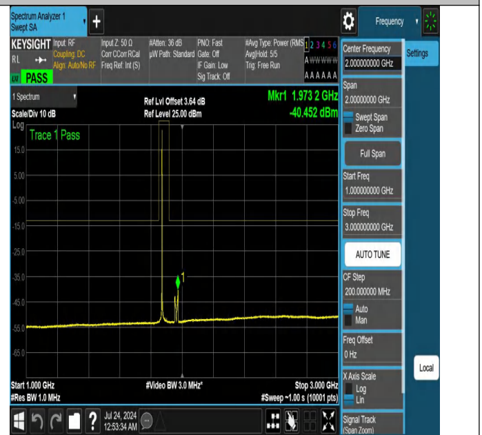
NTNV-N25-PC3-15-25-M-DFT-PI2BPSK-Edge_1RB_Left-1000-3000-Ant1-PASS
