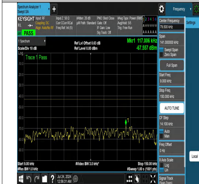
NTN-N25-PC3-15-25-M-DFT-QPSK-Edge_1RB_Right-0.009-0. 15-Ant1-PASS
