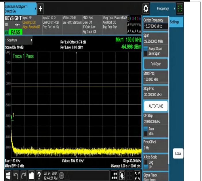
NTNV-N25-PC3-15-20-H-DFT-QPSK-Edge_1RB_Left-0.15-30-Ant 1-PASS
