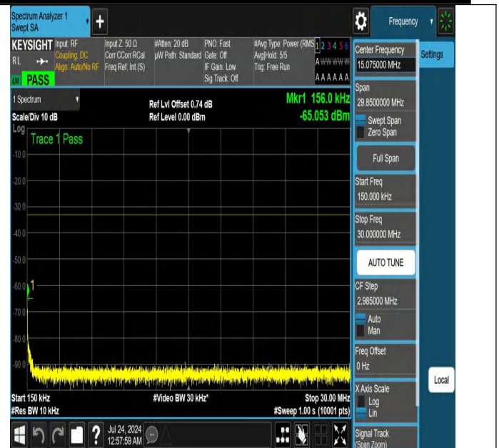
NTNV-N25-PC3-15-25-H-DFT-PI2BPSK-Edge_1RB_Left-0.15-30-Ant1-PASS
