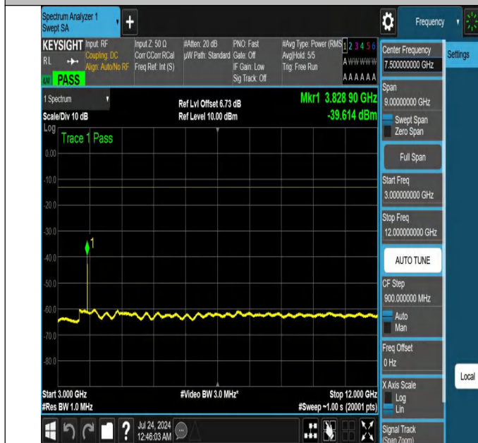
NTN-N25-PC3-15-20-H-DFT-QPSK-Edge_1RB_Right-3000-12000-Ant1-PASS
