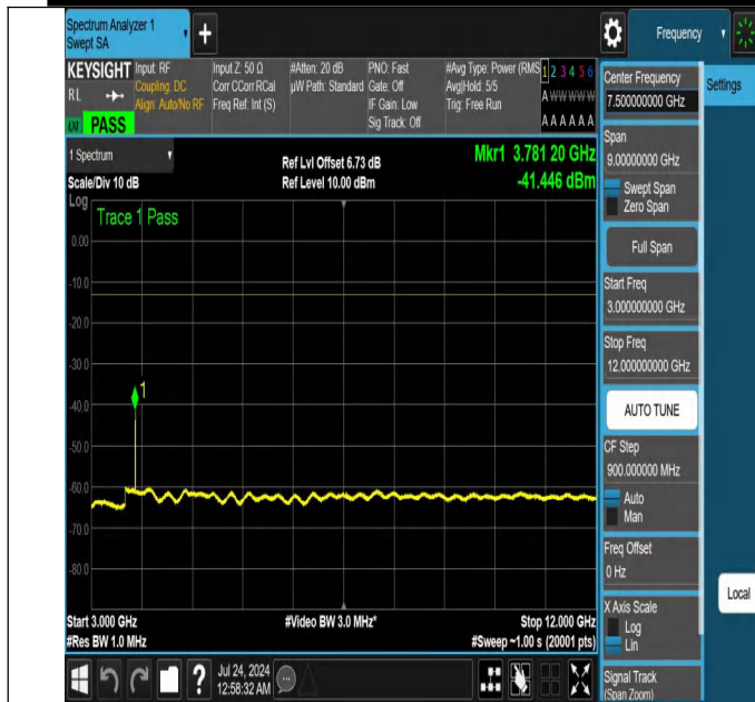
NTNV-N25-PC3-15-25-H-DFT-PI2BPSK-Edge_1RB_Left-3000-1 2000-Ant1-PASS
