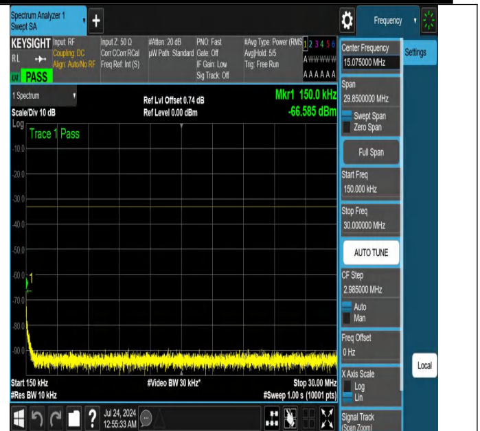
NTNV-N25-PC3-15-25-M-DFT-QPSK-Edge_1RB_Left-0.15-30-Ant 1-PASS
