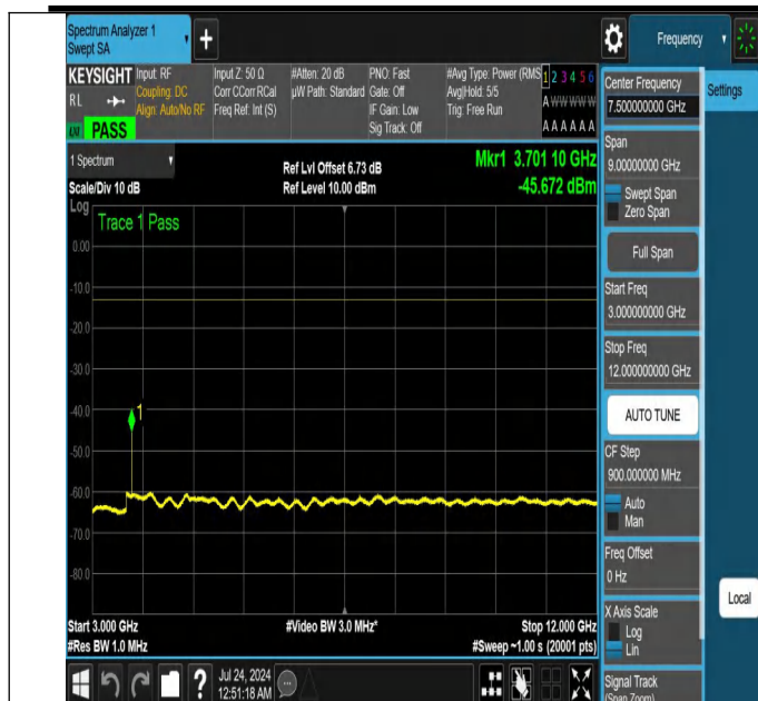
NTNV-N25-PC3-15-25-L-DFT-QPSK-Edge_1RB_Left-3000-1200 0-Ant1-PASS
