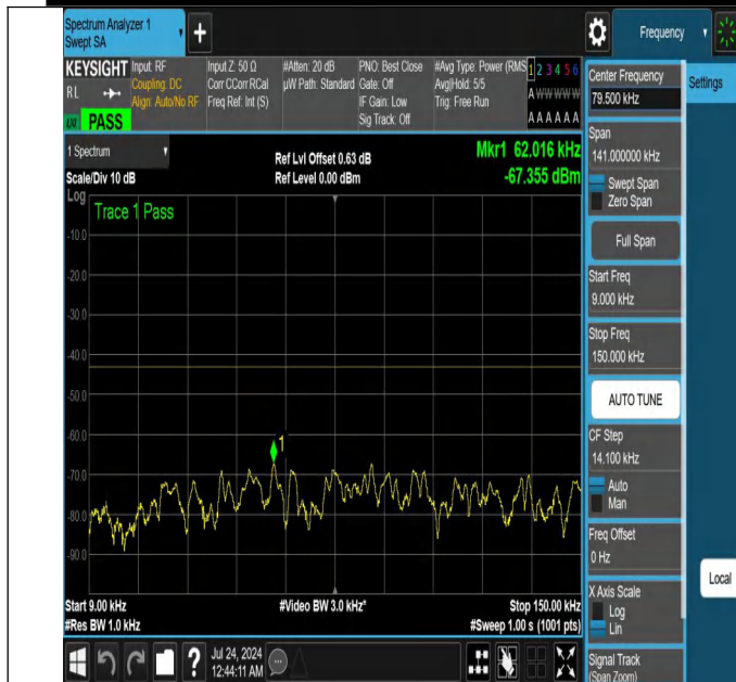
NTNV-N25-PC3-15-20-H-DFT-QPSK-Edge_1RB_Left-0.009-0.15 -Ant1-PASS
