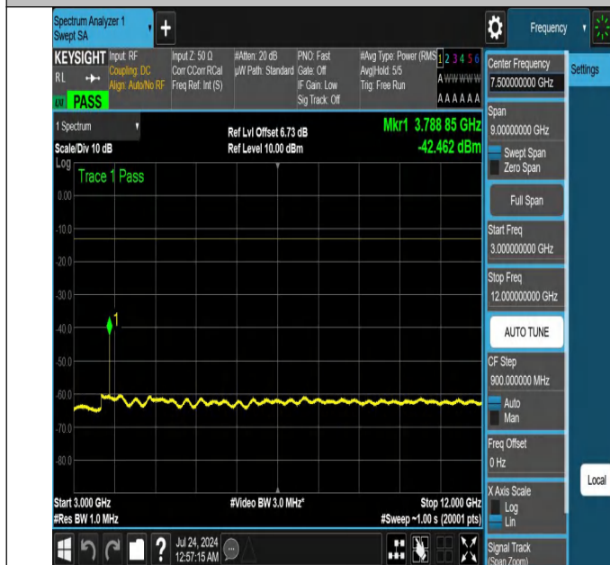
NTNV-N25-PC3-15-25-M-DFT-QPSK-Edge_1RB_Right-3000-12000-Ant1-PASS
