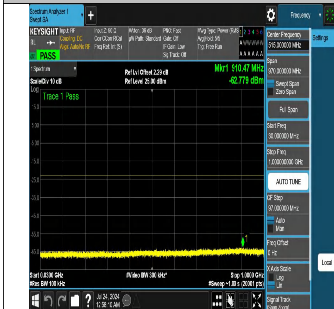
NTNV-N25-PC3-15-25-H-DFT-PI2BPSK-Edge_1RB_Left-30-1000-Ant1-PASS
