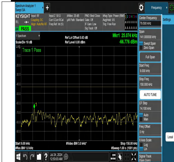
NTNV-N25-PC3-15-25-M-DFT-PI2BPSK-Edge_1RB_Left-0.009-0.15-Ant1-PASS
