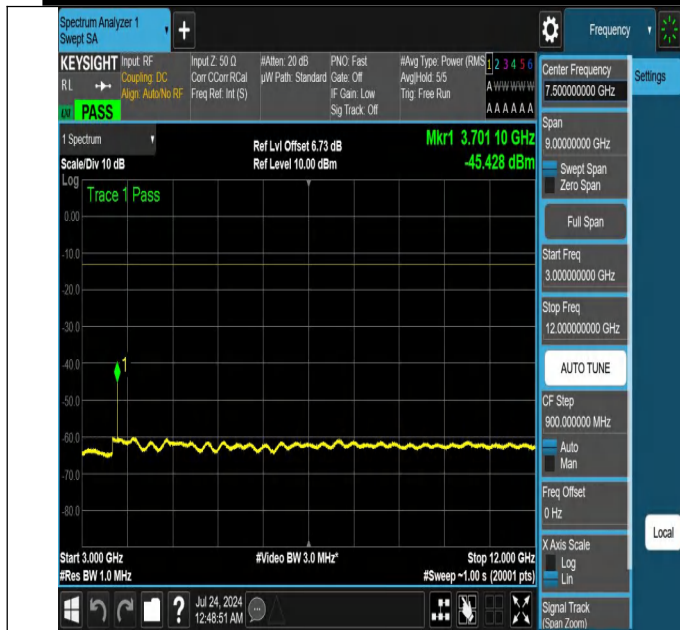
NTN-N25-PC3-15-25-L-DFT-PI2BPSK-Edge_1RB_Left-3000-12000-Ant1-PASS
