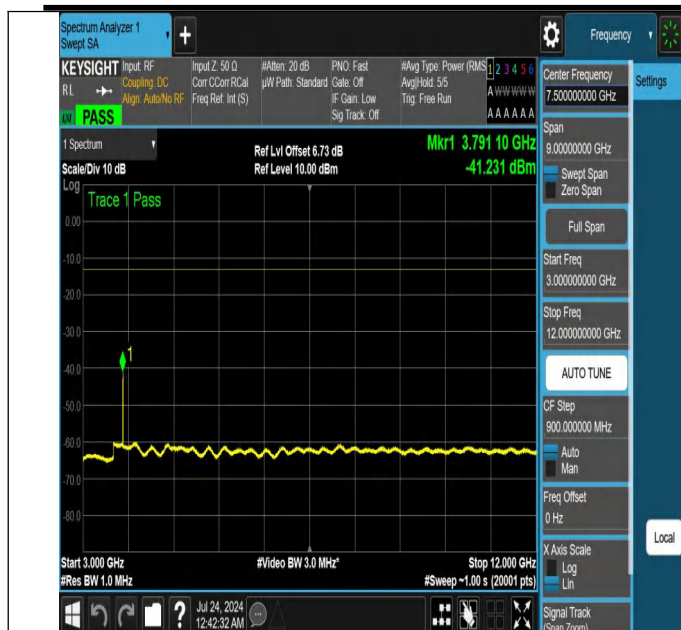
NTNV-N25-PC3-15-20-H-DFT-PI2BPSK-Edge_1RB_Left-3000-1 2000-Ant1-PASS
