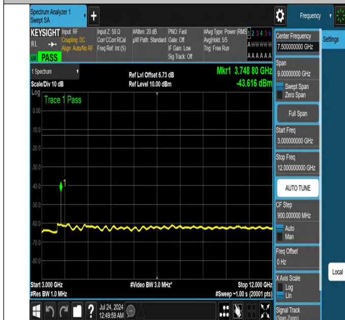
NTNV-N25-PC3-15-25-L-DFT-PI2BPSK-Edge_1RB_Right-3000-12000-Ant1-PASS
