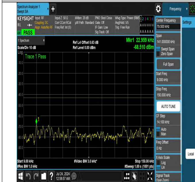
NTNV-N25-PC3-15-25-H-DFT-PI2BPSK-Edge_1RB_Right-0.009- 0.15-Ant1-PASS
