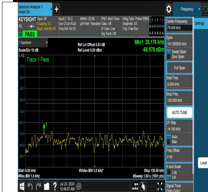
NTNV-N25-PC3-15-25-L-DFT-PI2BPSK-Edge_1RB_Left-0.009-0.15-Ant1-PASS
