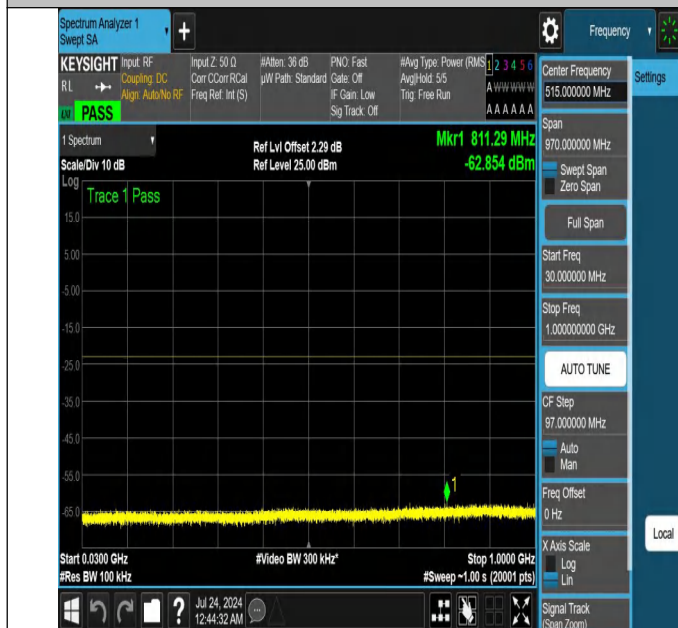
NTNV-N25-PC3-15-20-H-DFT-QPSK-Edge_1RB_Left-30-1000-A nt1-PASS
