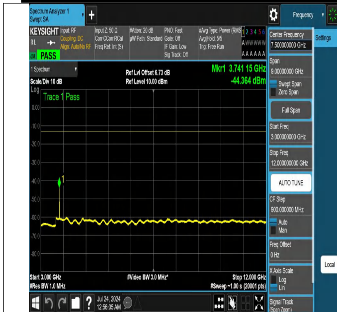
NTN-N25-PC3-15-25-M-DFT-QPSK-Edge_1RB_Left-3000-1200 0-Ant1-PASS
