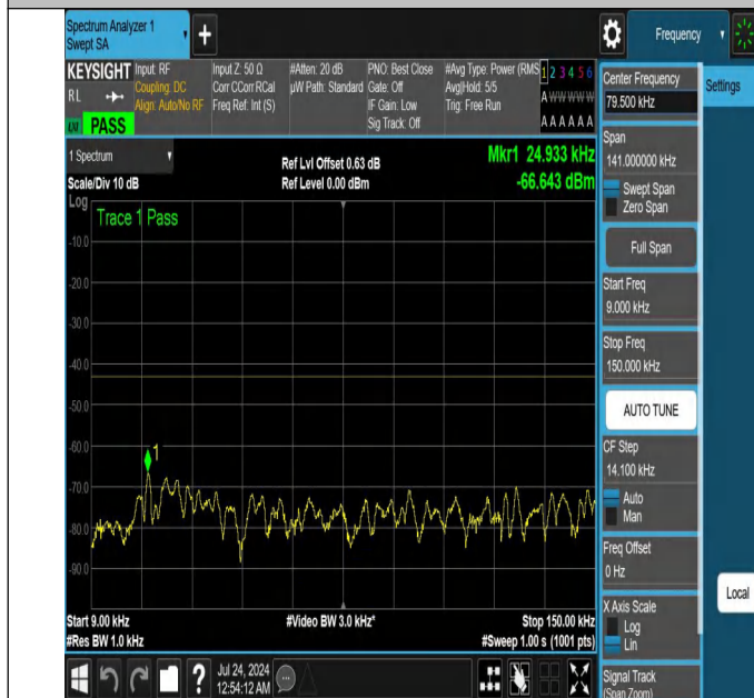
NTNV-N25-PC3-15-25-M-DFT-PI2BPSK-Edge_1RB_Right-0.009 -0.15-Ant1-PASS
