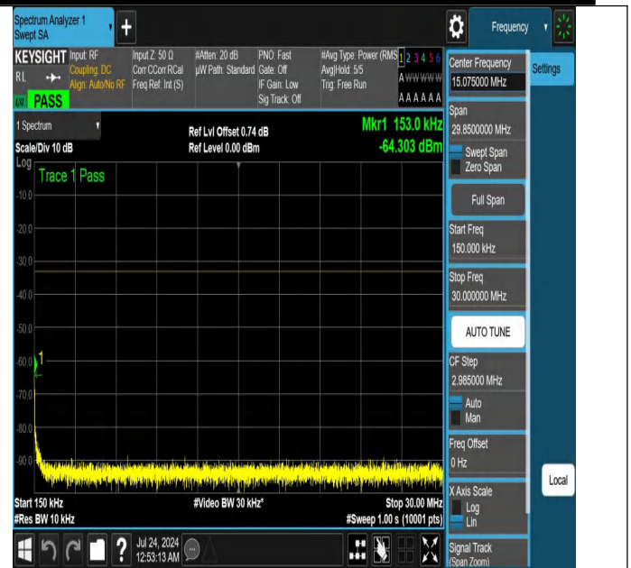
NTNV-N25-PC3-15-25-M-DFT-PI2BPSK-Edge_1RB_Left-0.15-30-Ant1-PASS
