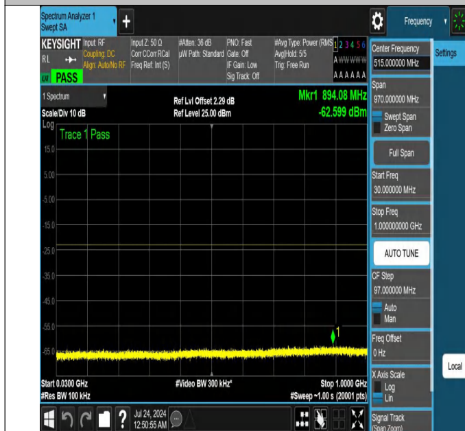
NTNV-N25-PC3-15-25-L-DFT-QPSK-Edge_1RB_Left-30-1000-Ant1-PASS
