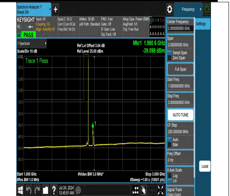
NTN-N25-PC3-15-20-H-DFT-QPSK-Edge_1RB_Right-1000-300-0-Ant1-PASS
