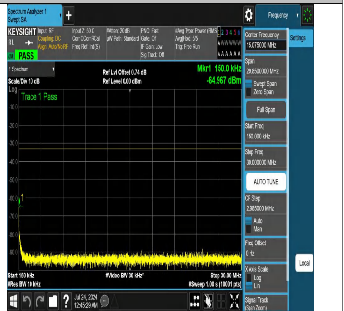
NTNV-N25-PC3-15-20-H-DFT-QPSK-Edge_1RB_Right-0.15-30-A nt1-PASS
