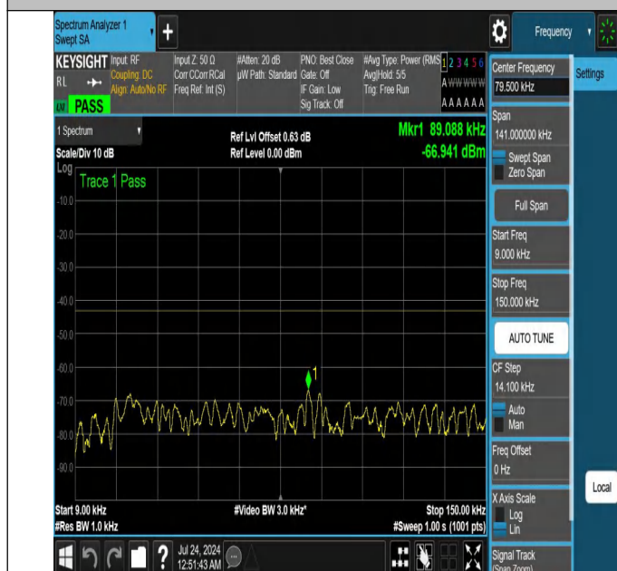
NTNV-N25-PC3-15-25-L-DFT-QPSK-Edge_1RB_Right-0.009-0.1 5-Ant1-PASS
