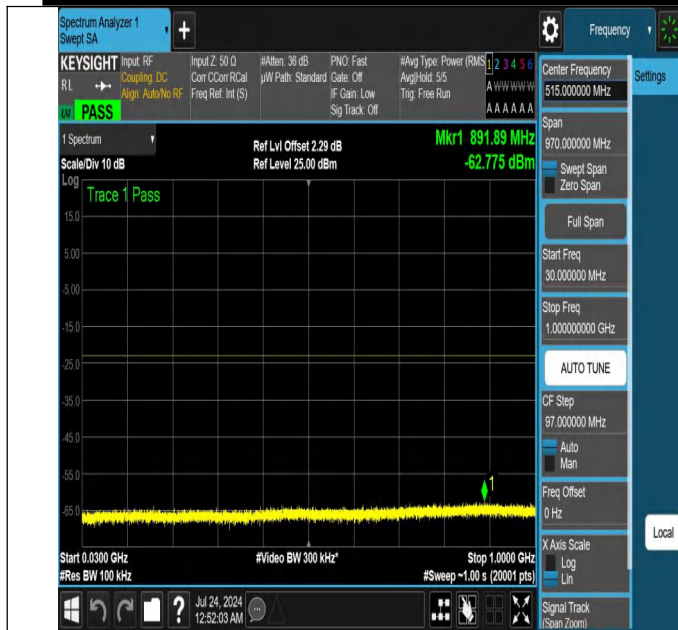
NTNV-N25-PC3-15-25-L-DFT-QPSK-Edge_1RB_Right-30-1000-Ant1-PASS
