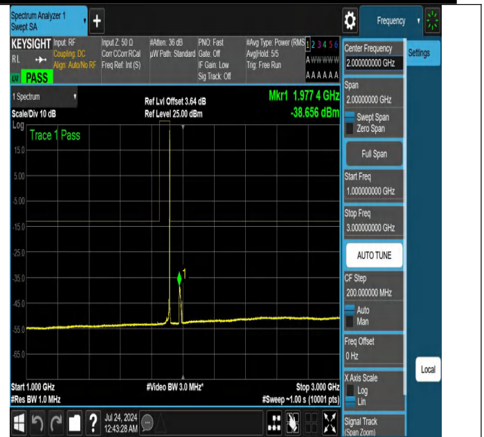
NTNV-N25-PC3-15-20-H-DFT-PI2BPSK-Edge_1RB_Right-1000-3000-Ant1-PASS
