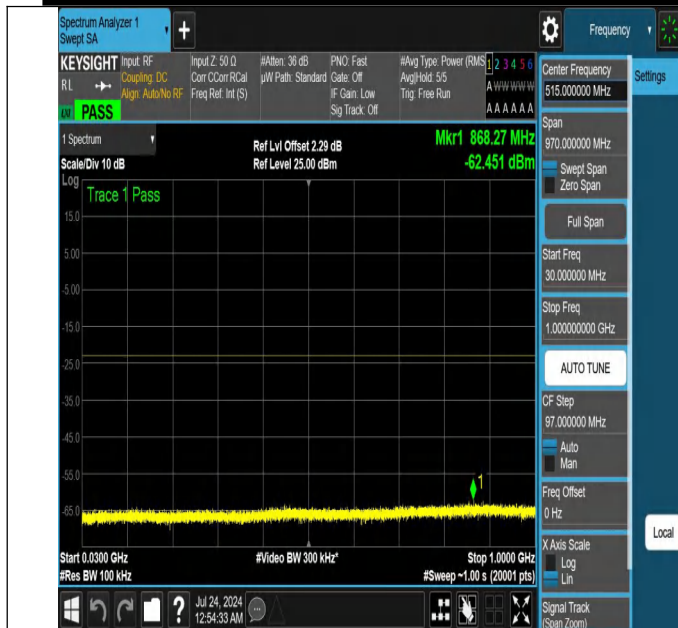
NTN-N25-PC3-15-25-M-DFT-PI2BPSK-Edge_1RB_Right-30-1000-Ant1-PASS
