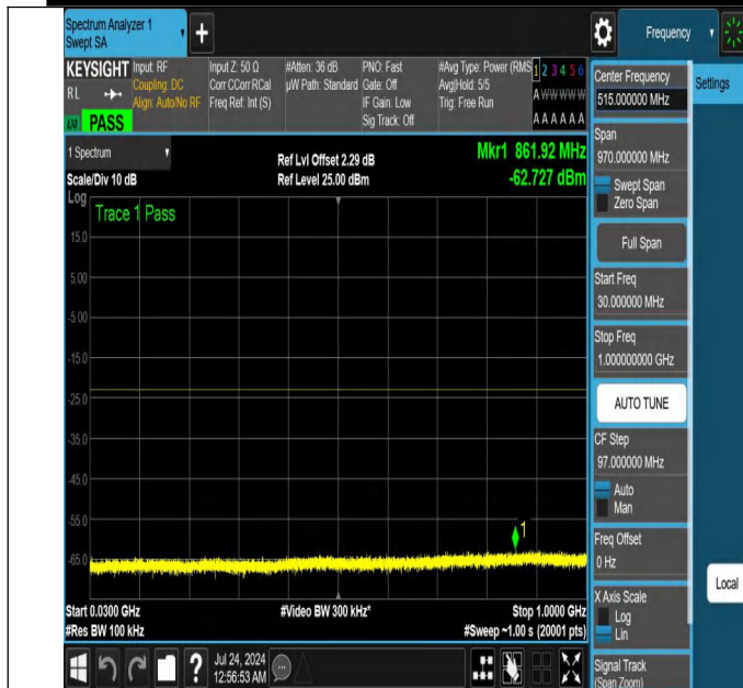
NTNV-N25-PC3-15-25-M-DFT-QPSK-Edge_1RB_Right-30-1000-Ant1-PASS
