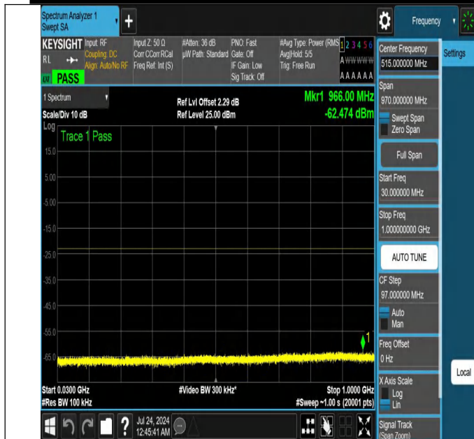
NTN-N25-PC3-15-20-H-DFT-QPSK-Edge_1RB_Right-30-1000-Ant1-PASS
