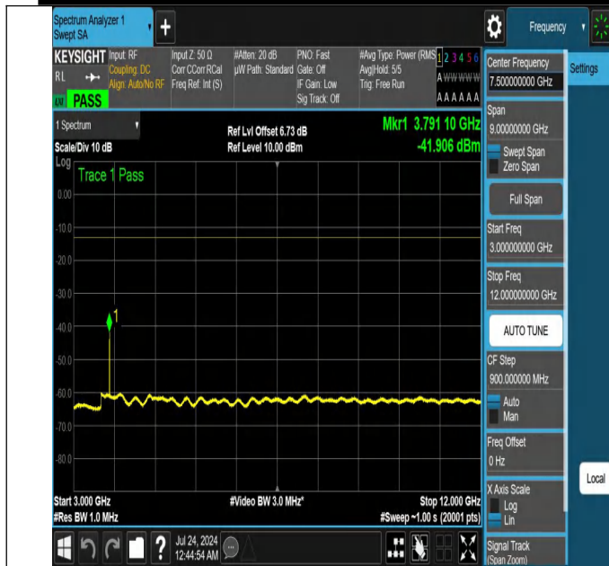
NTNV-N25-PC3-15-20-H-DFT-QPSK-Edge_1RB_Left-3000-1200 0-Ant1-PASS
