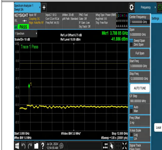
NTN-N25-PC3-15-25-M-DFT-PI2BPSK-Edge_1RB_Right-3000-12000-Ant1-PASS
