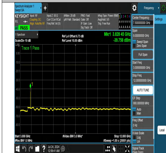
NTNV-N25-PC3-15-25-H-DFT-PI2BPSK-Edge_1RB_Right-3000-12000-Ant1-PASS
