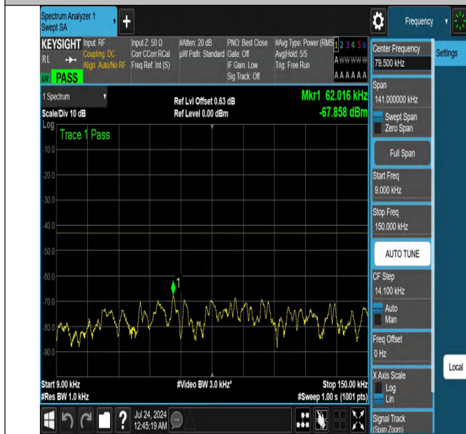
NTNV-N25-PC3-15-20-H-DFT-QPSK-Edge_1RB_Right-0.009-0.1 5-Ant1-PASS
