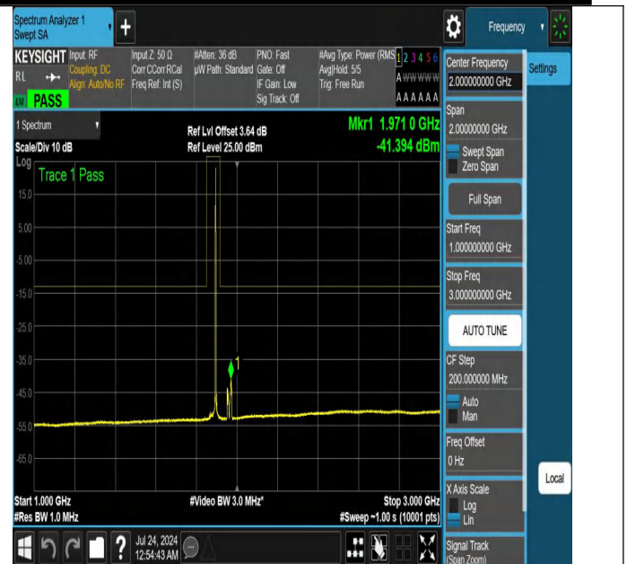
NTN-N25-PC3-15-25-M-DFT-PI2BPSK-Edge_1RB_Right-1000-3000-Ant1-PASS
