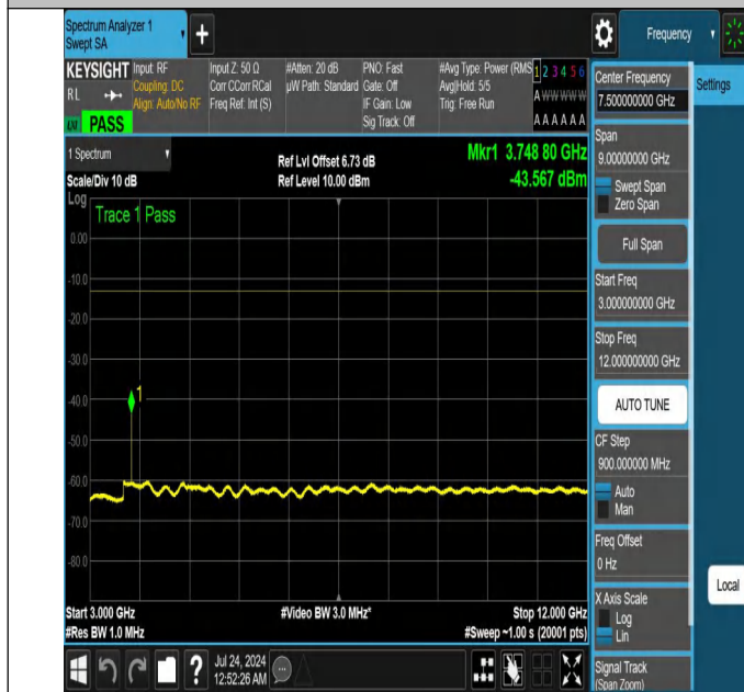
NTNV-N25-PC3-15-25-L-DFT-QPSK-Edge_1RB_Right-3000-12000-Ant1-PASS
