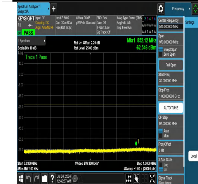
NTNV-N25-PC3-15-25-L-DFT-PI2BPSK-Edge_1RB_Right-30-1000-Ant1-PASS
