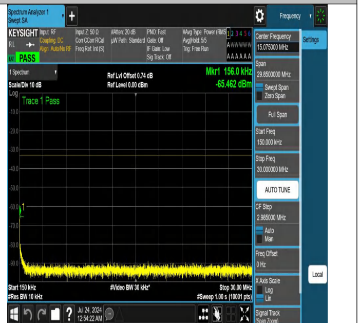
NTNV-N25-PC3-15-25-M-DFT-PI2BPSK-Edge_1RB_Right-0.15-3 0-Ant1-PASS
