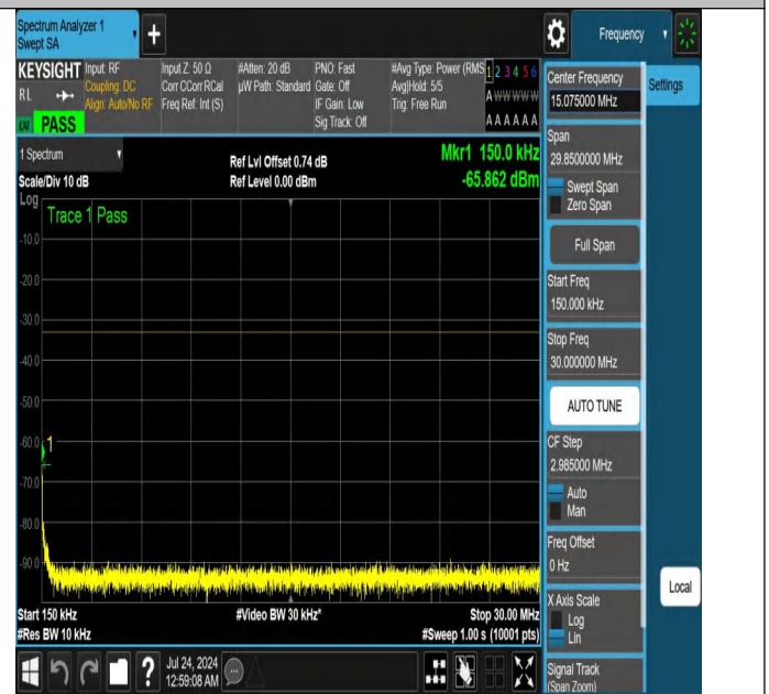
NTNV-N25-PC3-15-25-H-DFT-PI2BPSK-Edge_1RB_Right-0.15-3 0-Ant1-PASS
