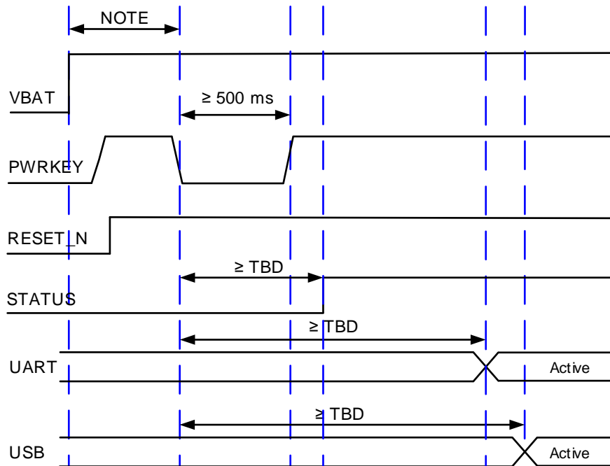
Figure 13: Turn-on Timing
