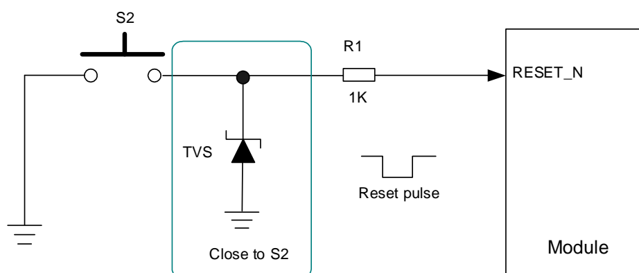
Figure 16: Reference Circuit of RESET_N with a Button
