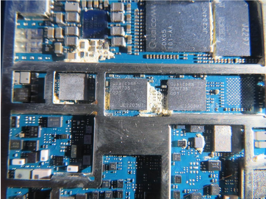
(7) EUT Photo
