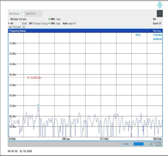
66-66-10MHz-15MHz-16QAM-16QAM-132025-132145-1RB#0-ORB#0-0.009~0.15MHz-PASS
