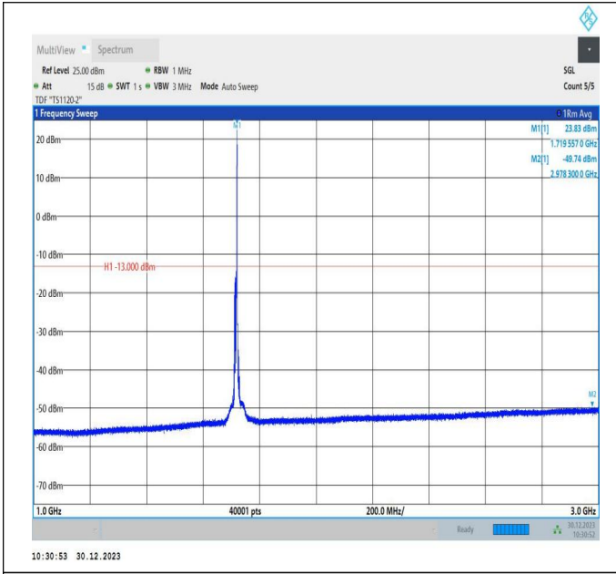
66-66-10MHz-15MHz-64QAM-64QAM-132025-132145-1RB# 49-ORB#0-1000~3000MHz-PASS
