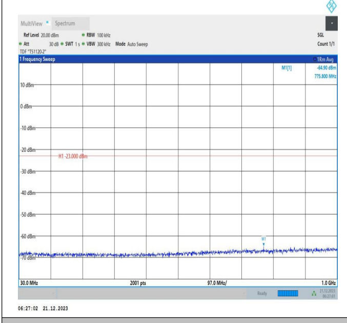
66-66-10MHz-15MHz-16QAM-16QAM-132025-132145-1RB# 49-ORB#0-30~1000MHz-PASS
