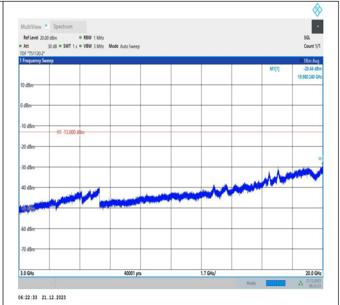
66-66-10MHz-15MHz-16QAM-16QAM-132025-132145-1RB# 0-ORB#0-3000~20000MHz-PASS
