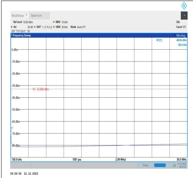
66-66-10MHz-15MHz-QPSK-QPSK-132025-132145-1RB#49 -ORB#0-0.15~30MHz-PASS
