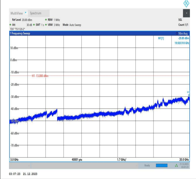
66-66-5MHz-20MHz-QPSK-QPSK-132428-132572-1RB#24-ORB#0-3000~20000MHz-PASS
