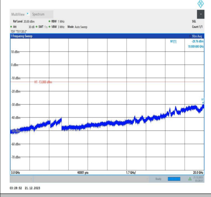
66-66-5MHz-20MHz-16QAM-16QAM-132428-132572-1RB#0 -1RB#99-3000~20000MHz-PASS
