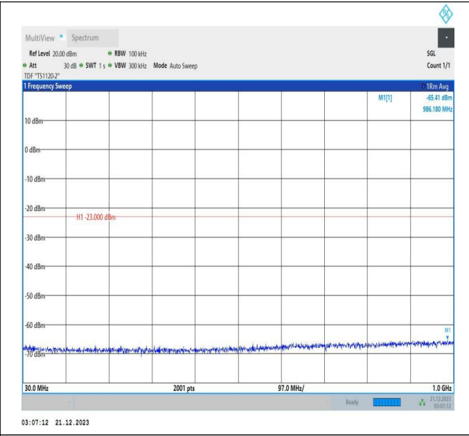
66-66-5MHz-20MHz-QPSK-QPSK-132428-132572-1RB#24-ORB#0-30~1000MHz-PASS
