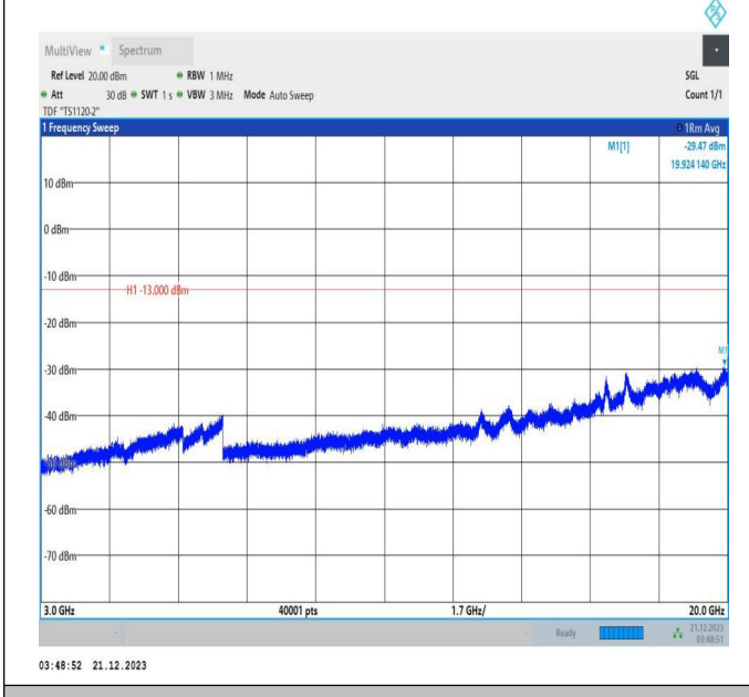
66-66-5MHz-20MHz-16QAM-16QAM-132428-132572-25RB# 0-100RB#0-3000~20000MHz-PASS
