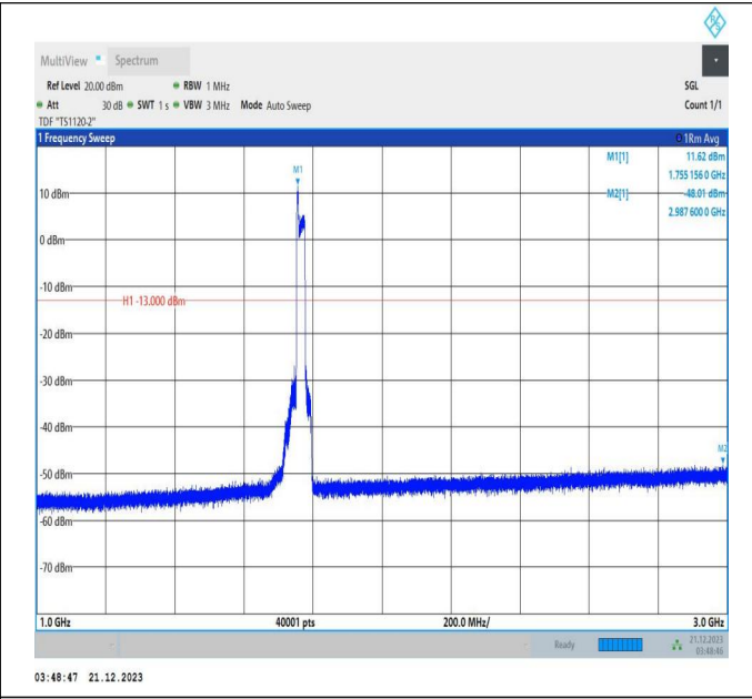
66-66-5MHz-20MHz-16QAM-16QAM-132428-132572-25RB# 0-100RB#0-1000~3000MHz-PASS
