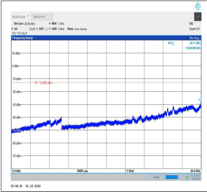
66-66-5MHz-20MHz-64QAM-64QAM-132428-132572-1RB#0-1RB#99-3000~20000MHz-PASS
