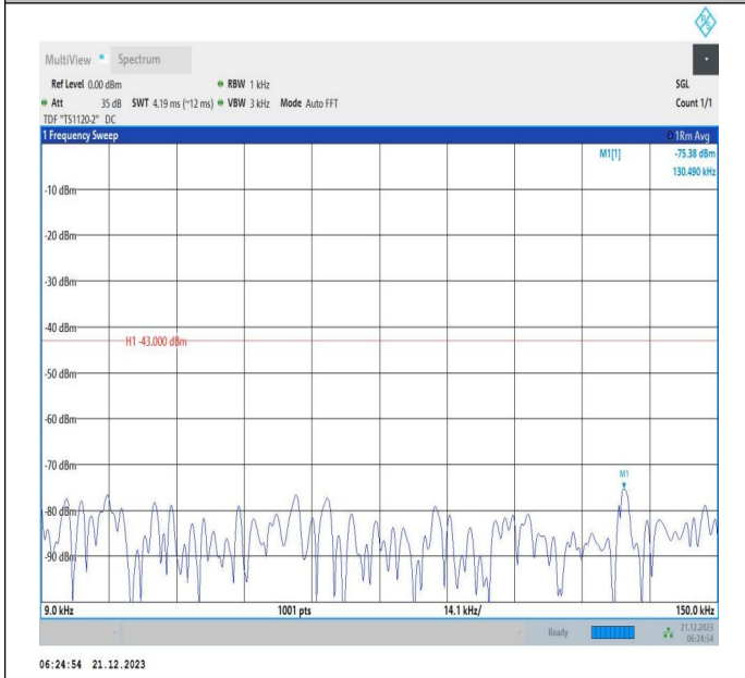
66-66-10MHz-15MHz-64QAM-64QAM-132025-132145-1RB# 0-ORB#0-0.009~0.15MHz-PASS
