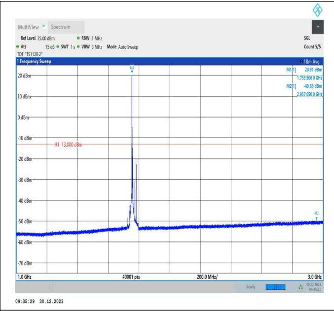
66-66-5MHz-20MHz-64QAM-64QAM-132428-132572-1RB#0 -ORB#0-1000~3000MHz-PASS
