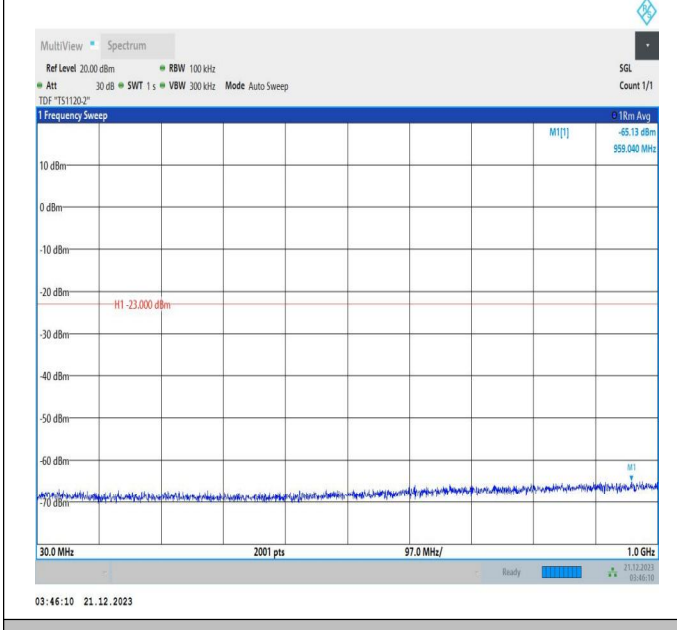
66-66-5MHz-20MHz-64QAM-64QAM-132428-132572-1RB#0 -1RB#99-30~1000MHz-PASS
