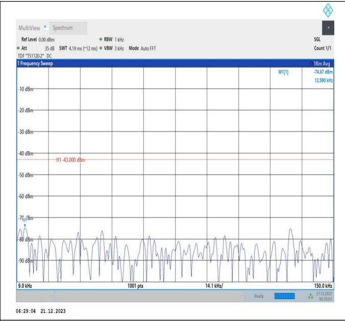
66-66-10MHz-15MHz-64QAM-64QAM-132025-132145-1RB# 49-ORB#0-0.009~0.15MHz-PASS
