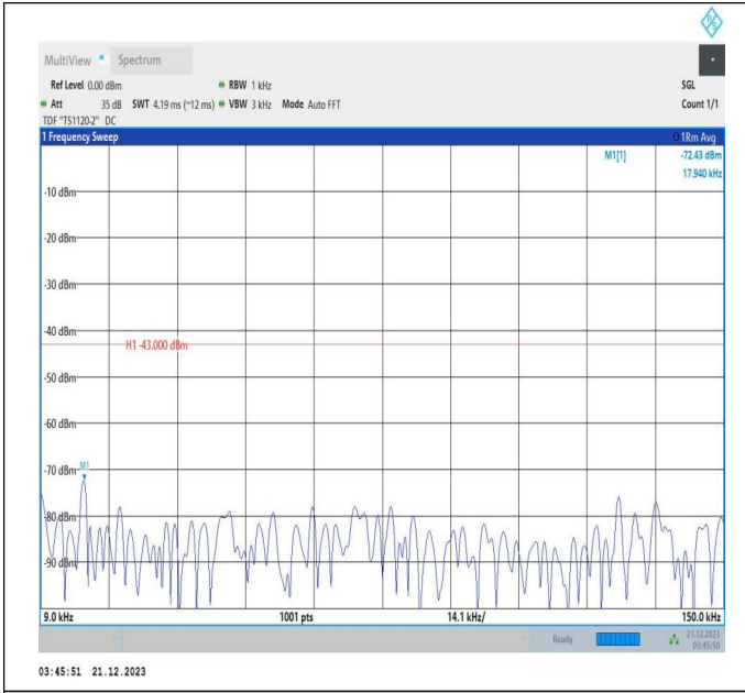
66-66-5MHz-20MHz-64QAM-64QAM-132428-132572-1RB#0 -1RB#99-0.009~0.15MHz-PASS
