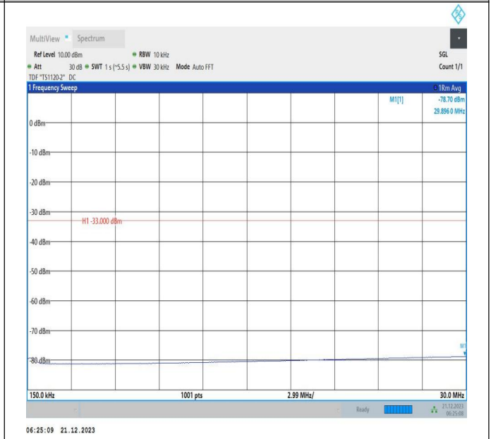
66-66-10MHz-15MHz-64QAM-64QAM-132025-132145-1RB# 0-ORB#0-0.15~30MHz-PASS
