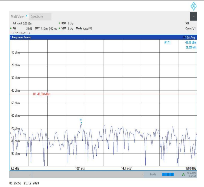
66-66-10MHz-15MHz-QPSK-QPSK-132025-132145-1RB#49 -ORB#0-0.009~0.15MHz-PASS
