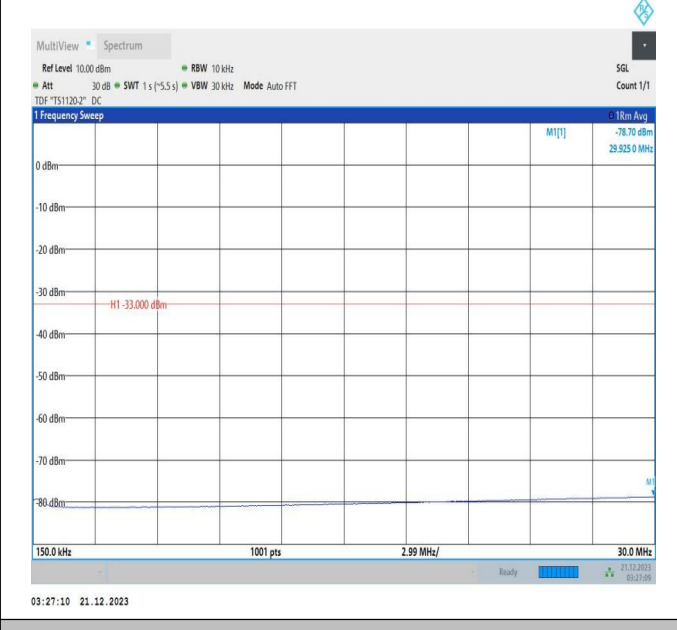
66-66-5MHz-20MHz-QPSK-QPSK-132428-132572-1RB#0-1 RB#99-0.15~30MHz-PASS
