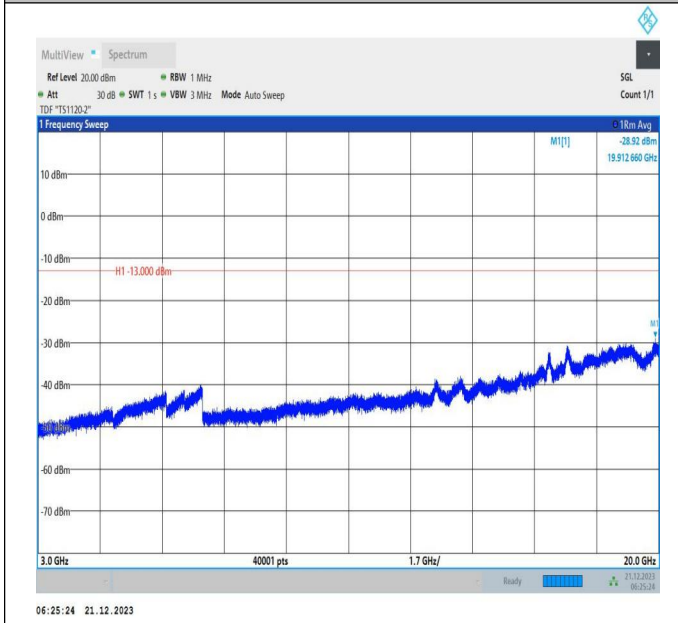
66-66-10MHz-15MHz-64QAM-64QAM-132025-132145-1RB# 0-ORB#0-3000~20000MHz-PASS
