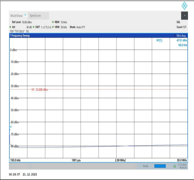
66-66-10MHz-15MHz-16QAM-16QAM-132025-132145-1RB# 49-ORB#0-0.15~30MHz-PASS
