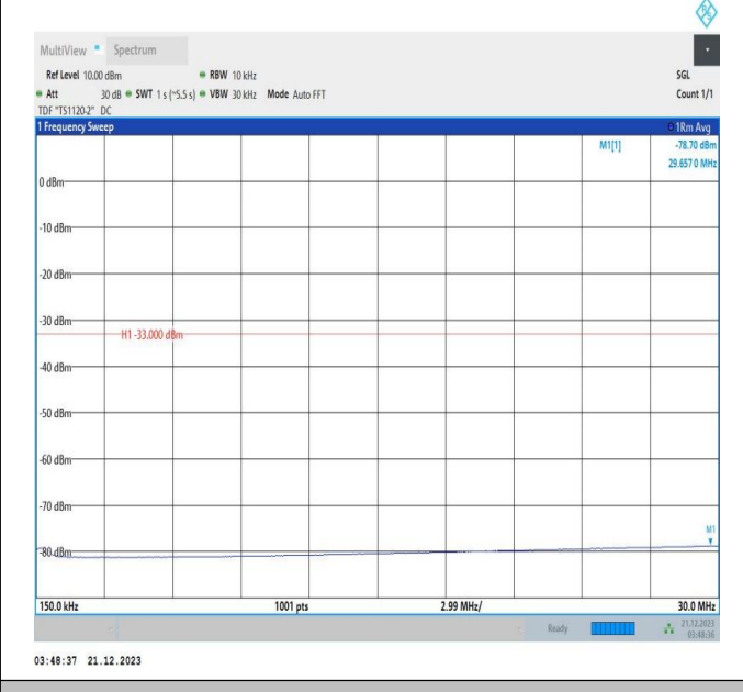
66-66-5MHz-20MHz-16QAM-16QAM-132428-132572-25RB#0-100RB#0-0.15~30MHz-PASS
