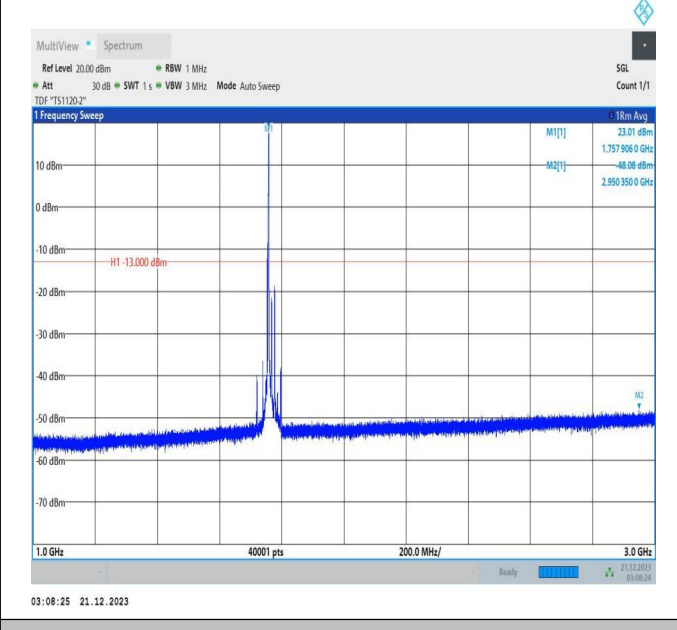
66-66-5MHz-20MHz-16QAM-16QAM-132428-132572-1RB#2 4-ORB#0-1000~3000MHz-PASS
