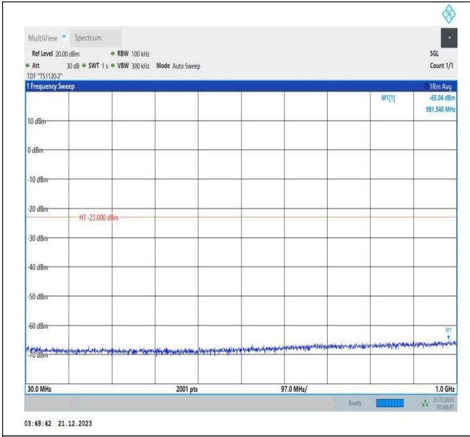
66-66-5MHz-20MHz-16QAM-16QAM-132428-132572-25RB# 0-100RB#0-30~1000MHz-PASS
