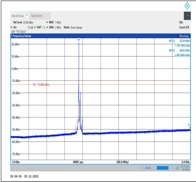
66-66-5MHz-20MHz-64QAM-64QAM-132428-132572-1RB#2 4-ORB#0-1000~3000MHz-PASS
