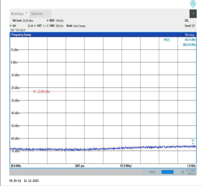
66-66-10MHz-15MHz-64QAM-64QAM-132025-132145-1RB# 49-ORB#0-30~1000MHz-PASS
