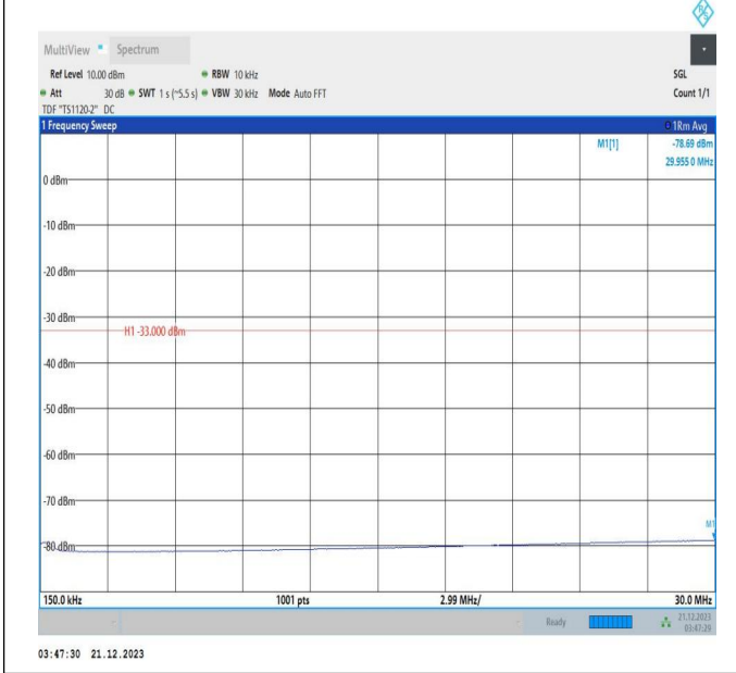
66-66-5MHz-20MHz-QPSK-QPSK-132428-132572-25RB#0-100RB#0-0.15~30MHz-PASS
