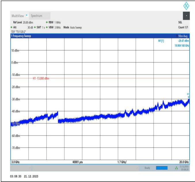
66-66-5MHz-20MHz-16QAM-16QAM-132428-132572-1RB#2 4-ORB#0-3000~20000MHz-PASS
