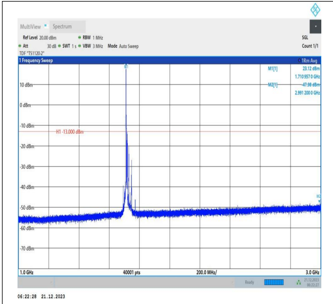
66-66-10MHz-15MHz-16QAM-16QAM-132025-132145-1RB# 0-ORB#0-1000~3000MHz-PASS
