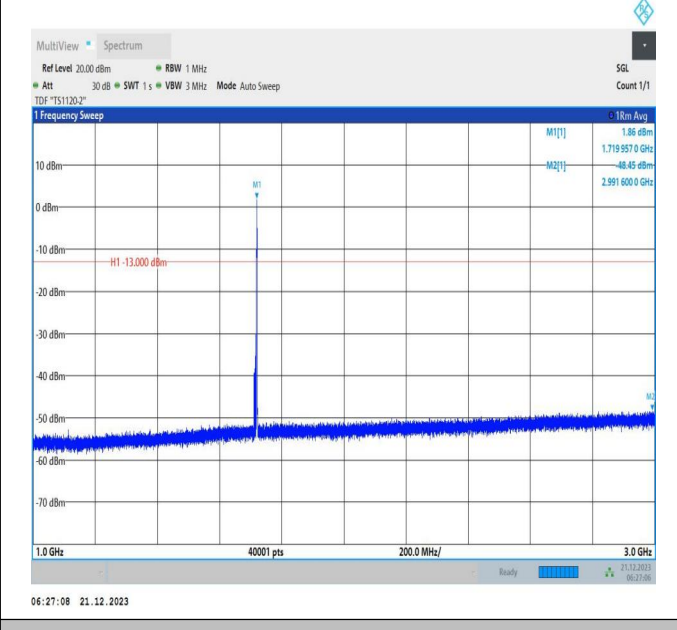
66-66-10MHz-15MHz-16QAM-16QAM-132025-132145-1RB# 49-ORB#0-1000~3000MHz-PASS
