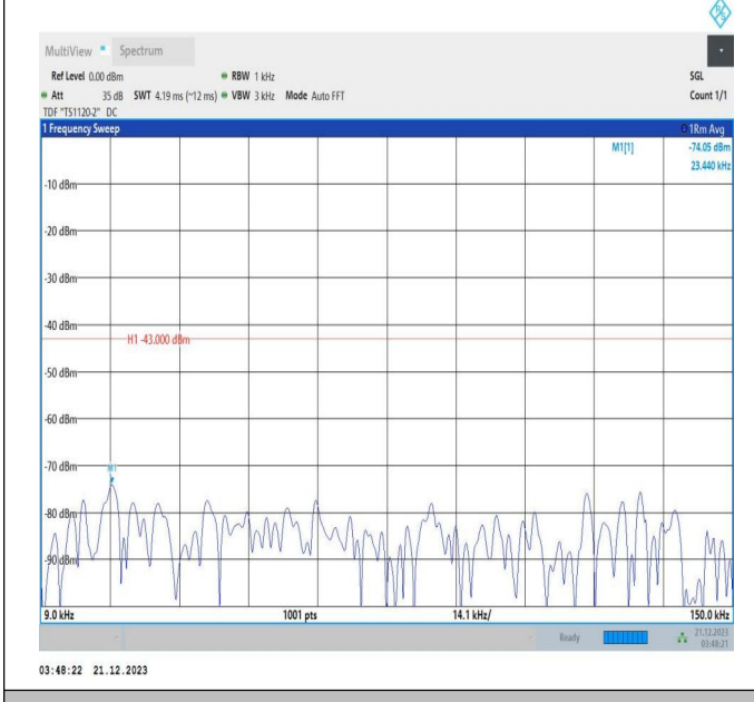
66-66-5MHz-20MHz-16QAM-16QAM-132428-132572-25RB#0-100RB#0-0.009~0.15MHz-PASS
