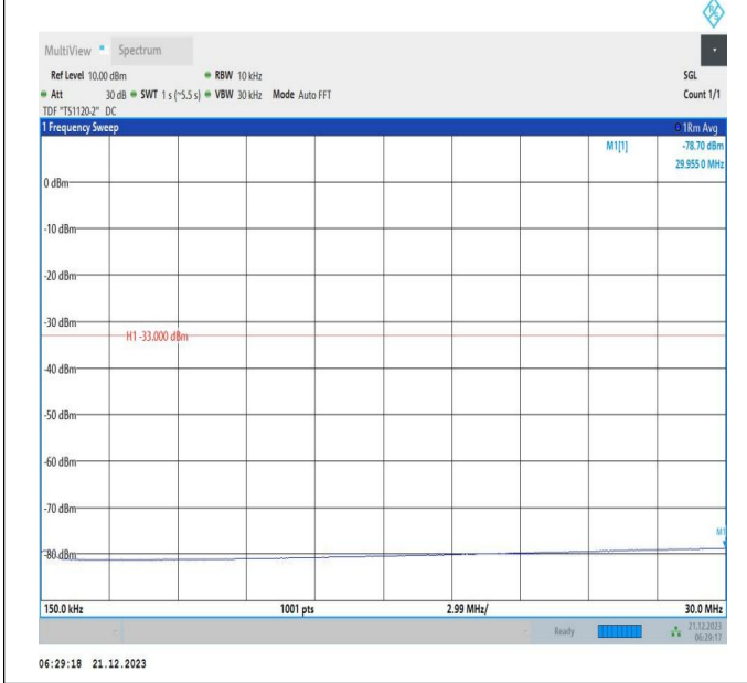
66-66-10MHz-15MHz-64QAM-64QAM-132025-132145-1RB# 49-ORB#0-0.15~30MHz-PASS
