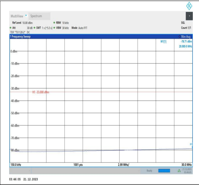
66-66-5MHz-20MHz-64QAM-64QAM-132428-132572-1RB#0 -1RB#99-0.15~30MHz-PASS
