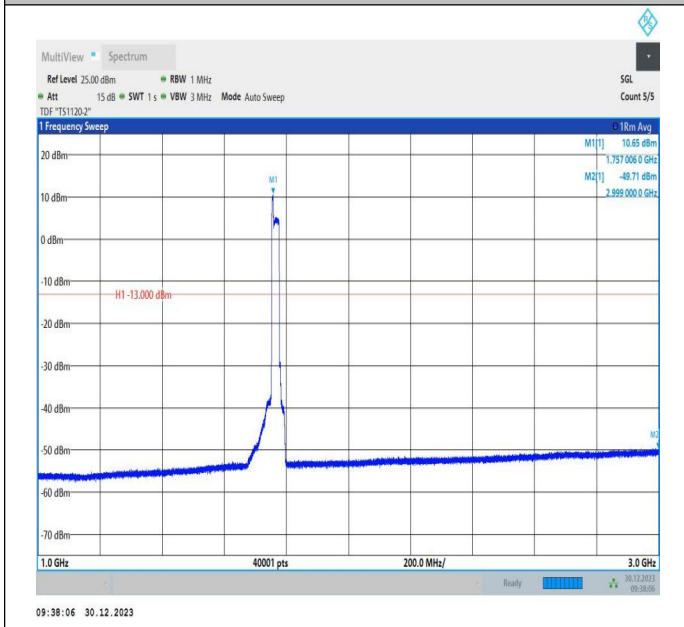
66-66-5MHz-20MHz-64QAM-64QAM-132428-132572-25RB# 0-100RB#0-1000~3000MHz-PASS
