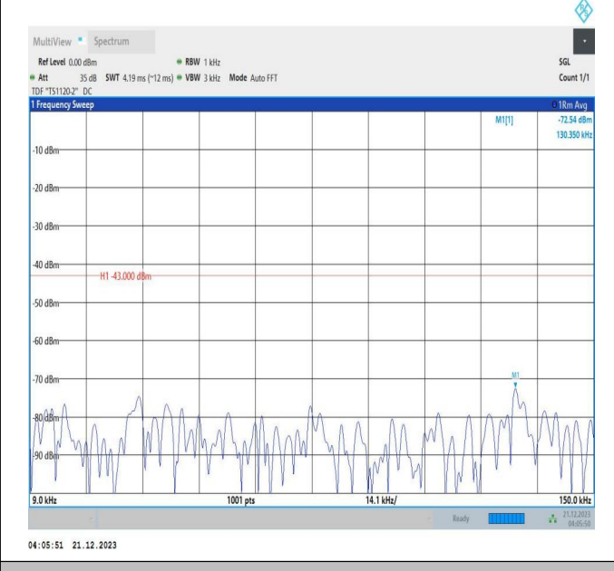
66-66-5MHz-20MHz-64QAM-64QAM-132428-132572-25RB# 0-100RB#0-0.009~0.15MHz-PASS
