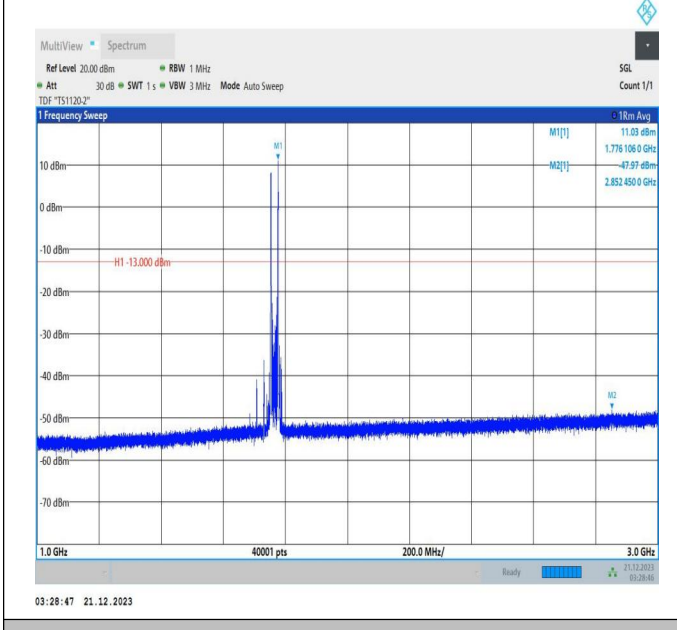
66-66-5MHz-20MHz-16QAM-16QAM-132428-132572-1RB#0 -1RB#99-1000~3000MHz-PASS
