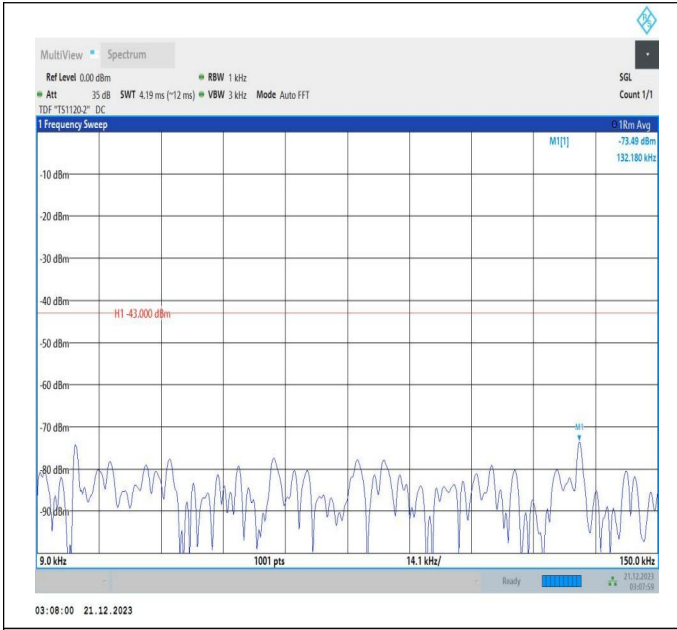
66-66-5MHz-20MHz-16QAM-16QAM-132428-132572-1RB#2 4-ORB#0-0.009~0.15MHz-PASS
