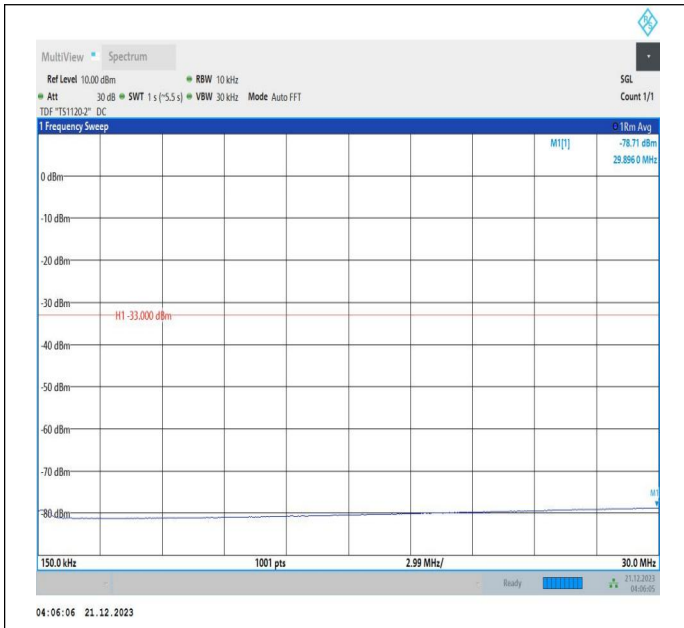
66-66-5MHz-20MHz-64QAM-64QAM-132428-132572-25RB# 0-100RB#0-0.15~30MHz-PASS
