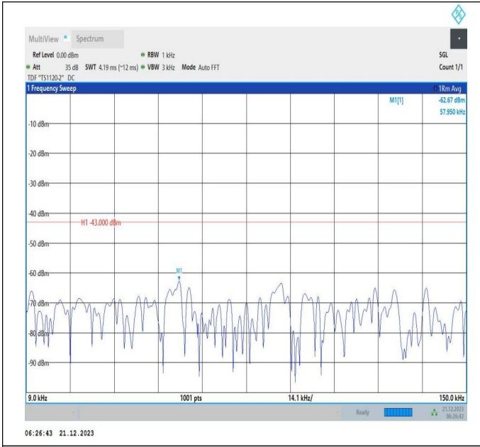
66-66-10MHz-15MHz-16QAM-16QAM-132025-132145-1RB# 49-ORB#0-0.009~0.15MHz-PASS
