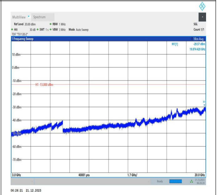
66-66-10MHz-15MHz-QPSK-QPSK-132025-132145-1RB#49 -ORB#0-3000~20000MHz-PASS
