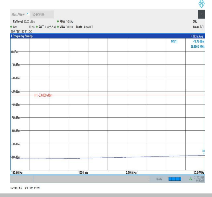
66-66-10MHz-15MHz-QPSK-QPSK-132025-132145-1RB#0- 1RB#74-0.15~30MHz-PASS
