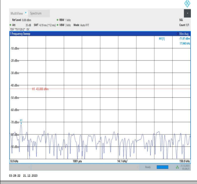
66-66-5MHz-20MHz-16QAM-16QAM-132428-132572-1RB#0-1 -1RB#99-0.009~0.15MHz-PASS
