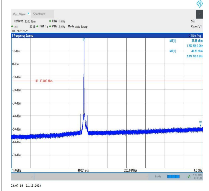
66-66-5MHz-20MHz-QPSK-QPSK-132428-132572-1RB#24-ORB#0-1000~3000MHz-PASS
