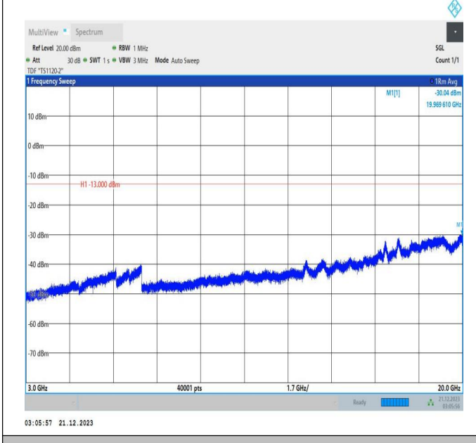
66-66-5MHz-20MHz-64QAM-64QAM-132428-132572-1RB#0 -ORB#0-3000~20000MHz-PASS
