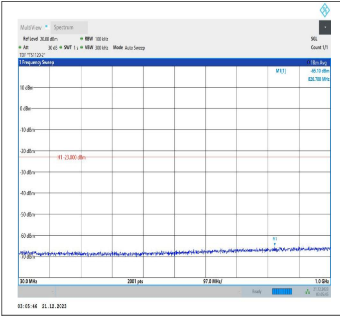
66-66-5MHz-20MHz-64QAM-64QAM-132428-132572-1RB#0 -ORB#0-30~1000MHz-PASS
