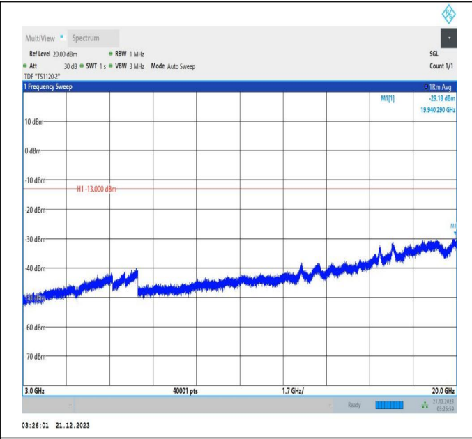
66-66-5MHz-20MHz-64QAM-64QAM-132428-132572-1RB#2 4-ORB#0-3000~20000MHz-PASS
