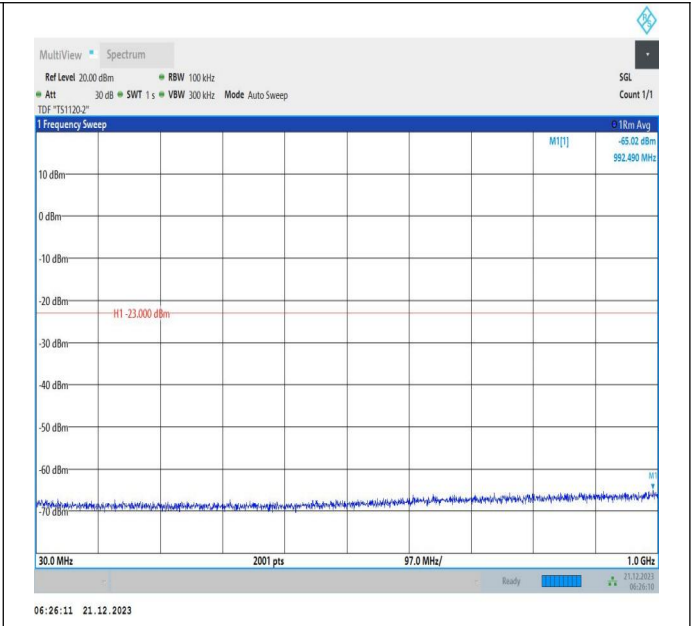
66-66-10MHz-15MHz-QPSK-QPSK-132025-132145-1RB#49 -ORB#0-30~1000MHz-PASS
