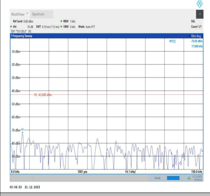
66-66-5MHz-20MHz-QPSK-QPSK-132428-132572-1RB#24- ORB#0-0.009~0.15MHz-PASS
