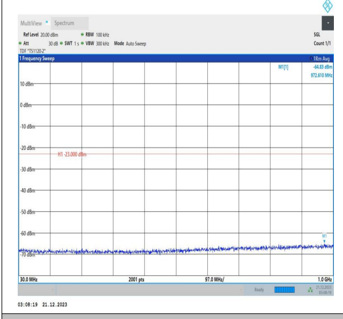
66-66-5MHz-20MHz-16QAM-16QAM-132428-132572-1RB#2 4-ORB#0-30~1000MHz-PASS
