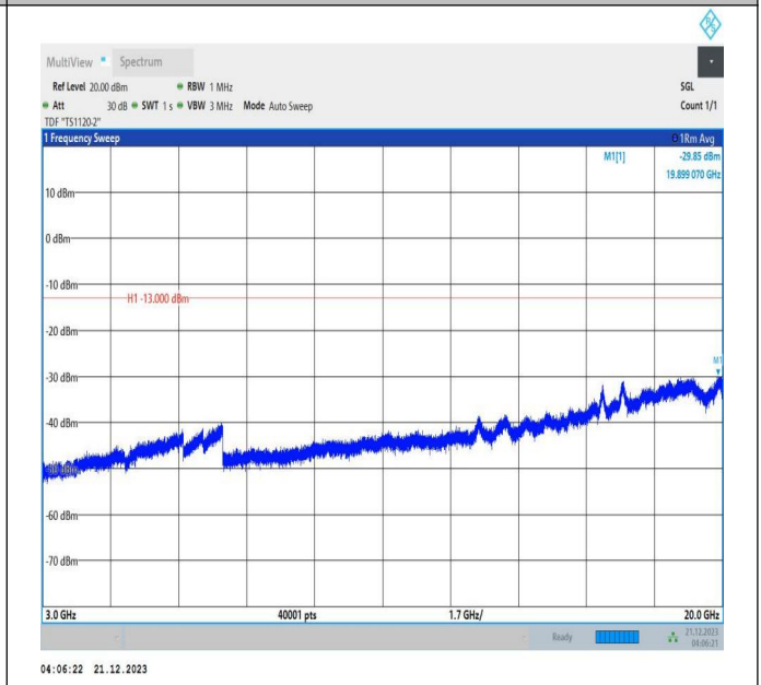
66-66-5MHz-20MHz-64QAM-64QAM-132428-132572-25RB# 0-100RB#0-3000~20000MHz-PASS
