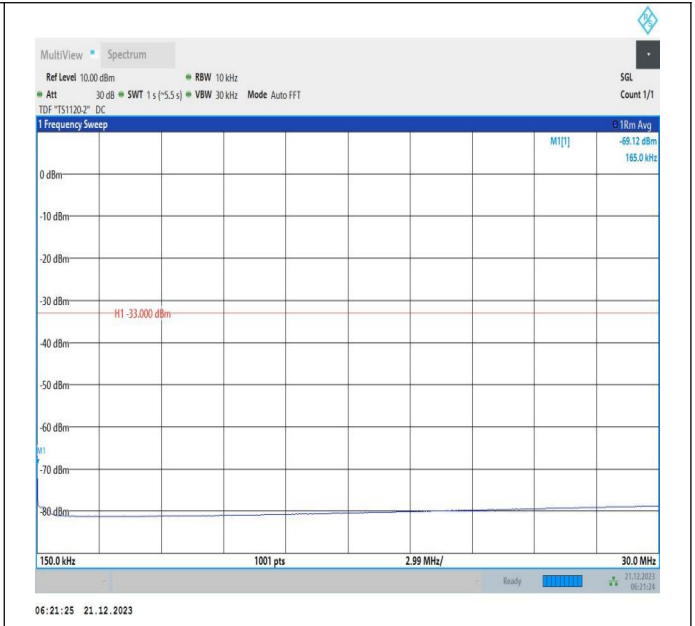
66-66-10MHz-15MHz-QPSK-QPSK-132025-132145-1RB#0-ORB#0-0.15~30MHz-PASS
