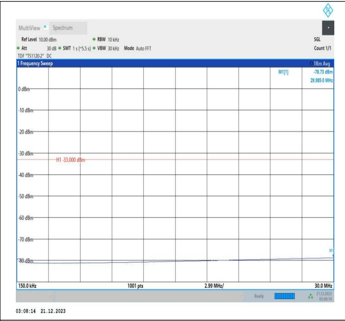
66-66-5MHz-20MHz-16QAM-16QAM-132428-132572-1RB#2 4-ORB#0-0.15~30MHz-PASS
