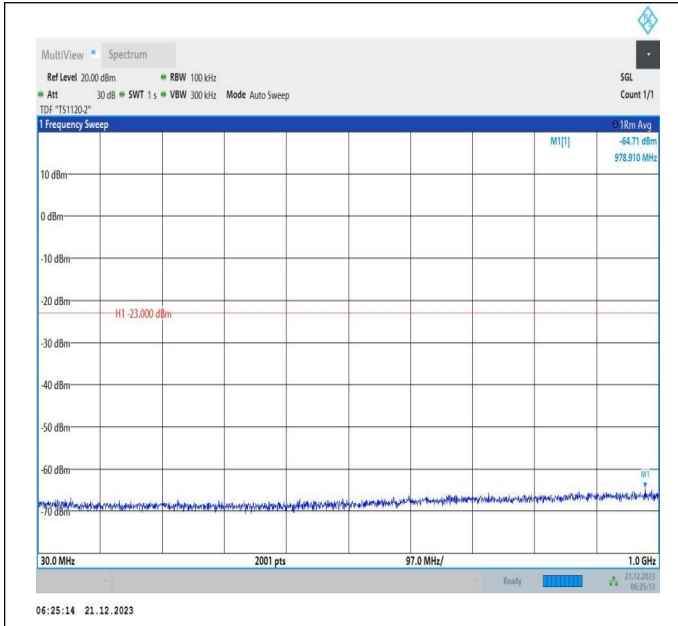
66-66-10MHz-15MHz-64QAM-64QAM-132025-132145-1RB# 0-ORB#0-30~1000MHz-PASS
