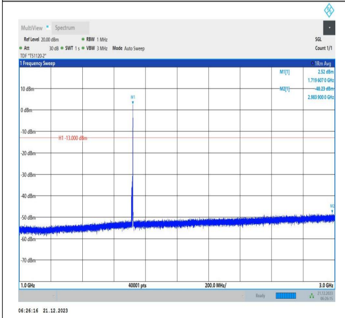
66-66-10MHz-15MHz-QPSK-QPSK-132025-132145-1RB#49 -ORB#0-1000~3000MHz-PASS
