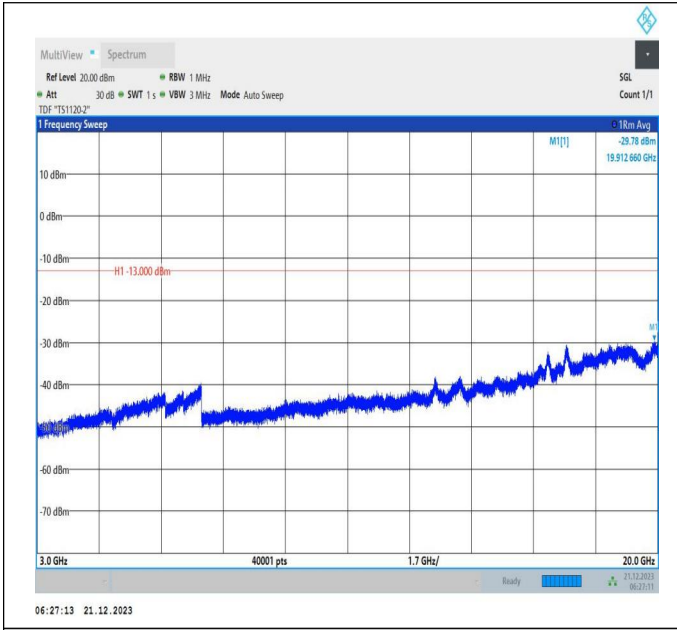
66-66-10MHz-15MHz-16QAM-16QAM-132025-132145-1RB# 49-ORB#0-3000~20000MHz-PASS
