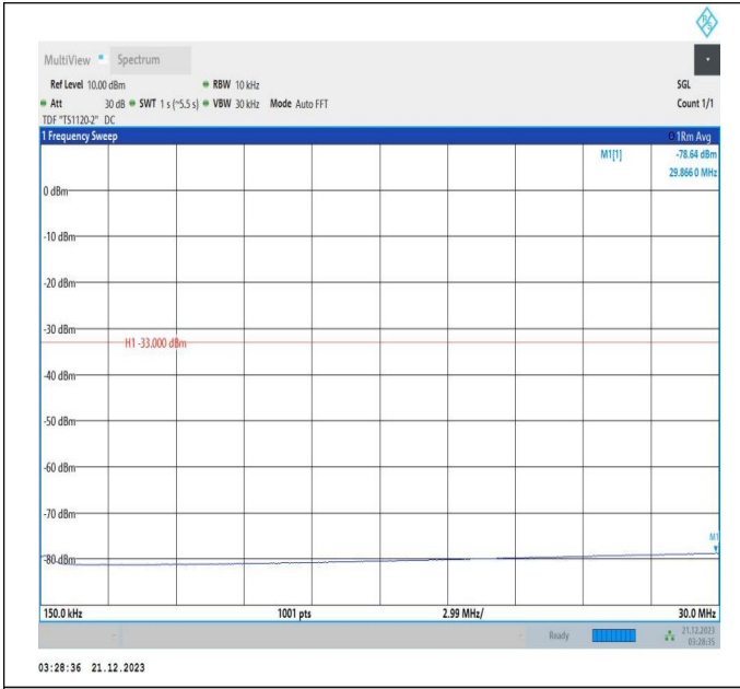
66-66-5MHz-20MHz-16QAM-16QAM-132428-132572-1RB#0 -1RB#99-0.15~30MHz-PASS
