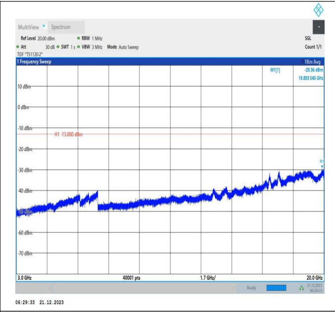
66-66-10MHz-15MHz-64QAM-64QAM-132025-132145-1RB# 49-ORB#0-3000~20000MHz-PASS
