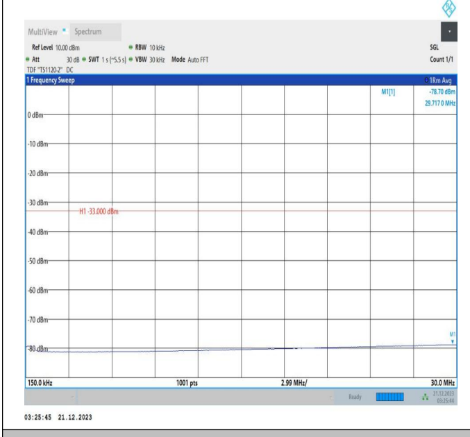
66-66-5MHz-20MHz-64QAM-64QAM-132428-132572-1RB#2 4-ORB#0-0.15~30MHz-PASS
