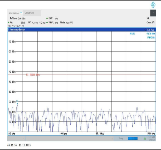
66-66-5MHz-20MHz-64QAM-64QAM-132428-132572-1RB#2 4-ORB#0-0.009~0.15MHz-PASS
