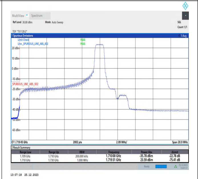
10MHz-10MHz_16QAM@16QAM-16QAM@16QAM_132022-132121_1RB#49@50RB#0-0RB#0@50RB#0
