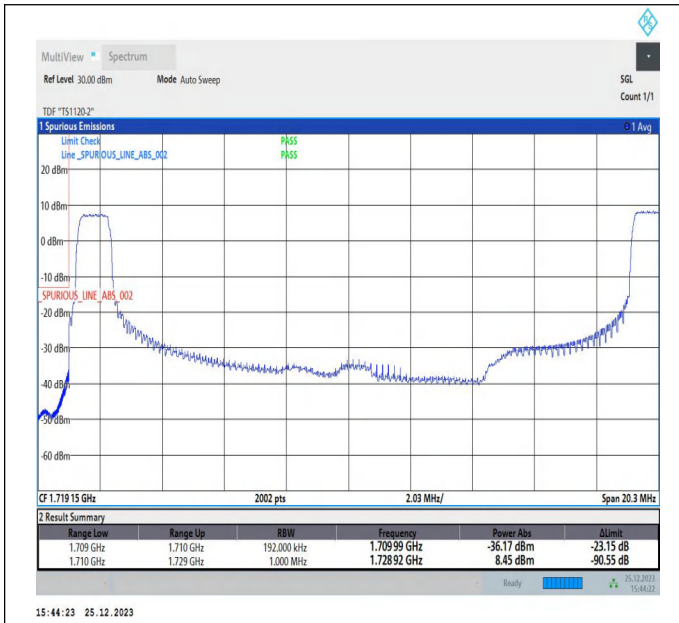
15MHz-5MHz_16QAM@16QAM-16QAM@16QAM_132047-132140_1RB#0@75RB#0-1RB#24@25RB#0
