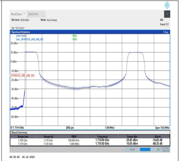
5MHz-5MHz_16QAM@16QAM-16QAM@16QAM_131997-132045_1RB#0@25RB#0-1RB#15@25RB#0
