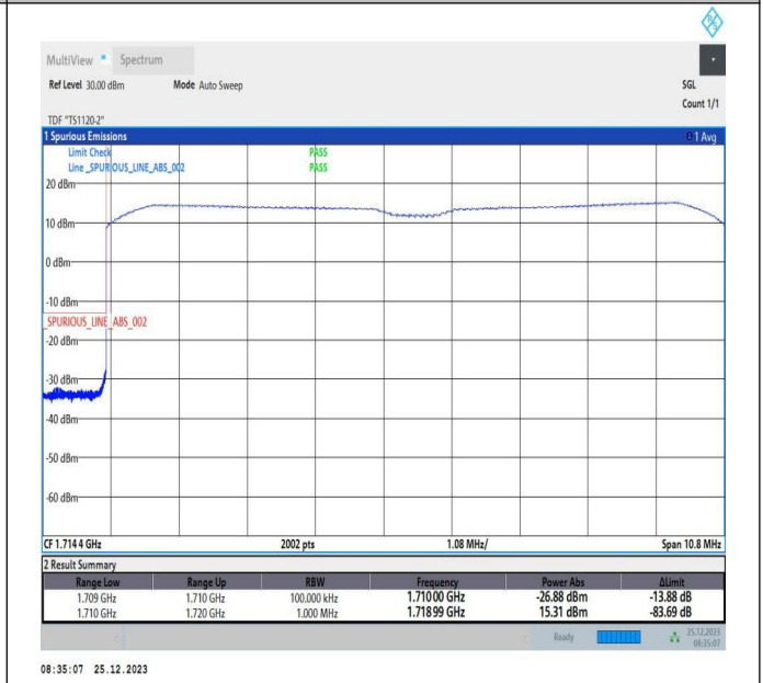
5MHz-5MHz_16QAM@16QAM-16QAM@16QAM_131997-132045_25RB#0@25RB#0-25RB#0@25RB#0
