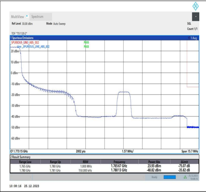
5MHz-10MHz_16QAM@16QAM-16QAM@16QAM_132550-1 32622_1RB#0@25RB#0-0RB#0@50RB#0
