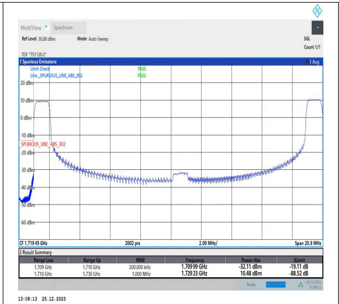
10MHz-10MHz_16QAM@16QAM-16QAM@16QAM_132022-132121_1RB#0@50RB#0-1RB#49@50RB#0
