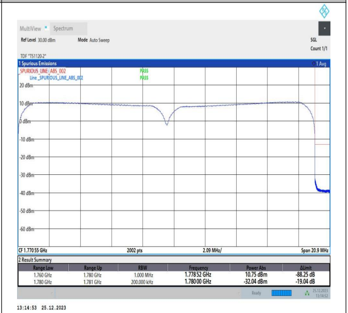
10MHz-10MHz_16QAM@16QAM-16QAM@16QAM_132523-132622_50RB#0@50RB#0-50RB#0@50RB#0
