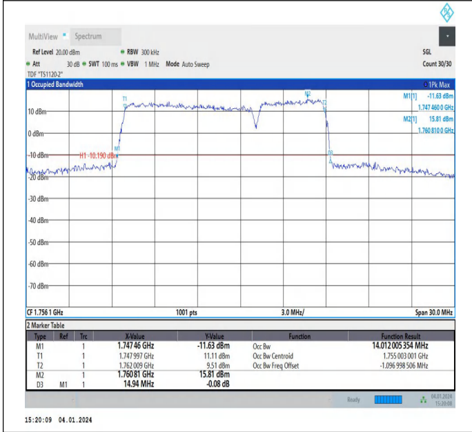
66-66-10MHz-5MHz-64QAM-64QAM-132397-132469-50RB# 0-25RB#0-PASS
