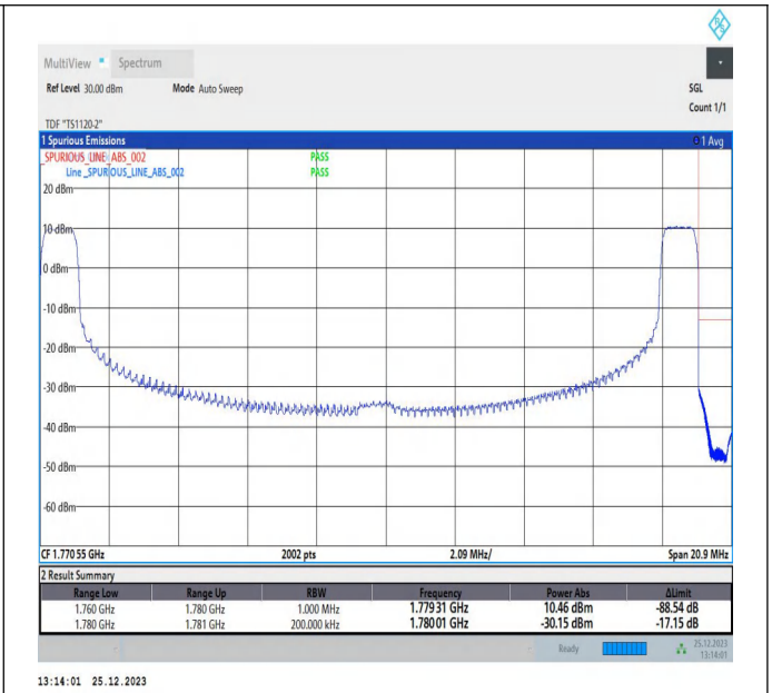
10MHz-10MHz_16QAM@16QAM-16QAM@16QAM_132523-132622_1RB#0@50RB#0-1RB#49@50RB#0
