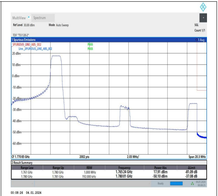
5MHz-15MHz_QPSK@QPSK-QPSK@QPSK_132504-132597_1RB#24@25RB#0-0RB#0@75RB#0
