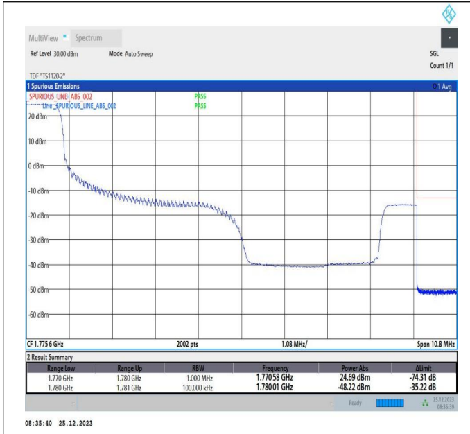
5MHz-5MHz_QPSK@QPSK-QPSK@QPSK_132599-132647_1RB#0@25RB#0-0RB#0@25RB#0
