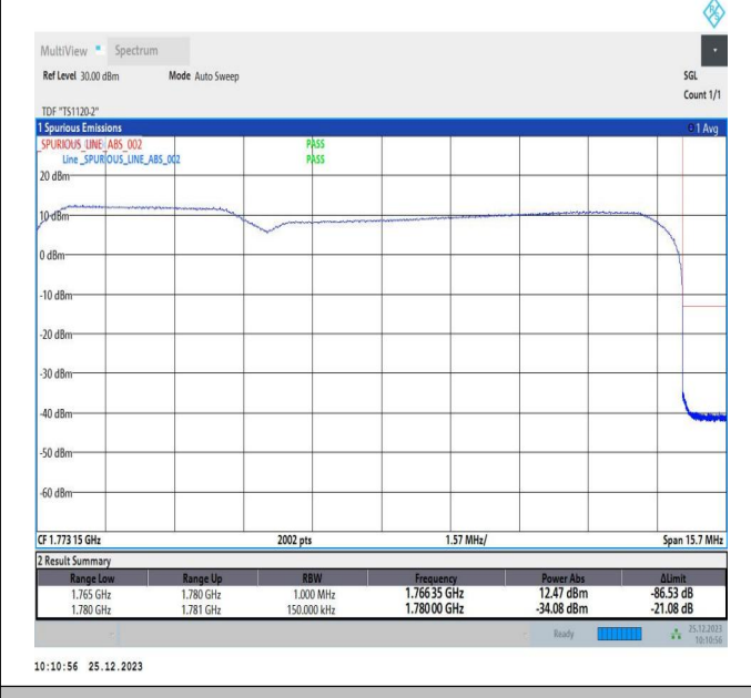
5MHz-10MHz_16QAM@16QAM-16QAM@16QAM_132550-132622_25RB#0@25RB#0-50RB#0@50RB#0
