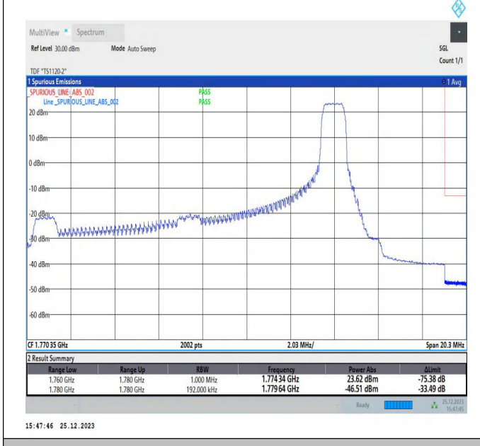
15MHz-5MHz_16QAM@16QAM-16QAM@16QAM_132549-132642_1RB#74@75RB#0-0RB#0@25RB#0
