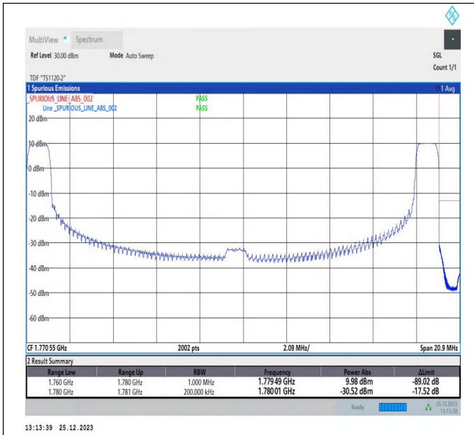
10MHz-10MHz_QPSK@QPSK-QPSK@QPSK_132523-132622_1RB#0@50RB#0-1RB#49@50RB#0
