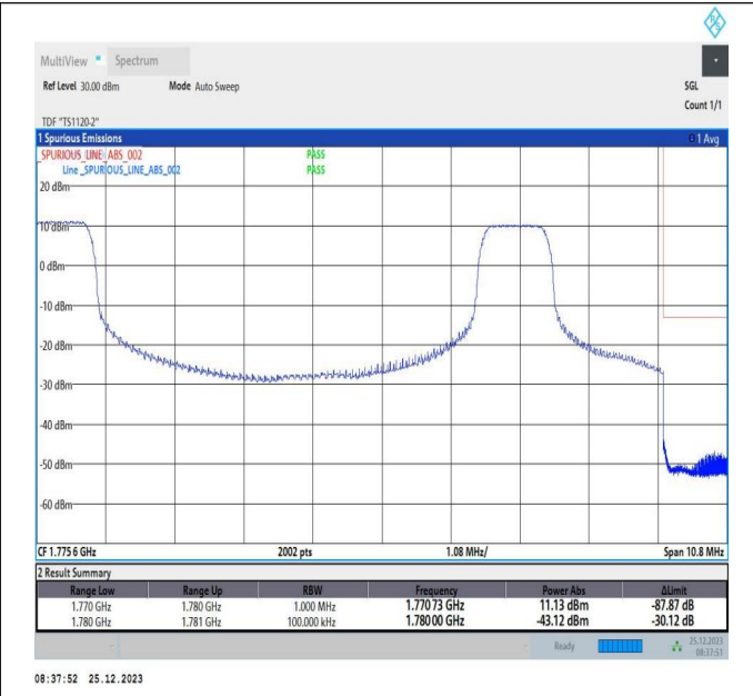
5MHz-5MHz_16QAM@16QAM-16QAM@16QAM_132599-132647_1RB#0@25RB#0-1RB#15@25RB#0
