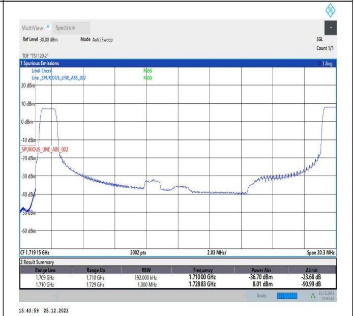
15MHz-5MHz_QPSK@QPSK-QPSK@QPSK_132047-132140_1RB#0@75RB#0-1RB#24@25RB#0
