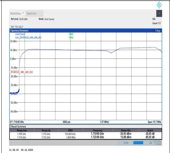
10MHz-5MHz_16QAM@16QAM-16QAM@16QAM_132022-1 32094_50RB#0@50RB#0-25RB#0@25RB#0
