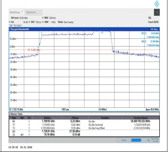
66-66-15MHz-5MHz-64QAM-64QAM-132047-132140-75RB# 0-25RB#0-PASS
