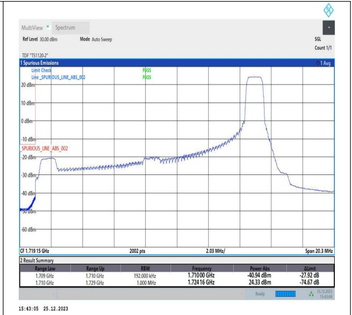
15MHz-5MHz_QPSK@QPSK-QPSK@QPSK_132047-132140_1RB#74@75RB#0-0RB#0@25RB#0
