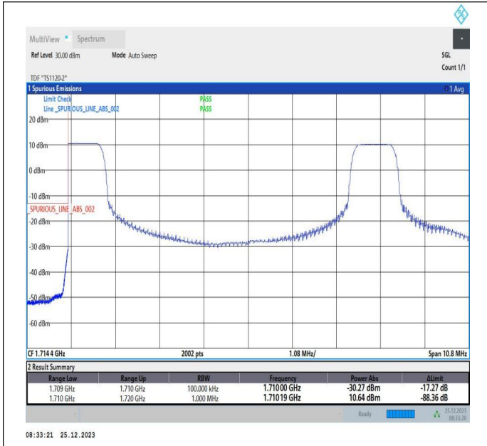
5MHz-5MHz_QPSK@QPSK-QPSK@QPSK_131997-132045_1RB#0@25RB#0-1RB#15@25RB#0
