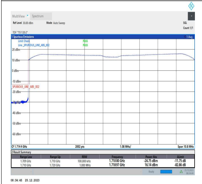
5MHz-5MHz_QPSK@QPSK-QPSK@QPSK_131997-132045_25RB#0@25RB#0-25RB#0@25RB#0
