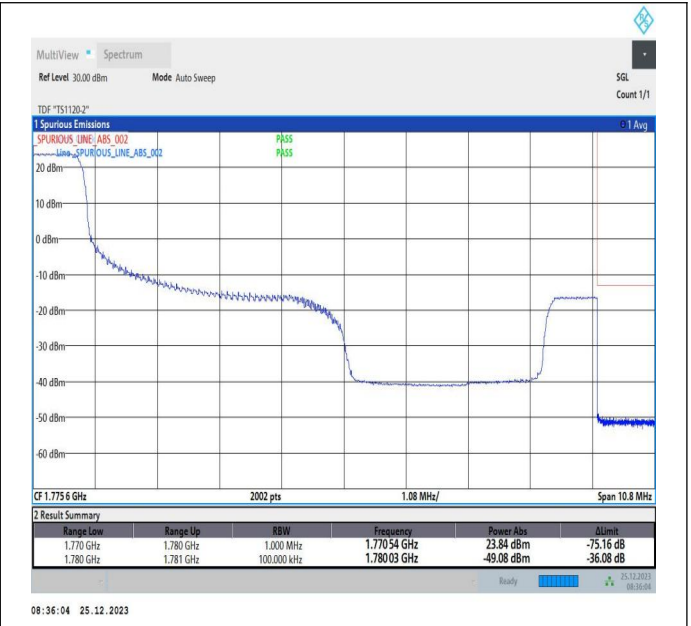
5MHz-5MHz_16QAM@16QAM-16QAM@16QAM_132599-132647_1RB#0@25RB#0-0RB#0@25RB#0
