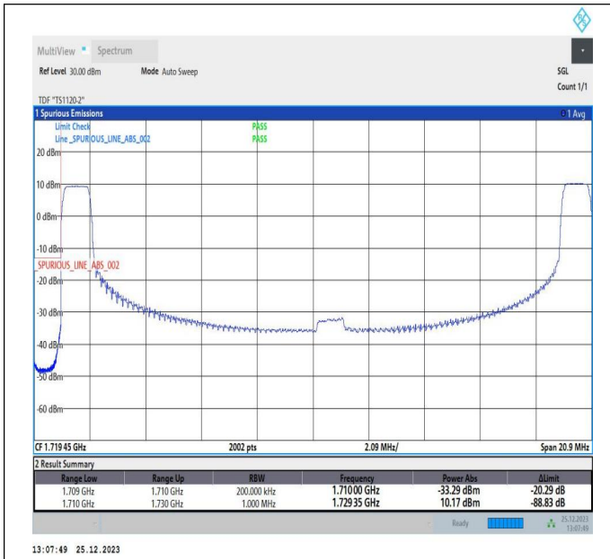
10MHz-10MHz_QPSK@QPSK-QPSK@QPSK_132022-132121_1RB#0@50RB#0-1RB#49@50RB#0
