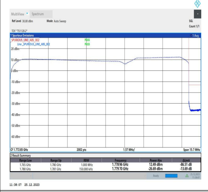
10MHz-5MHz_16QAM@16QAM-16QAM@16QAM_132572-1 32644_50RB#0@50RB#0-25RB#0@25RB#0
