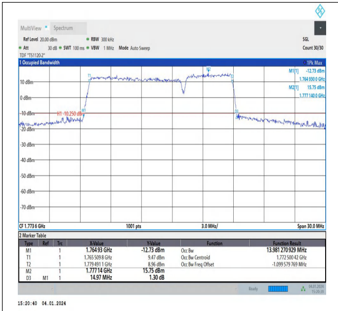
66-66-10MHz-5MHz-64QAM-64QAM-132572-132644-50RB#0-25RB#0-PASS
