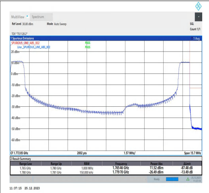
10MHz-5MHz_16QAM@16QAM-16QAM@16QAM_132572-1 32644_1RB#0@50RB#0-1RB#24@25RB#0
