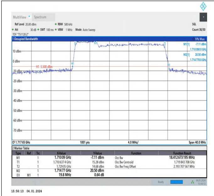
66-66-5MHz-15MHz-64QAM-64QAM-132002-132095-25RB# 0-75RB#0-PASS
