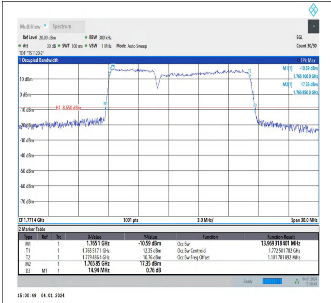
66-66-5MHz-10MHz-64QAM-64QAM-132550-132622-25RB# 0-50RB#0-PASS
