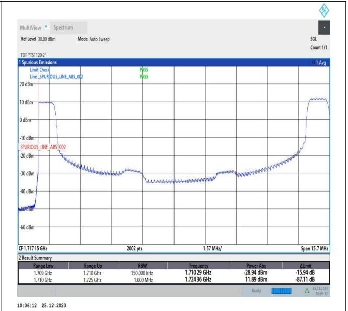
5MHz-10MHz_16QAM@16QAM-16QAM@16QAM_132000-132072_1RB#0@25RB#0-1RB#49@50RB#0
