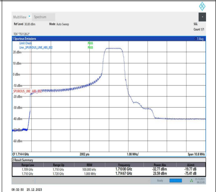
5MHz-5MHz_16QAM@16QAM-16QAM@16QAM_131997-132045_1RB#24@25RB#0-0RB#0@25RB#0
