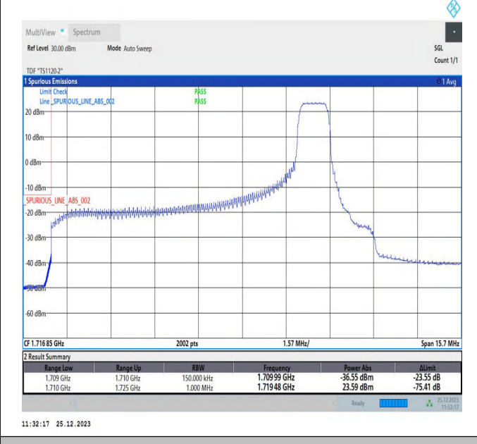
10MHz-5MHz_16QAM@16QAM-16QAM@16QAM_132022-1 32094_1RB#49@50RB#0-0RB#0@25RB#0
