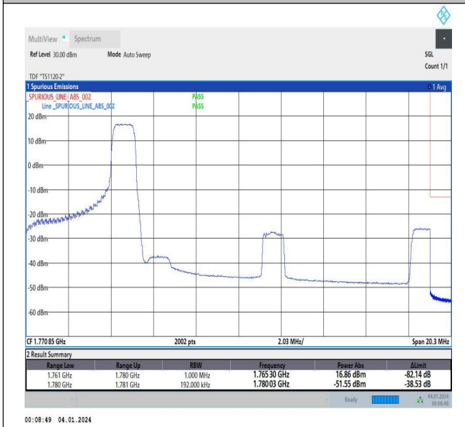
5MHz-15MHz_16QAM@16QAM-16QAM@16QAM_132504-132597_1RB#24@25RB#0-0RB#0@75RB#0
