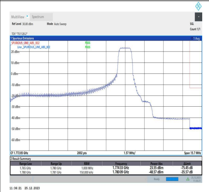
10MHz-5MHz_16QAM@16QAM-16QAM@16QAM_132572-1 32644_1RB#49@50RB#0-0RB#0@25RB#0
