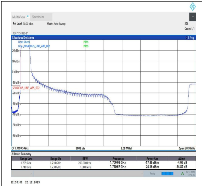
10MHz-10MHz_QPSK@QPSK-QPSK@QPSK_132022-1321_21_1RB#0@50RB#0-0RB#0@50RB#0
