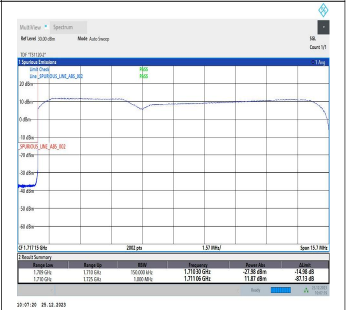
5MHz-10MHz_16QAM@16QAM-16QAM@16QAM_132000-132072_25RB#0@25RB#0-50RB#0@50RB#0
