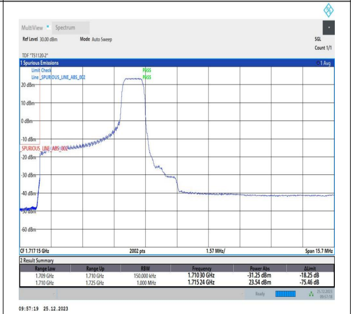
5MHz-10MHz_16QAM@16QAM-16QAM@16QAM_132000-1 32072_1RB#24@25RB#0-0RB#0@50RB#0
