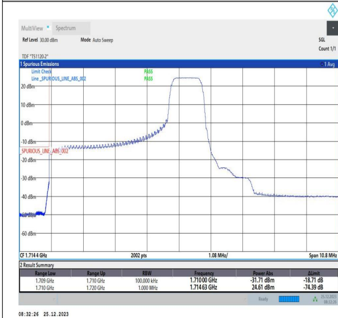
5MHz-5MHz_QPSK@QPSK-QPSK@QPSK_131997-132045_1RB#24@25RB#0-0RB#0@25RB#0
