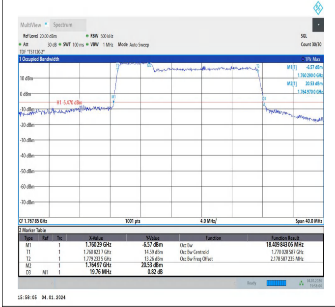
66-66-5MHz-15MHz-64QAM-64QAM-132504-132597-25RB# 0-75RB#0-PASS
