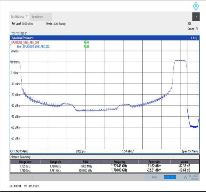
5MHz-10MHz_16QAM@16QAM-16QAM@16QAM_132550-132622_1RB#0@25RB#0-1RB#49@50RB#0
