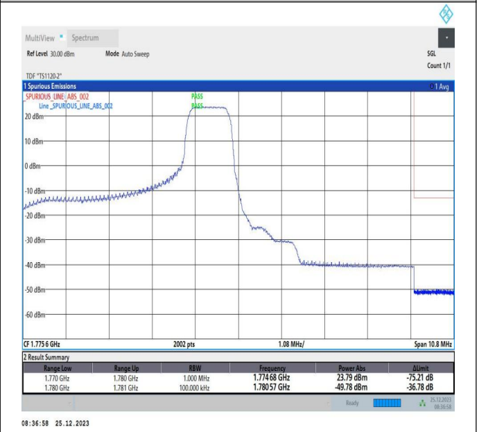
5MHz-5MHz_16QAM@16QAM-16QAM@16QAM_132599-132647_1RB#24@25RB#0-0RB#0@25RB#0
