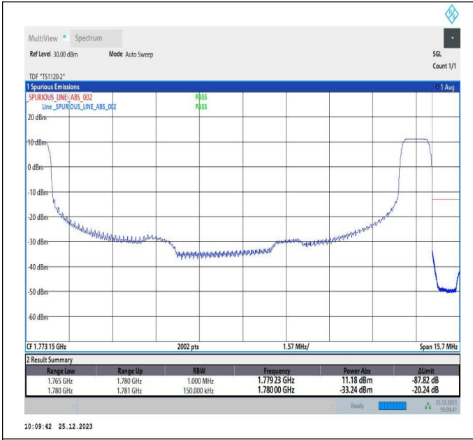
5MHz-10MHz_QPSK@QPSK-QPSK@QPSK_132550-13262_2_1RB#0@25RB#0-1RB#49@50RB#0
