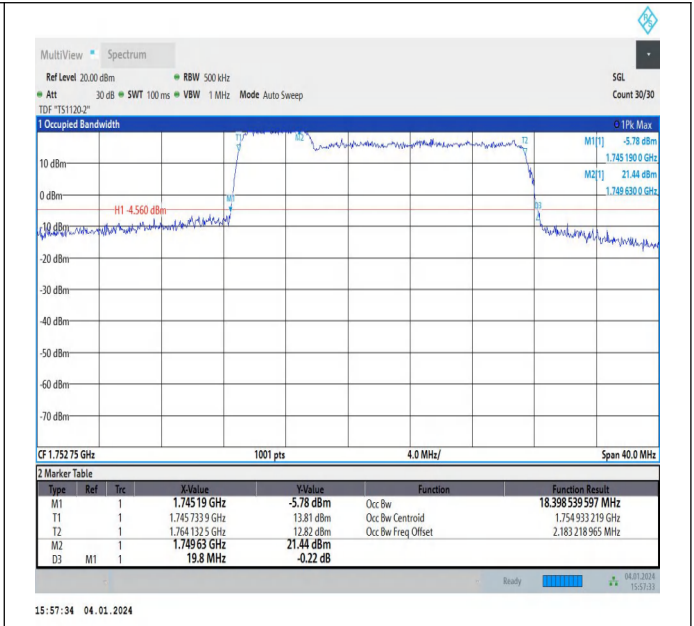
66-66-5MHz-15MHz-64QAM-64QAM-132353-132446-25RB# 0-75RB#0-PASS
