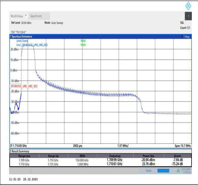
10MHz-5MHz_16QAM@16QAM-16QAM@16QAM_132022-1 32094_1RB#0@50RB#0-0RB#0@25RB#0
