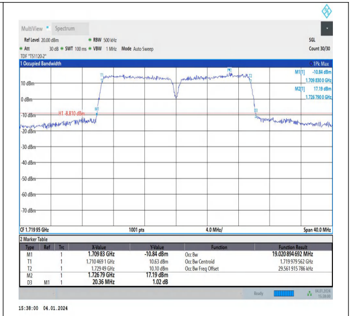
66-66-10MHz-10MHz-64QAM-64QAM-132022-132121-50RB#0-50RB#0-PASS
