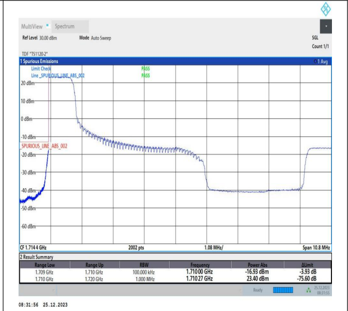
5MHz-5MHz_16QAM@16QAM-16QAM@16QAM_131997-132045_1RB#0@25RB#0-0RB#0@25RB#0
