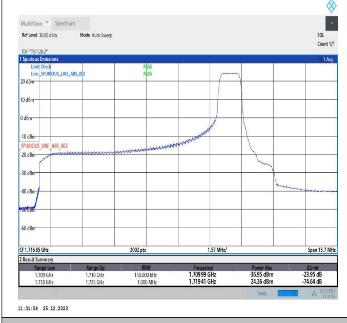
10MHz-5MHz_QPSK@QPSK-QPSK@QPSK_132022-13209 4_1RB#49@50RB#0-0RB#0@25RB#0
