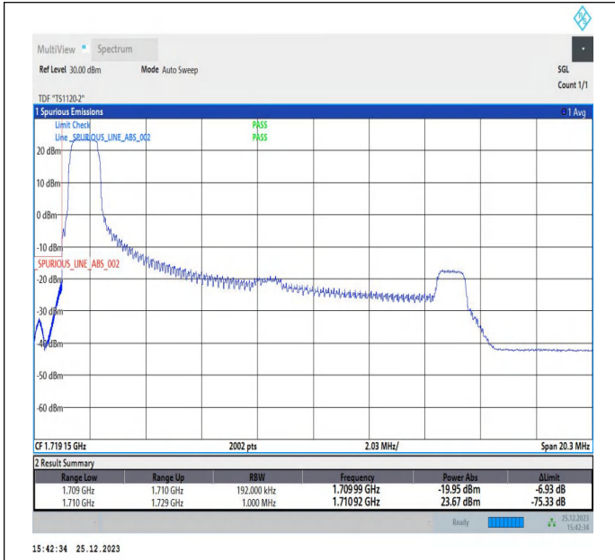
15MHz-5MHz_16QAM@16QAM-16QAM@16QAM_132047-132140_1RB#0@75RB#0-0RB#0@25RB#0
