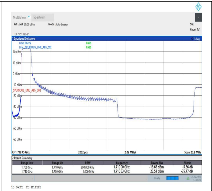
10MHz-10MHz_16QAM@16QAM-16QAM@16QAM_132022-132121_1RB#0@50RB#0-0RB#0@50RB#0
