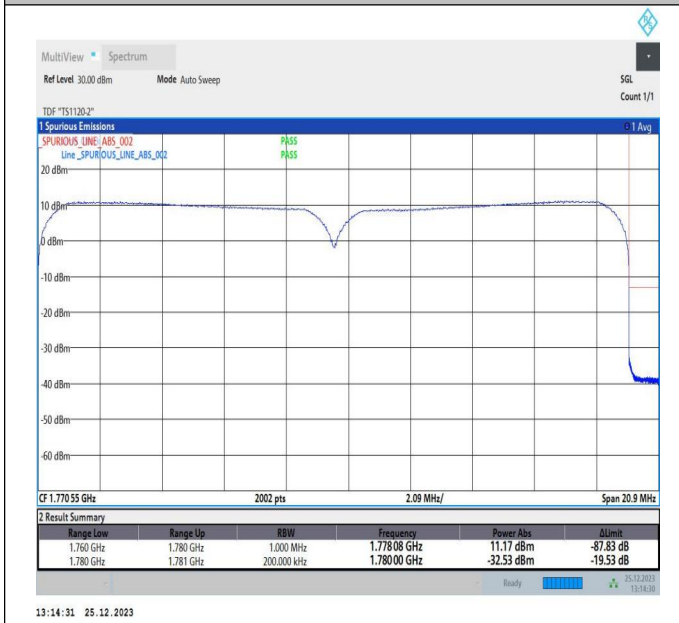
10MHz-10MHz_QPSK@QPSK-QPSK@QPSK_132523-132622_50RB#0@50RB#0-50RB#0@50RB#0
