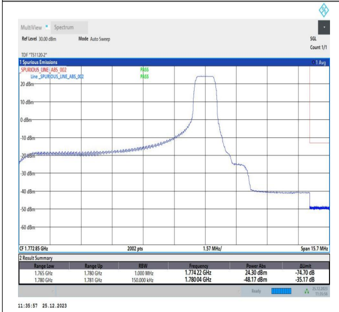
10MHz-5MHz_QPSK@QPSK-QPSK@QPSK_132572-13264 4_1RB#49@50RB#0-0RB#0@25RB#0
