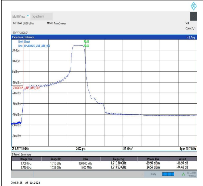
5MHz-10MHz_QPSK@QPSK-QPSK@QPSK_132000-13207 2_1RB#24@25RB#0-0RB#0@50RB#0
