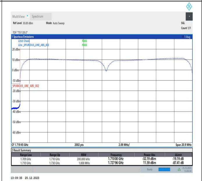
10MHz-10MHz_16QAM@16QAM-16QAM@16QAM_132022-132121_50RB#0@50RB#0-50RB#0@50RB#0
