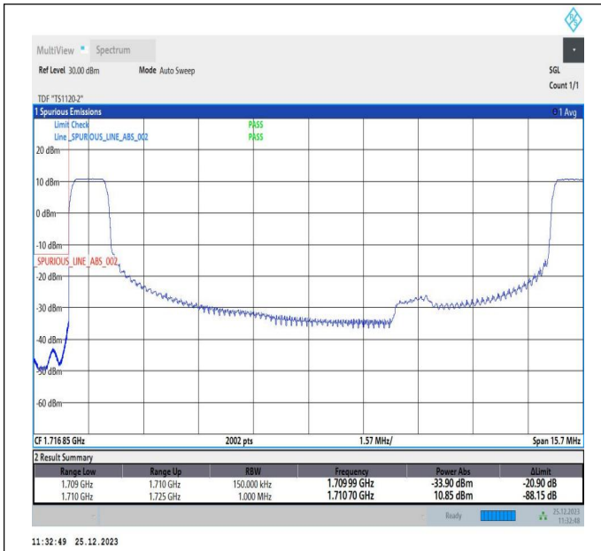
10MHz-5MHz_QPSK@QPSK-QPSK@QPSK_132022-13209 4_1RB#0@50RB#0-1RB#24@25RB#0
