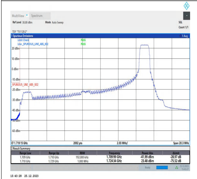
15MHz-5MHz_16QAM@16QAM-16QAM@16QAM_132047-132140_1RB#74@75RB#0-0RB#0@25RB#0
