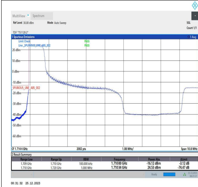
5MHz-5MHz_QPSK@QPSK-QPSK@QPSK_131997-132045_1RB#0@25RB#0-0RB#0@25RB#0
