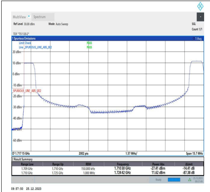
5MHz-10MHz_QPSK@QPSK-QPSK@QPSK_132000-132072_1RB#0@25RB#0-1RB#49@50RB#0
