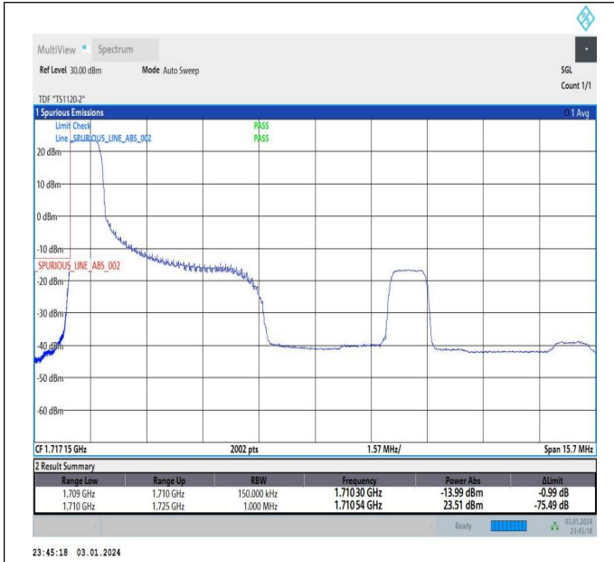
5MHz-10MHz_QPSK@QPSK-QPSK@QPSK_132000-13207 2_1RB#0@25RB#0-0RB#0@50RB#0
