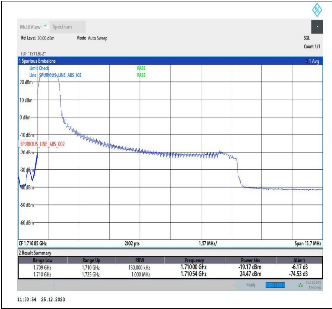
10MHz-5MHz_QPSK@QPSK-QPSK@QPSK_132022-13209 4_1RB#0@50RB#0-0RB#0@25RB#0
