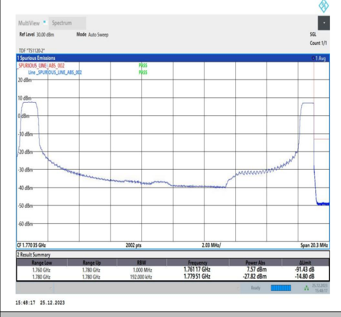
15MHz-5MHz_QPSK@QPSK-QPSK@QPSK_132549-13264_2_1RB#0@75RB#0-1RB#24@25RB#0
