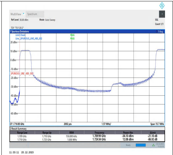
10MHz-5MHz_16QAM@16QAM-16QAM@16QAM_132022-1 32094_1RB#0@50RB#0-1RB#24@25RB#0
