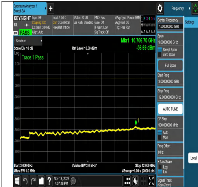
NTNV_N5_PC3_15_20_L_TID1_N/A_3000_12000_#1
