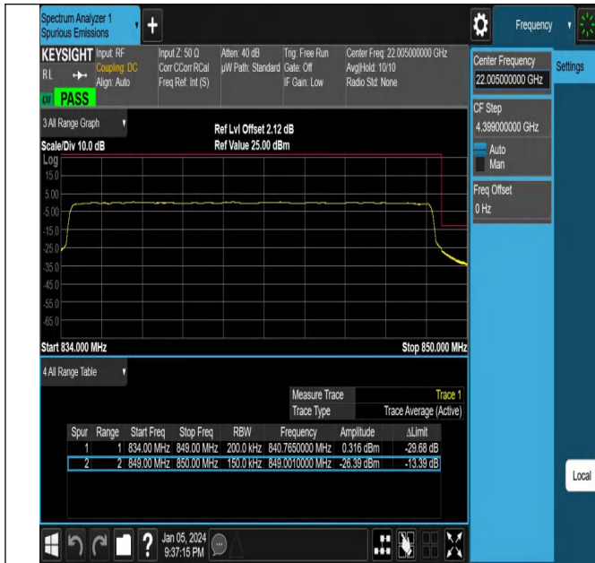
NTNV_N5_PC3_15_15_H_TID22_#1
