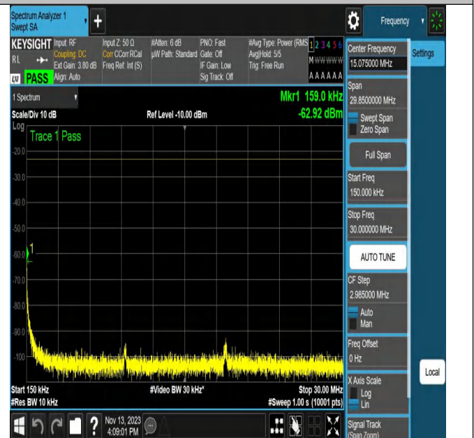
NTNV_N5_PC3_15_20_L_TID2_N/A_0.15_30_#1
