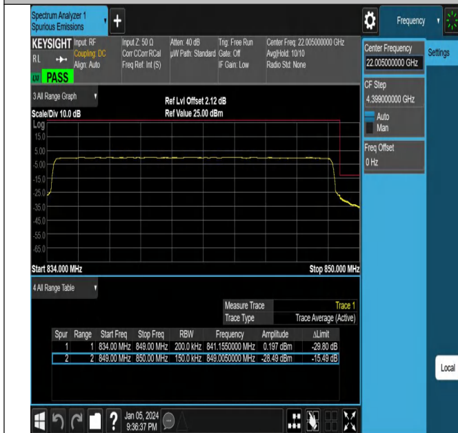
NTNV_N5_PC3_15_15_H_TID19_#1
