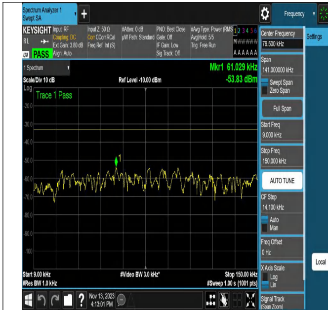
NTNV_N5_PC3_15_20_L_TID5_N/A_0.009_0.15_#1
