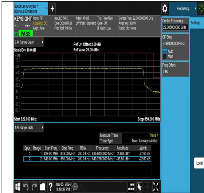
NTNV_N5_PC3_15_20_H_TID4_#1
