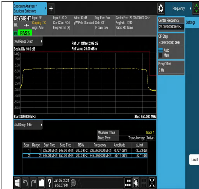
NTNV_N5_PC3_15_20_H_TID22_#1
