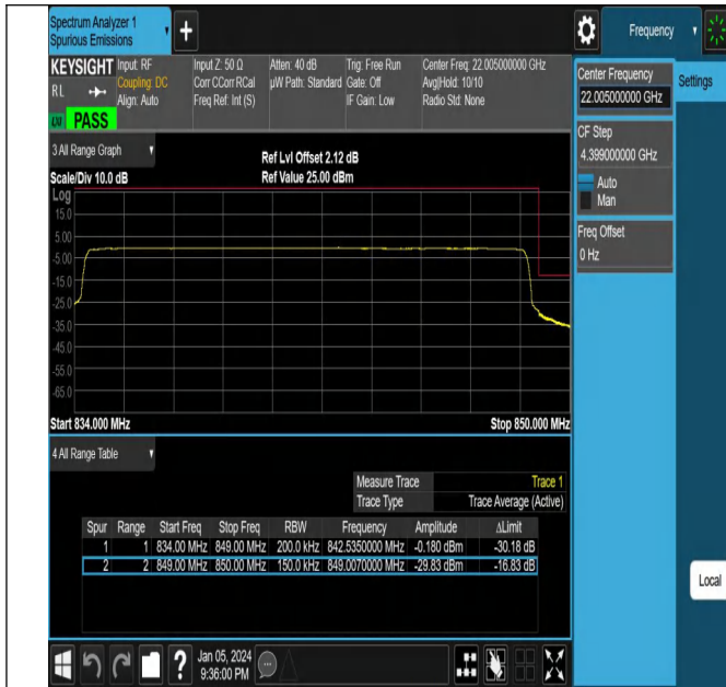
NTNV_N5_PC3_15_15_H_TID16_#1
