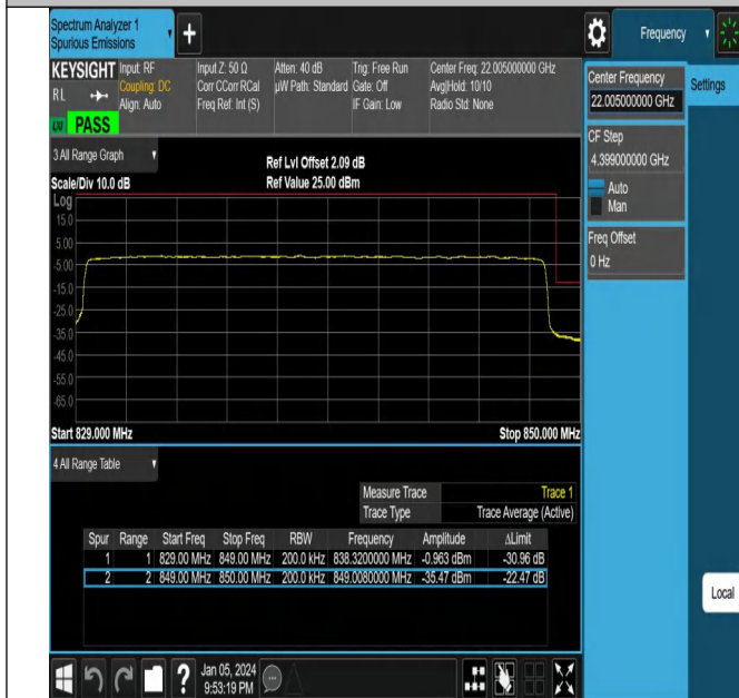
NTNV_N5_PC3_15_20_H_TID19_#1
