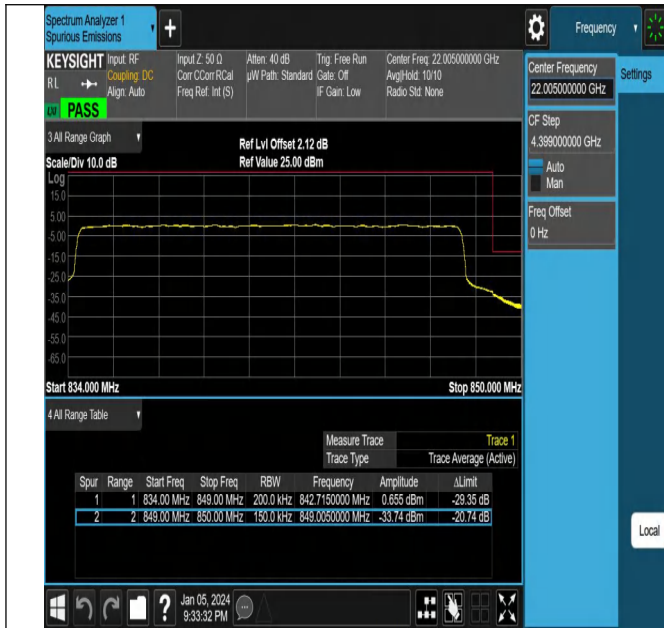
NTNV_N5_PC3_15_15_H_TID10_#1
