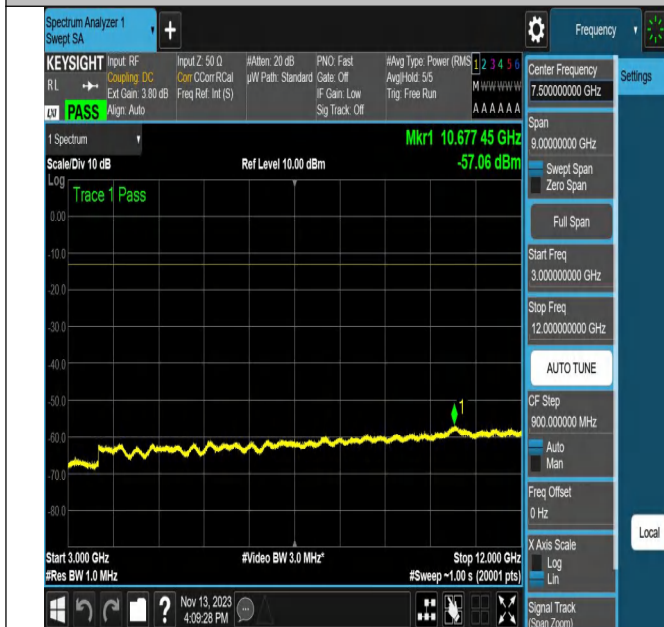
NTNV_N5_PC3_15_20_L_TID2_N/A_3000_12000_#1
