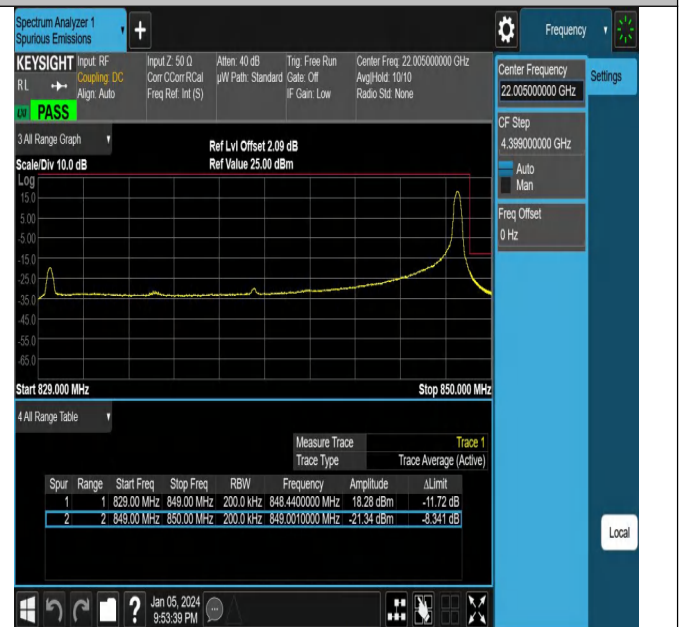
NTNV_N5_PC3_15_20_H_TID21_#1
