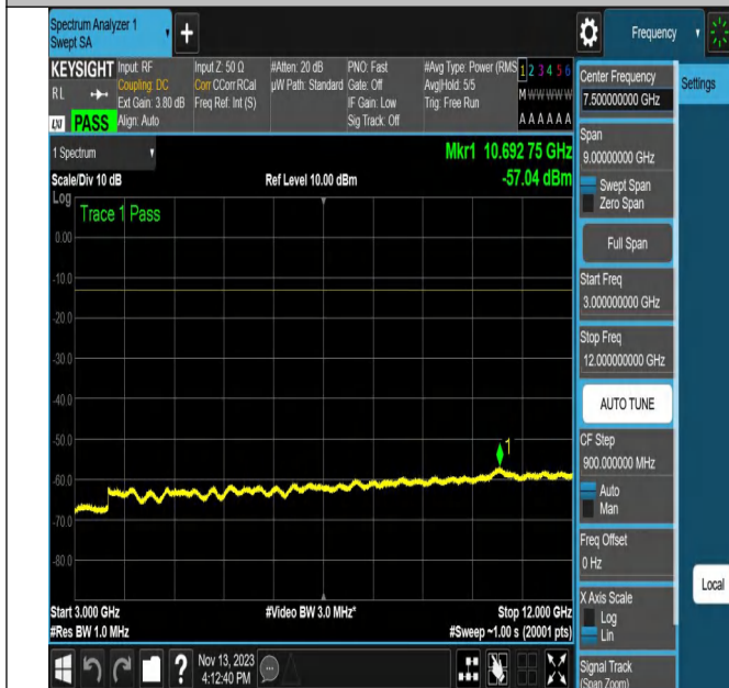
NTNV_N5_PC3_15_20_L_TID4_N/A_3000_12000_#1
