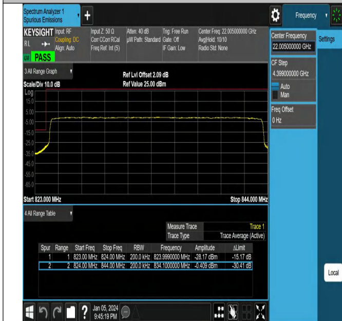
NTNV_N5_PC3_15_20_L_TID22_#1
