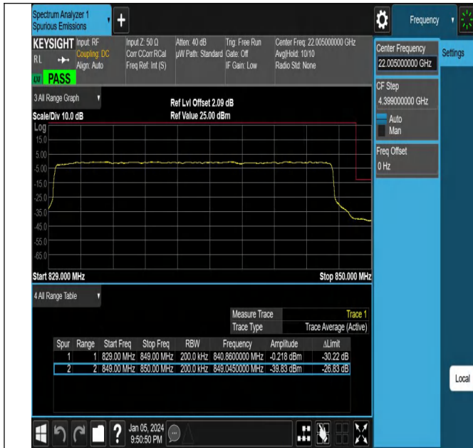
NTNV_N5_PC3_15_20_H_TID10_#1
