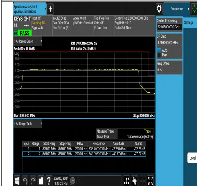
NTNV_N5_PC3_15_20_H_TID1_#1
