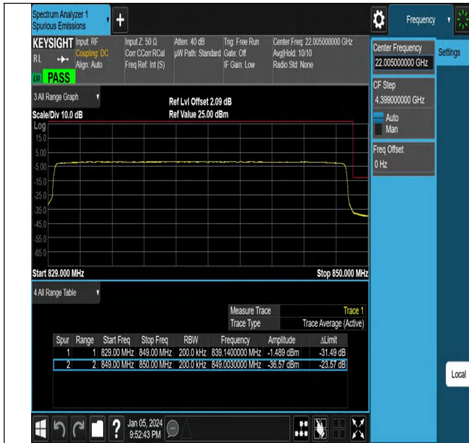
NTNV_N5_PC3_15_20_H_TID16_#1
