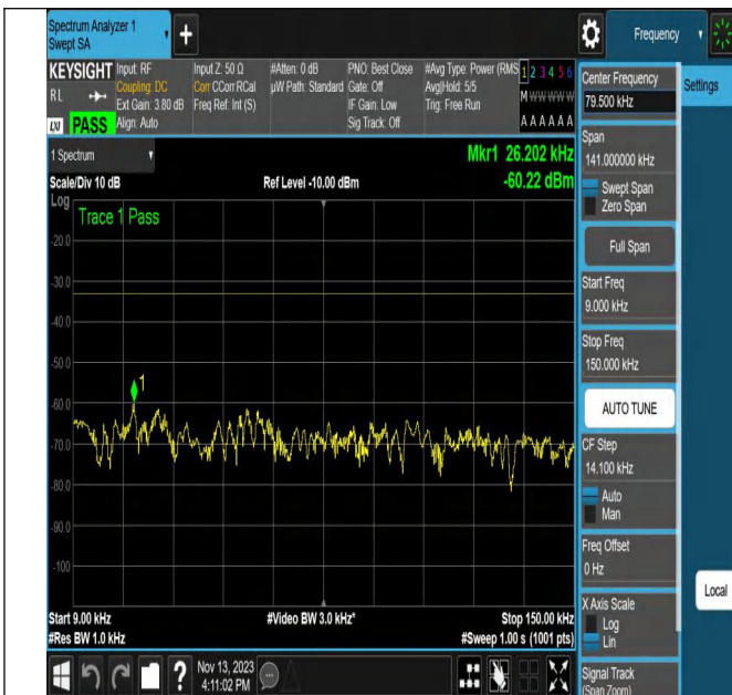
NTNV_N5_PC3_15_20_L_TID3_N/A_0.009_0.15_#1
