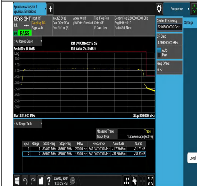
NTNV_N5_PC3_15_15_H_TID25_#1
