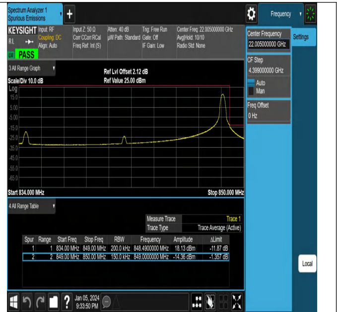
NTNV_N5_PC3_15_15_H_TID12_#1
