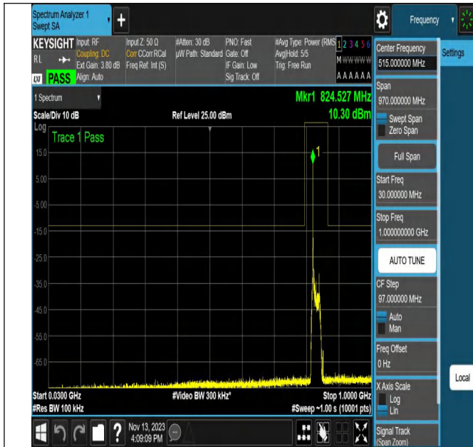
NTNV_N5_PC3_15_20_L_TID2_N/A_30_1000_#1
