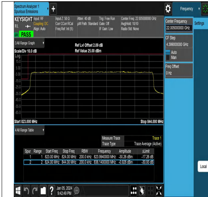
NTNV_N5_PC3_15_20_L_TID13_#1
