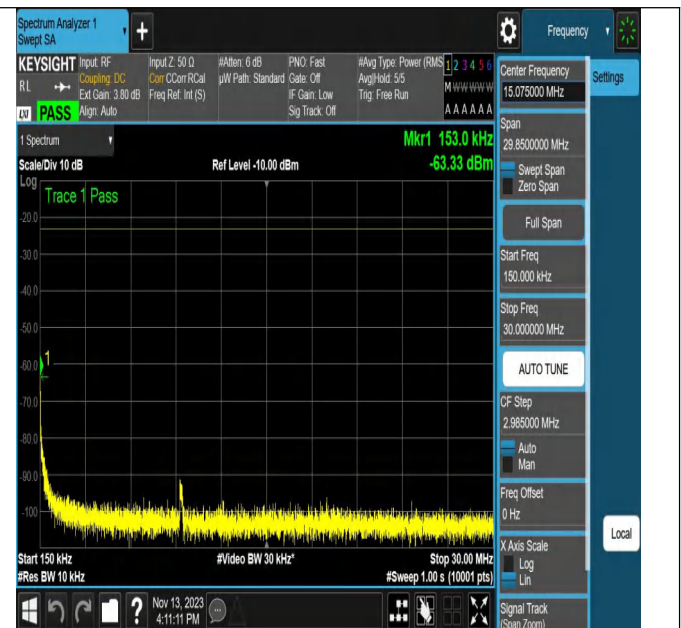
NTNV_N5_PC3_15_20_L_TID3_N/A_0.15_30_#1
