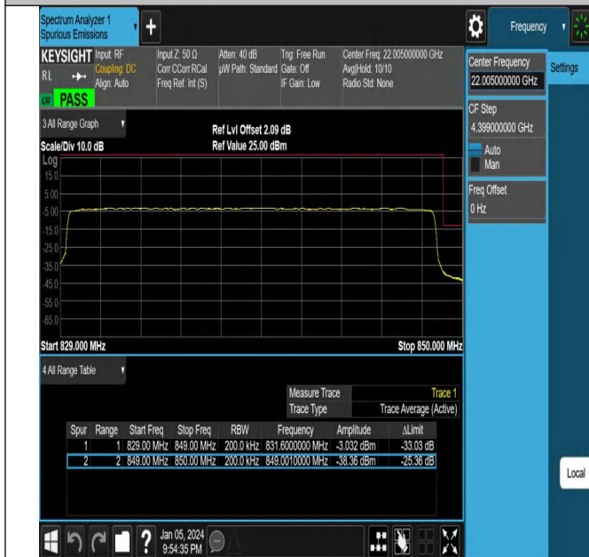
NTNV_N5_PC3_15_20_H_TID25_#1
