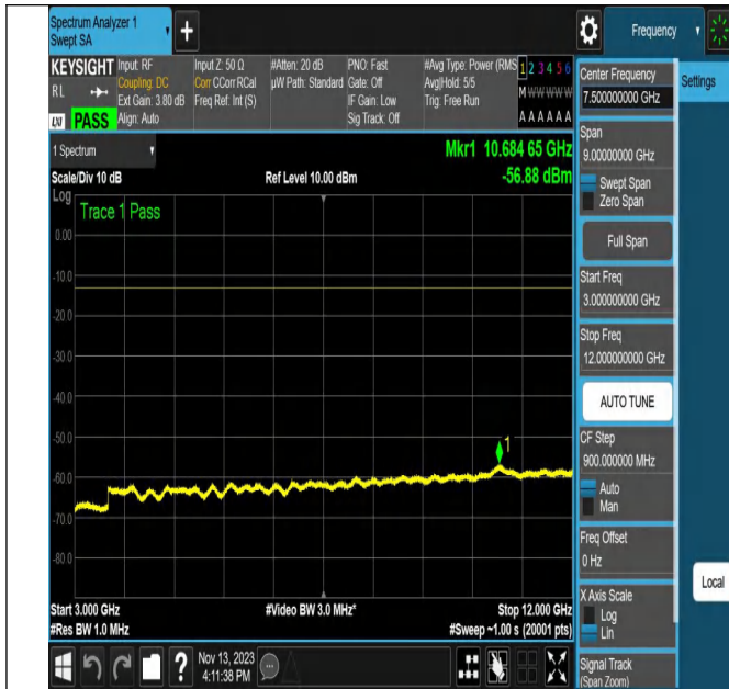
NTNV_N5_PC3_15_20_L_TID3_N/A_3000_12000_#1
