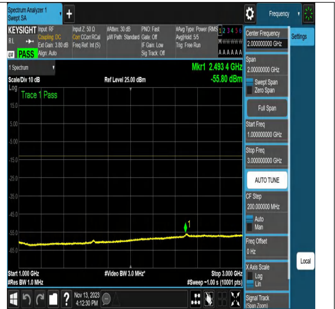
NTNV_N5_PC3_15_20_L_TID4_N/A_1000_3000_#1
