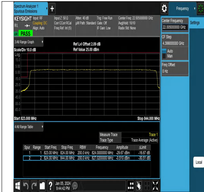
NTNV_N5_PC3_15_20_L_TID19_#1
