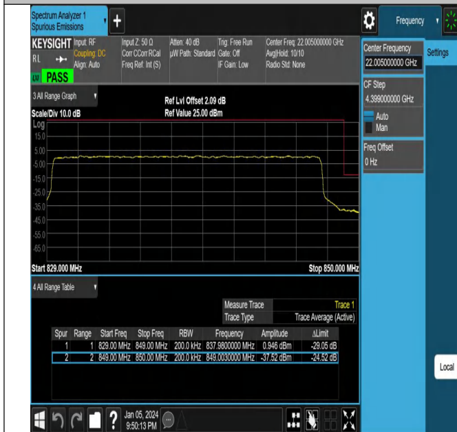
NTNV_N5_PC3_15_20_H_TID7_#1
