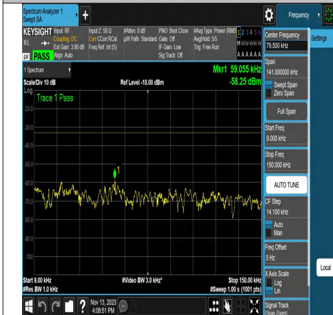
NTNV_N5_PC3_15_20_L_TID2_N/A_0.009_0.15_#1
