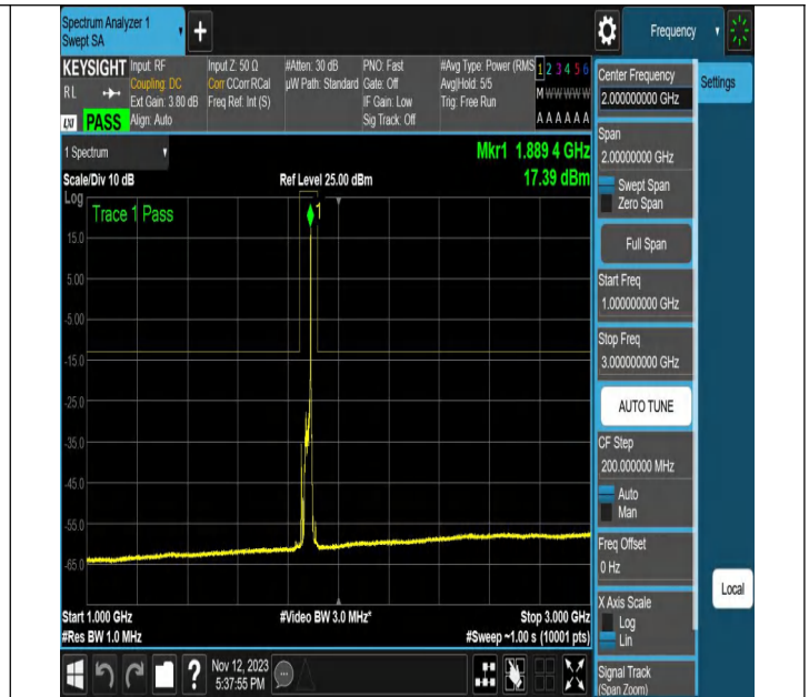
NTNV-N2-PC3-15-20-M-DFT-PI2BPSK-Edge_1RB_Right-Ant1- PASS
