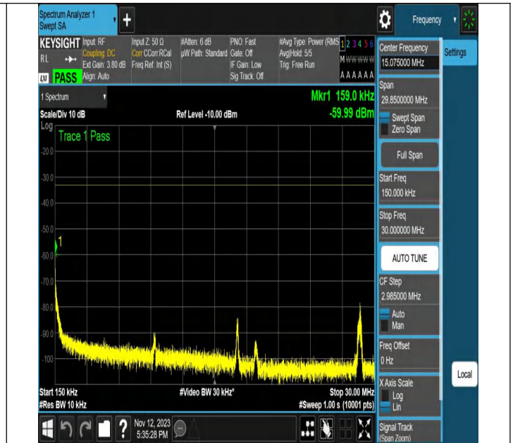
NTNV-N2-PC3-15-20-M-DFT-PI2BPSK-Edge_1RB_Left-Ant1-P
