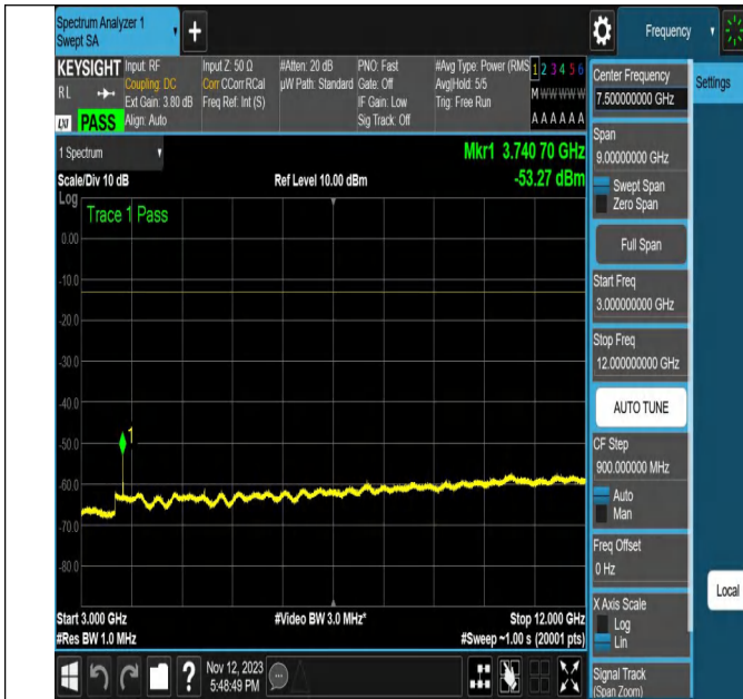
NTVN-N2-PC3-15-20-M-DFT-256QAM-Edge_1RB_Left-Ant1-PA
