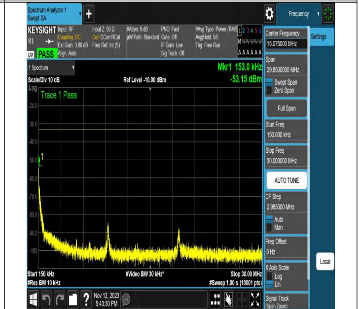
NTNV-N2-PC3-15-20-M-DFT-16QAM-Edge_1RB_Right-Ant1-P
