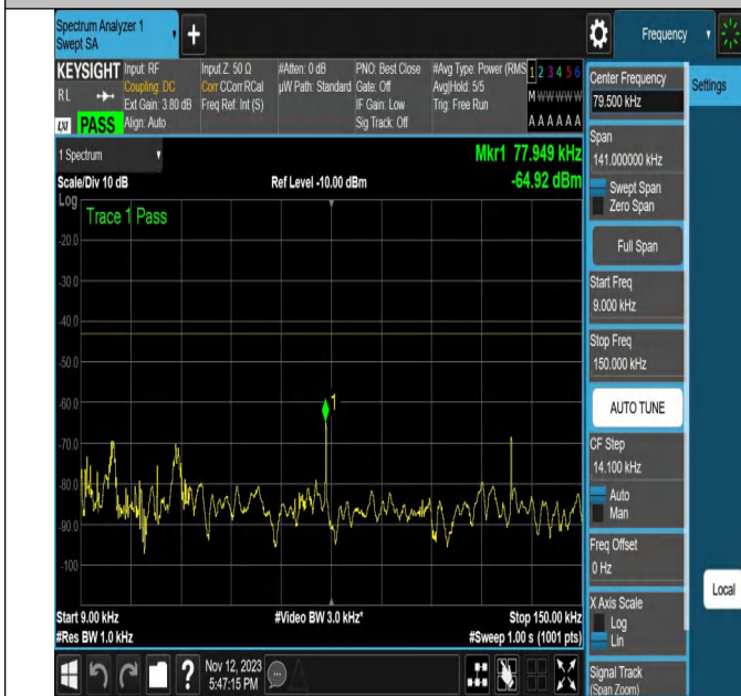
NTNV-N2-PC3-15-20-M-DFT-256QAM-Outer_Full-Ant1-PASS
