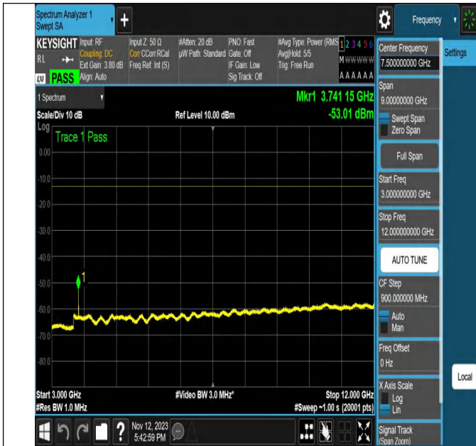
NTNV-N2-PC3-15-20-M-DFT-16QAM-Edge_1RB_Left-Ant1-PA
