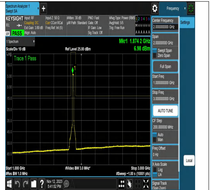
NTNV-N2-PC3-15-20-M-DFT-16QAM-Outer_Full-Ant1-PASS
