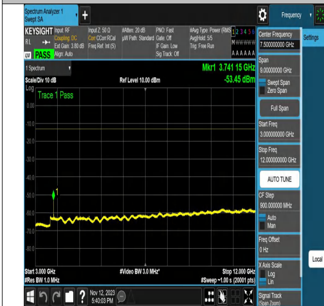
NTNV-N2-PC3-15-20-M-DFT-QPSK-Edge_1RB_Left-Ant1-PAS
