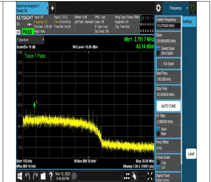
NTNV-N2-PC3-15-20-M-DFT-64QAM-Outer_Full-Ant1-PASS
