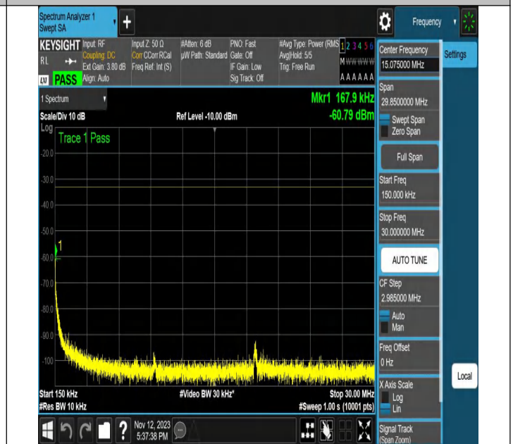
NTNV-N2-PC3-15-20-M-DFT-PI2BPSK-Edge_1RB_Right-Ant1- PASS
