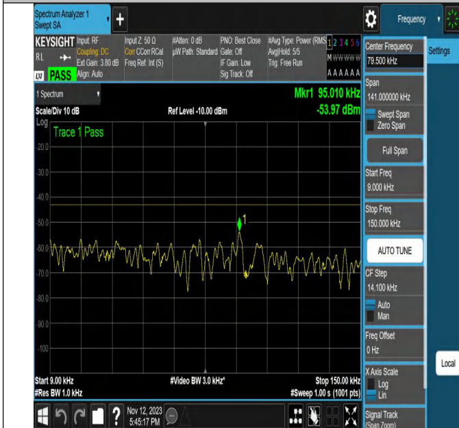
NTNV-N2-PC3-15-20-M-DFT-64QAM-Edge_1RB_Left-Ant1-PA
