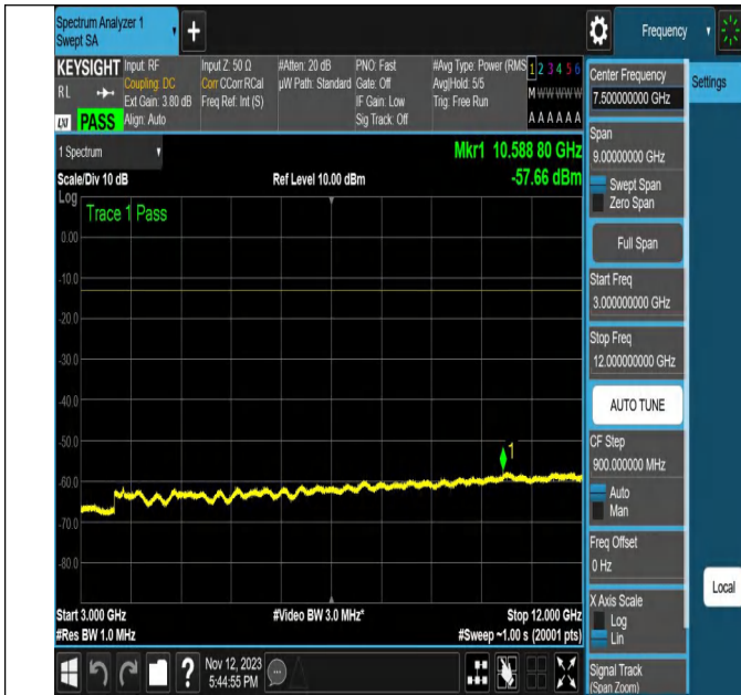
NTNV-N2-PC3-15-20-M-DFT-64QAM-Outer_Full-Ant1-PASS
