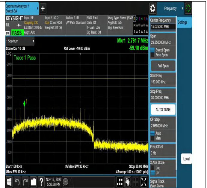
NTNV-N2-PC3-15-20-M-DFT-QPSK-Outer_Full-Ant1-PASS
