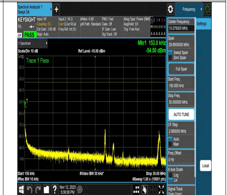
NTNV-N2-PC3-15-20-M-DFT-QPSK-Edge_1RB_Left-Ant1-PAS
