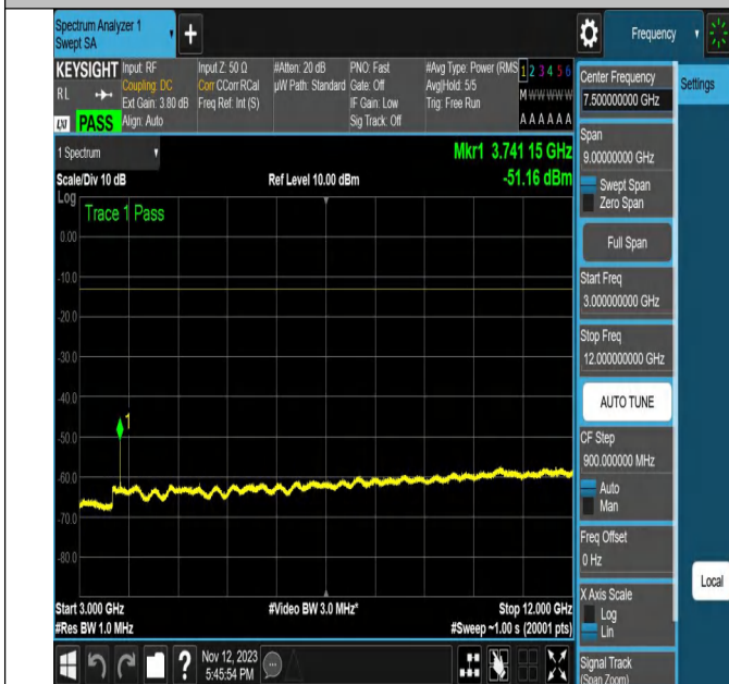
NTNV-N2-PC3-15-20-M-DFT-64QAM-Edge_1RB_Left-Ant1-PA
