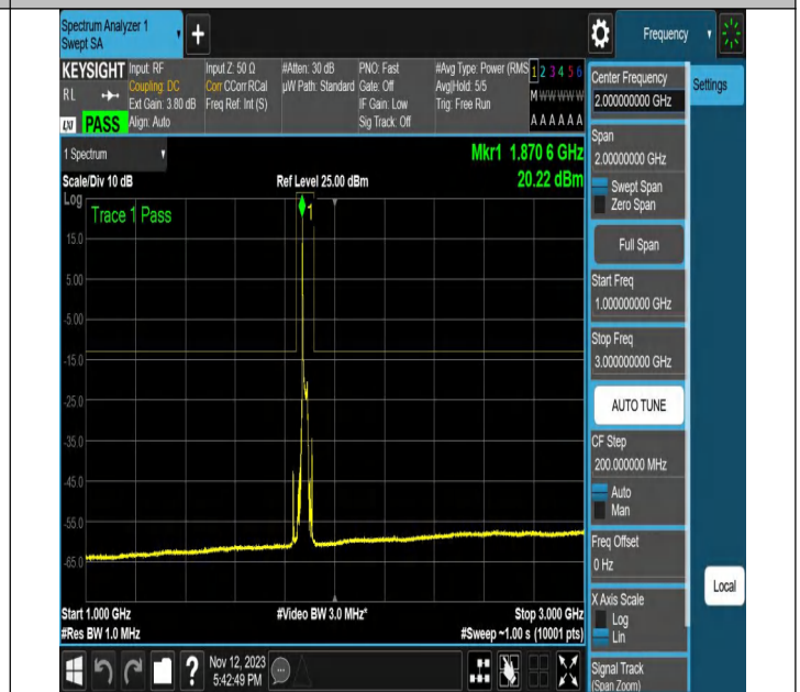
NTNV-N2-PC3-15-20-M-DFT-16QAM-Edge_1RB_Left-Ant1-PA
