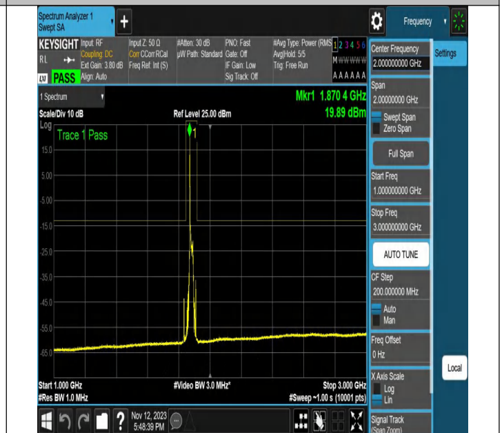
NTNV-N2-PC3-15-20-M-DFT-256QAM-Edge_1RB_Left-Ant1-PA
