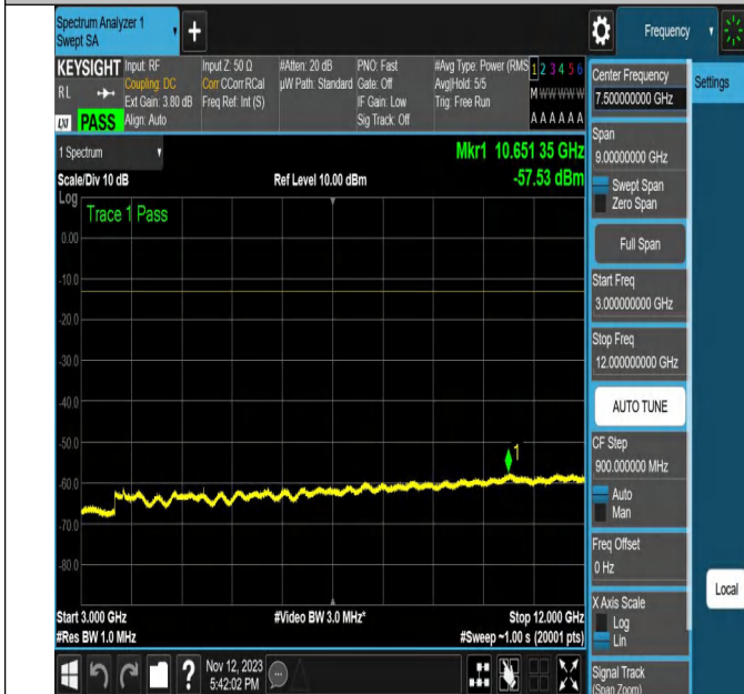
NTNV-N2-PC3-15-20-M-DFT-16QAM-Outer_Full-Ant1-PASS
