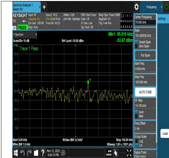
NTNV-N2-PC3-15-20-M-DFT-64QAM-Edge_1RB_Right-Ant1-P
