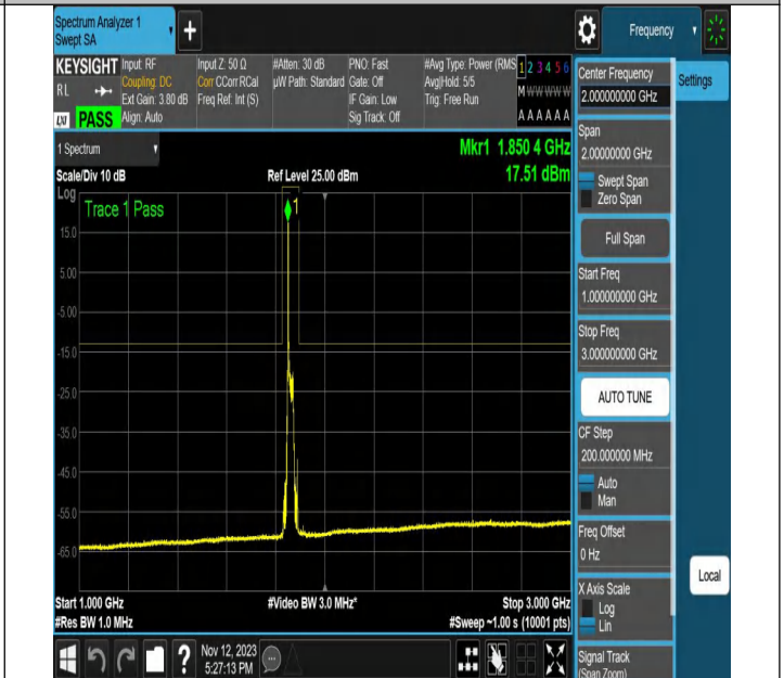
NTNV-N2-PC3-15-20-L-CP-64QAM-Edge_1RB_Left-Ant1-PASS
