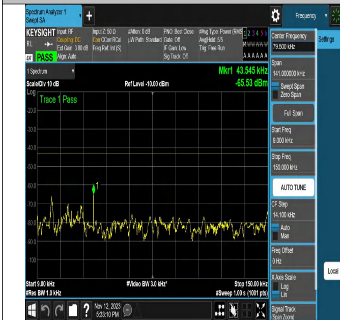
NTVN-N2-PC3-15-20-M-DFT-PI2BPSK-Outet_Full-Ant1-PASS
