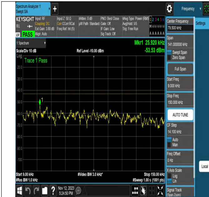
NTVN-N2-PC3-15-20-L-CP-16QAM-Edge_1RB_Right-Ant1-PAS
