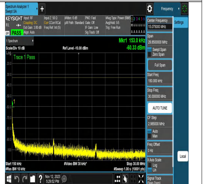
NTNV-N2-PC3-15-20-L-CP-256QAM-Edge_1RB_Left-Ant1-PAS
