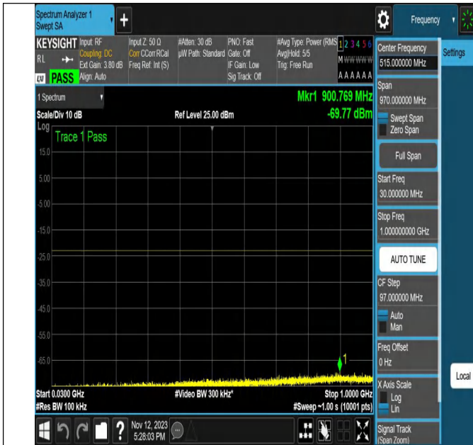
NTNV-N2-PC3-15-20-L-CP-64QAM-Edge_1RB_Right-Ant1-PAS
