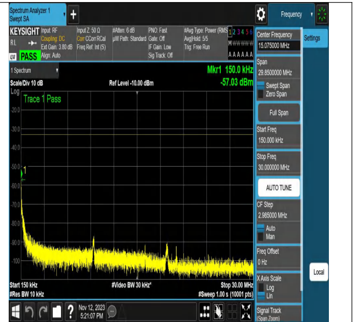
NTNV-N2-PC3-15-20-L-CP-QPSK-Edge_1RB_Left-Ant1-PASS
