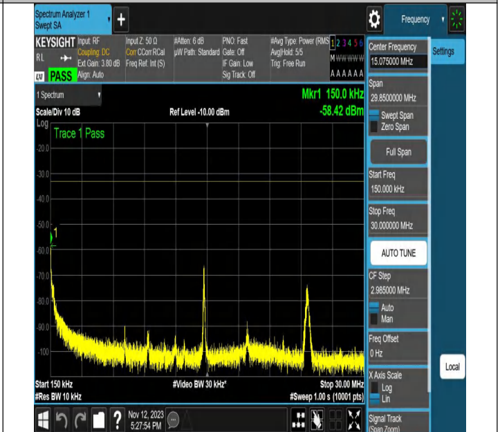
NTNV-N2-PC3-15-20-L-CP-64QAM-Edge_1RB_Right-Ant1-PAS
