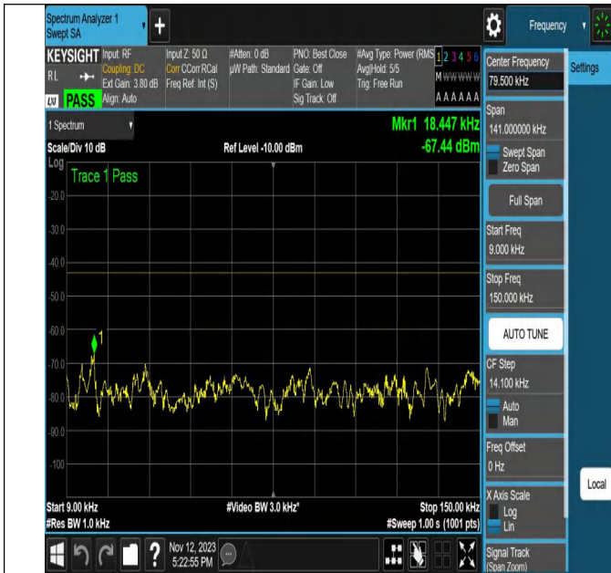
NTNV-N2-PC3-15-20-L-CP-16QAM-Outer_Full-Ant1-PASS
