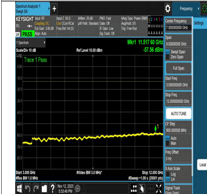
NTNV-N2-PC3-15-20-M-DFT-PI2BPSK-Outter_Full-Ant1-PASS
