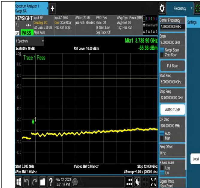
NTVN-N2-PC3-15-20-L-CP-256QAM-Edge_1RB_Right-Ant1-PA
