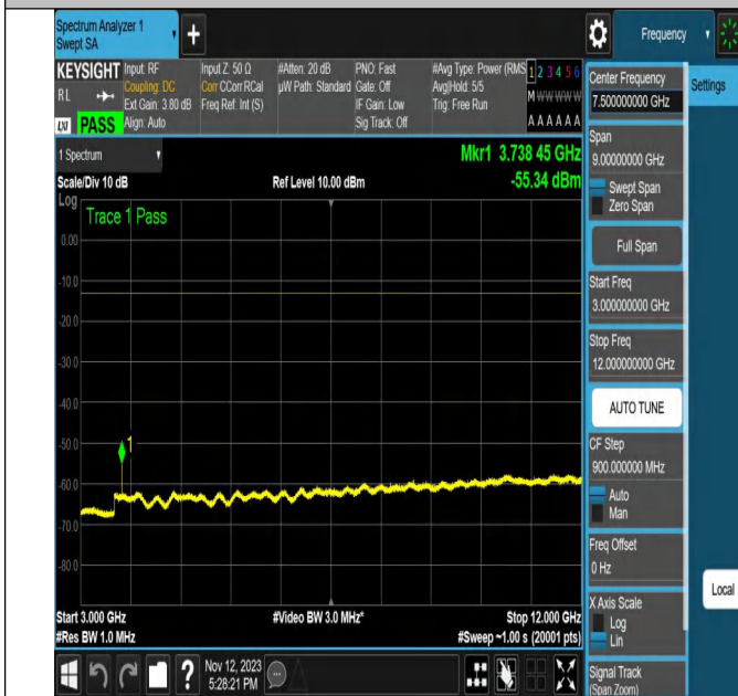
NTNV-N2-PC3-15-20-L-CP-64QAM-Edge_1RB_Right-Ant1-PAS
