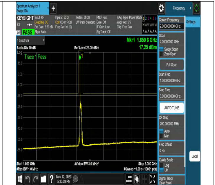
NTVN-N2-PC3-15-20-L-CP-256QAM-Edge_1RB_Left-Ant1-PAS
