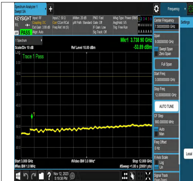
NTNV-N2-PC3-15-20-L-DFT-256QAM-Edge_1RB_Right-Ant1-P ASS
