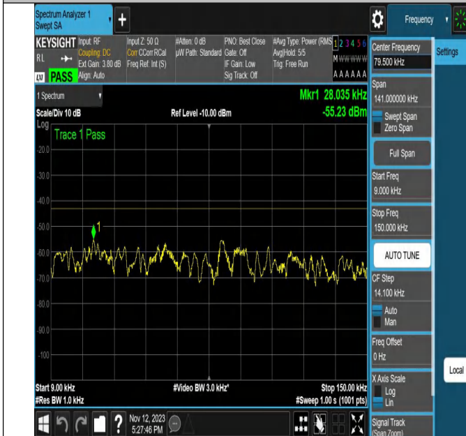
NTNV-N2-PC3-15-20-L-CP-64QAM-Edge_1RB_Right-Ant1-PAS
