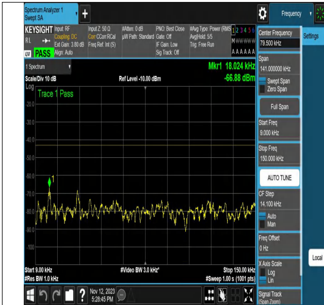
NTNV-N2-PC3-15-20-L-CP-256QAM-Outer_Full-Ant1-PASS
