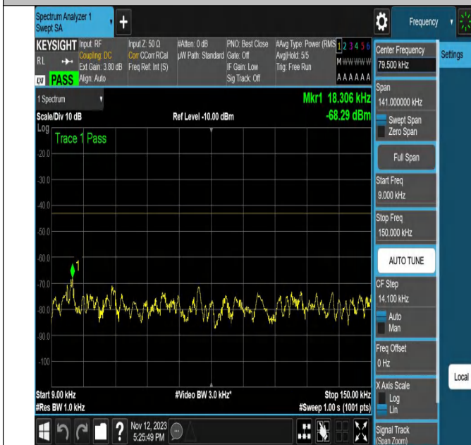
NTVN-N2-PC3-15-20-L-CP-64QAM-Outer_Full-Ant1-PASS
