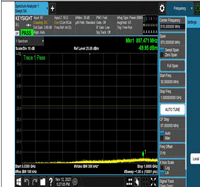
NTNV-N2-PC3-15-20-L-CP-64QAM-Edge_1RB_Left-Ant1-PASS
