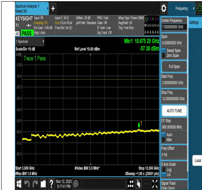
NTNV-N2-PC3-15-20-L-DFT-256QAM-Outer_Full-Ant1-PASS
