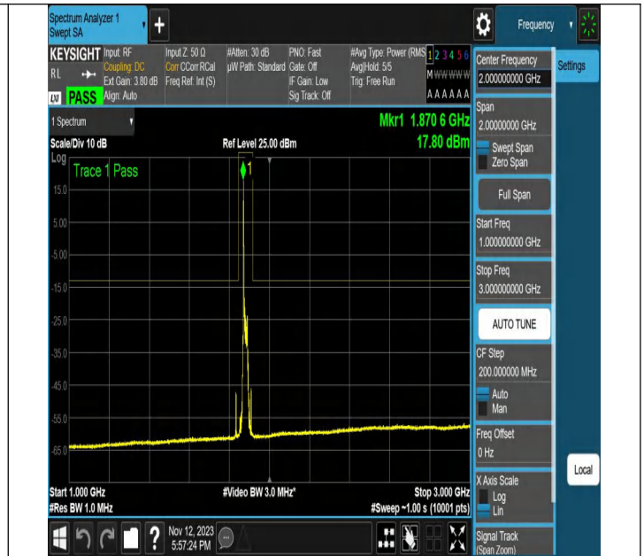
NTVN-N2-PC3-15-20-L-DFT-16QAM-Edge_1RB_Left-Ant1-PAS
