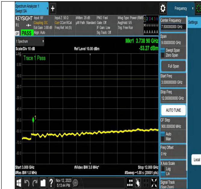
NTNV-N2-PC3-15-20-L-DFT-16QAM-Edge_1RB_Right-Ant1-PA
