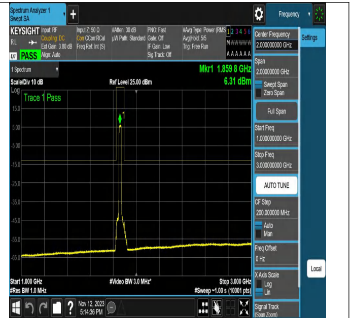
NTNV-N2-PC3-15-20-L-DFT-64QAM-Outer_Full-Ant1-PASS
