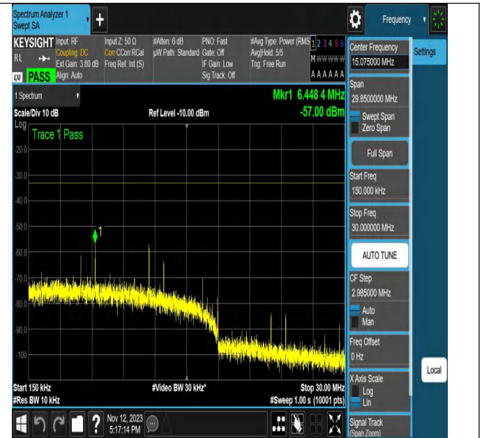
NTNV-N2-PC3-15-20-L-DFT-256QAM-Outer_Full-Ant1-PASS
