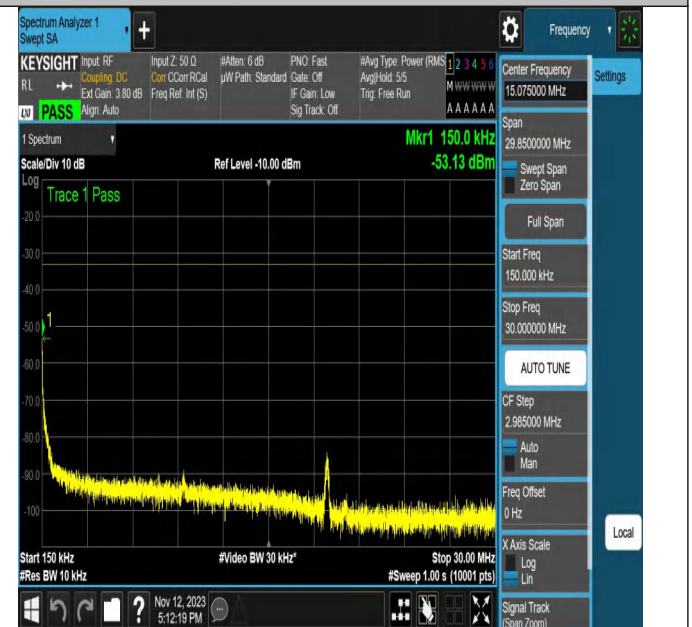
NTNV-N2-PC3-15-20-L-DFT-16QAM-Edge_1RB_Left-Ant1-PAS
