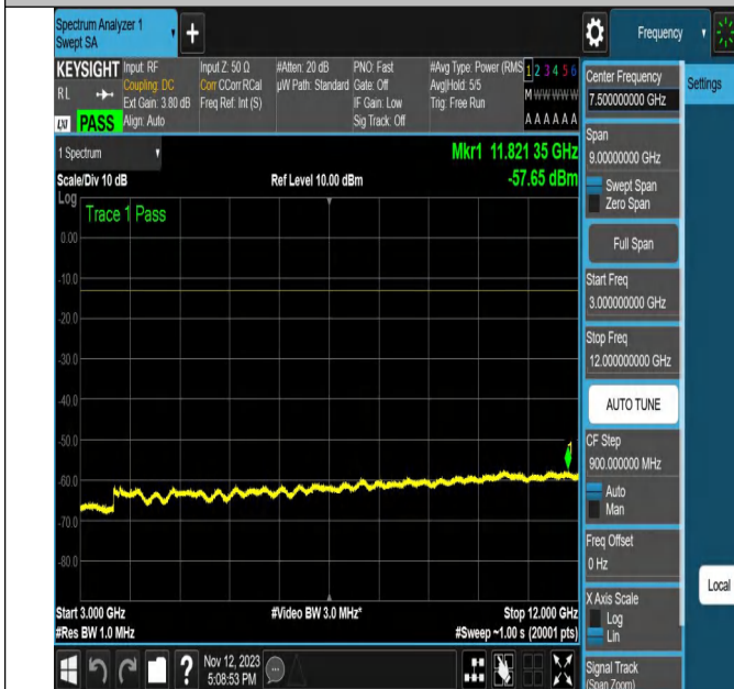
NTNV-N2-PC3-15-20-L-DFT-QPSK-Outer_Full-Ant1-PASS
