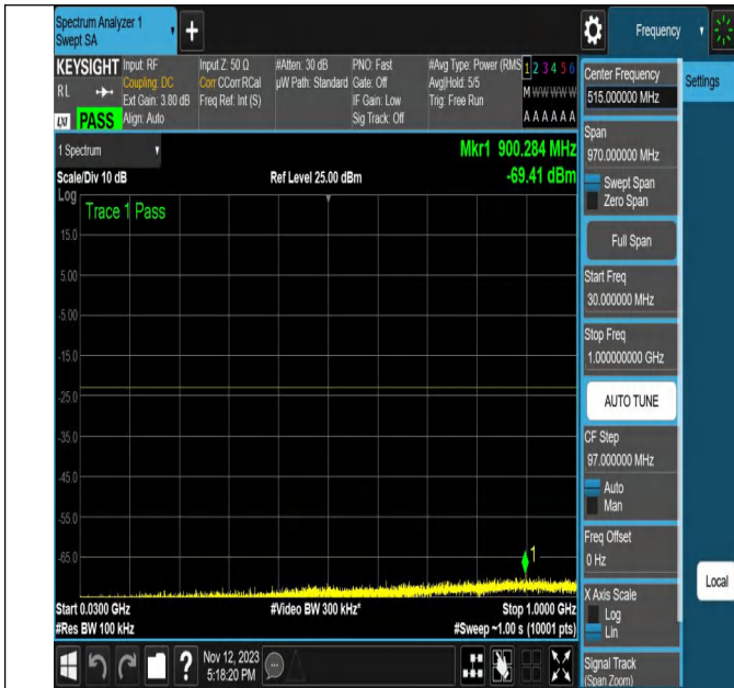
NTNV-N2-PC3-15-20-L-DFT-256QAM-Edge_1RB_Left-Ant1-PA
