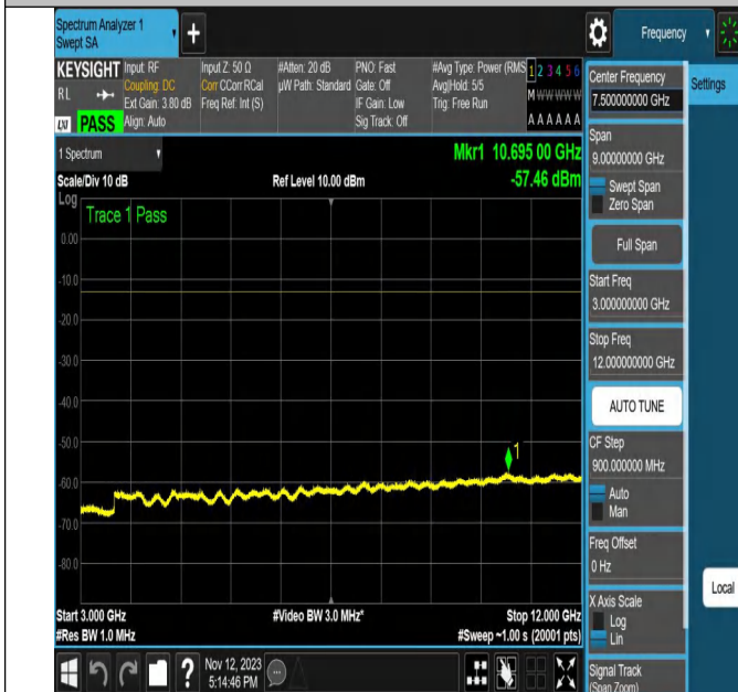
NTNV-N2-PC3-15-20-L-DFT-64QAM-Outer_Full-Ant1-PASS
