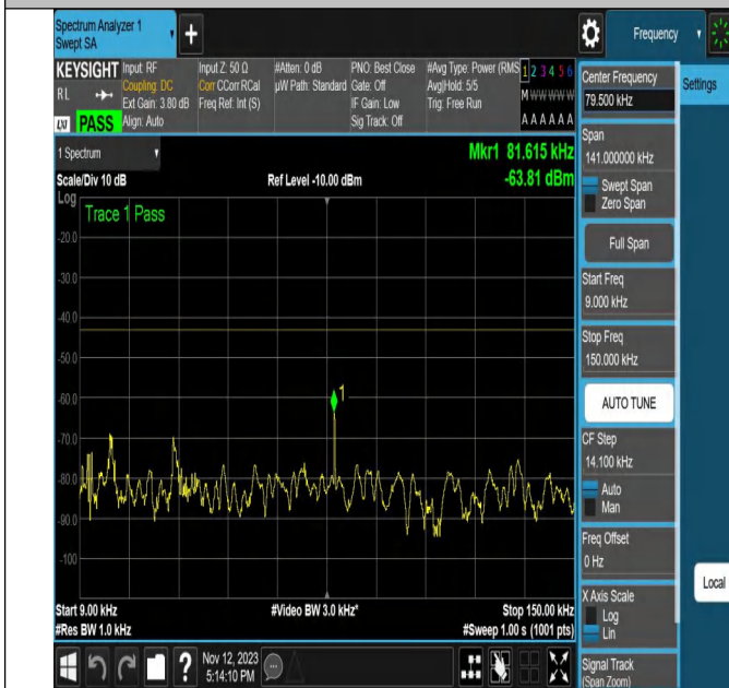
NTNV-N2-PC3-15-20-L-DFT-64QAM-Outer_Full-Ant1-PASS
