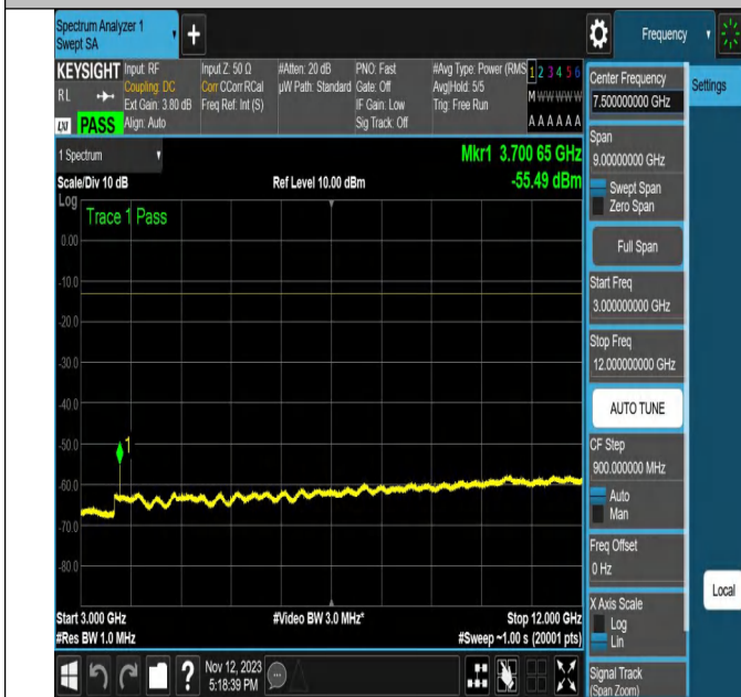
NTNV-N2-PC3-15-20-L-DFT-256QAM-Edge_1RB_Left-Ant1-PA
