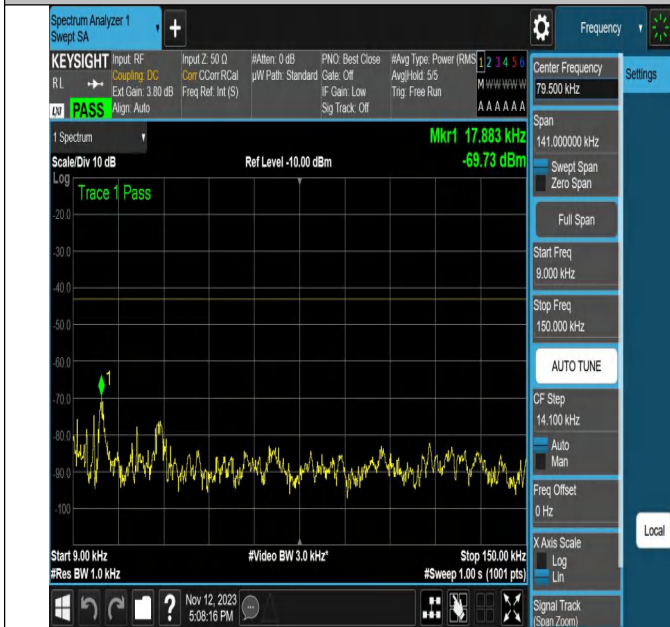
NTVN-N2-PC3-15-20-L-DFT-QPSK-Outer_Full-Ant1-PASS
