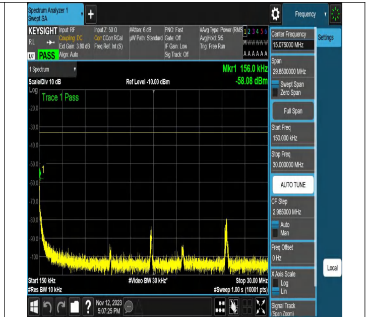
NTNV-N2-PC3-15-20-L-DFT-PI2BPSK-Edge_1RB_Right-Ant1-P ASS
