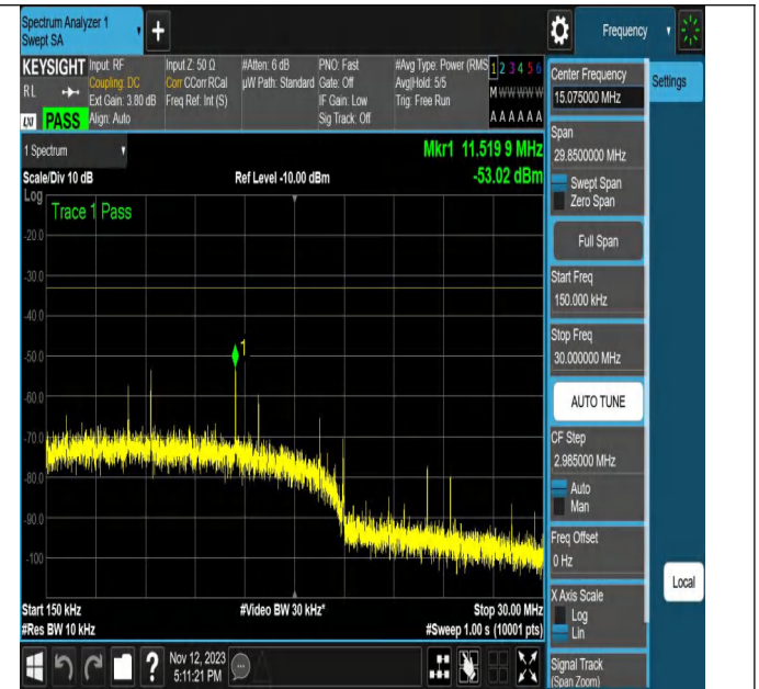
NTNV-N2-PC3-15-20-L-DFT-16QAM-Outer_Full-Ant1-PASS
