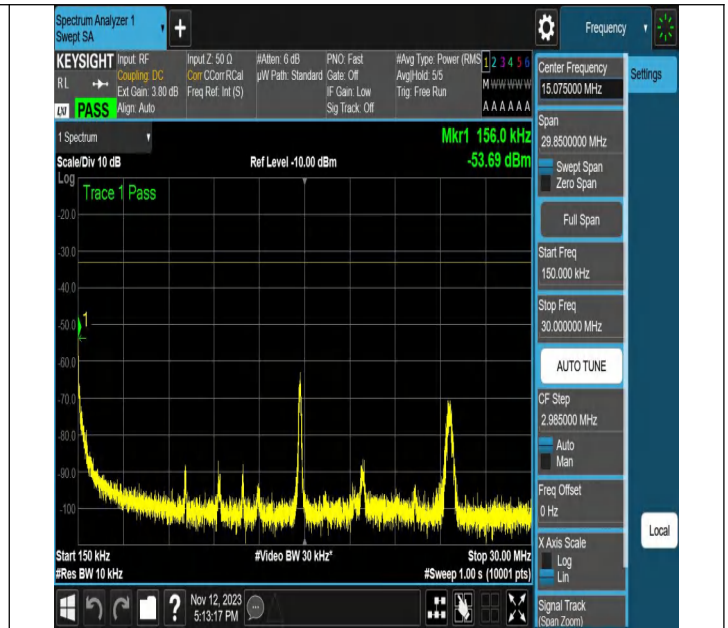
NTNV-N2-PC3-15-20-L-DFT-16QAM-Edge_1RB_Right-Ant1-PA
