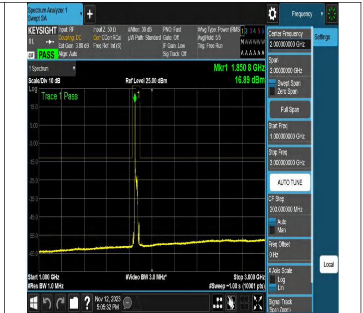
NTVN-N2-PC3-15-20-L-DFT-PI2BPSK-Edge_1RB_Left-Ant1-PA
