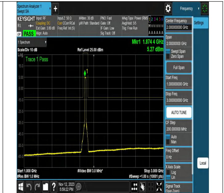
NTNV-N2-PC3-15-20-L-DFT-64QAM-Edge_1RB_Right-Ant1-PA
