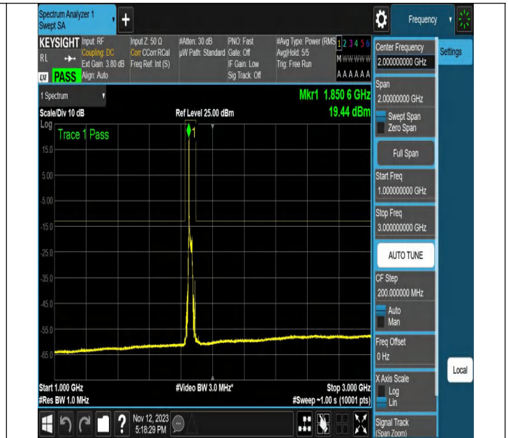
NTNV-N2-PC3-15-20-L-DFT-256QAM-Edge_1RB_Left-Ant1-PA
