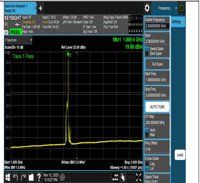
NTNV-N2-PC3-15-20-L-DFT-256QAM-Edge_1RB_Right-Ant1-P
