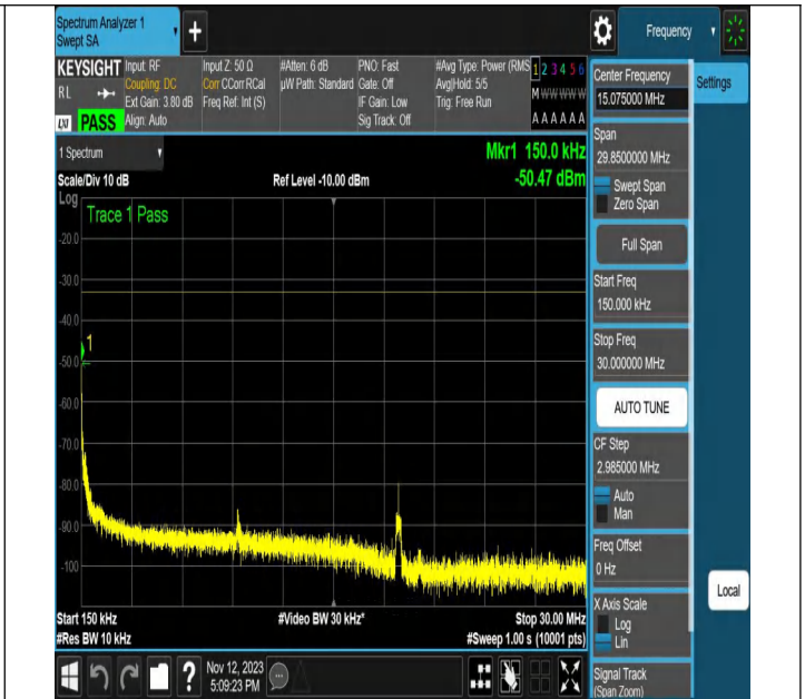
NTNV-N2-PC3-15-20-L-DFT-QPSK-Edge_1RB_Left-Ant1-PASS
