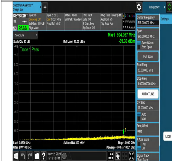
NTNV-N2-PC3-15-20-L-DFT-256QAM-Edge_1RB_Right-Ant1-P
