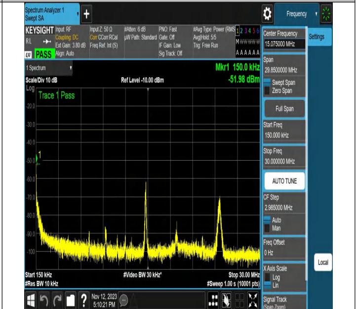
NTNV-N2-PC3-15-20-L-DFT-QPSK-Edge_1RB_Right-Ant1-PAS
