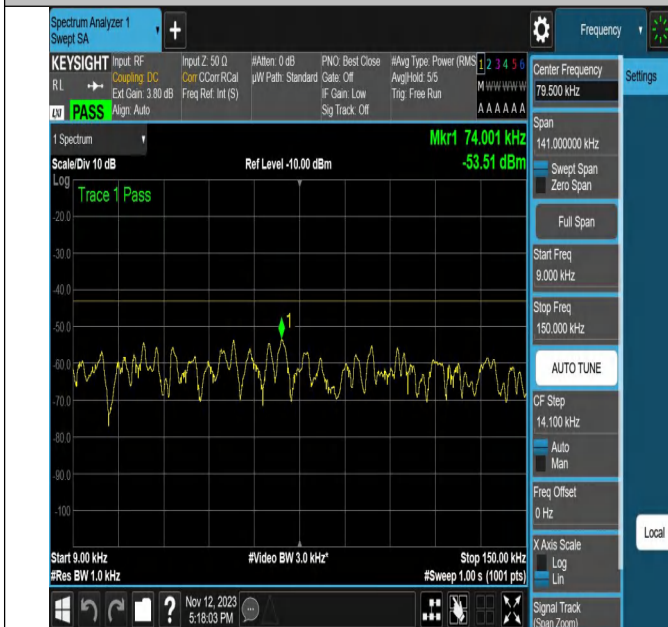
NTNV-N2-PC3-15-20-L-DFT-256QAM-Edge_1RB_Left-Ant1-PA
