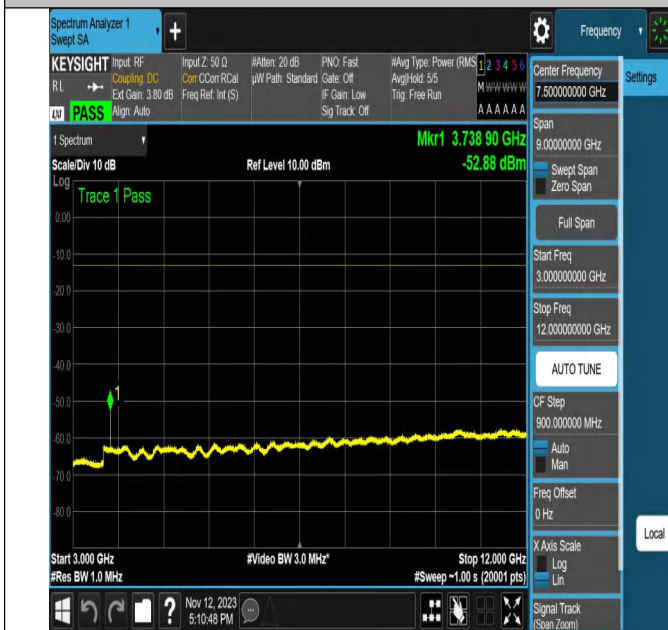
NTNV-N2-PC3-15-20-L-DFT-QPSK-Edge_1RB_Right-Ant1-PAS
