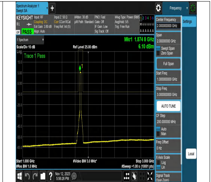
NTNV-N2-PC3-15-20-L-DFT-QPSK-Edge_1RB_Right-Ant1-PAS
