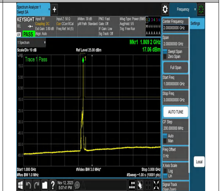
NTNV-N2-PC3-15-20-L-DFT-PI2BPSK-Edge_1RB_Right-Ant1-P ASS
