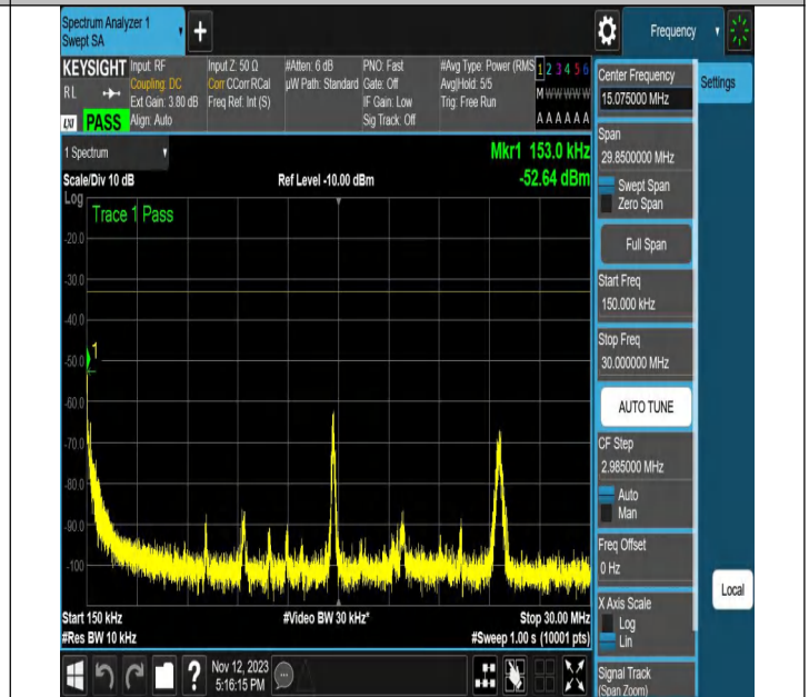
NTVN-N2-PC3-15-20-L-DFT-64QAM-Edge_1RB_Right-Ant1-PA
