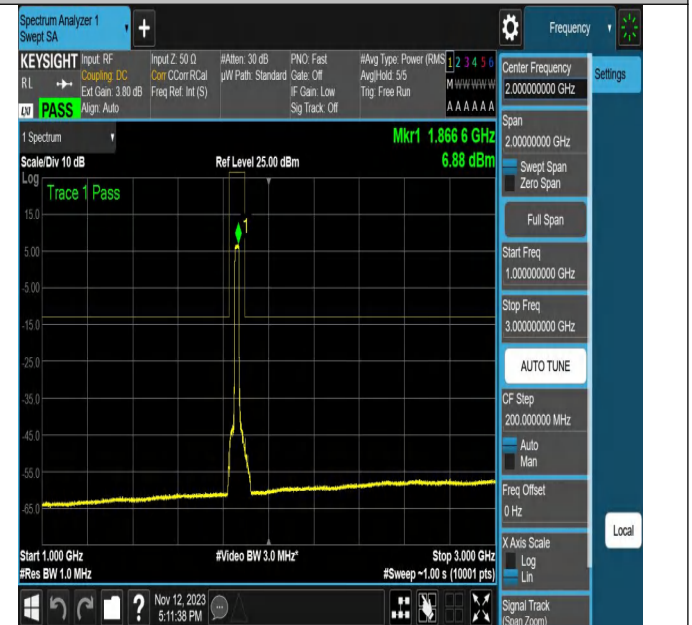
NTNV-N2-PC3-15-20-L-DFT-16QAM-Outer_Full-Ant1-PASS
