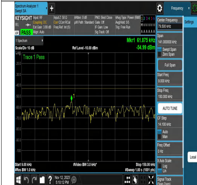
NTNV-N2-PC3-15-20-L-DFT-QPSK-Edge_1RB_Right-Ant1-PAS
