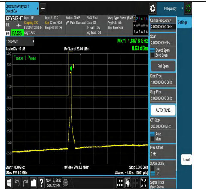
NTNV-N2-PC3-15-20-L-DFT-QPSK-Outer_Full-Ant1-PASS
