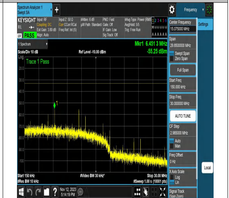
NTNV-N2-PC3-15-20-L-DFT-64QAM-Outer_Full-Ant1-PASS
