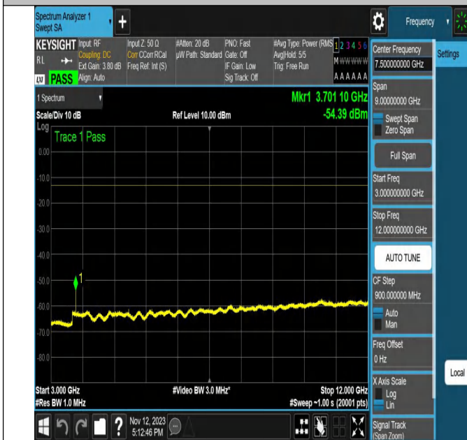
NTVN-N2-PC3-15-20-L-DFT-16QAM-Edge_1RB_Left-Ant1-PAS
