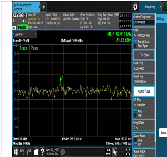
NTNV-N2-PC3-15-20-L-DFT-QPSK-Edge_1RB_Left-Ant1-PASS
