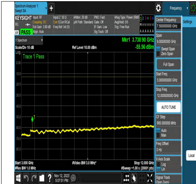
NTVN-N2-PC3-15-20-L-DFT-PI2BPSK-Edge_1RB_Right-Ant1-P ASS
