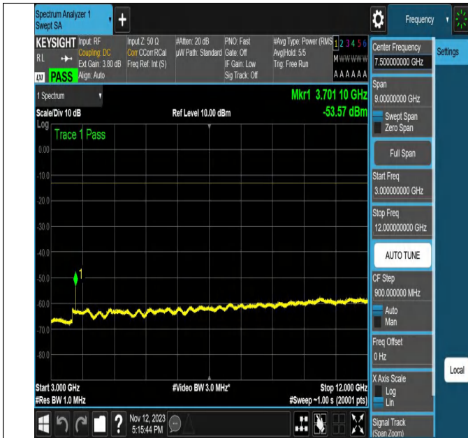
NTVN-N2-PC3-15-20-L-DFT-64QAM-Edge_1RB_Left-Ant1-PAS
