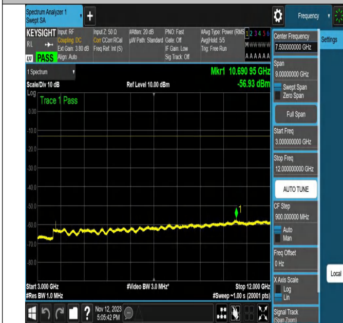
NTVN-N2-PC3-15-20-L-DFT-PI2BPSK-Edge_1RB_Left-Ant1-PA
