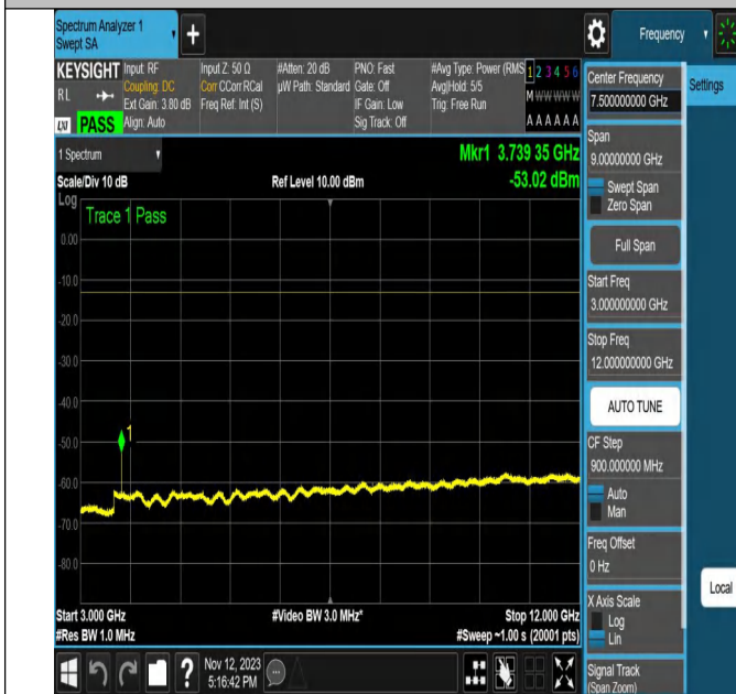
NTNV-N2-PC3-15-20-L-DFT-64QAM-Edge_1RB_Right-Ant1-PA
