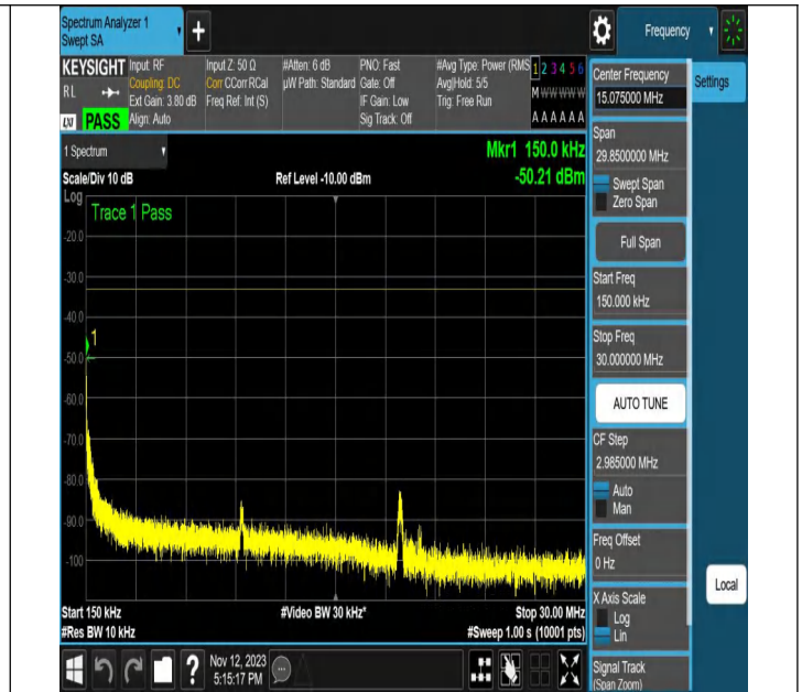
NTNV-N2-PC3-15-20-L-DFT-64QAM-Edge_1RB_Left-Ant1-PAS
