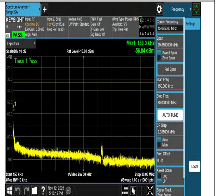
NTNV-N2-PC3-15-20-L-DFT-256QAM-Edge_1RB_Left-Ant1-PA
