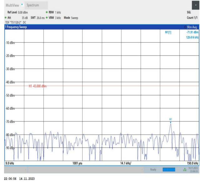
Band66_15MHz_16QAM_132047_1RB#0_0.009~0.15_0.009~0.15
