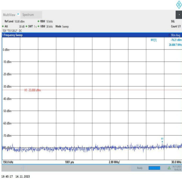
Band66_1.4MHz_16QAM_132665_1RB#0_0.15~30_0.15~30
