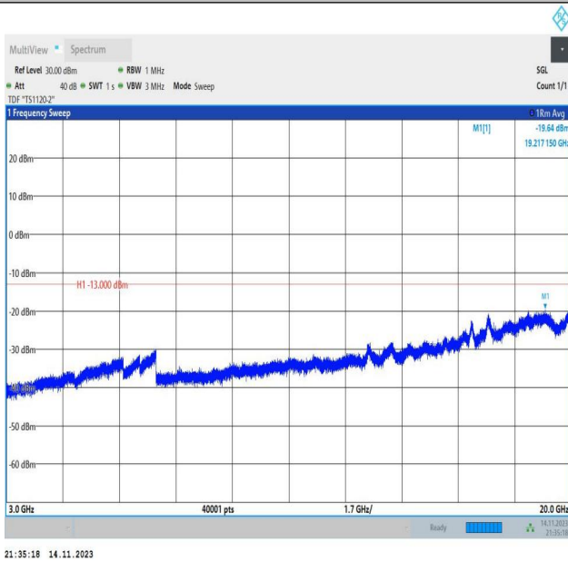
Band66_10MHz_QPSK_132022_1RB#0_3000~20000_3000~20000
