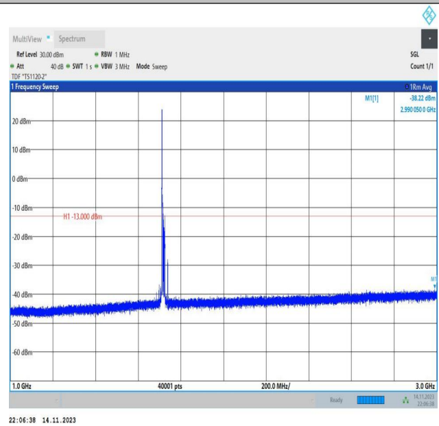
Band66_15MHz_QPSK_132047_1RB#0_1000~3000_1000~3000
