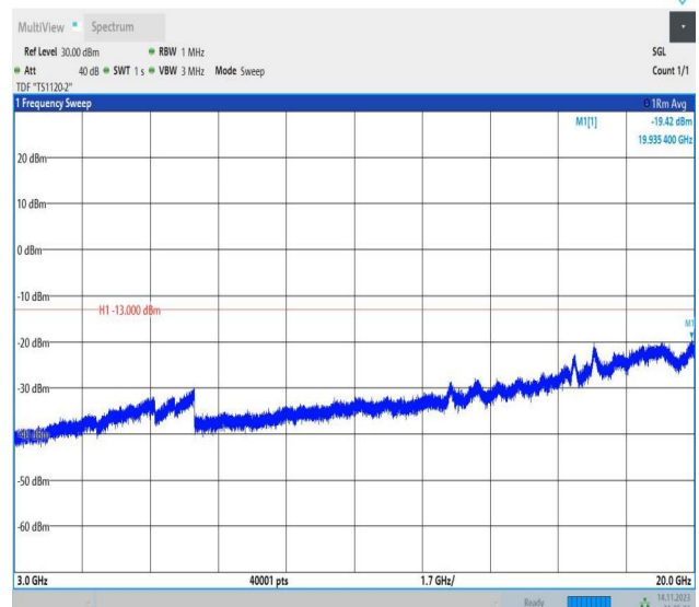
Band66_5MHz_16QAM_132322_1RB#0_3000~20000_3000~20000
