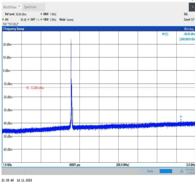
Band66_10MHz_16QAM_132022_1RB#0_1000~3000_1000~3000
