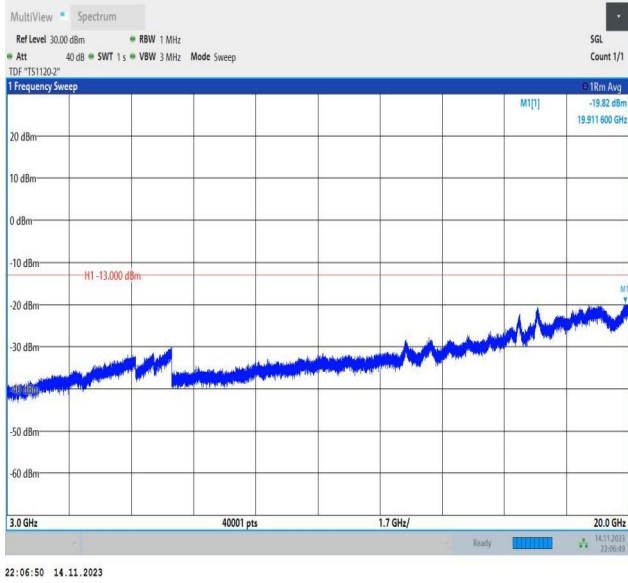
Band66_15MHz_QPSK_132047_1RB#0_3000~20000_3000~20000
