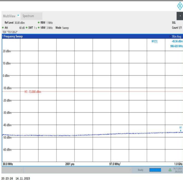
Band66_3MHz_QPSK_132322_1RB#0_30~1000_30~1000
