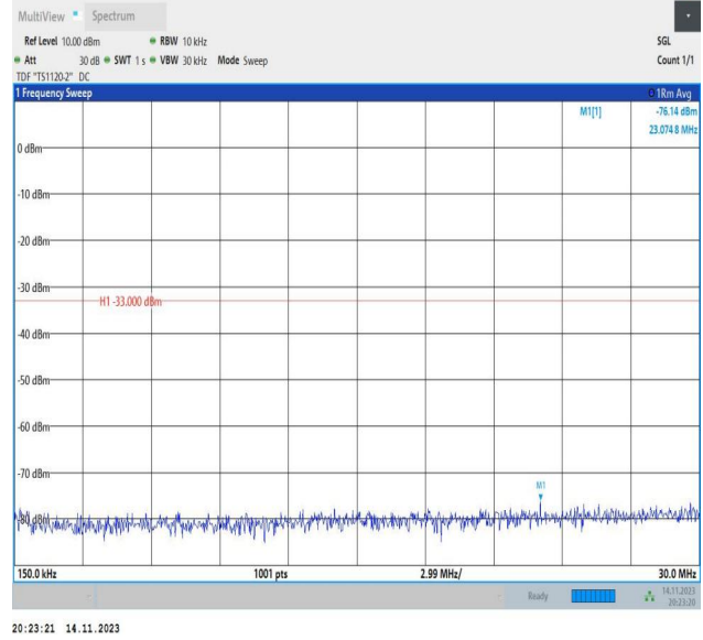
Band66_3MHz_QPSK_132322_1RB#0_0.15~30_0.15~30
