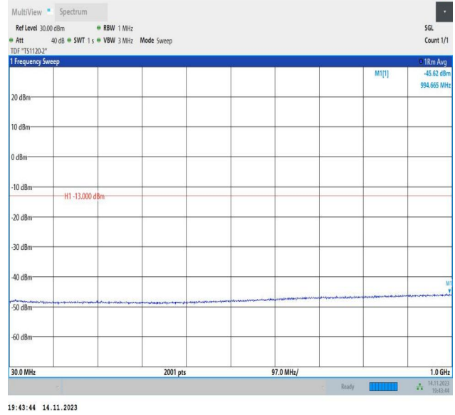
Band66_1.4MHz_16QAM_132322_1RB#0_30~1000_30~1000
