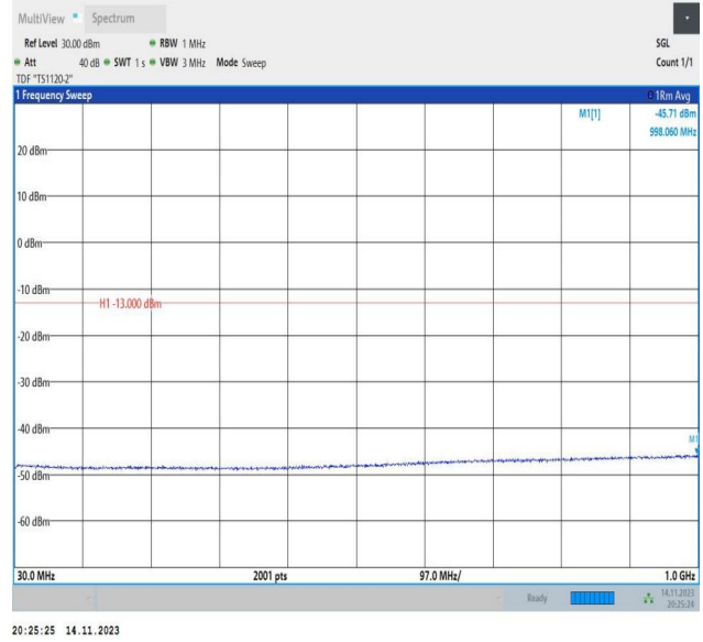
Band66_3MHz_16QAM_132657_1RB#0_30~1000_30~1000
