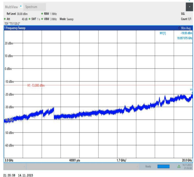
Band66_10MHz_16QAM_132022_1RB#0_3000~20000_3000~20000
