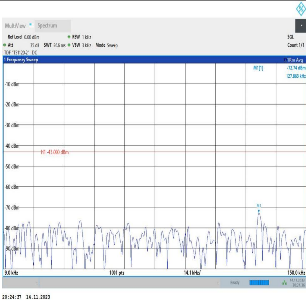
Band66_3MHz_QPSK_132657_1RB#0_0.009~0.15_0.009~0.15
