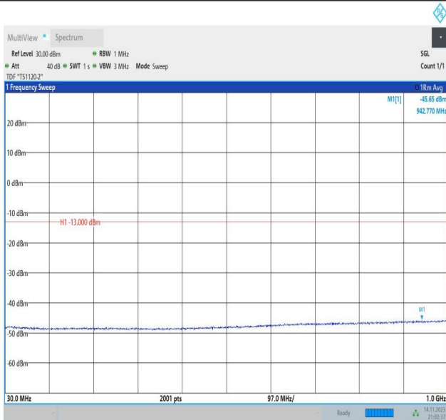
Band66_5MHz_QPSK_131997_1RB#0_30~1000_30~1000
