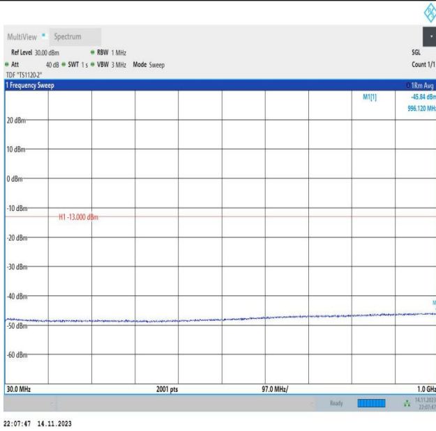
Band66_15MHz_QPSK_132322_1RB#0_30~1000_30~1000
