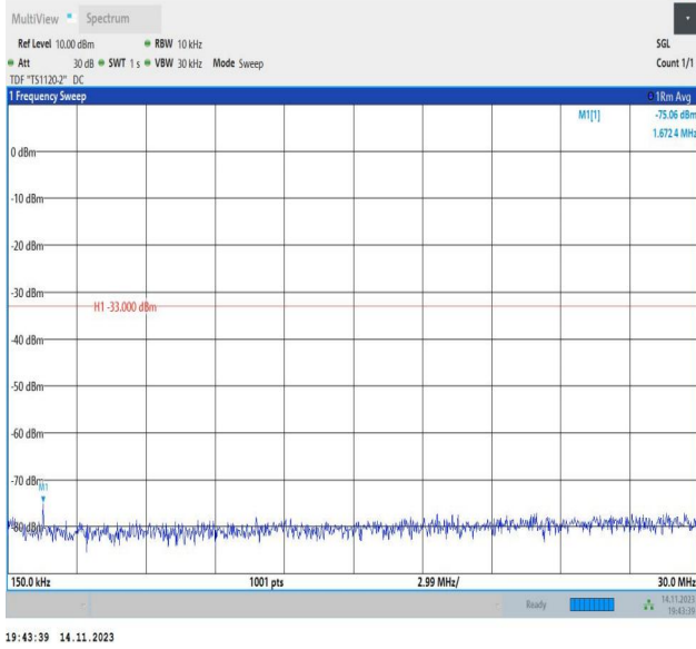
Band66_1.4MHz_16QAM_132322_1RB#0_0.15~30_0.15~30
