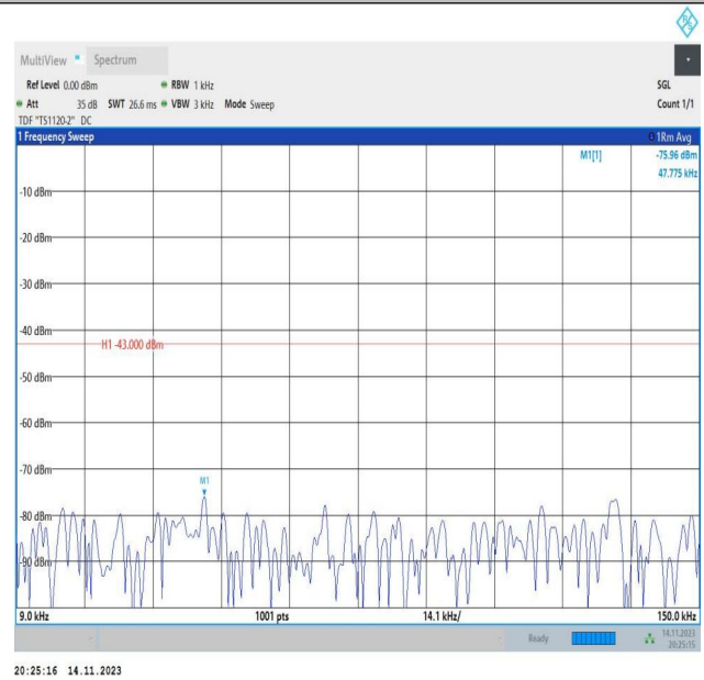
Band66_3MHz_16QAM_132657_1RB#0_0.009~0.15_0.009~0.15 15
