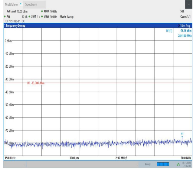
Band66_5MHz_QPSK_131997_1RB#0_0.15~30_0.15~30
