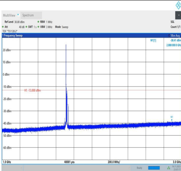
Band66_15MHz_16QAM_132047_1RB#0_1000~3000_1000~3000
