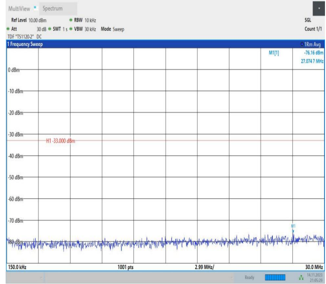
Band66_5MHz_QPSK_132647_1RB#0_0.15~30_0.15~30
