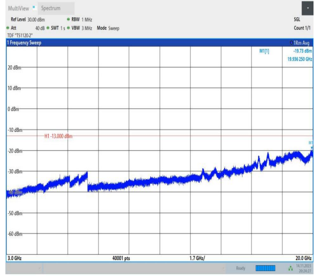
Band66_3MHz_16QAM_132322_1RB#0_3000~20000_3000~20000
