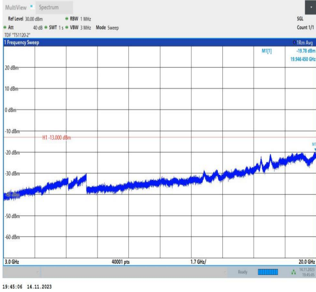
Band66_1.4MHz_QPSK_132665_1RB#0_3000~20000_3000~20000
