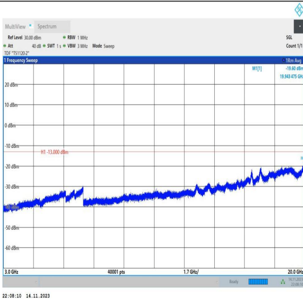
Band66_15MHz_QPSK_132322_1RB#0_3000~20000_3000~20000
