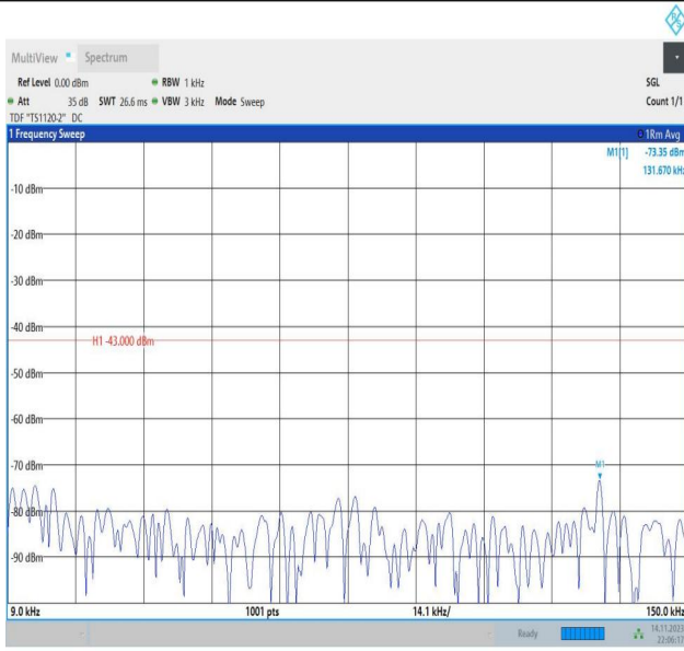
Band66_15MHz_QPSK_132047_1RB#0_0.009~0.15_0.009~0.15
