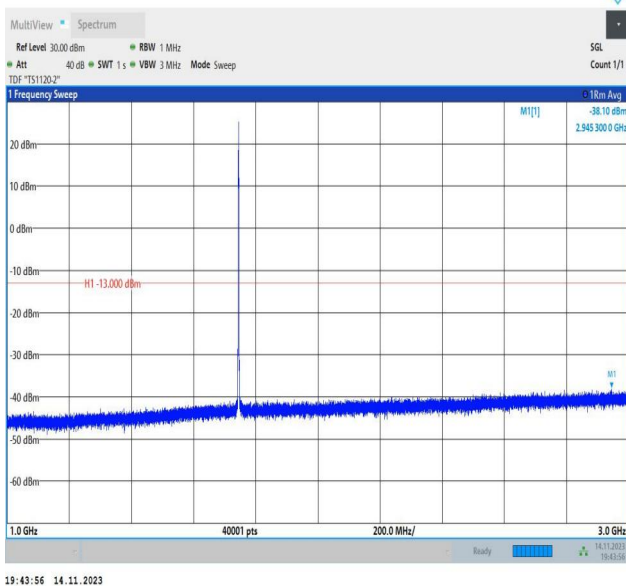
Band66_1.4MHz_16QAM_132322_1RB#0_1000~3000_1000~3000
