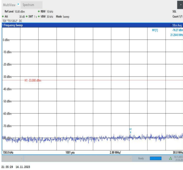
Band66_10MHz_16QAM_132022_1RB#0_0.15~30_0.15~30
