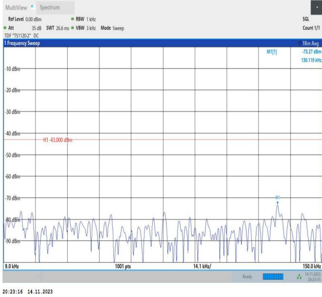
Band66_3MHz_QPSK_132322_1RB#0_0.009~0.15_0.009~0.
