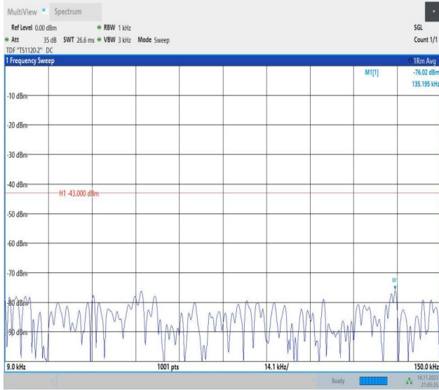
Band66_5MHz_QPSK_132647_1RB#0_0.009~0.15_0.009~0.
