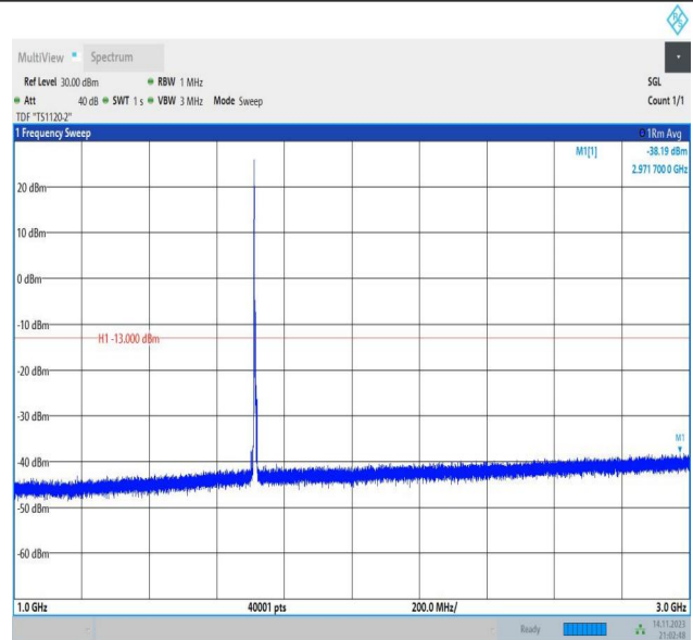
Band66_5MHz_QPSK_131997_1RB#0_1000~3000_1000~300
