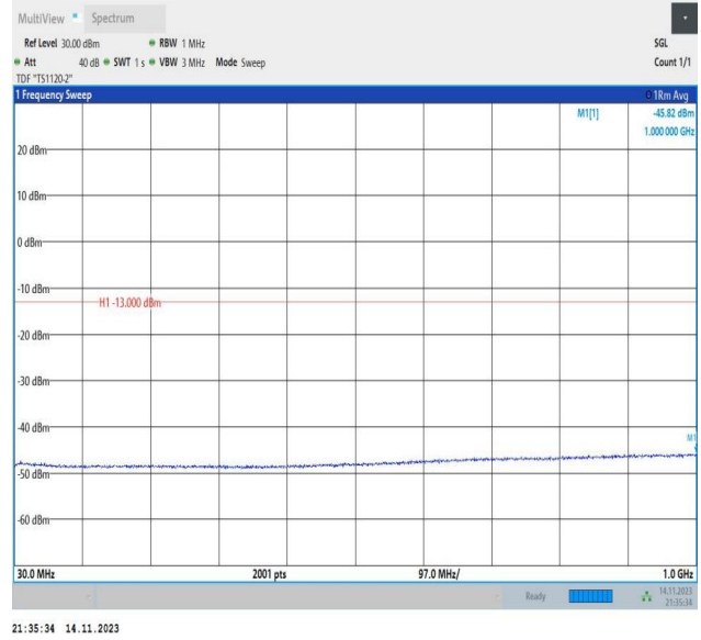
Band66_10MHz_16QAM_132022_1RB#0_30~1000_30~1000
