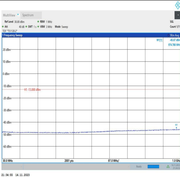
Band66_10MHz_QPSK_132022_1RB#0_30~1000_30~1000
