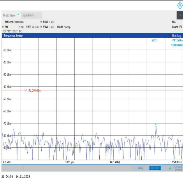
Band66_5MHz_QPSK_132322_1RB#0_0.009~0.15_0.009~0.15
