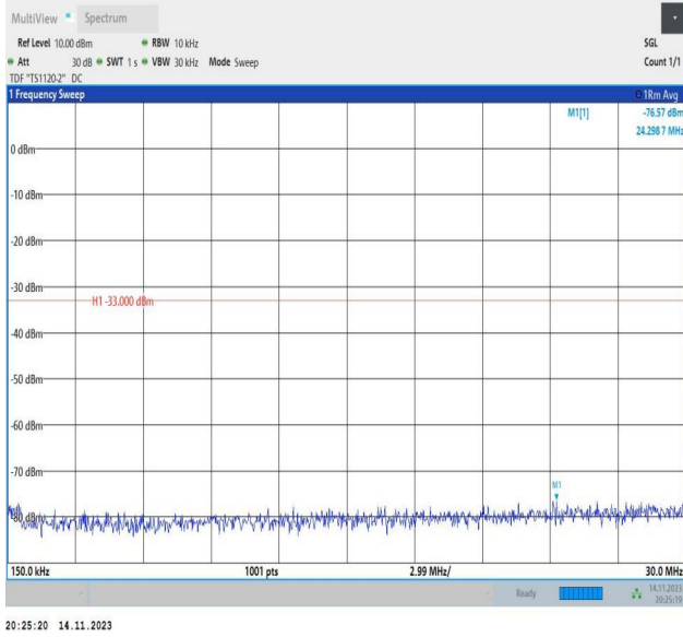
Band66_3MHz_16QAM_132657_1RB#0_0.15~30_0.15~30
