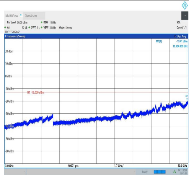
Band66_15MHz_16QAM_132047_1RB#0_3000~20000_3000~20000
