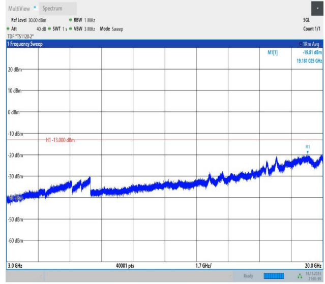
Band66_5MHz_16QAM_131997_1RB#0_3000~20000_3000~20000
