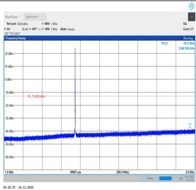
Band66_3MHz_QPSK_132322_1RB#0_1000~3000_1000~300
