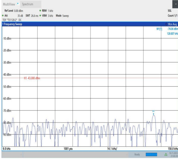
Band66_5MHz_QPSK_131997_1RB#0_0.009~0.15_0.009~0.
