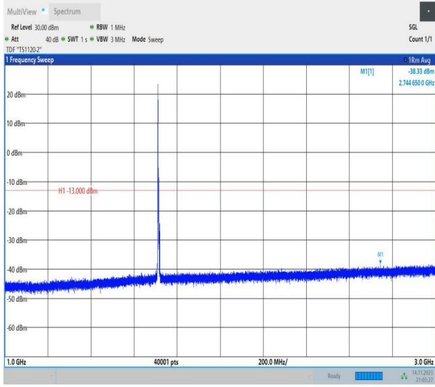
Band66_5MHz_16QAM_131997_1RB#0_1000~3000_1000~3000
