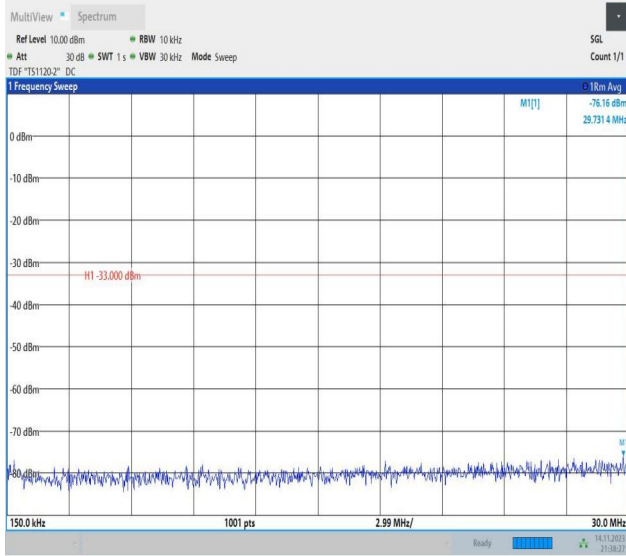
Band66_10MHz_16QAM_132622_1RB#0_0.15~30_0.15~30
