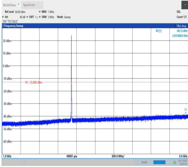
Band66_3MHz_16QAM_132322_1RB#0_1000~3000_1000~3000
