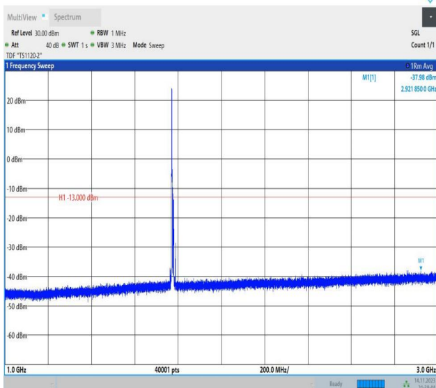
Band66_10MHz_16QAM_132622_1RB#0_1000~3000_1000~3000
