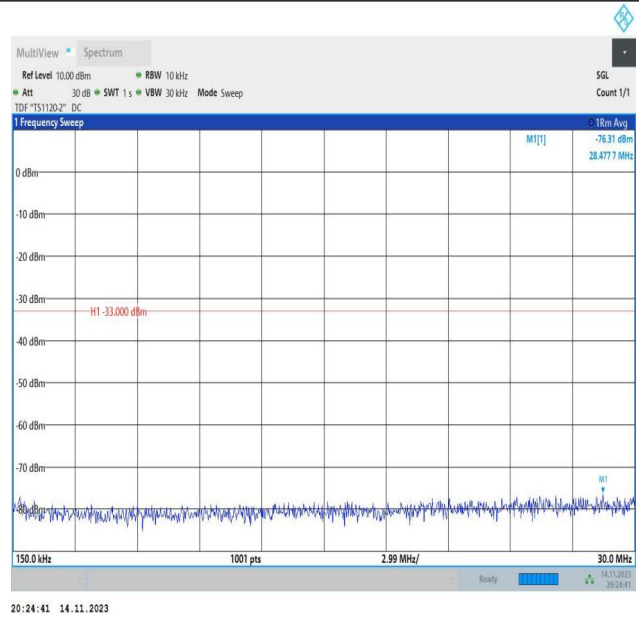
Band66_3MHz_QPSK_132657_1RB#0_0.15~30_0.15~30
