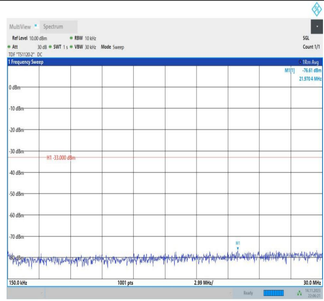
Band66_15MHz_QPSK_132047_1RB#0_0.15~30_0.15~30
