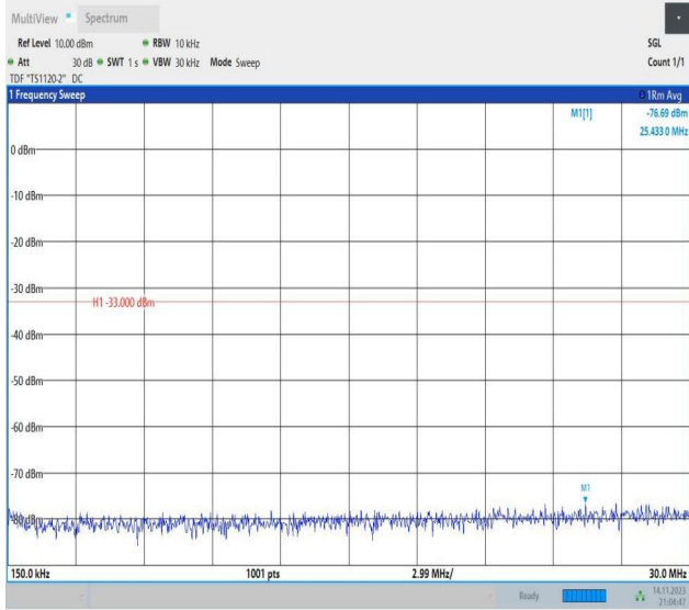
Band66_5MHz_16QAM_132322_1RB#0_0.15~30_0.15~30
