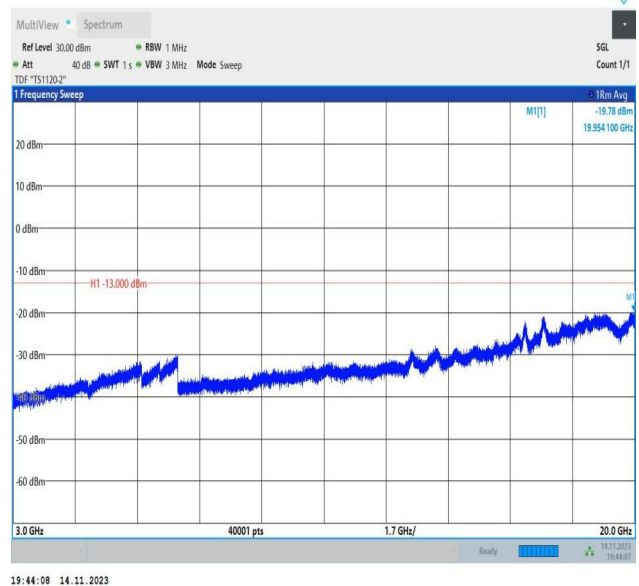
Band66_1.4MHz_16QAM_132322_1RB#0_3000~20000_3000~20000
