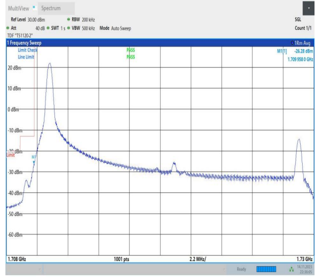
Band66_20MHz_16QAM_132072_1RB#0
