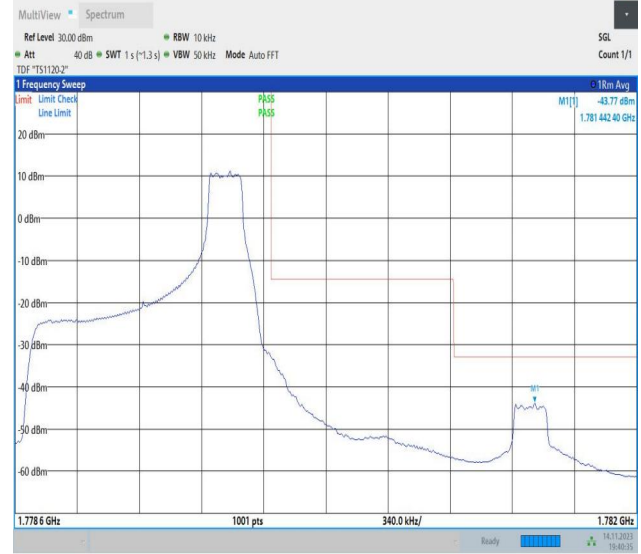
Band66_1.4MHz_16QAM_132665_1RB#5
