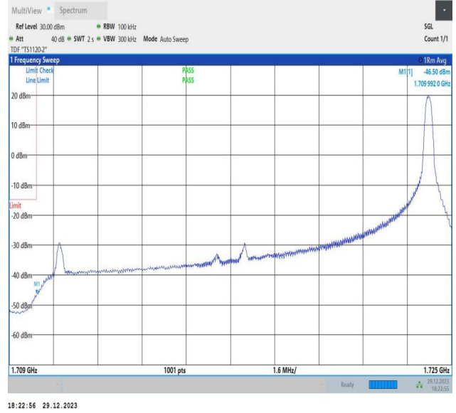
Band66_15MHz_64QAM_132047_1RB#74
