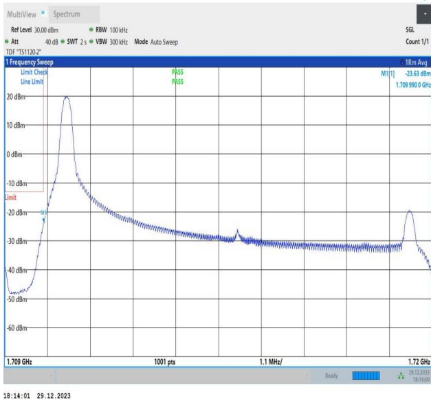
Band66_10MHz_64QAM_132022_1RB#0
