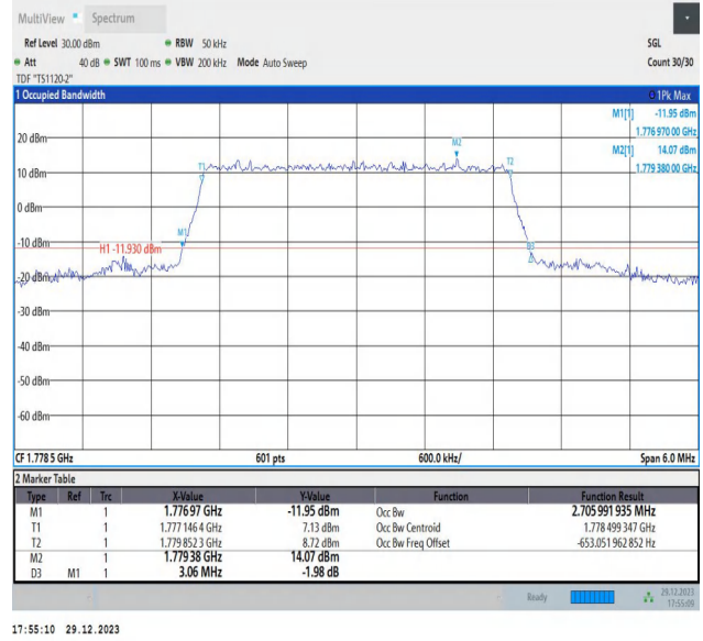
Band66-3MHz-64QAM-132657-15RB#0-PASS
