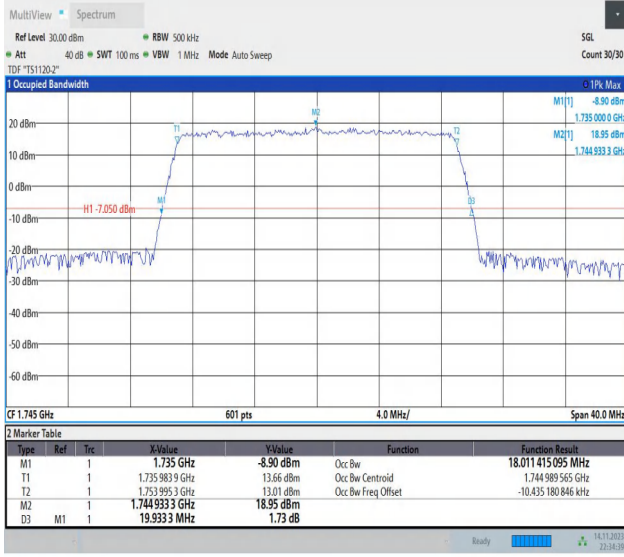
Band66-20MHz-QPSK-132322-100RB#0-PASS
