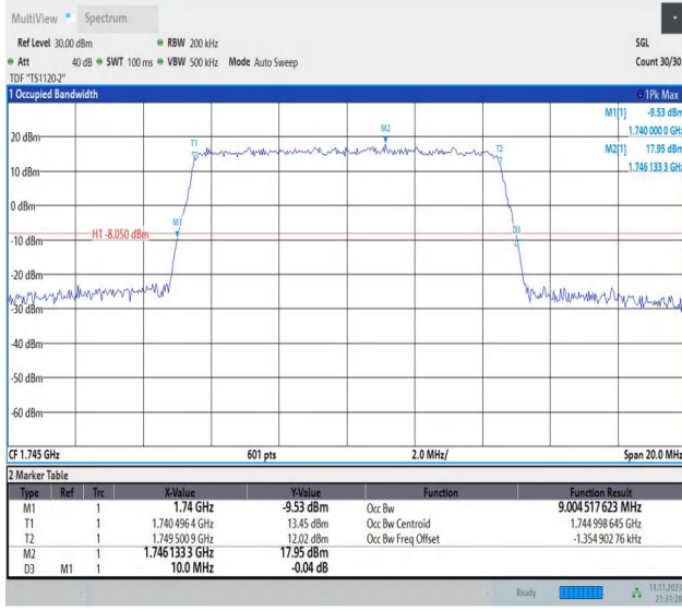
Band66-10MHz-QPSK-132322-50RB#0-PASS
