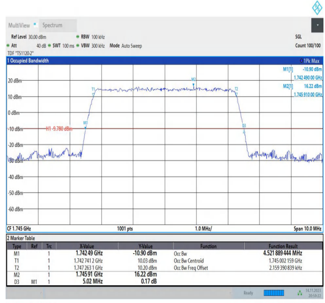
Band66-5MHz-16QAM-132322-25RB#0-PASS
