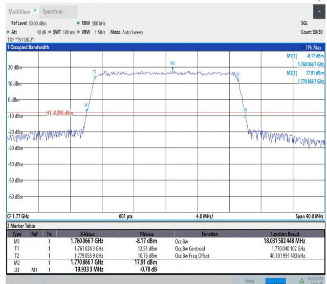
Band66-20MHz-16QAM-132572-100RB#0-PASS
