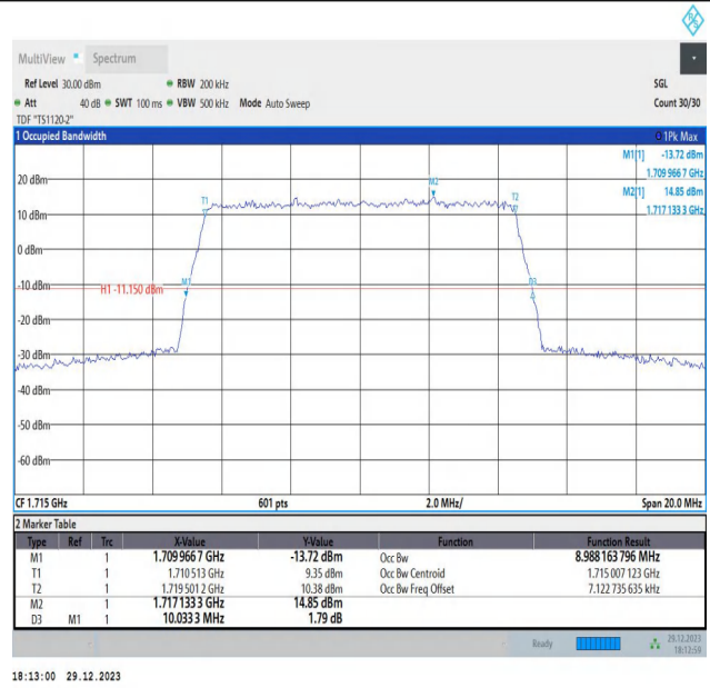
Band66-10MHz-64QAM-132022-50RB#0-PASS
