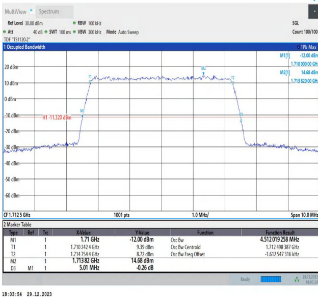
Band66-5MHz-64QAM-131997-25RB#0-PASS
