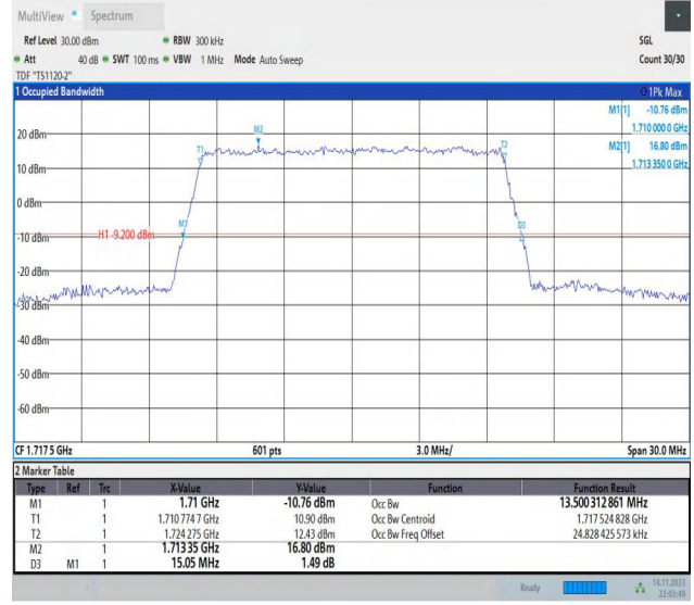
Band66-15MHz-16QAM-132047-75RB#0-PASS
