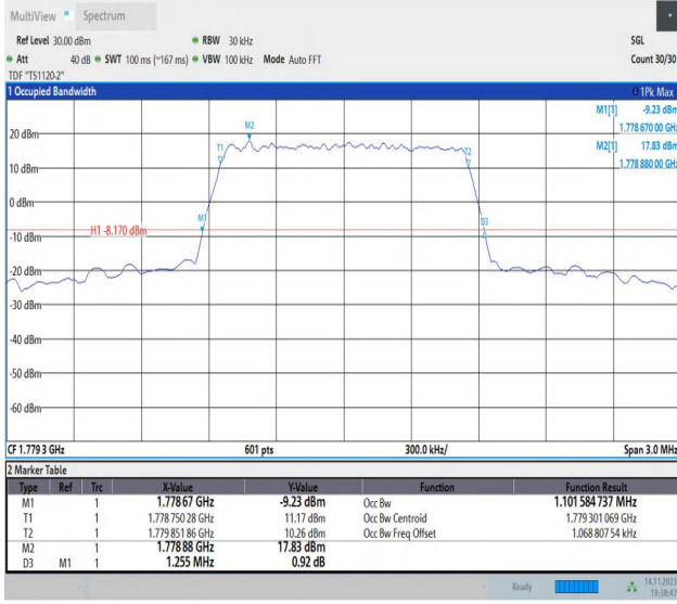
Band66-1.4MHz-QPSK-132665-6RB#0-PASS
