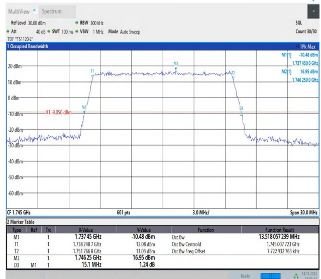
Band66-15MHz-16QAM-132322-75RB#0-PASS
