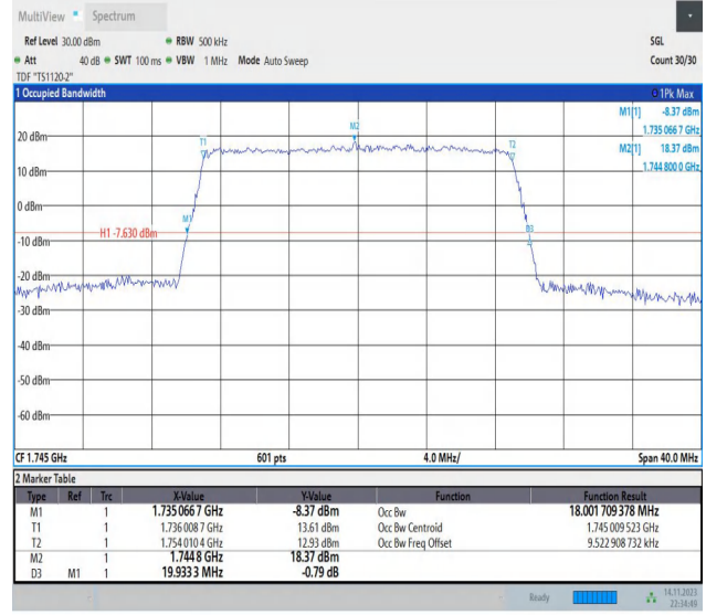
Band66-20MHz-16QAM-132322-100RB#0-PASS
