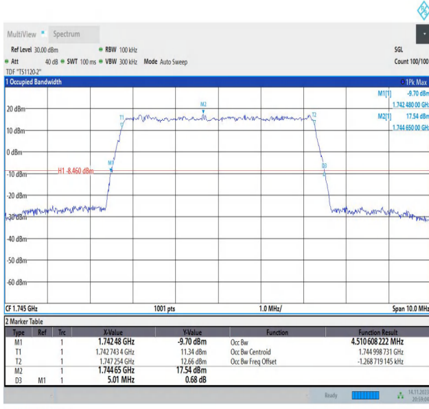
Band66-5MHz-QPSK-132322-25RB#0-PASS
