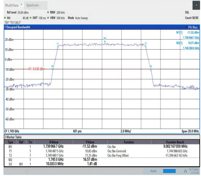
Band66-10MHz-16QAM-132322-50RB#0-PASS
