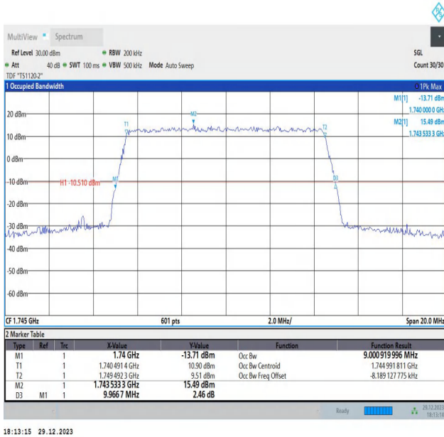
Band66-10MHz-64QAM-132322-50RB#0-PASS
