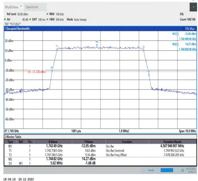
Band66-5MHz-64QAM-132322-25RB#0-PASS
