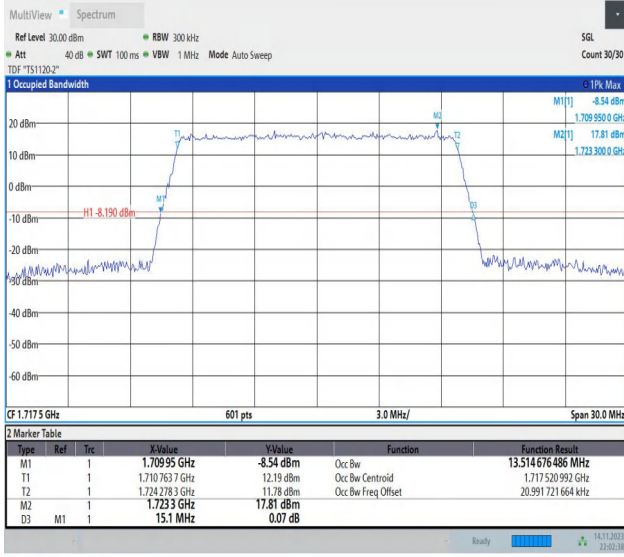
Band66-15MHz-QPSK-132047-75RB#0-PASS
