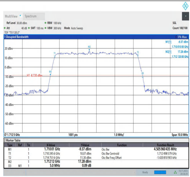
Band66-5MHz-16QAM-131997-25RB#0-PASS
