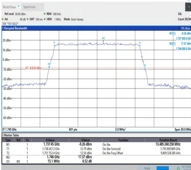
Band66-15MHz-QPSK-132322-75RB#0-PASS
