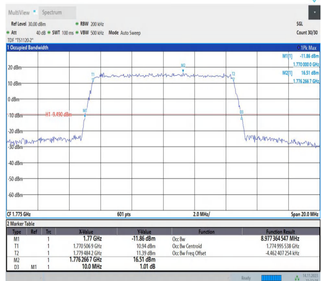
Band66-10MHz-16QAM-132622-50RB#0-PASS
