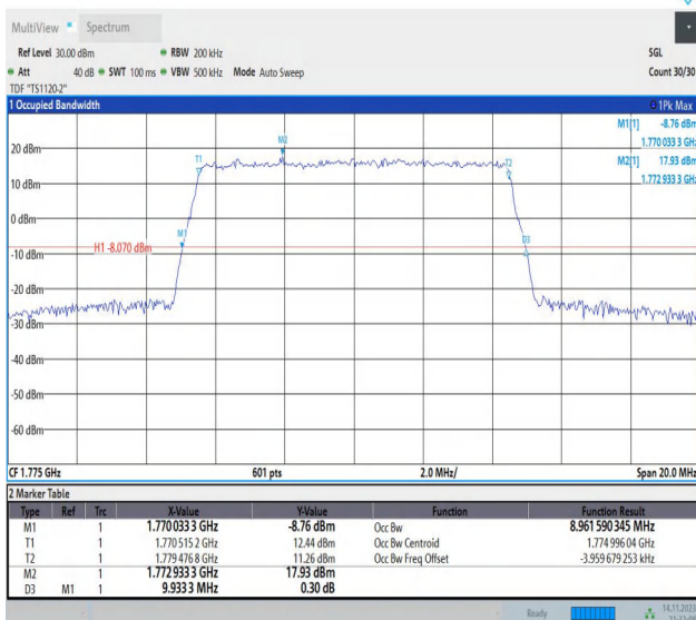
Band66-10MHz-QPSK-132622-50RB#0-PASS
