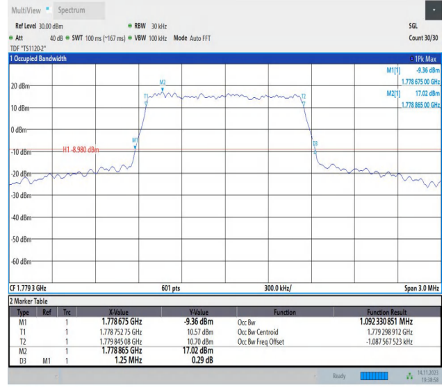
Band66-1.4MHz-16QAM-132665-6RB#0-PASS
