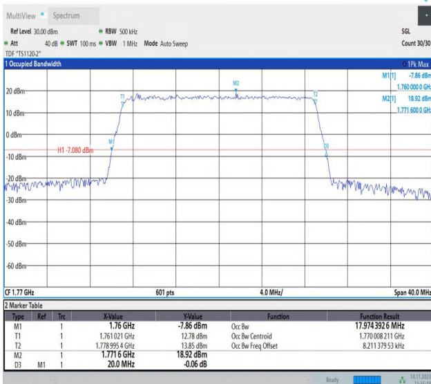
Band66-20MHz-QPSK-132572-100RB#0-PASS
