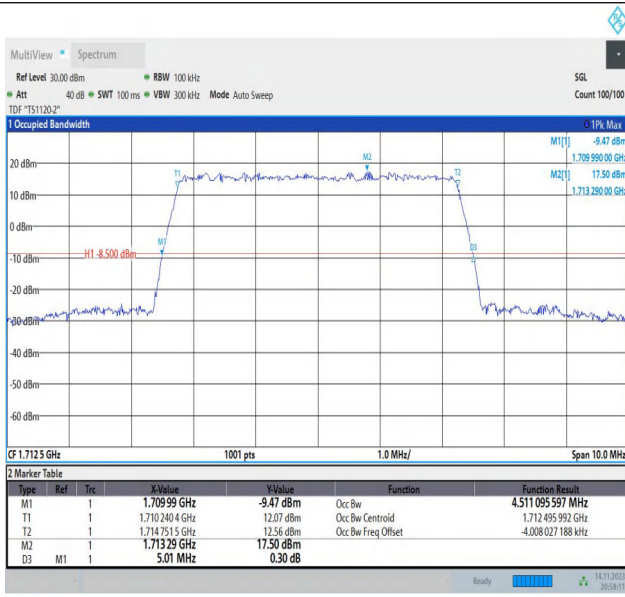
Band66-5MHz-QPSK-131997-25RB#0-PASS
