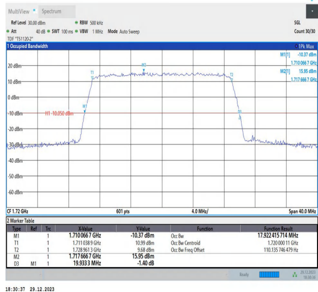
Band66-20MHz-64QAM-132072-100RB#0-PASS
